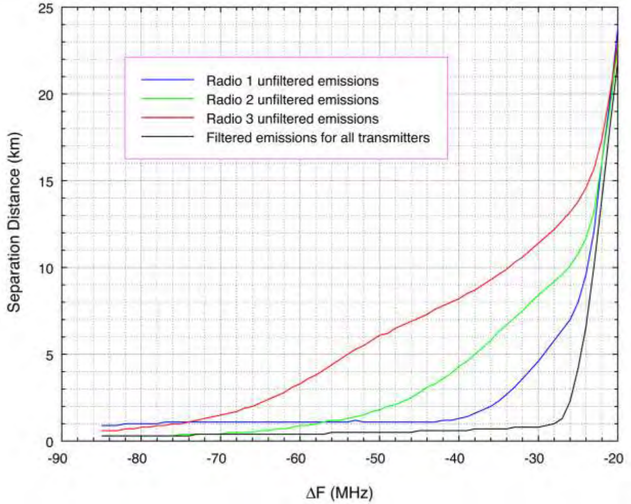
Figure D-10. Distance-frequency separation curves for ASR-8 and WiMAX, with WiMAX down-tilt angle = 0 degrees.
