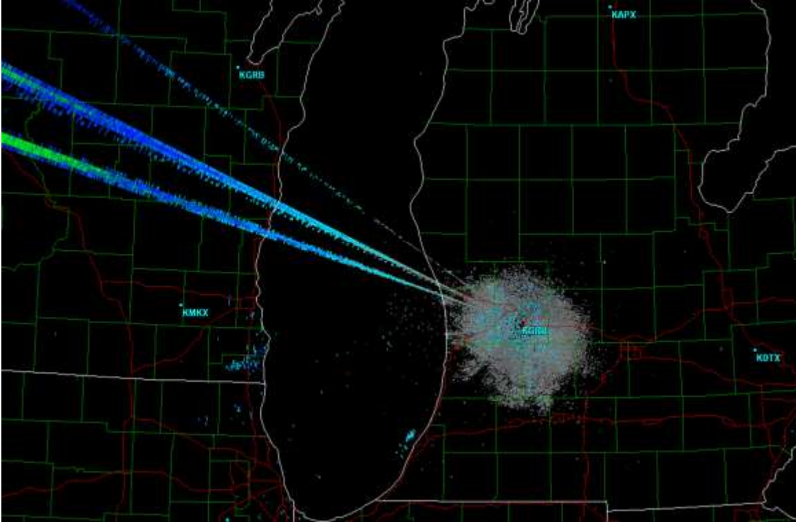
Figure 2. Strobes (three radial blue-and-green lines, compare to Figure 1) caused by interference in the Grand Rapids NEXRAD reflectivity data.
