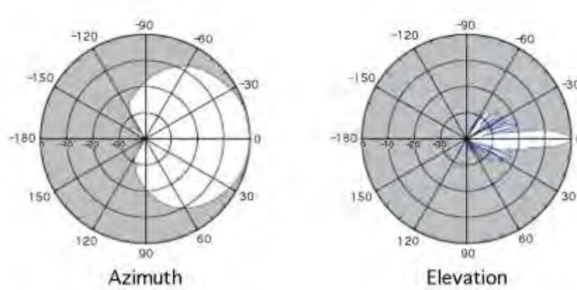
Figure 17. Antenna pattern of a typical WiMAX/LTE base station antenna, as measured by the manufacturer.
