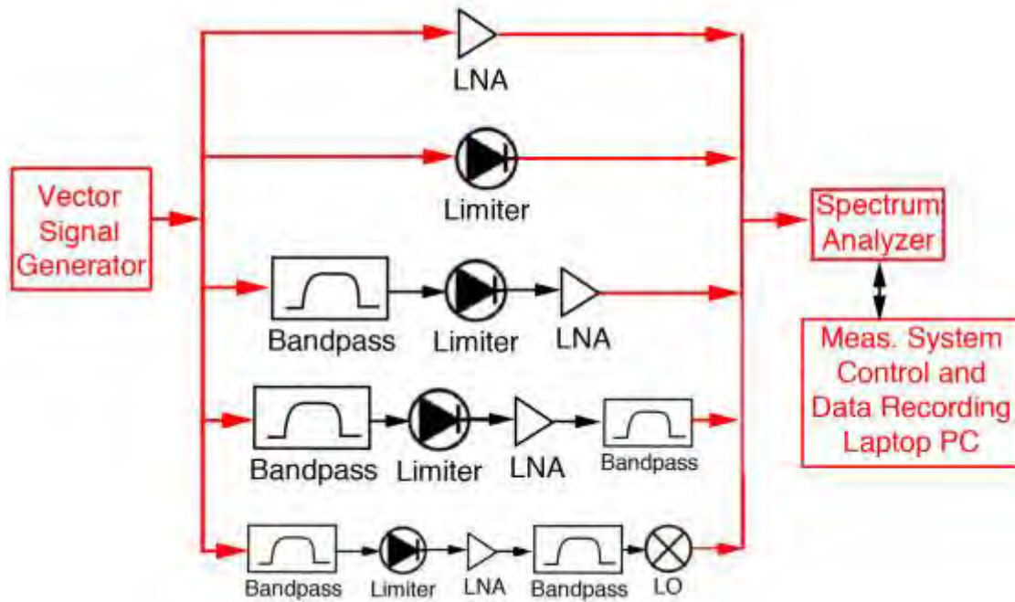
Figure 7. Schematic block diagram of NEXRAD receiver-component frequency-response characterization measurements. Measurement hardware is shown in red.
