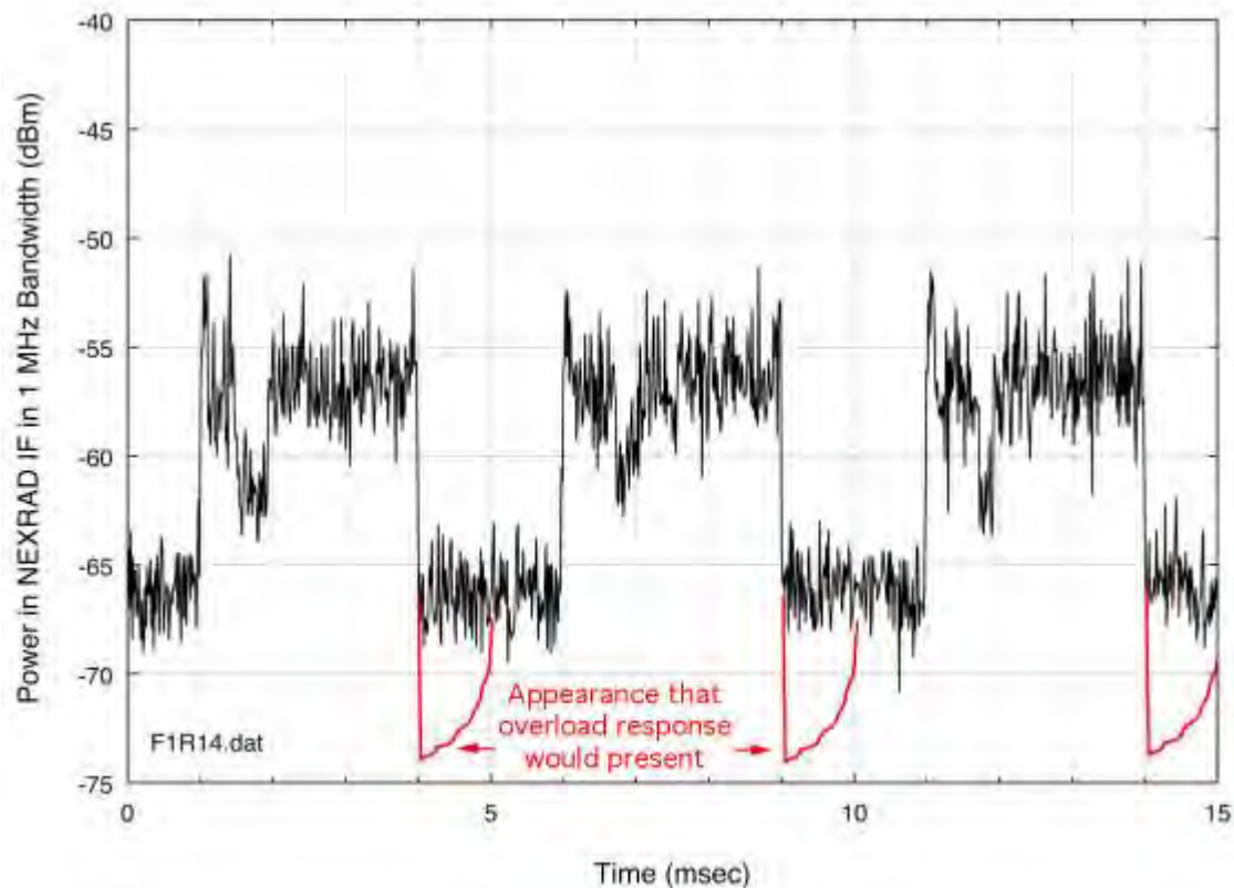
Figure 47. Top: Measured time-domain responses of an LNA in various amounts of overload, from [18]. Bottom: Data from Figure 40 as they would have appeared if the NEXRAD LNA had been compressed by front-end overload, with overload added graphically in red.
