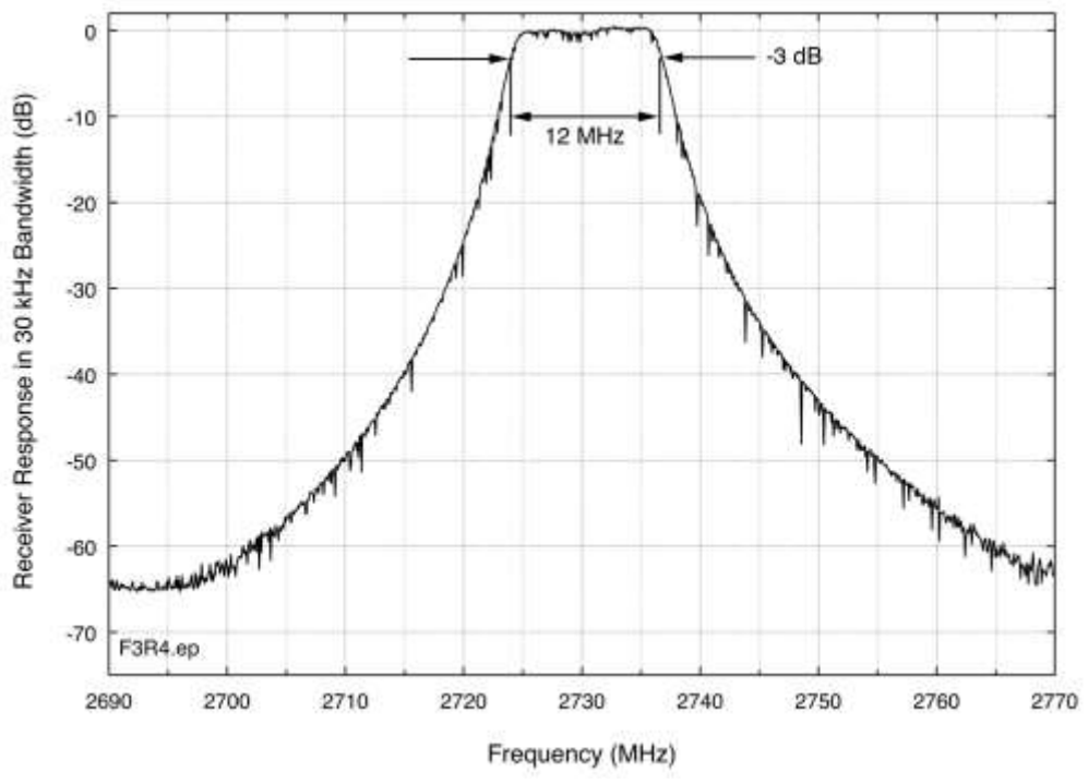
Figure C-13. ASR-9 receiver RF filter plus LNA response.
