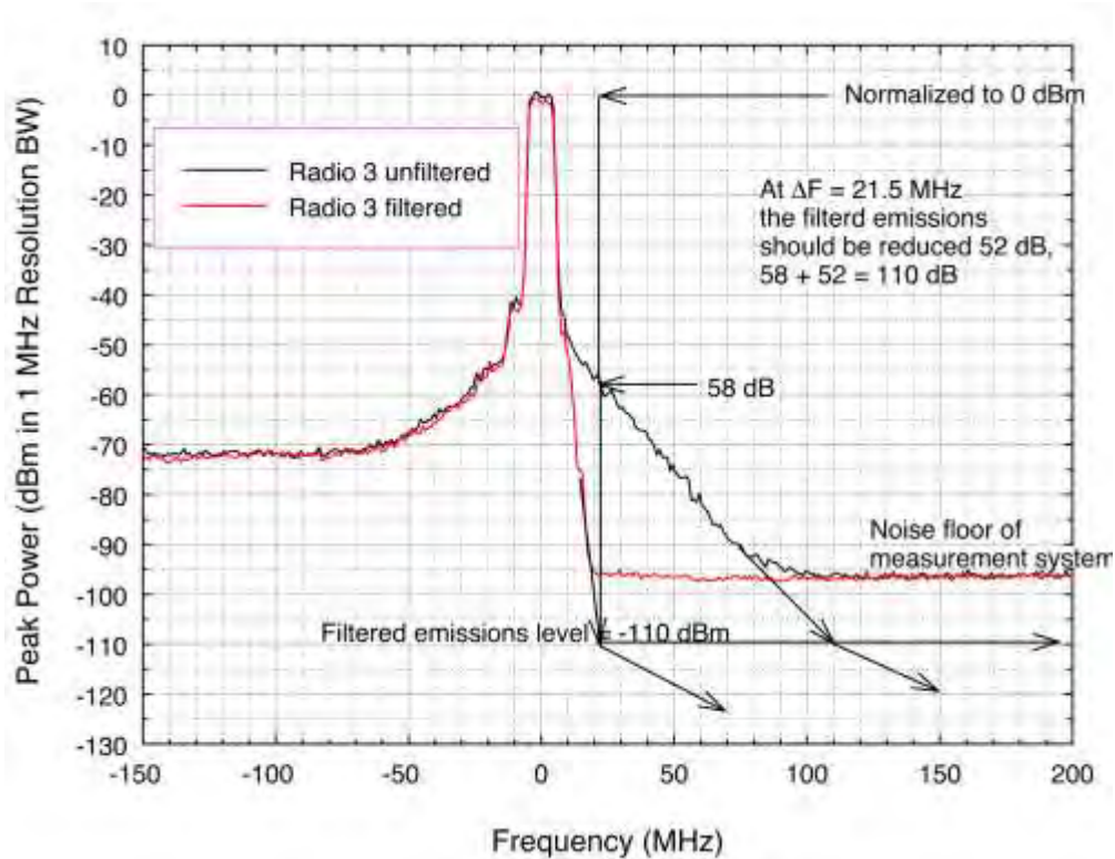
Figure 59. WiMAX Radio 3 emission spectra with and without output filtering.
