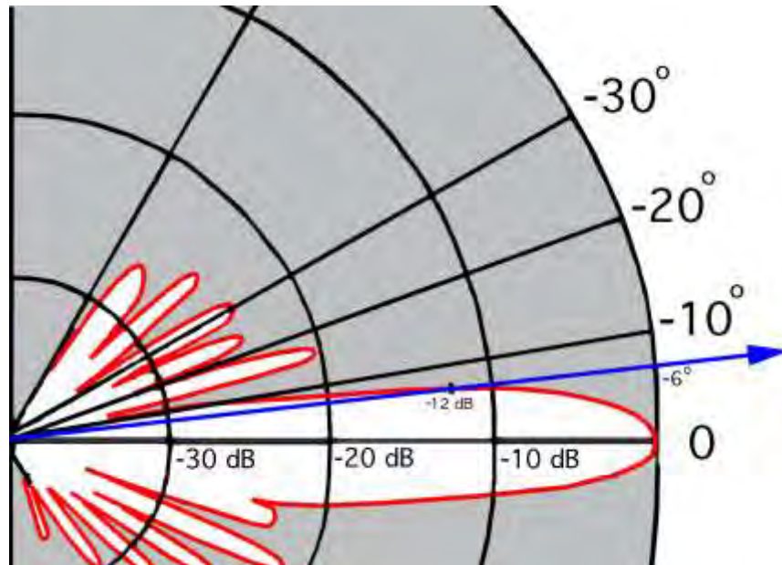
Figure 61. Detail of Figure 17, showing amount of down-tilt needed to achieve 12 dB of decoupling in the antenna pattern.
