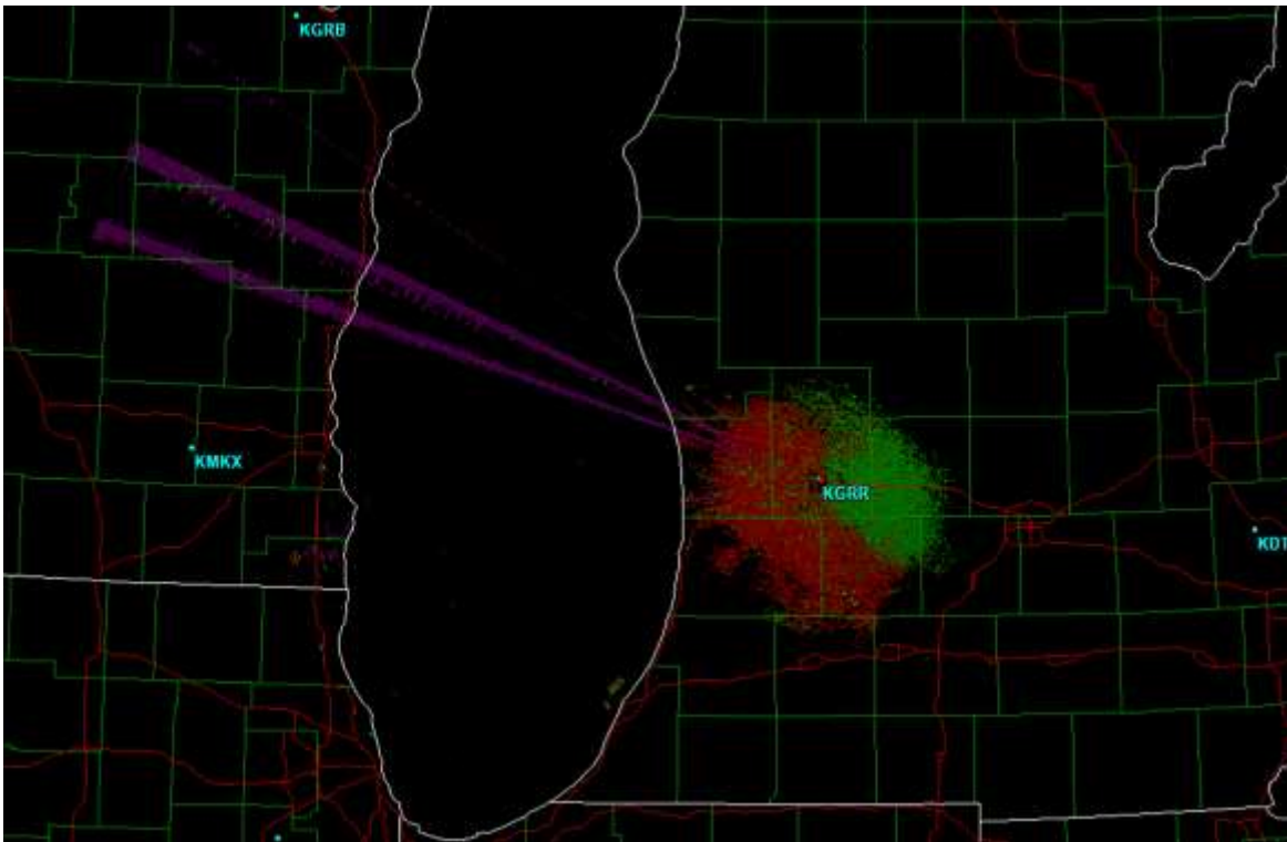
Figure 3. Strobes (two radial purple lines) in the Grand Rapids NEXRAD velocity data.
