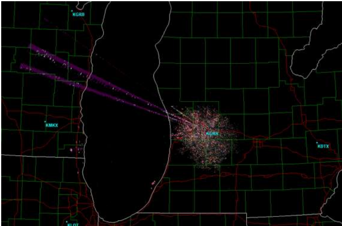
Figure 4. Strokes (two radial purple lines) in the Grand Rapids NEXRAD spectrum width data.
