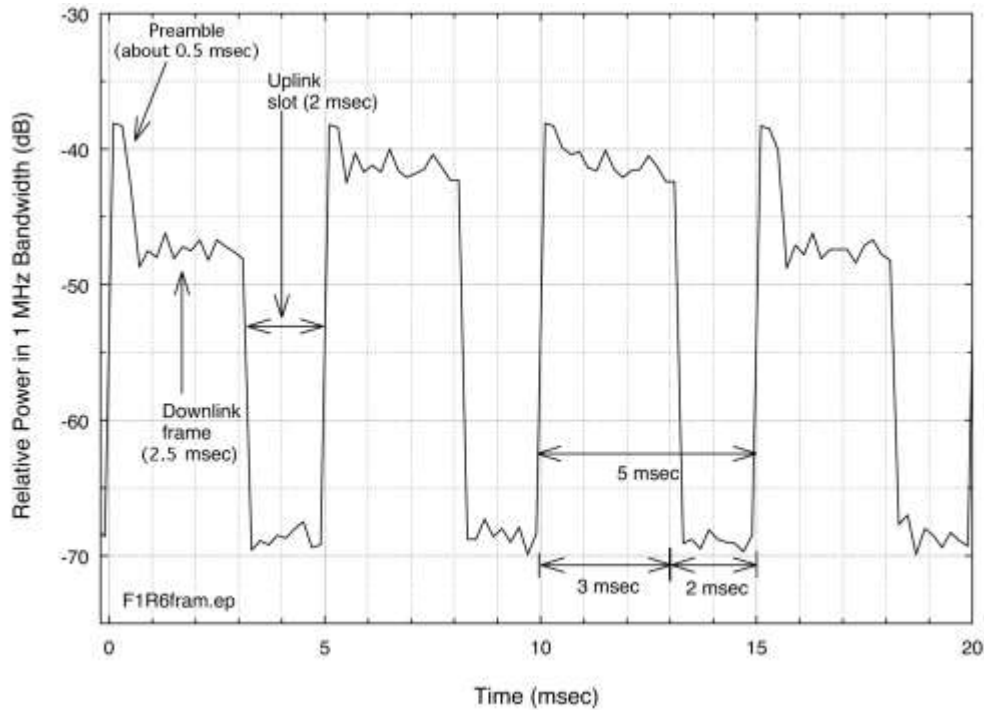
Figure 21. Measured time-domain characteristics of an operational BRS WiMAX base station signal. Preamble power is fixed while frame power levels vary.
