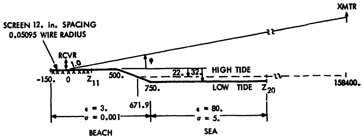
Figure 2. Geometry of Merrimac Light Coast Guard Station Sloping Beach Profile
