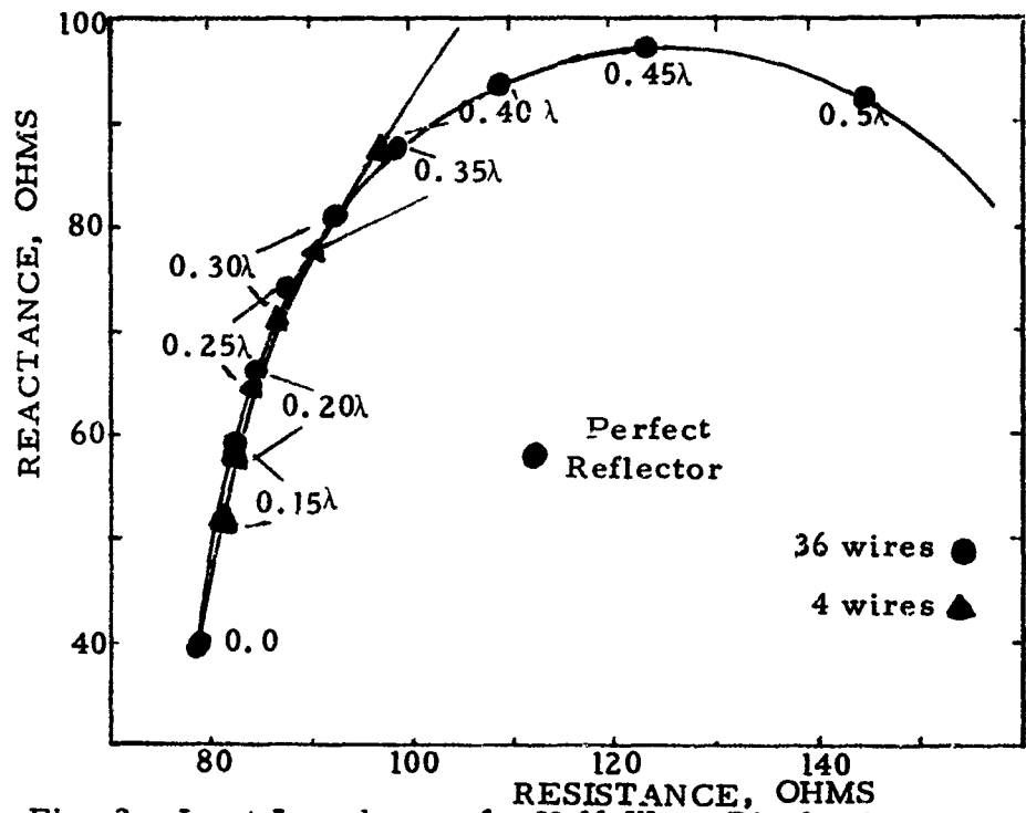
Fig. 2. Input Impedance of a Half-Wave Dipole Over a Radial Array of Wires of Varying Length.
