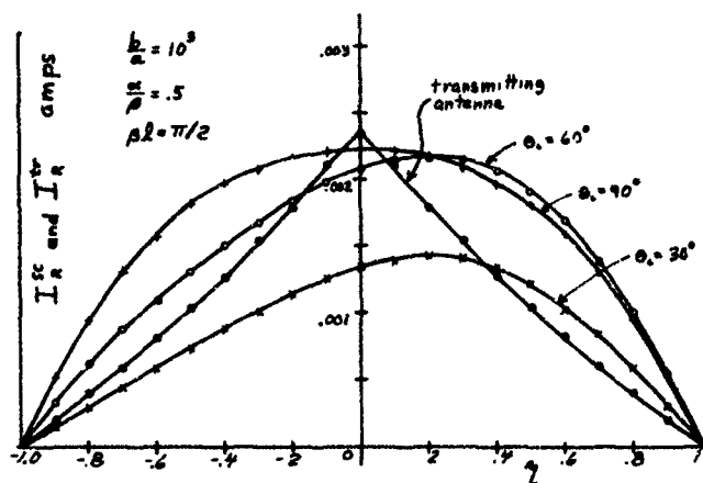
Short Circuit Current Dependence Upon Angle of Incidence ( E_0 = k volts/meter) and Transmitter Current for \alpha/\beta = .5 ( V_{gap} = 1 volt)
