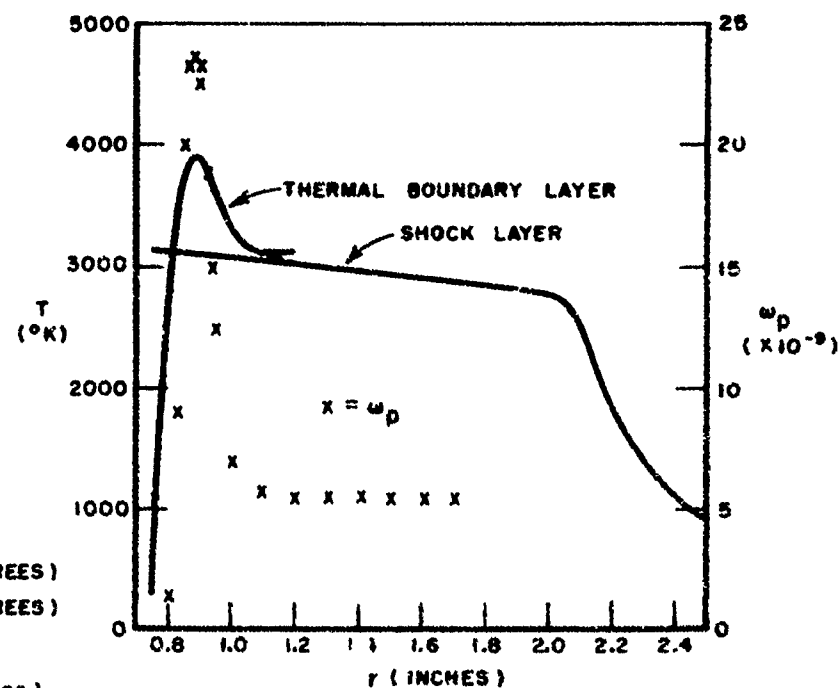
Fig. 6. RADIAL TEMPERATURE AND \omega_p PROFILES AT 140 kft, 2 INCHES FROM CYLINDER FACE.
