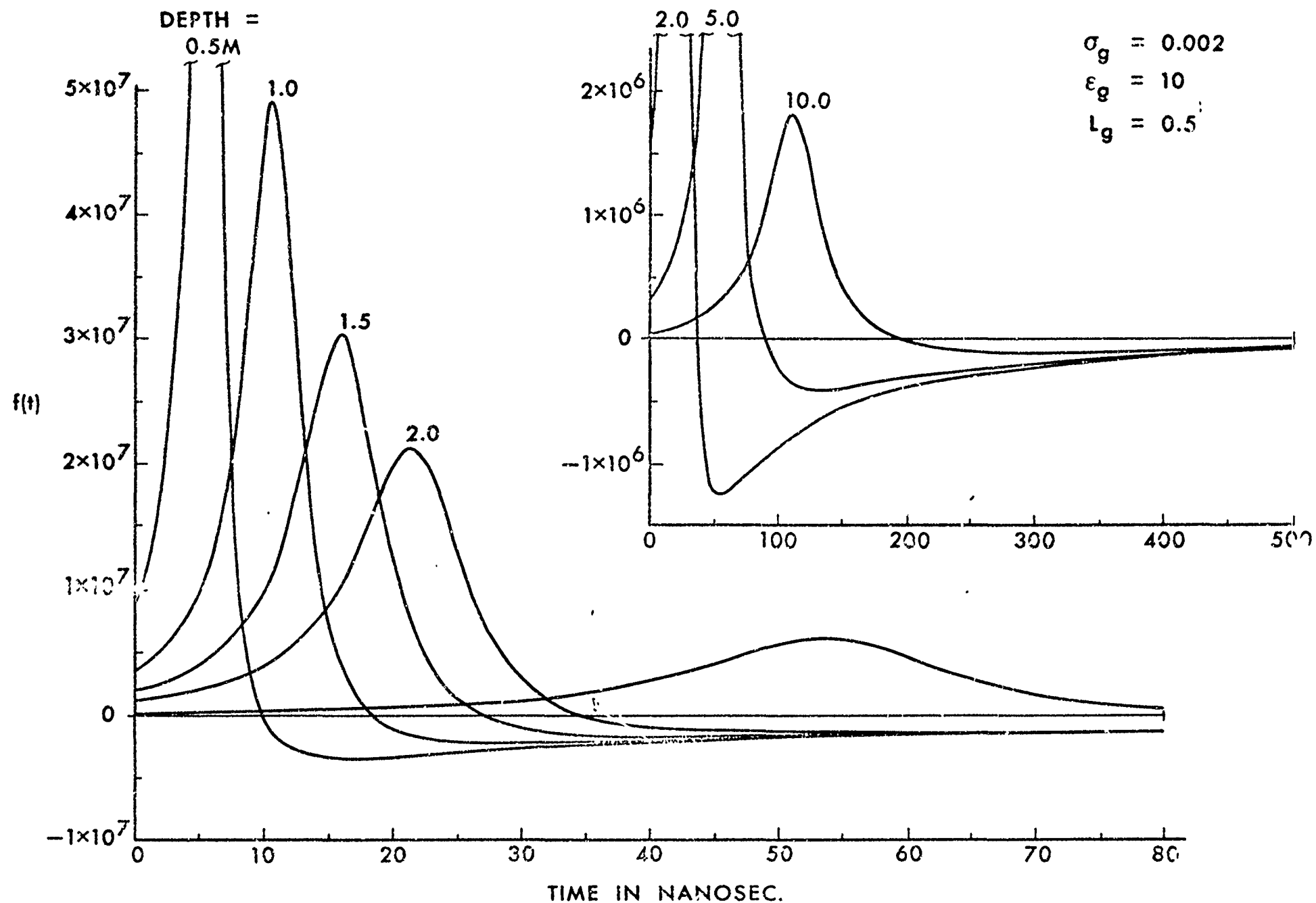
FIGURE 2: DELTA FUNCTION RESPONSE OF LOSSY EARTH AS A FUNCTION OF DEPTH
