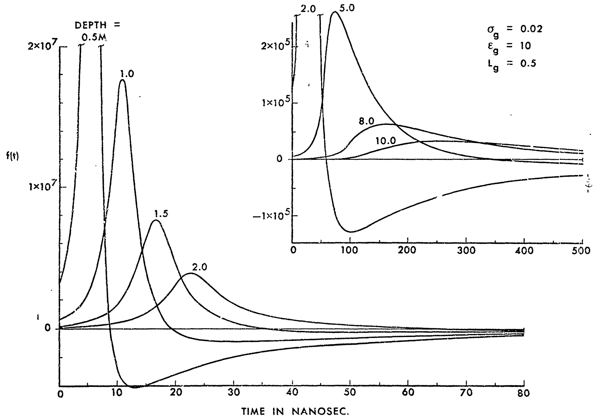
FIGURE 3: DELTA FUNCTION RESPONSE OF LOSSY EARTH AS A FUNCTION OF DEPTH
