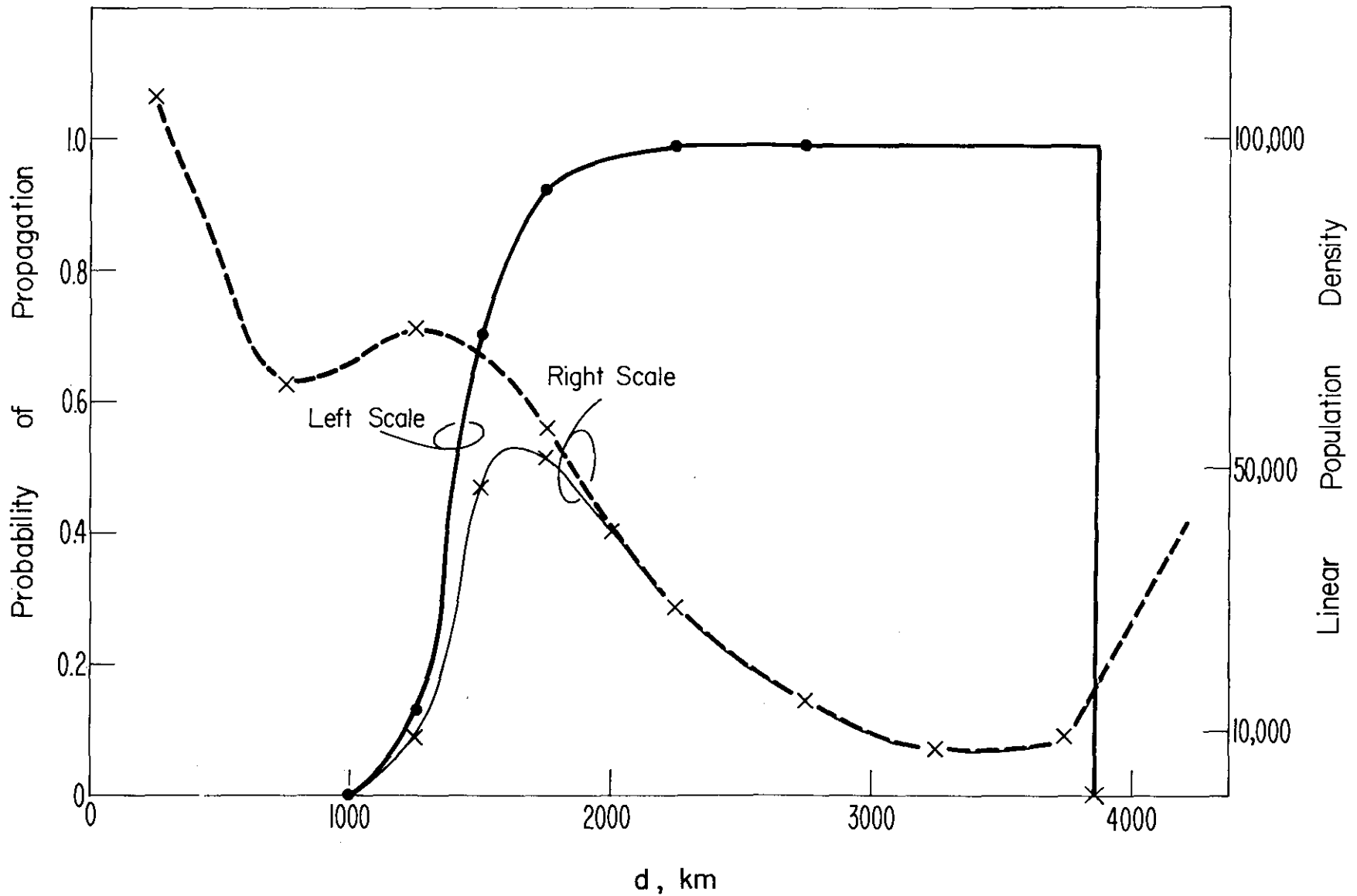
Figure B-6. Skywave propagation probability (heavy solid line) and population density (dashed line) as a function of distance from New York City. Propagation is for winter noon for sunspot number of 110. The lighter solid line is the product of the other two functions.
