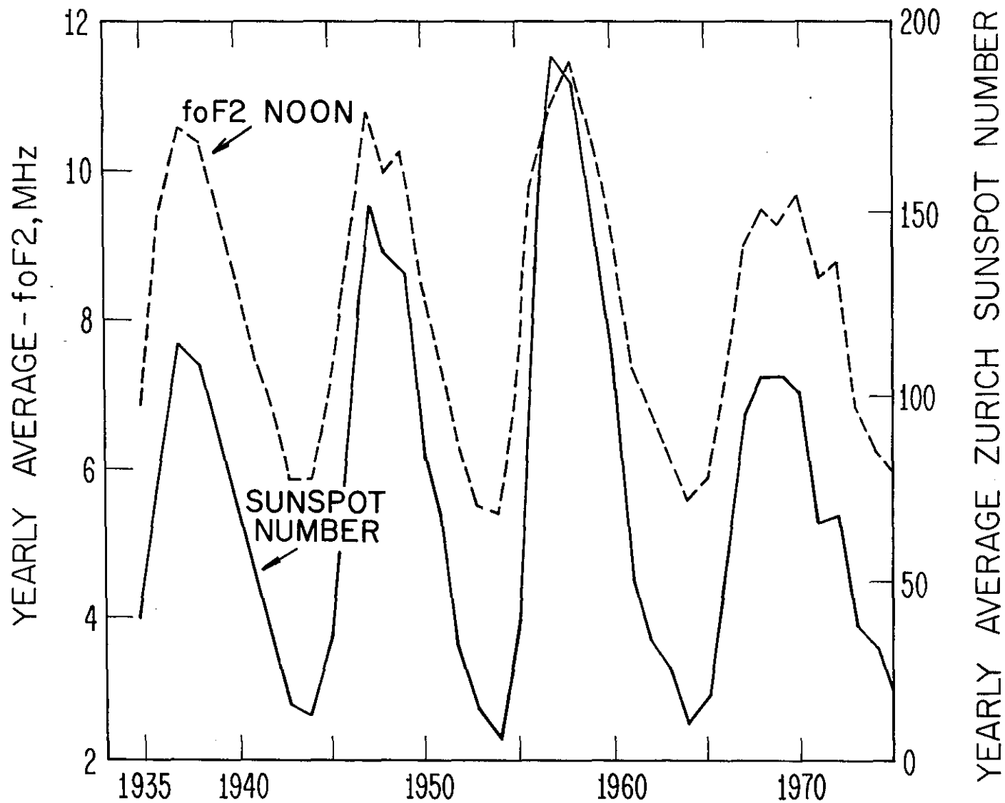
Figure 2. Yearly average sunspot number (solid line, right scale) and yearly average foF2 (dashed line, left scale) at noon near Washington, D.C., from 1935 until 1976. The ionospheric reflectivity is high during the peak of a sunspot cycle and is lower during the minima of the sunspot cycle.
