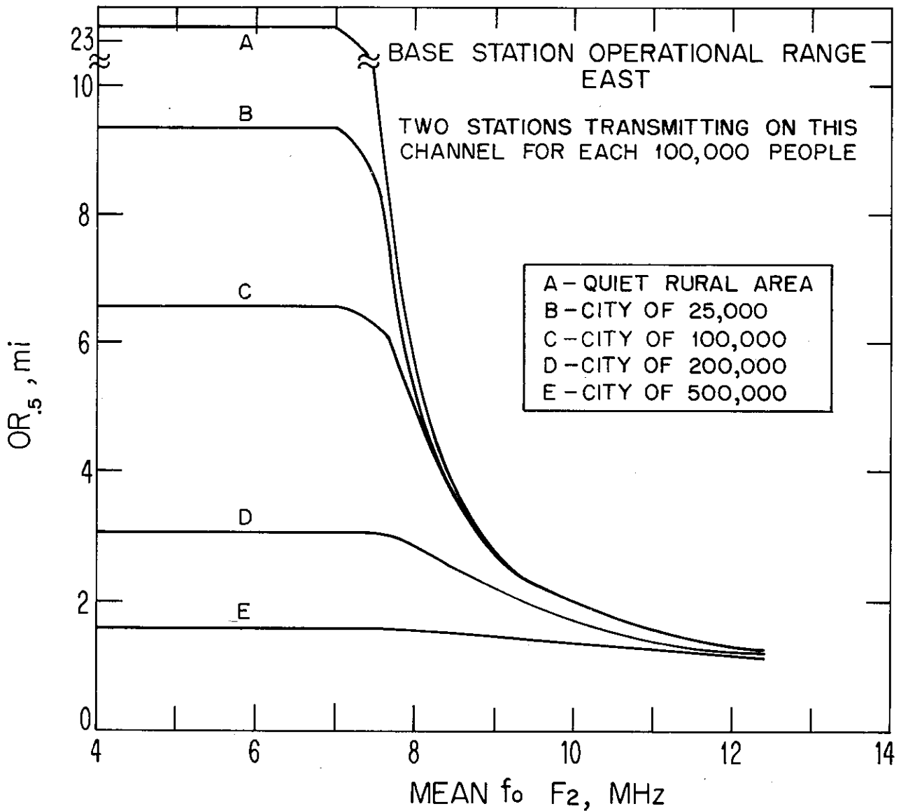
Figure C-7. Average operational range of a typical CB base station for the conditions described on figure, as a function of the ionospheric reflectivity parameter, mean f_o F_2 . The left side of the figure corresponds to low solar activity; the right side is representative of winter daytime conditions near the peak of a solar cycle. Mobile station operational range is less than half base station range.
