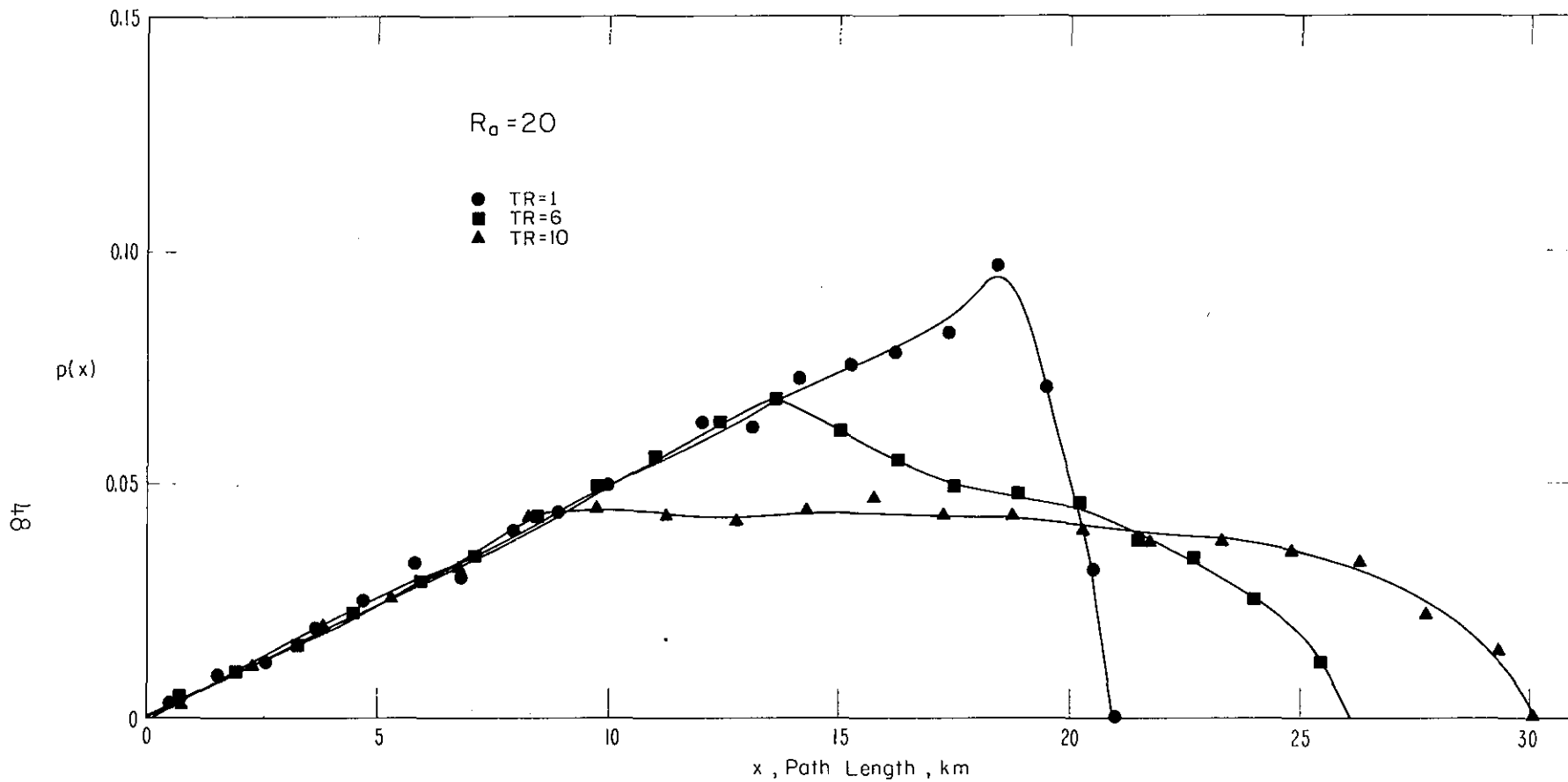
Figure B-3. Probability density functions for interfering path lengths, for three different wanted path lengths. The geometry is shown in Figure B-2.
