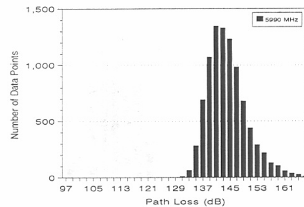
Figure C-22. Path loss distribution for high rise 3, floor 11, NLOS.
