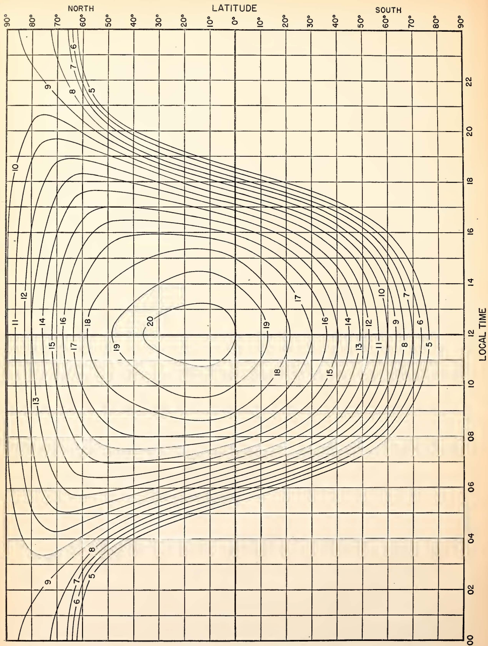
Fig. 11 E-LAYER 2000-MUF, IN Mc, PREDICTED FOR JUNE 1947
