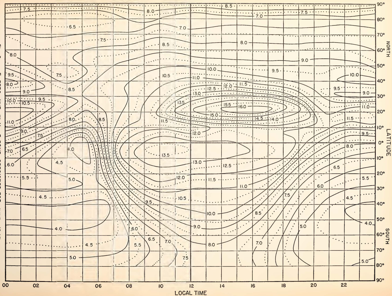
Fig. 9 F 2 ZERO-WUF, IN Mc, E ZONE, PREDICTED FOR JUNE 1947
