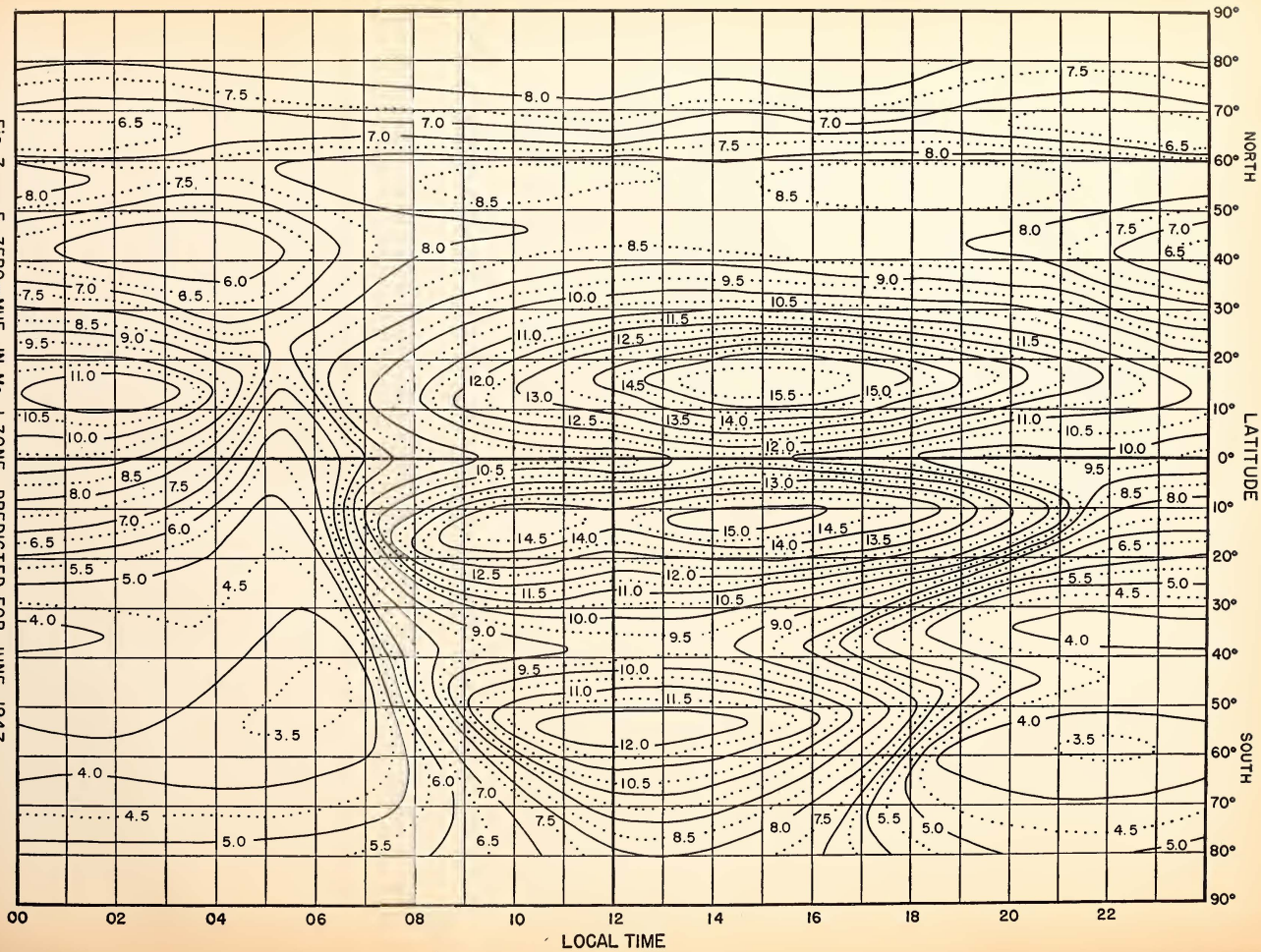
Fig. 7 F 2 ZERO-WUF, IN Mc, I ZONE, PREDICTED FOR JUNE 1947
