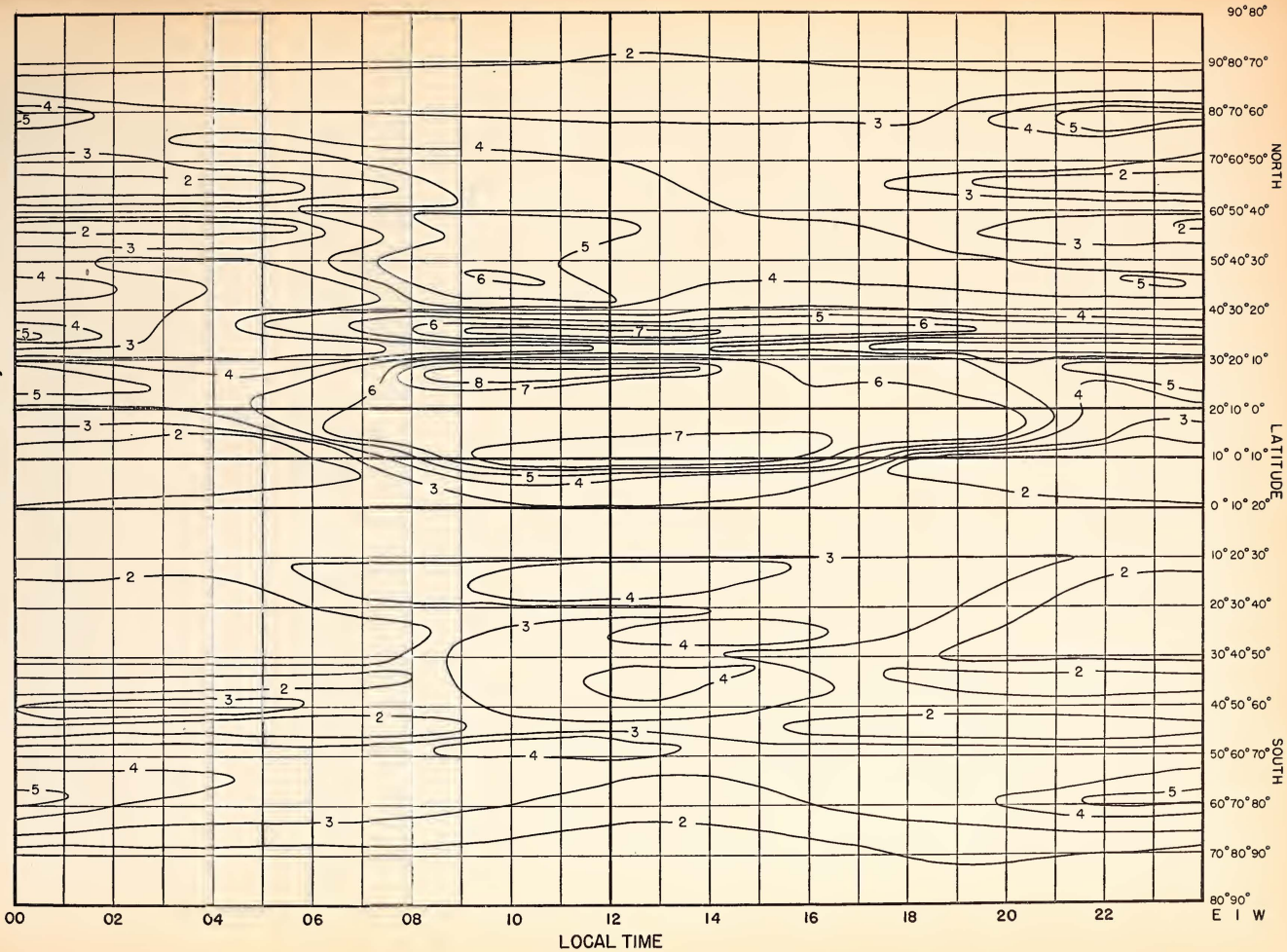
Fig. 12 MEDIAN f_{Es} , IN MC, PREDICTED FOR JUNE 1947
