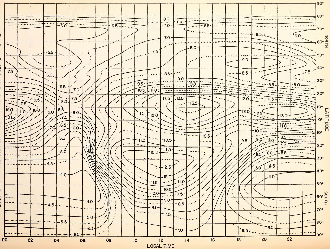
Fig. 5 F 2 ZERO-MUF, IN Mc, W ZONE, PREDICTED FOR JUNE 1947
