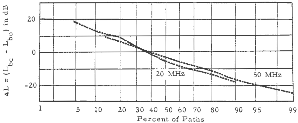
Figure 50. Cumulative distributions of basic transmission loss, observed and predicted, and of \Delta L , Colorado mountains, median \Delta h=580 m, f=50 and 20 MHz.
