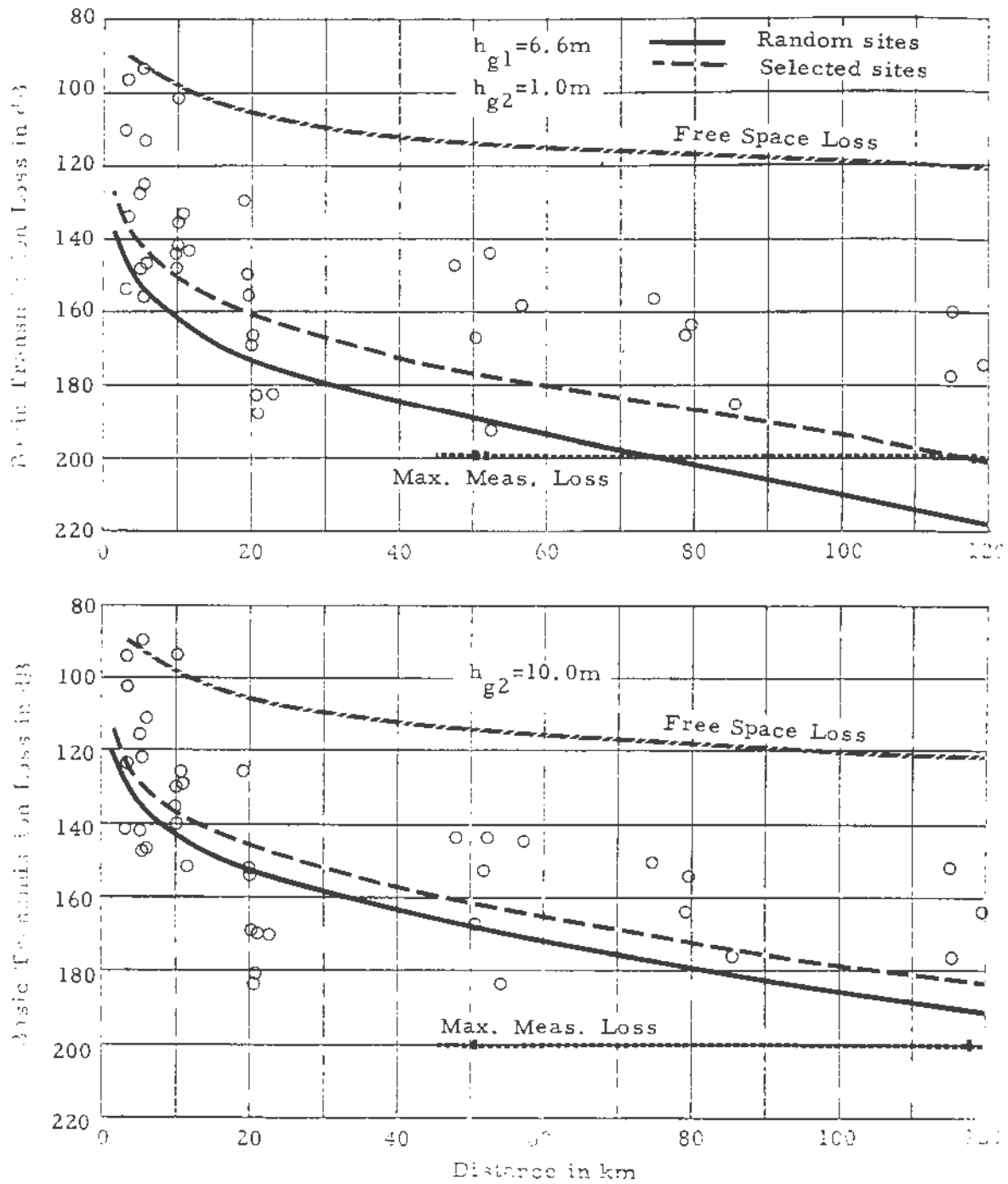
Figure 6. Basic transmission loss, measured and predicted, common receiver site R-2, \Delta h = 650\text{m} , f = 230\text{MHz} .
