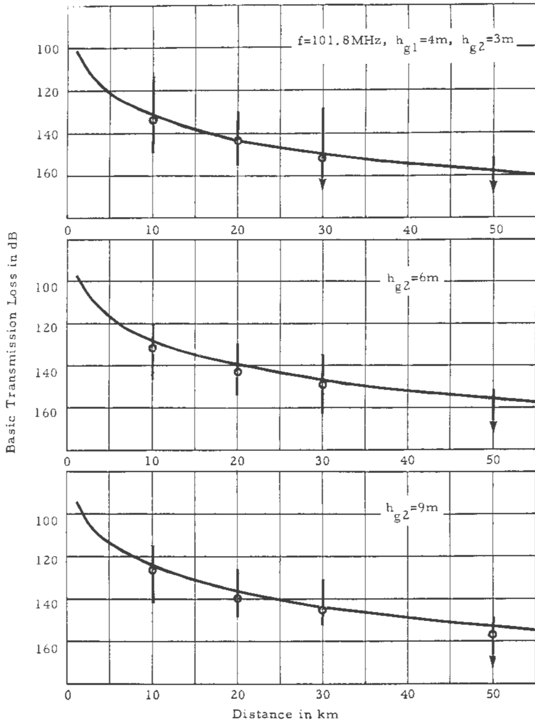
Figure 28. Basic transmission loss, Ohio, \Delta h=90\text{m} , f=101.8\text{MHz} , showing median and interdecile range of values at each nominal distance.
