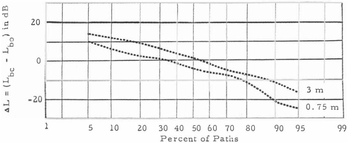
Figure 40. Cumulative distributions of basic transmission loss, observed and predicted, and of \Delta L , Laramie range, Wyoming, f=230 MHz.
