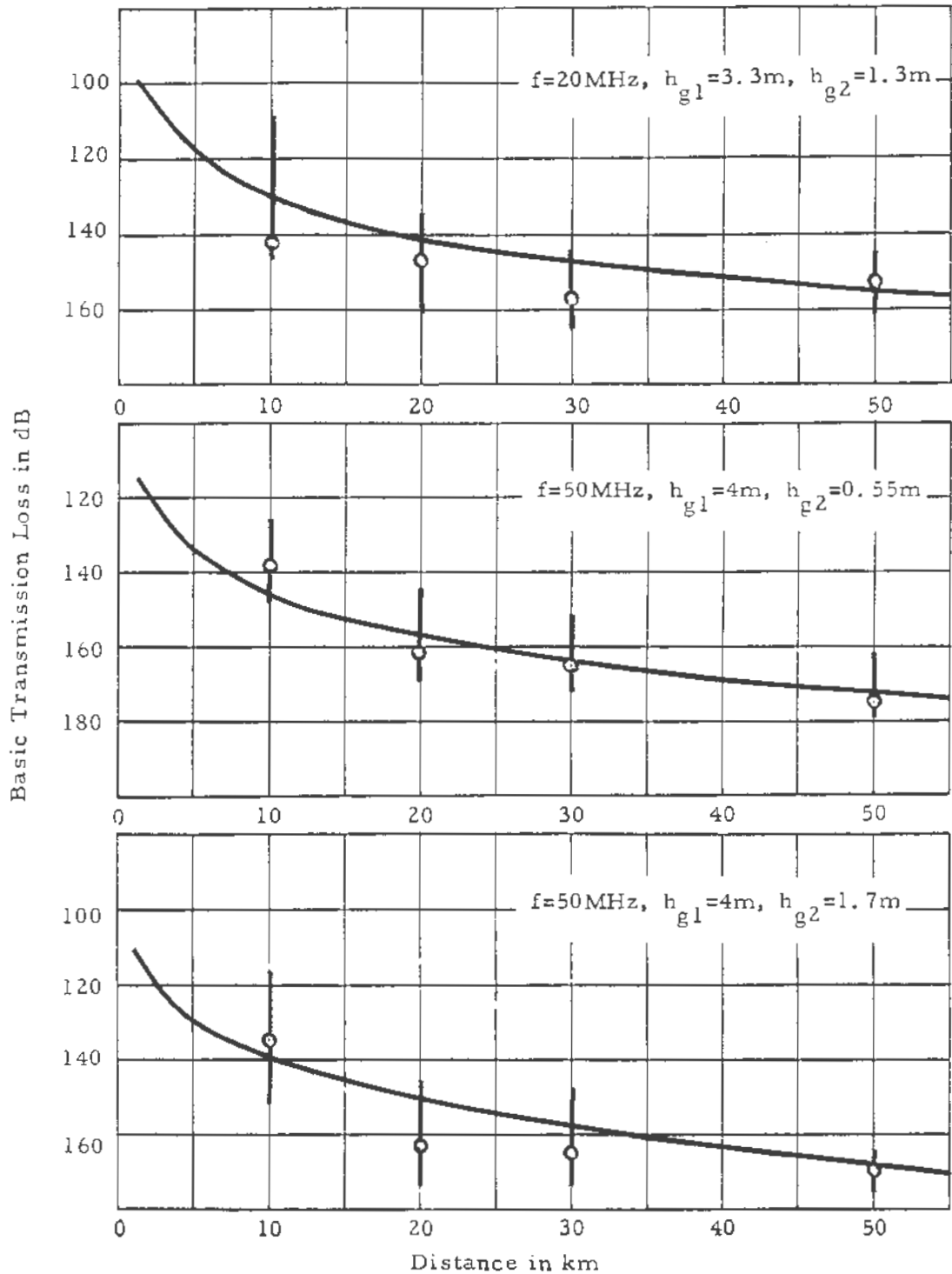
Figure 25. Basic transmission loss, Colorado mountains, \Delta h=650\text{m} , f=20 and 50\text{MHz} , showing median and interdecile range of values at each nominal distance.
