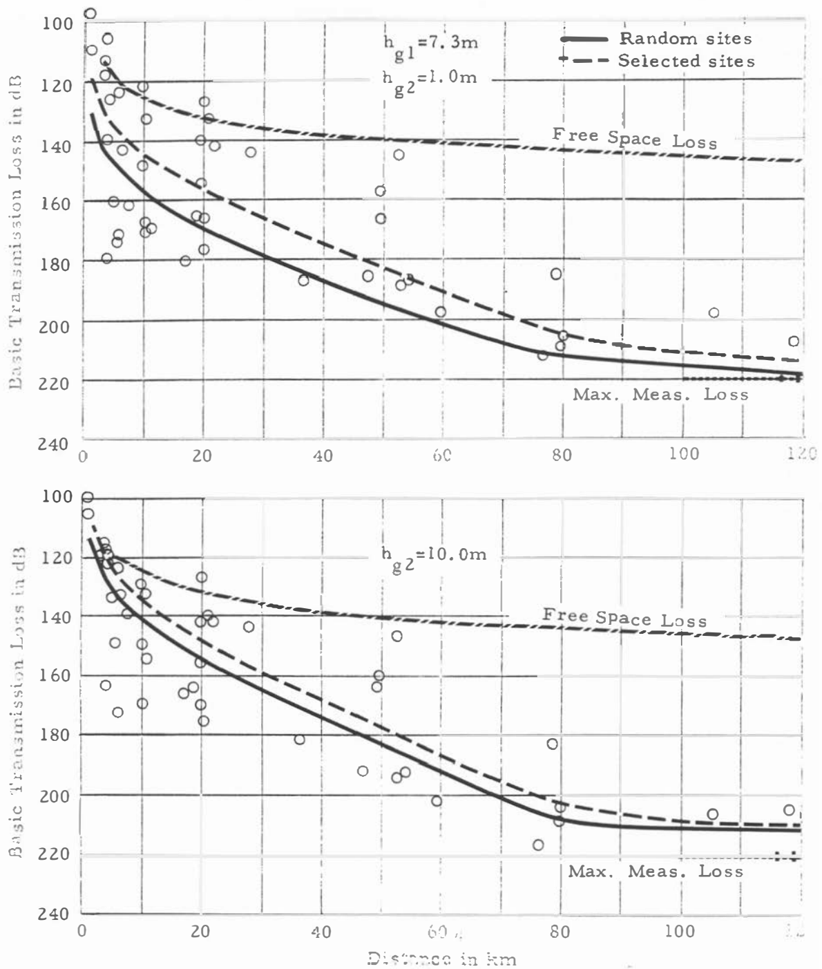
Figure 4. Basic transmission loss, measured and predicted, common receiver site R-1, \Delta h=90m , f=4595MHz .
