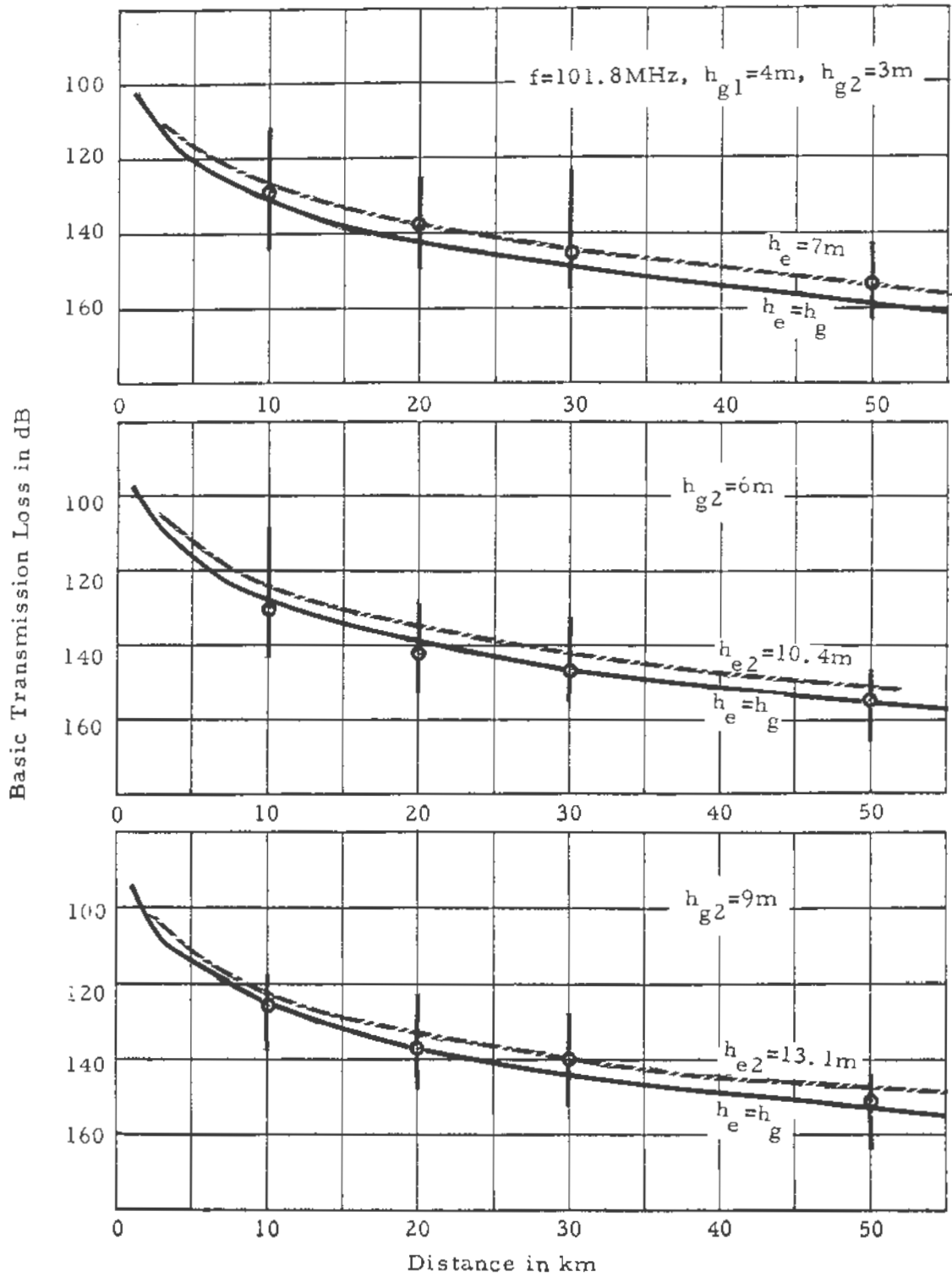
Figure 29. Basic transmission loss, Ohio, \Delta h=90\text{m} , f=101.8\text{MHz} , using alternate receiving locations, vertical polarization.
