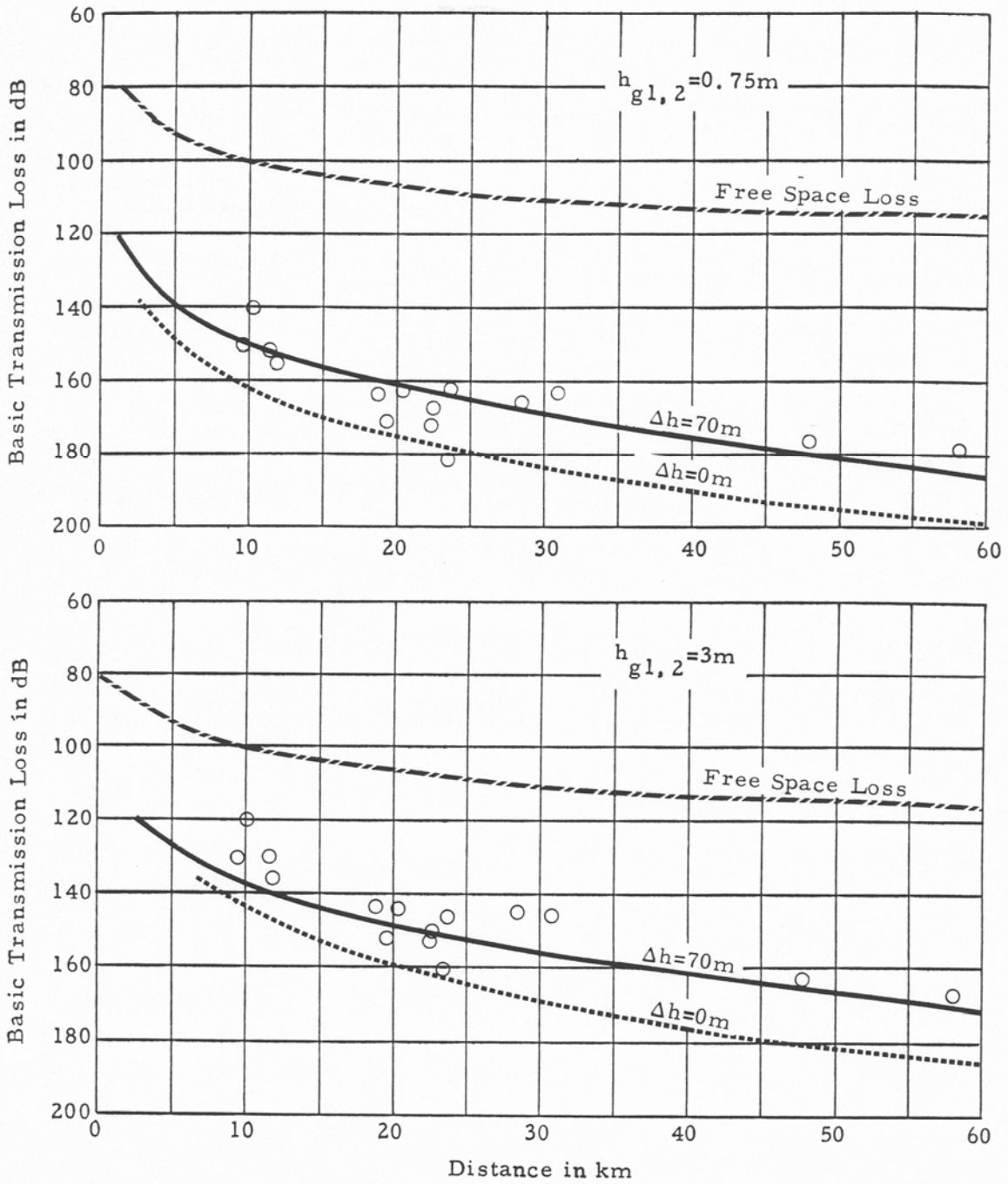
Figure 19. Basic transmission loss, measured and predicted, Ritzville area, Washington, \Delta h = 70m , f = 230MHz .
