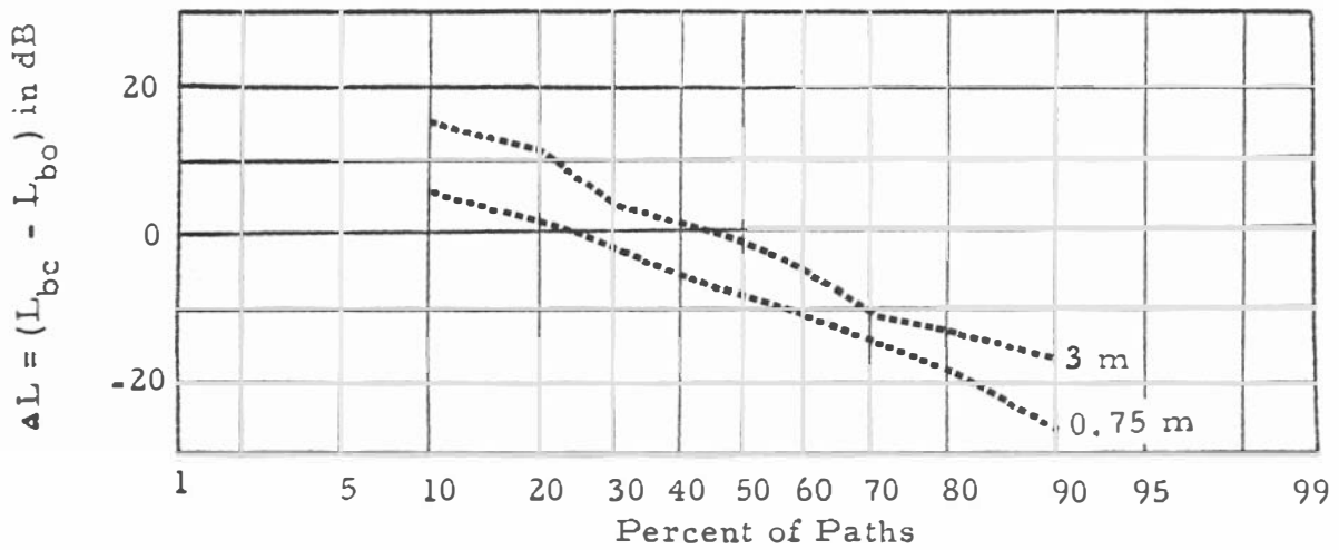
Figure 43. Cumulative distributions of basic transmission loss, observed and predicted, and of \Delta L , Idaho, f=416 MHz.
