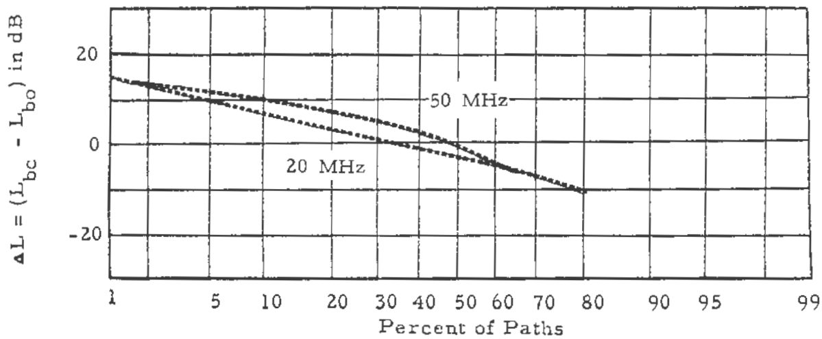
Figure 52. Cumulative distributions of basic transmission loss, observed and predicted, and of \Delta L , northeastern Ohio, median \Delta h=95 m, f=20 and 50 MHz.
