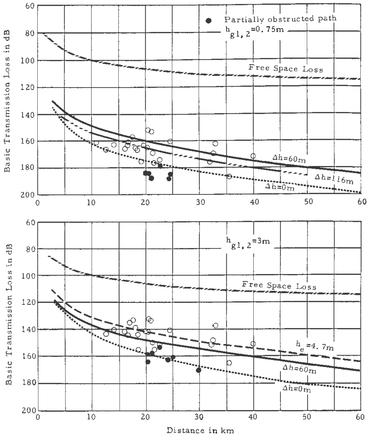
Figure 17. Basic transmission loss, measured and predicted, lava flows, Idaho, median. \Delta h = 60\text{m} , f = 230\text{MHz} .
