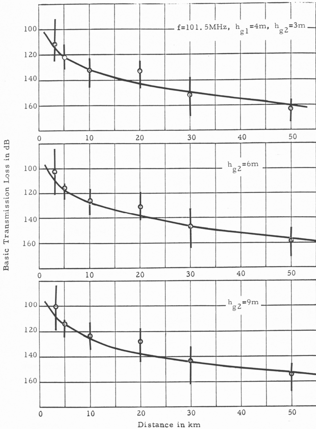
Figure 24. Basic transmission loss, Colorado plains, \Delta h=90\text{m} , f=101.5\text{MHz} , showing median and interdecile range of values at each nominal distance.
