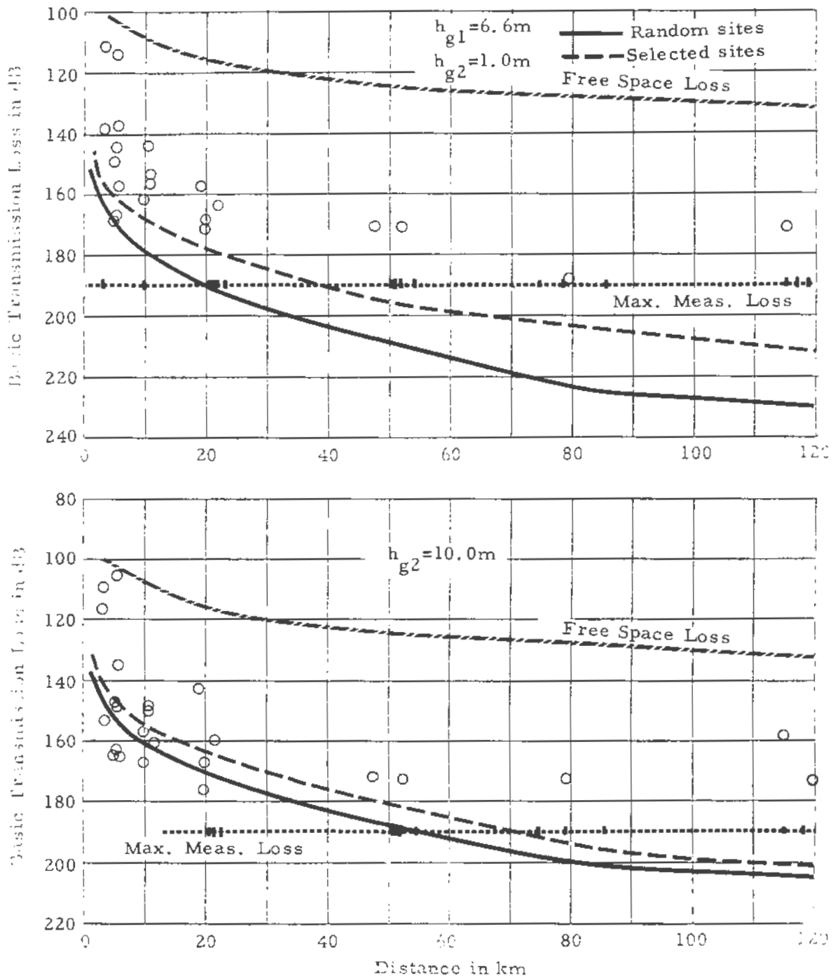
Figure 8. Basic transmission loss, measured and predicted, common receiver site R-2, \Delta h = 650\text{m} , f = 751\text{MHz} .
