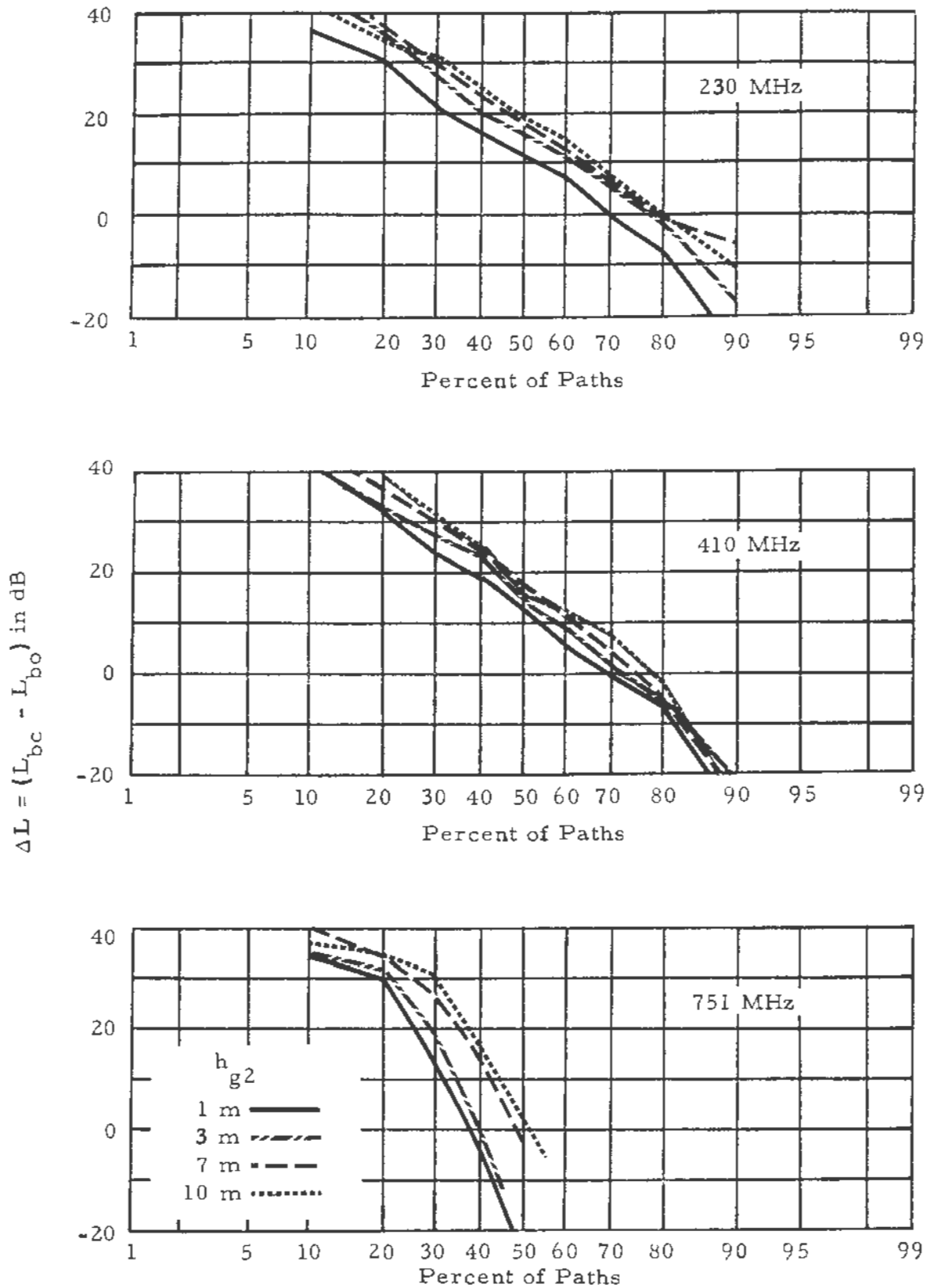
Figure 36. Cumulative distributions of \Delta L showing the effects of increasing receiver height, R-2, f-230, 410, and 751 MHz.
