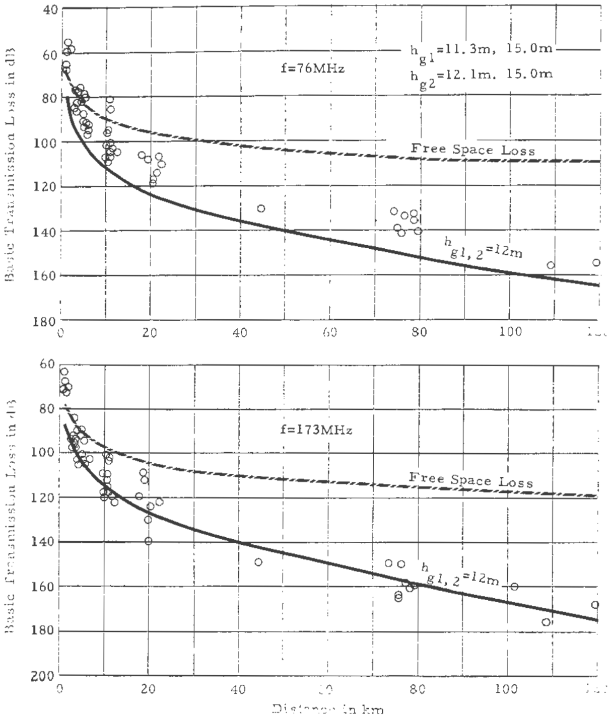
Figure 11. Basic transmission loss, measured and predicted, 51 paths in Virginia, \Delta h=85\text{m} , f=76 and 173\text{MHz} .
