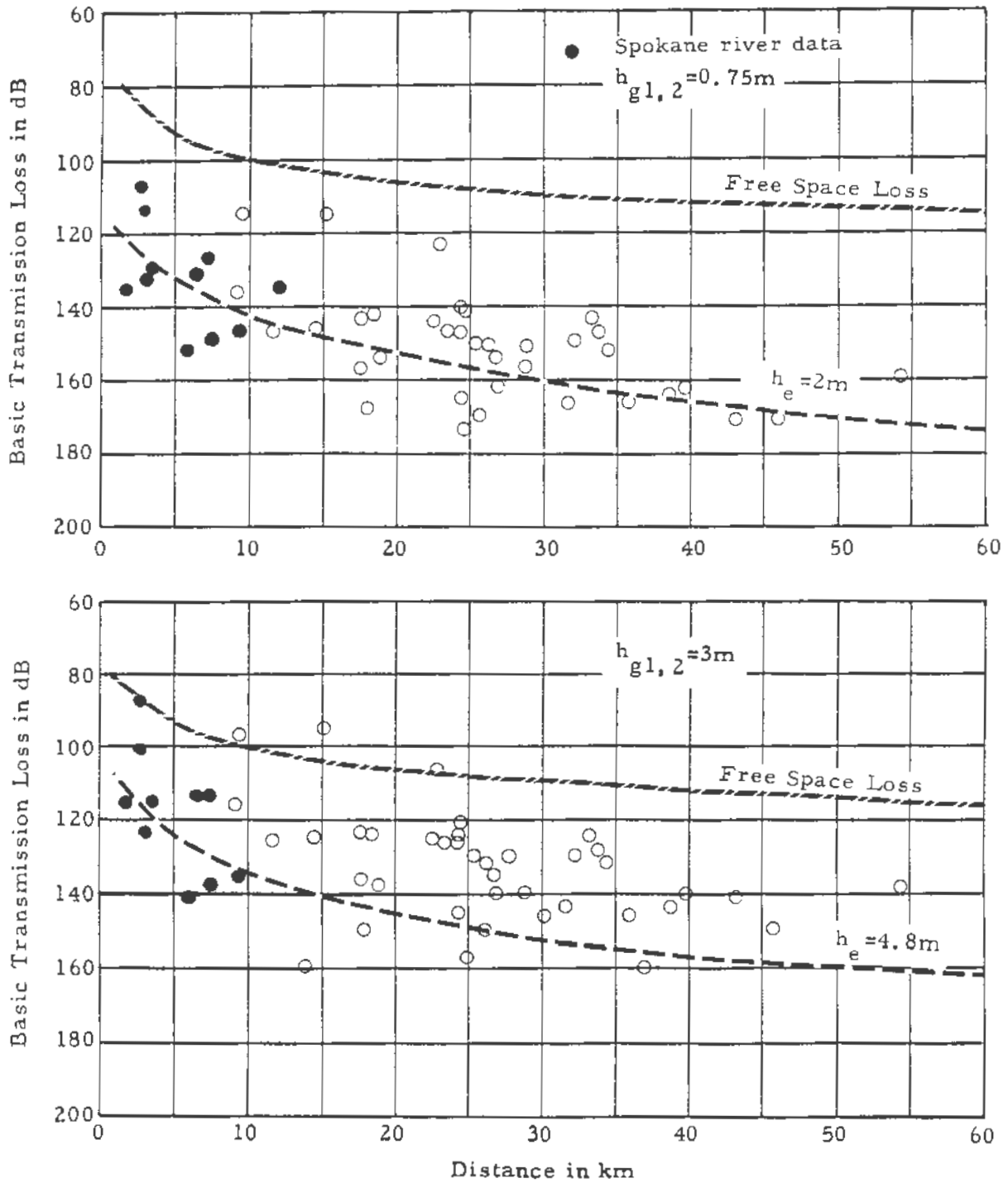
Figure 21. Basic transmission loss, measured and predicted, mountainous terrain, Washington, \Delta h=210 and 305m , f=230MHz .
