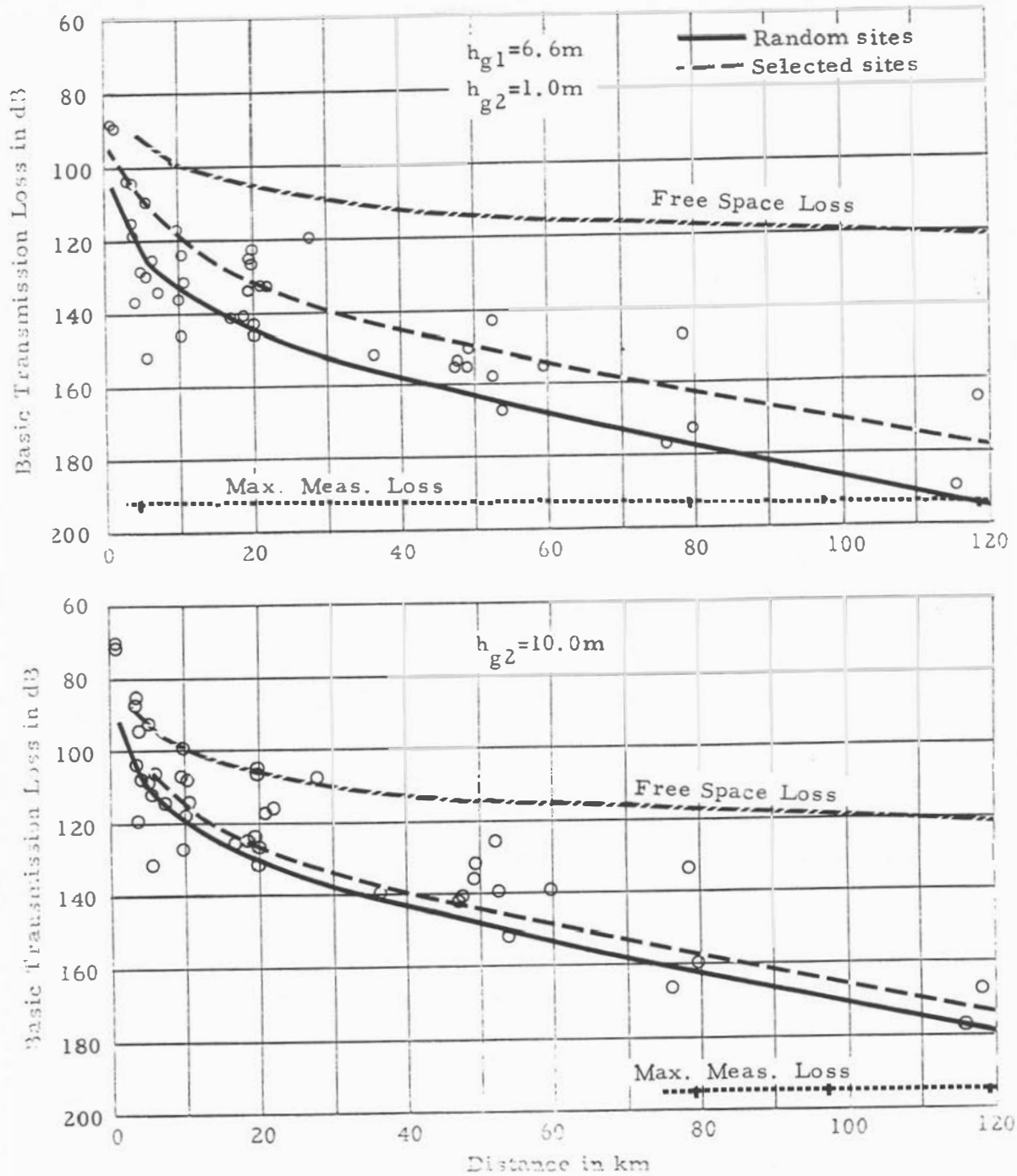
Figure 1. Basic transmission loss, measured and predicted, common receiver site R-1, \Delta h=90\text{m} , f=230\text{ MHz} .
