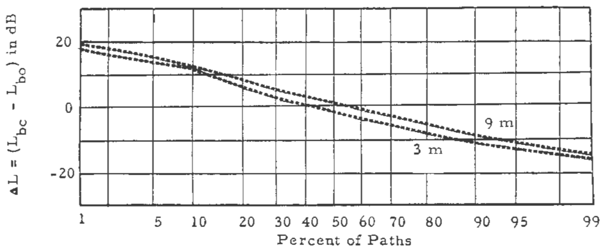
Figure 49. Cumulative distributions of basic transmission loss, observed and predicted, and of \Delta L , Colorado plains, median \Delta h=95 m, f=100 MHz.
