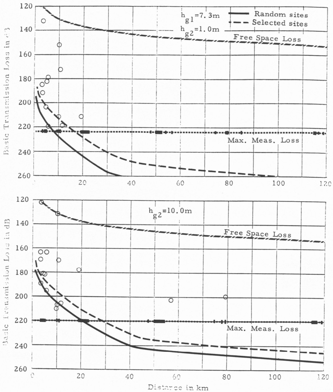
Figure 10. Basic transmission loss, measured and predicted, common receiver site R-2, \Delta h = 650\text{m} , f = 9190\text{MHz} .
