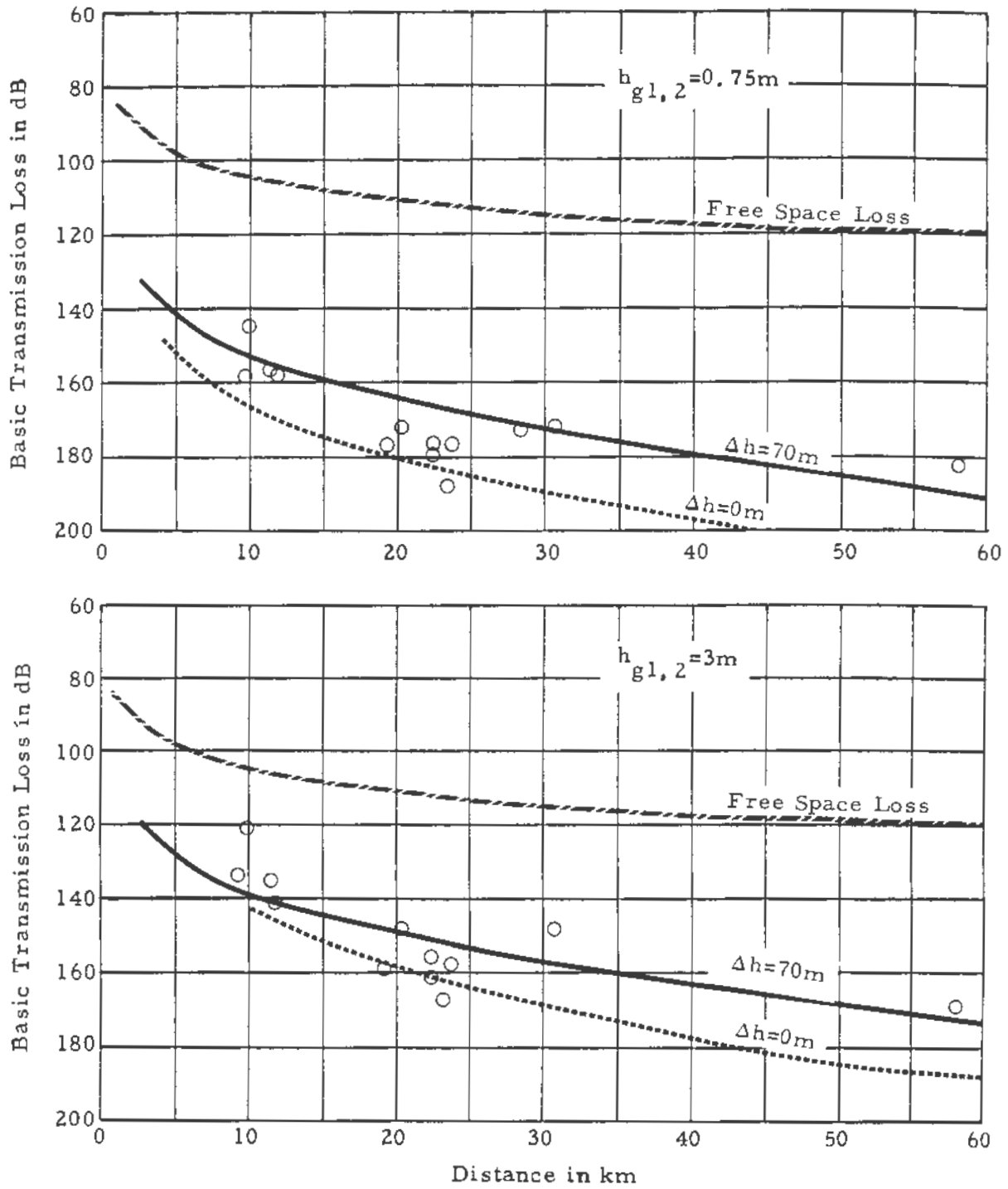
Figure 20. Basic transmission loss, measured and predicted, Ritzville area, Washington, \Delta h = 70m , f = 416MHz .
