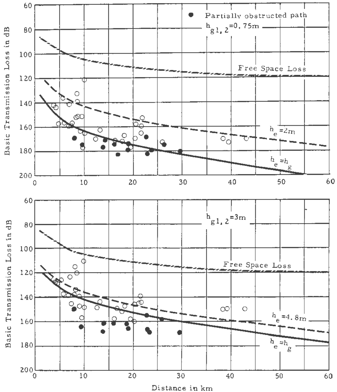
Figure 16. Basic transmission loss, measured and predicted, Laramie range, Wyoming, \Delta h = 120\text{m} , f = 416\text{MHz} .
