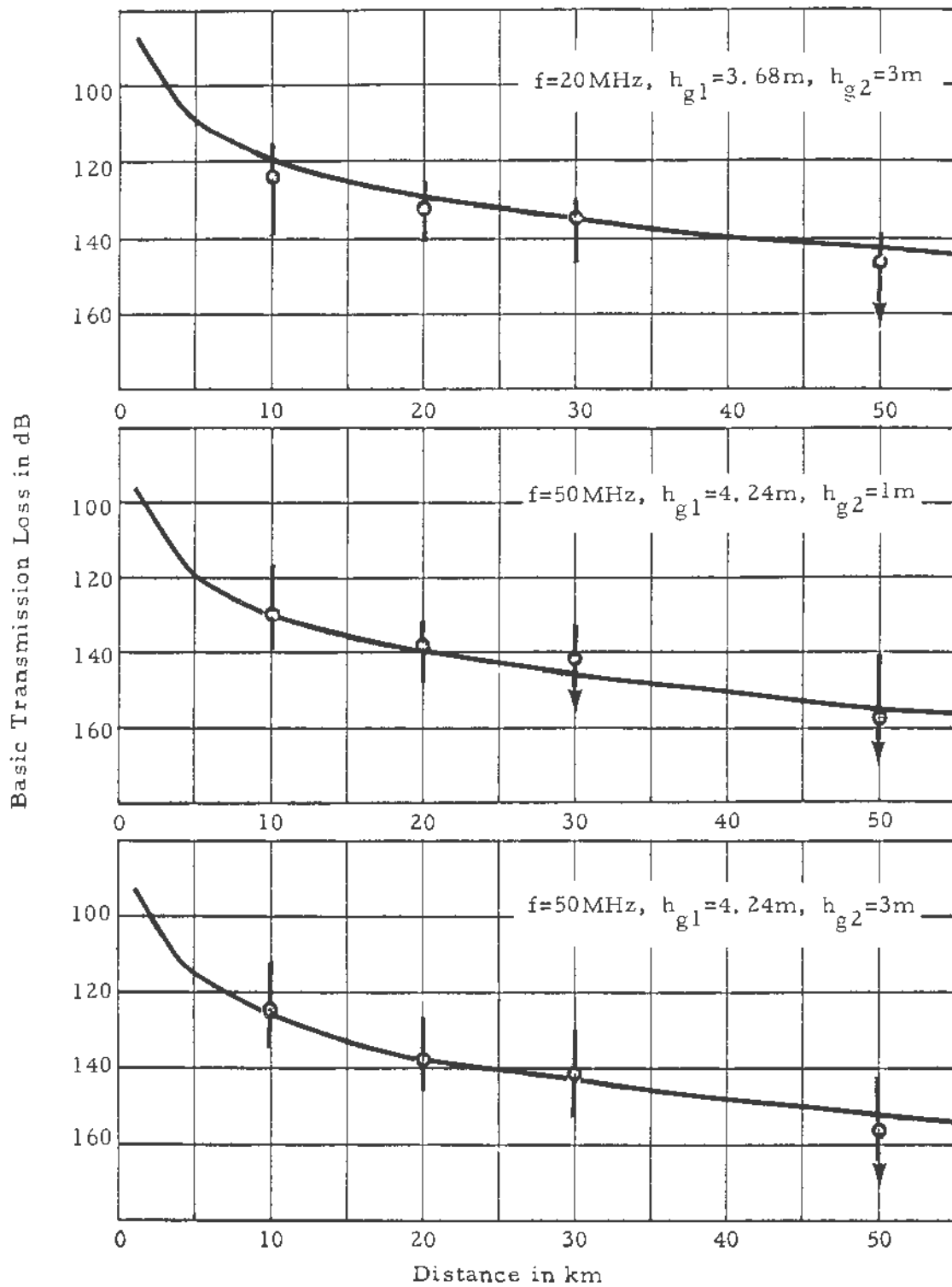
Figure 27. Basic transmission loss, Ohio, \Delta h=90\text{m} , f=20 and 50\text{MHz} , showing median and interdecile range of values at each nominal distance.
