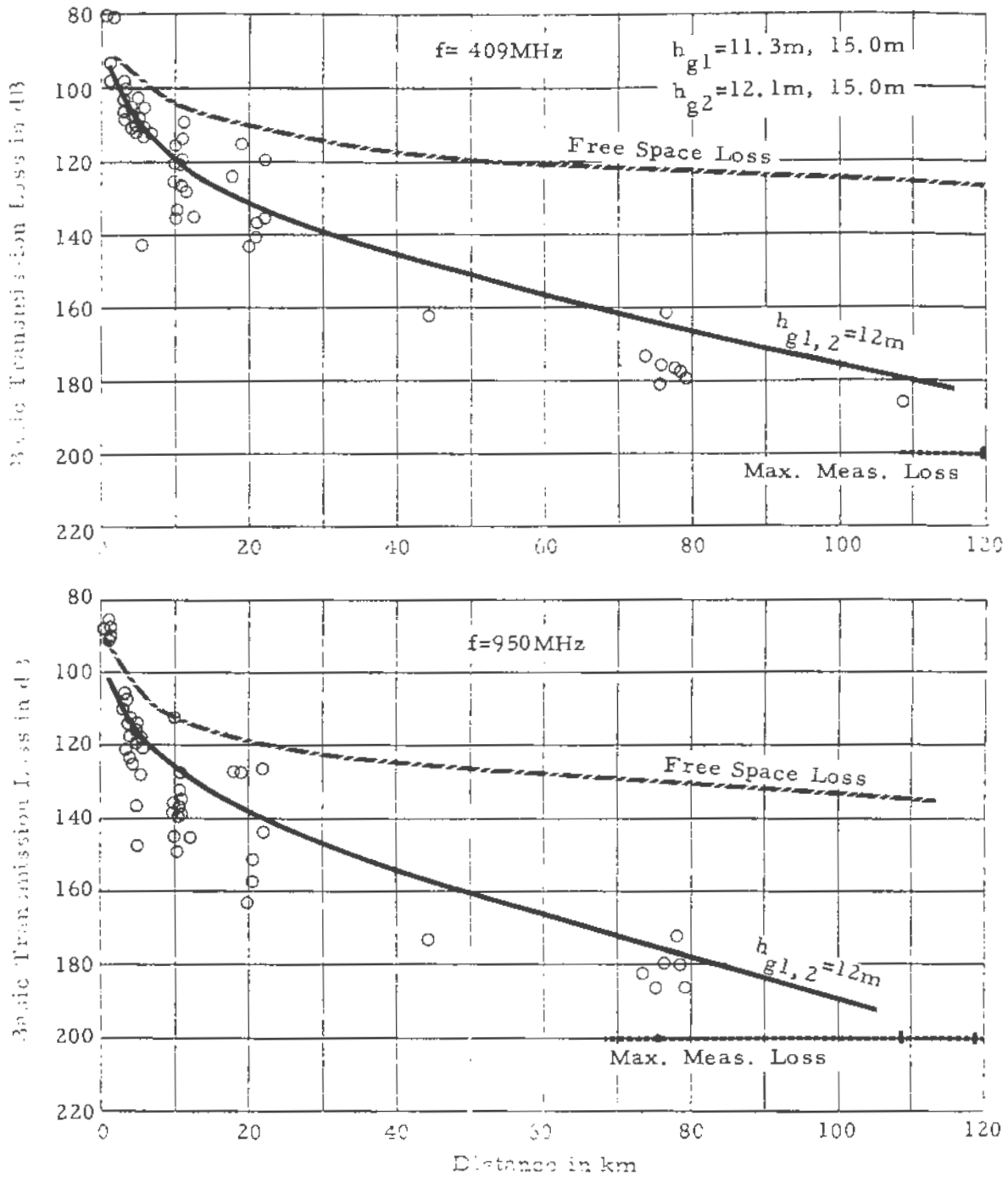
Figure 12. Basic transmission loss, measured and predicted, 51 paths in Virginia, \Delta h=85\text{m} , f=409 and 950\text{MHz} .
