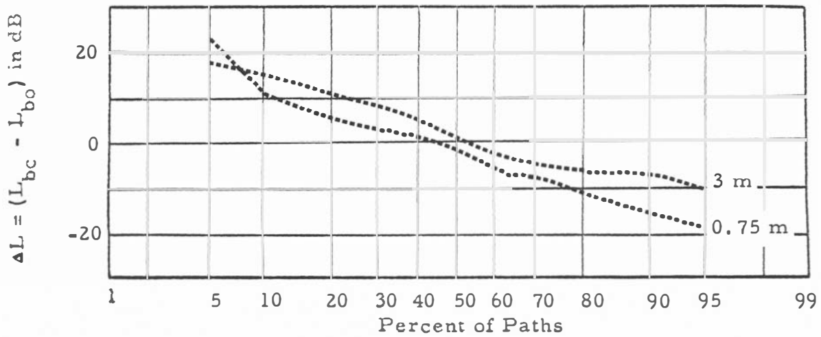
Figure 41. Cumulative distributions of basic transmission loss, observed and predicted, and of \Delta L , Wyoming, f=416 MHz.
