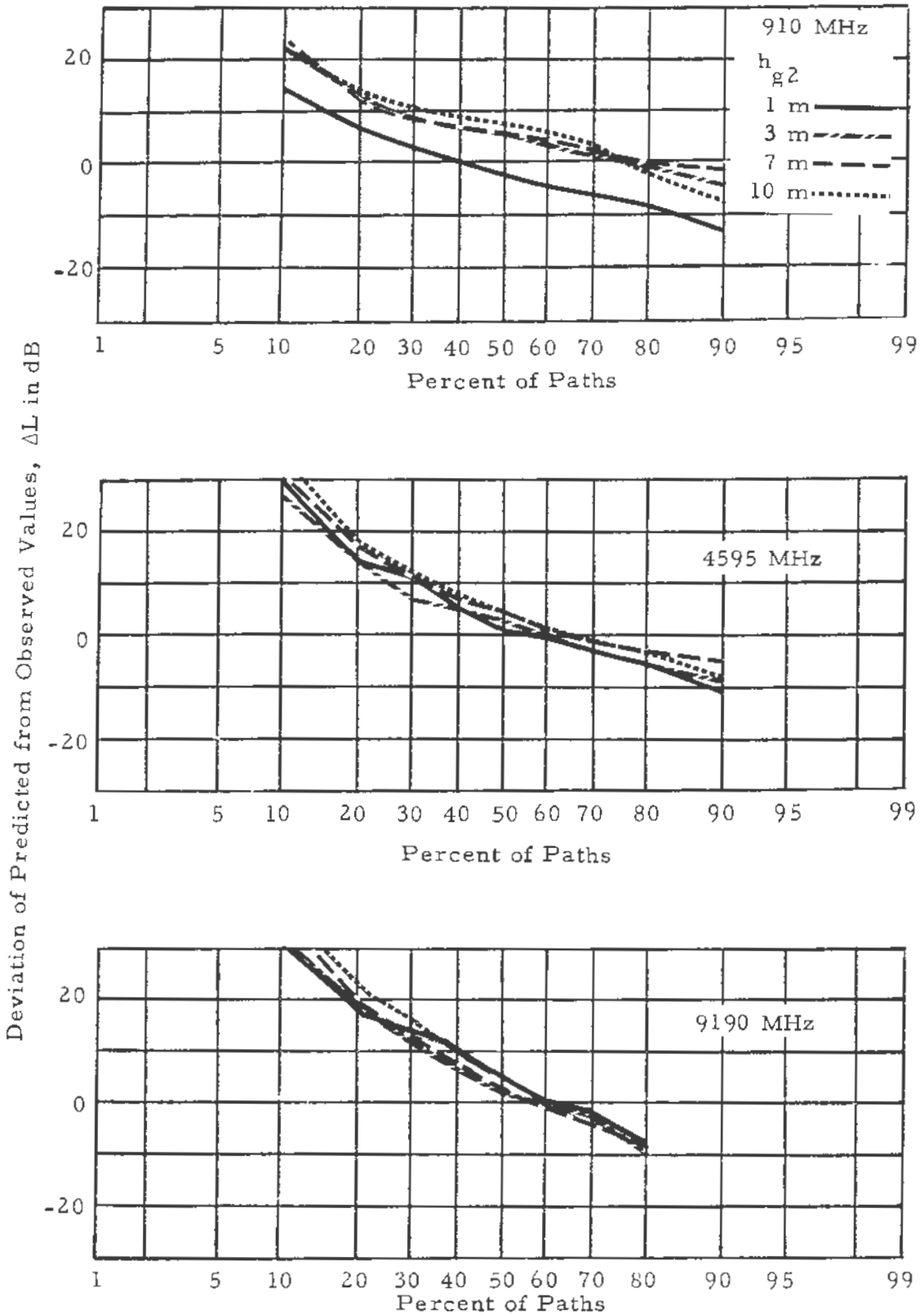
Figure 34 Cumulative distributions of \Delta L showing the effects of increasing receiver height, R-1, f=910, 4595, and 9190 MHz.
