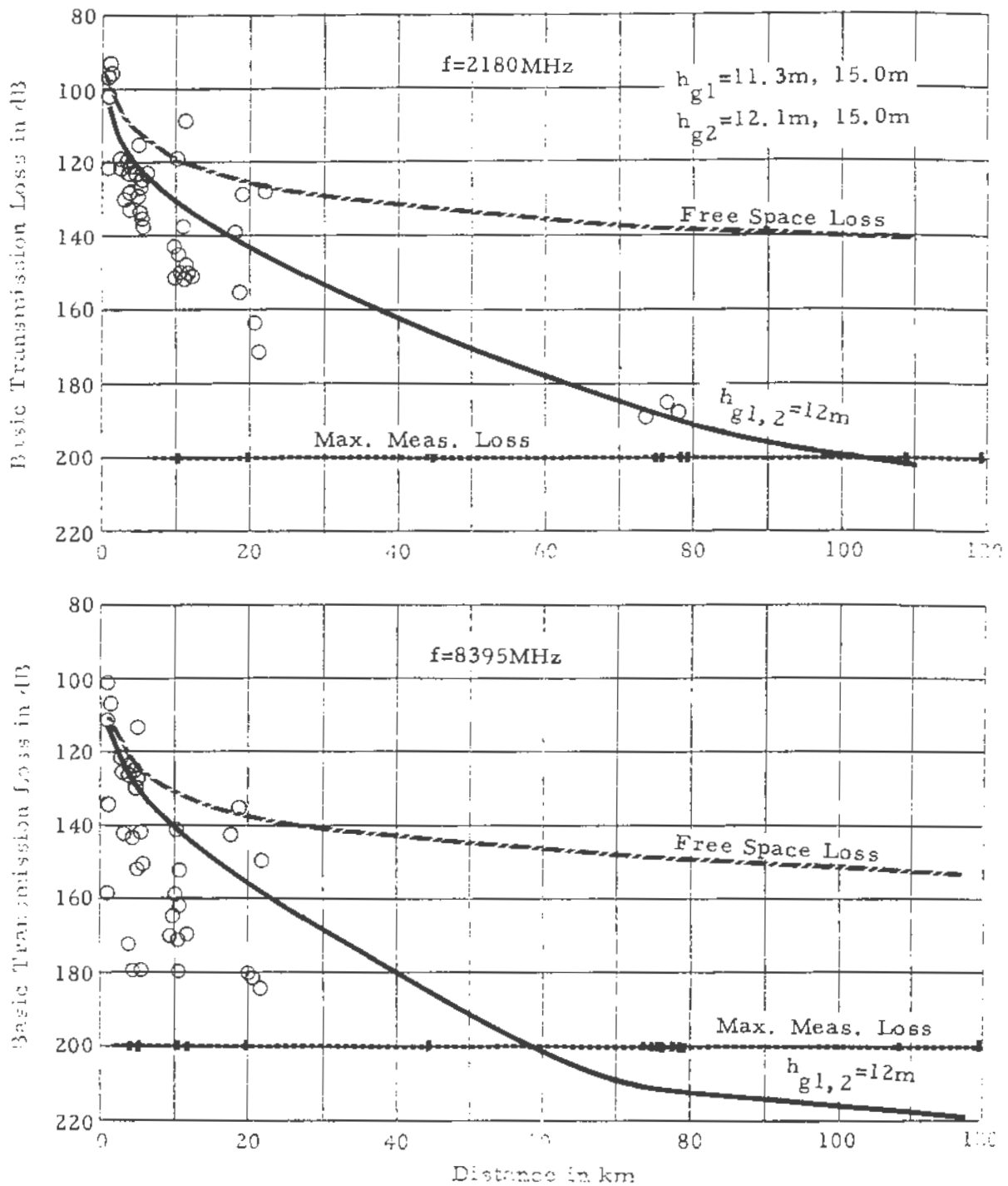
Figure 13. Basic transmission loss, measured and predicted, 51 paths in Virginia, \Delta h=85\text{m} , f=2180 and 8395\text{MHz} .
