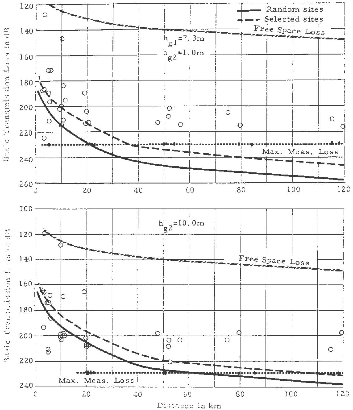
Figure 9. Basic transmission loss, measured and predicted, common receiver site R-2, \Delta h = 650\text{m} , f = 4595\text{MHz} .
