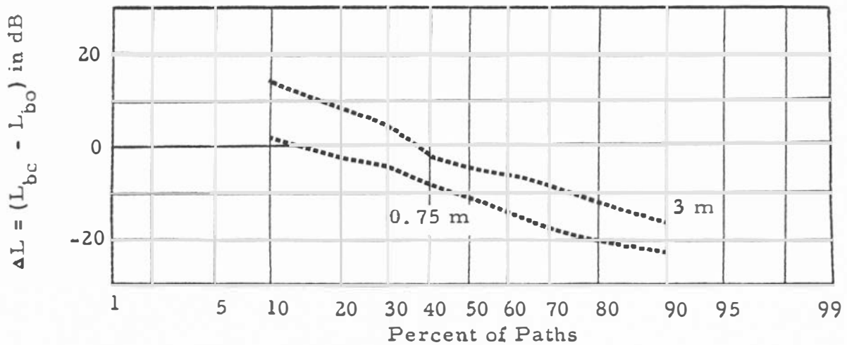
Figure 42. Cumulative distributions of basic transmission loss, observed and predicted, and of \Delta L , Idaho, f=230 MHz.
