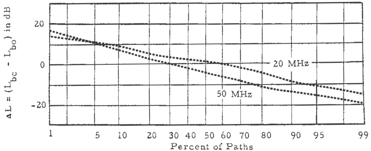
Figure 48. Cumulative distributions of basic transmission loss, observed and predicted, and of \Delta L , Colorado plains, medians \Delta h=95 m, f=20 and 50 MHz.
