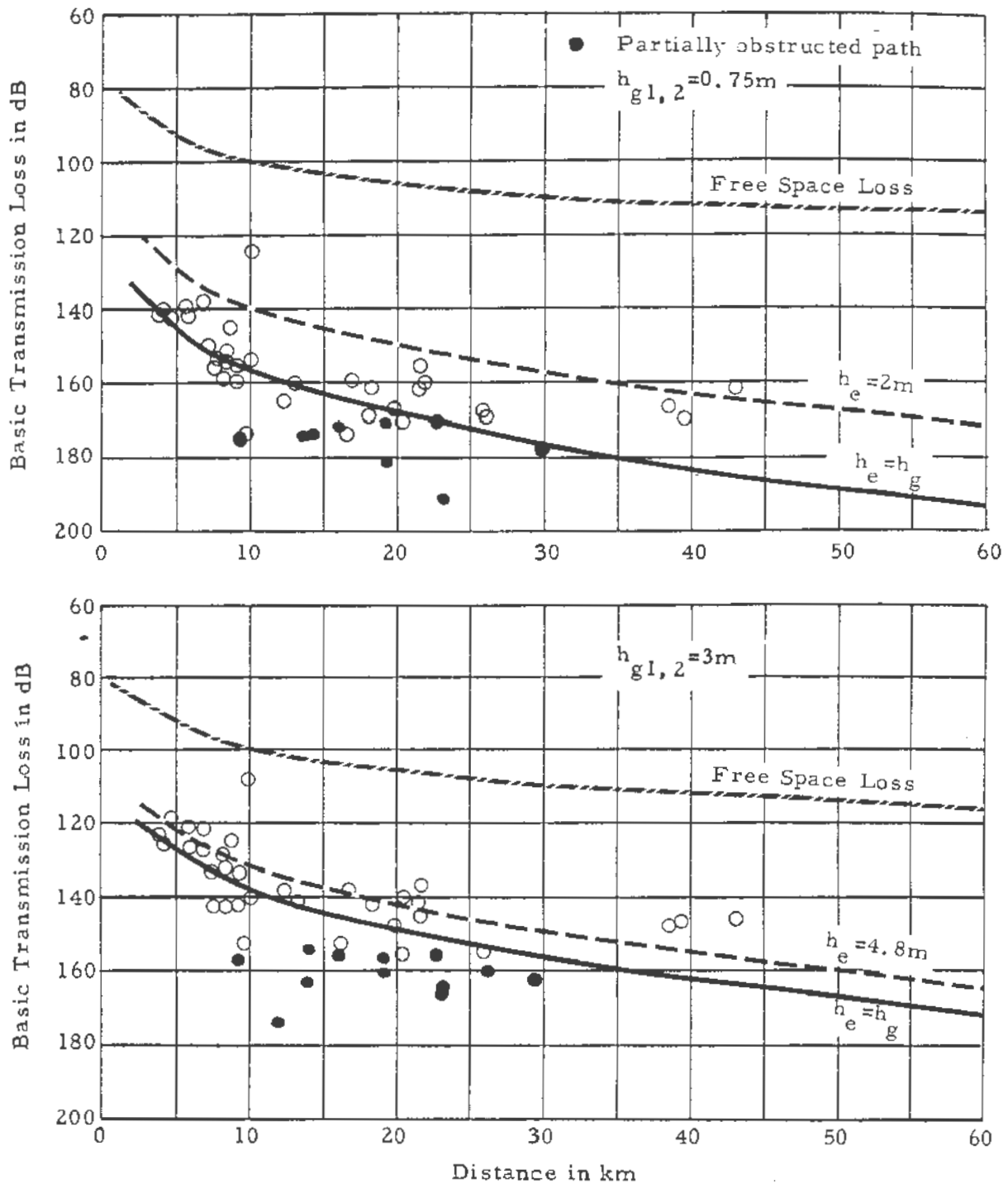
Figure 15. Basic transmission loss, measured and predicted, Laramie range, Wyoming, \Delta h=120m , f=230MHz .
