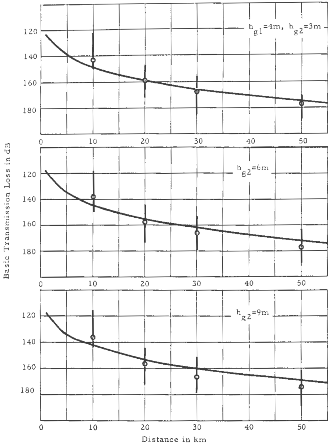
Figure 26. Basic transmission loss, Colorado mountains, \Delta h=650\text{m} , f=101,5\text{MHz} , showing median and interdecile range of values at each nominal distance.
