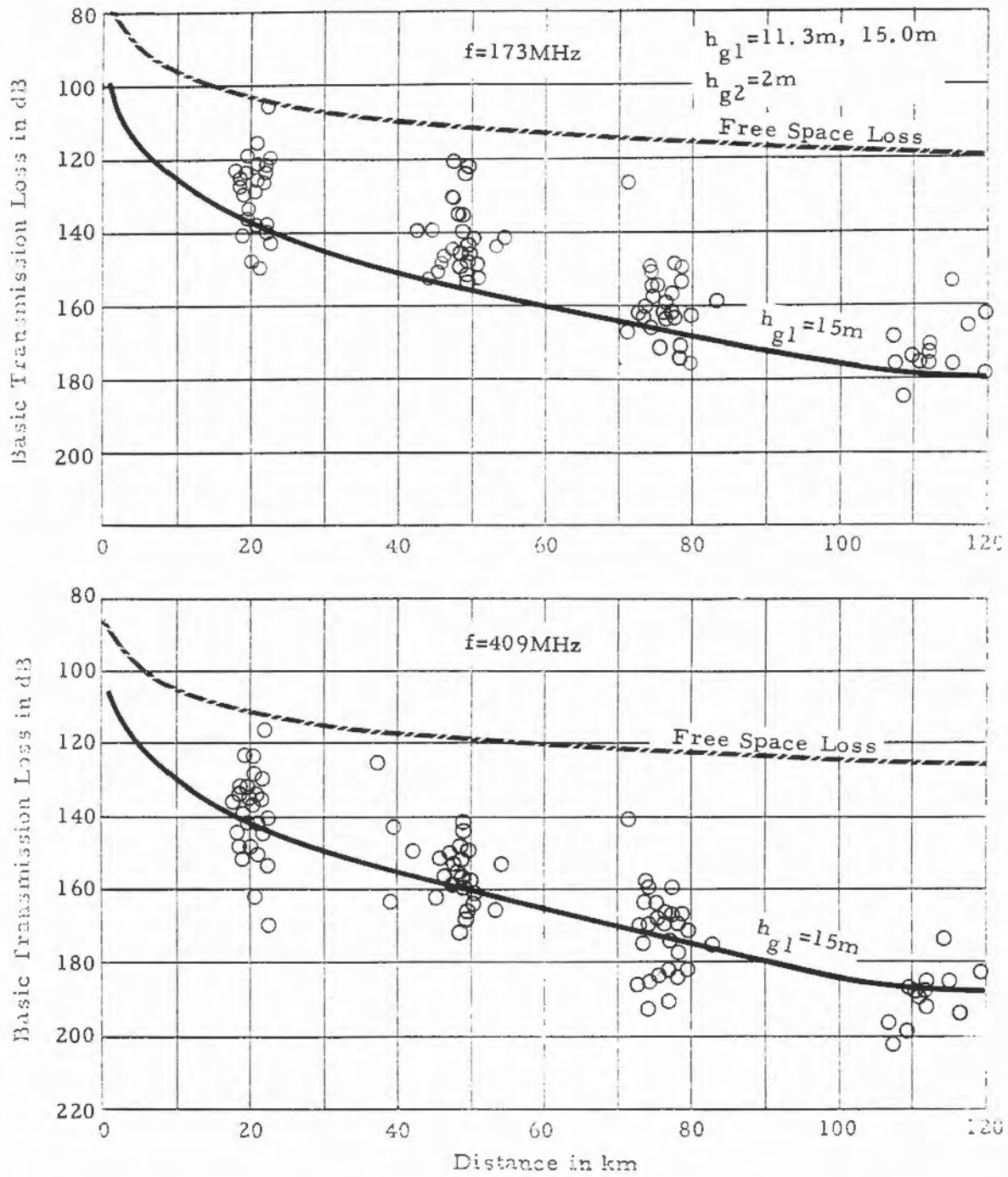
Figure 14. Basic transmission loss, measured and predicted, Virginia, all paths with h_{g2}=2\text{m} , f=173 and 409\text{MHz} .
