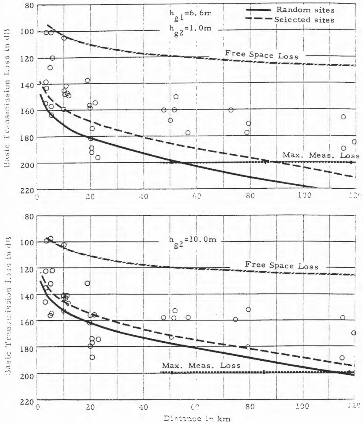
Figure 7. Basic transmission loss, measured and predicted, common receiver site R-2, \Delta h=650\text{m} , f=407\text{MHz} .
