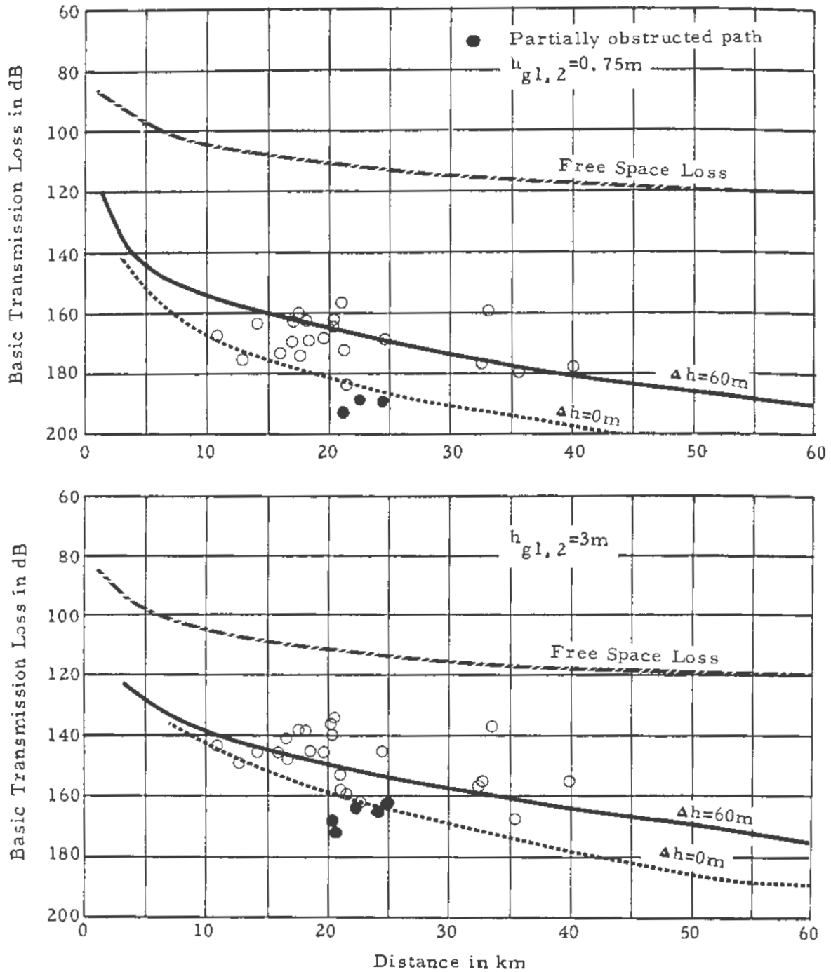
Figure 18. Basic transmission loss, measured and predicted, lava flows, Idaho, median \Delta h = 60\text{m} , f = 416\text{MHz} .
