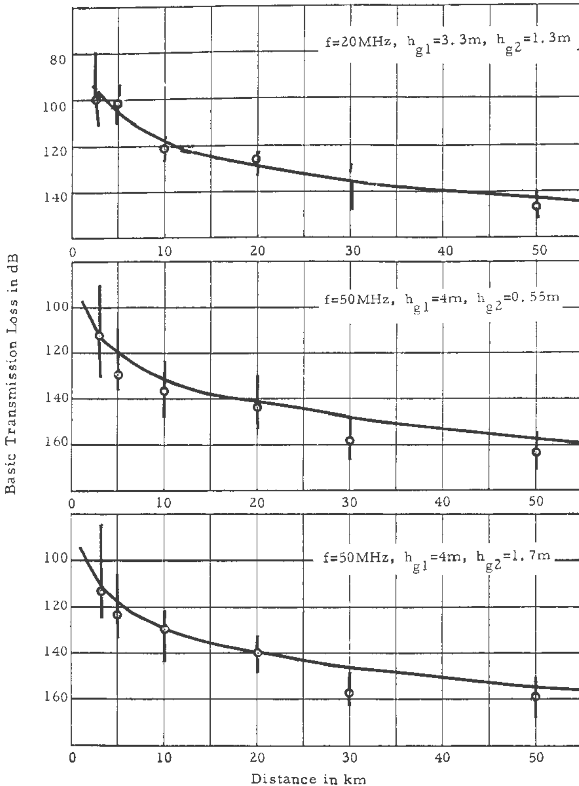
Figure 23. Basic transmission loss, Colorado plains, \Delta h=90\text{m} , f=20 and 50\text{MHz} , showing median and interdecile range of values at each nominal distance.
