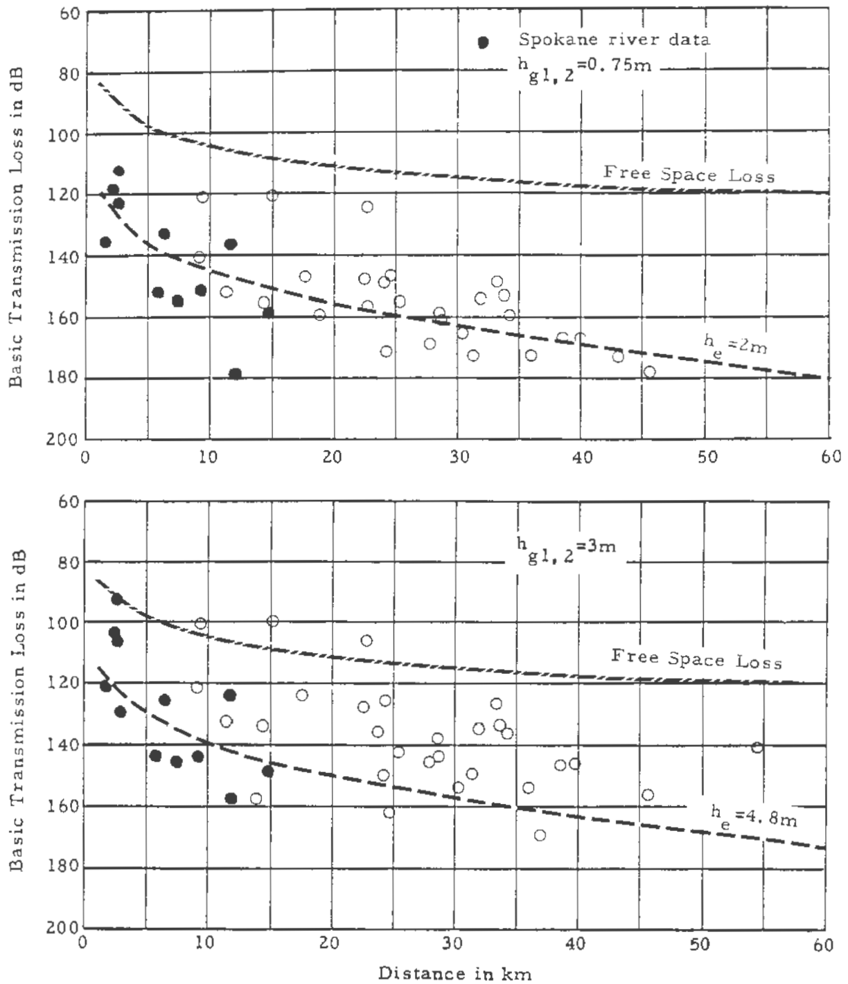
Figure 22. Basic transmission loss, measured and predicted, mountainous terrain, Washington, \Delta h = 210 and 305m , f = 416MHz .
