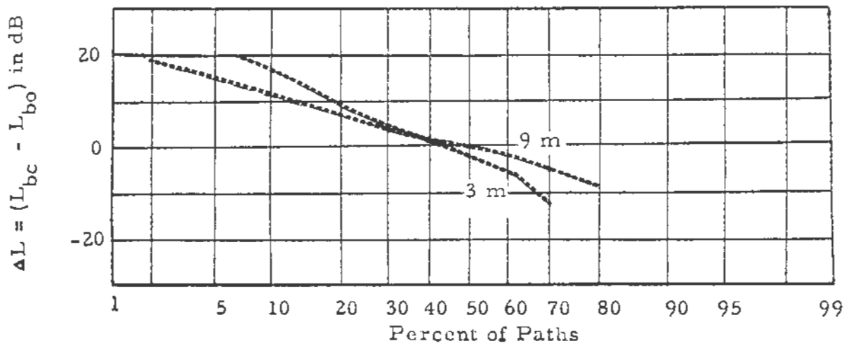
Figure 53. Cumulative distributions of basic transmission loss, observed and predicted, and of \Delta L , northeastern Ohio, median \Delta h=95 m, f=100 MHz.
