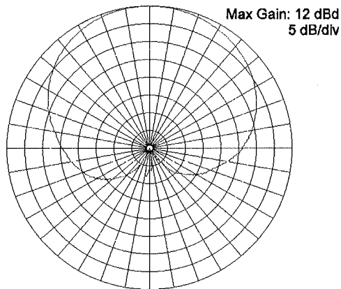
Figure 20. A log-periodic antenna horizontal-plane pattern
