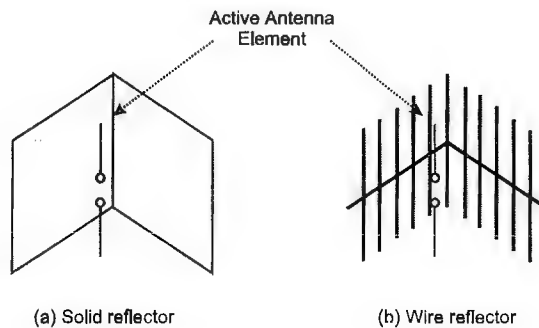
Figure 12. Corner-reflector antennas
