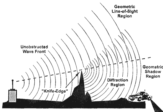
Figure 36. An example of diffraction
