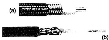
Figure 29. Coaxial cables commonly used for LMR — (a) base-station applications and (b) mobile applications
