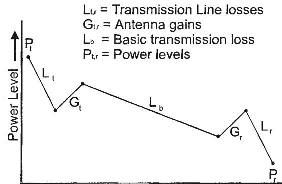
Figure 34. Gains and losses as described in the power-budget equation
