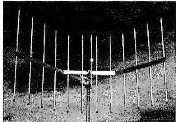
Figure 13. A typical corner-reflector antenna
