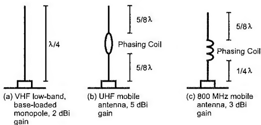
Figure 10. Typical mobile antennas
