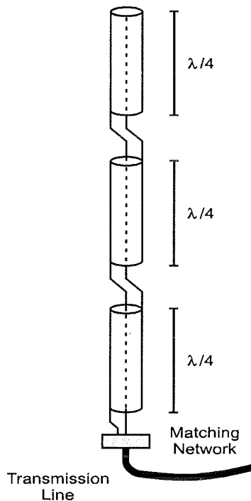
Figure 23. A coaxial collinear array
