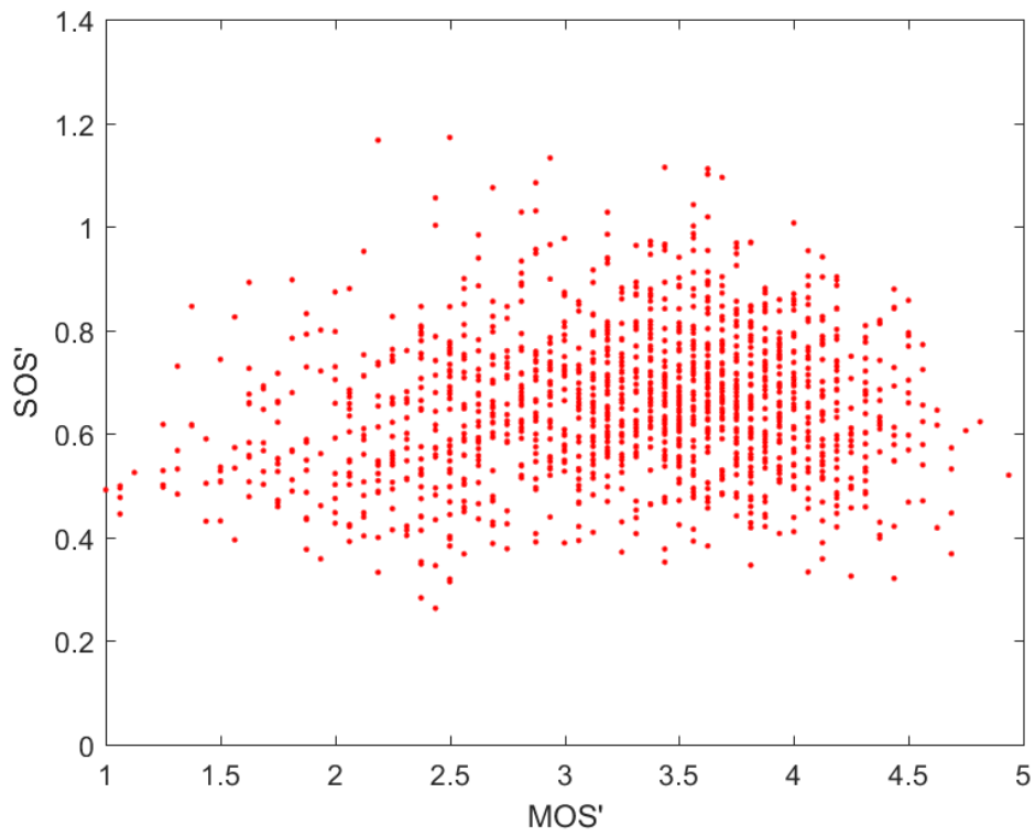
Figure 2. MOS versus SOS computed on raw lab data (top) and after overall bias removed from each subject's scores (bottom). MOS' and SOS' indicate modified values after bias removal.
