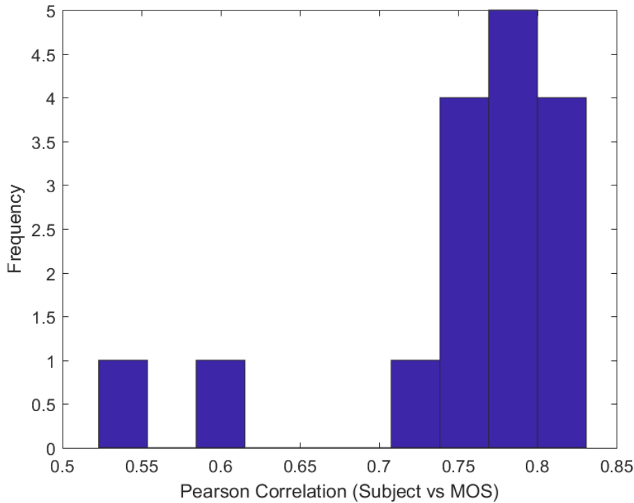
Figure 1. Pearson correlation between each subject's opinion scores and the overall MOS (lab data).
