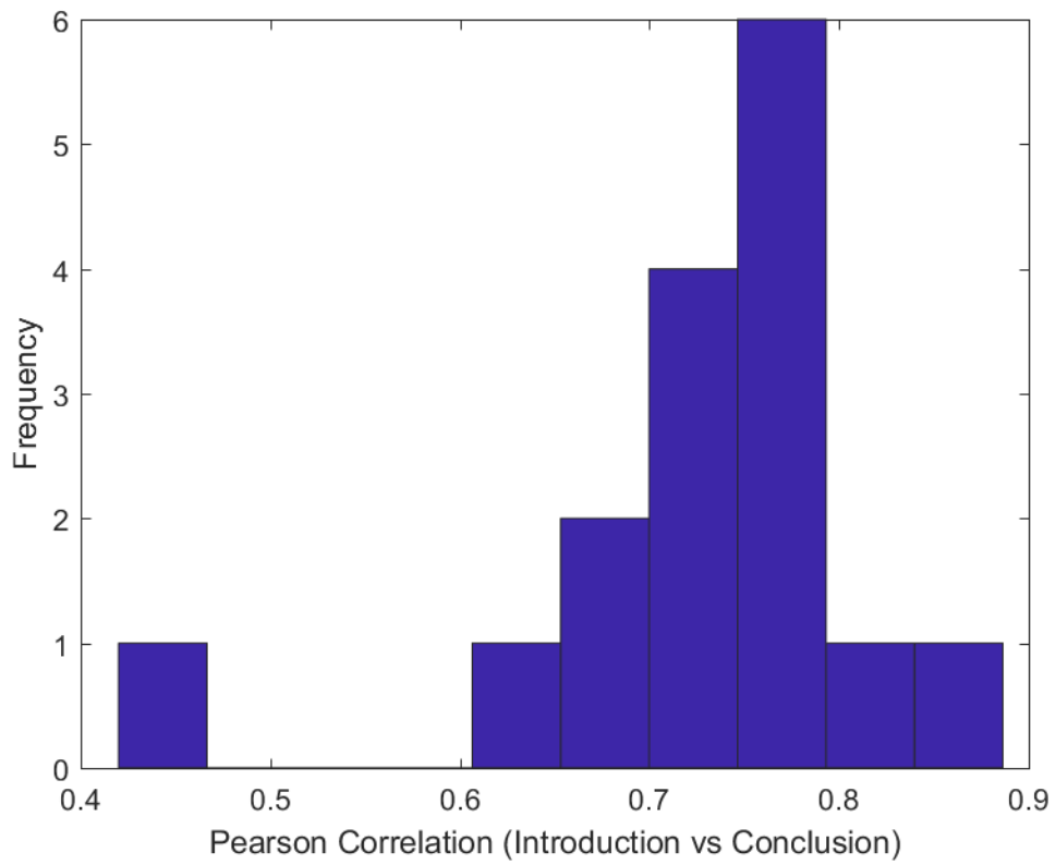
Figure 5. Pearson correlation between each subject's introduction session opinion scores and conclusion session opinion scores (lab data).
