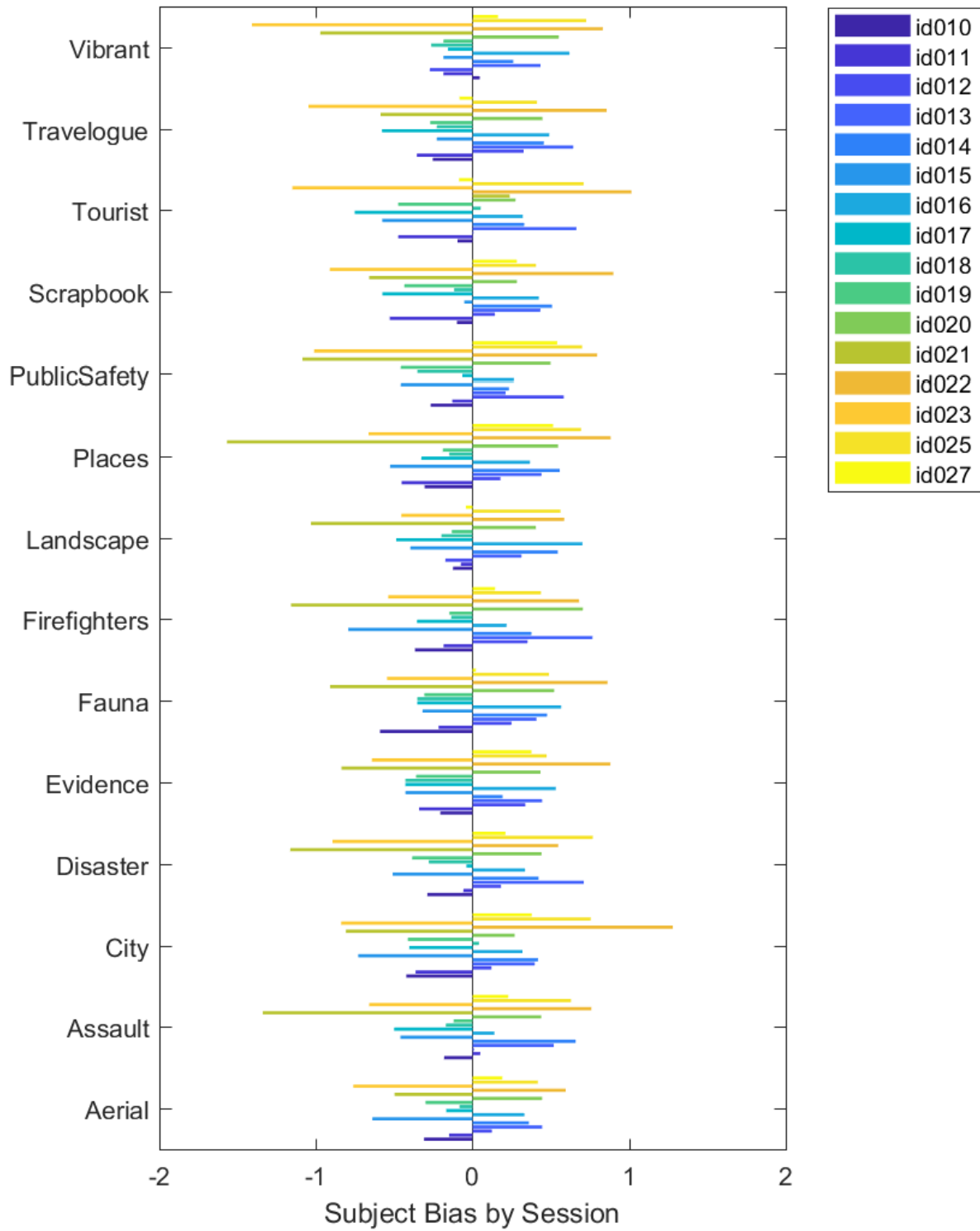
Figure 3. Subject bias for each session, computed on the unprocessed ratings (lab data).
