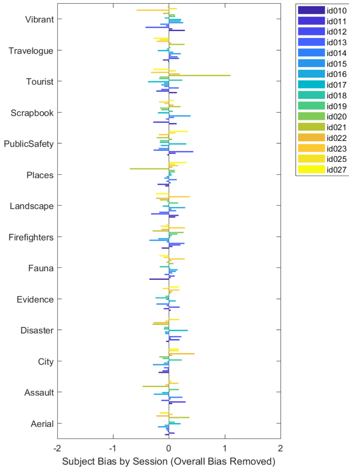
Figure 4. Subject bias for each session, after each subject's overall bias is removed (lab data).
