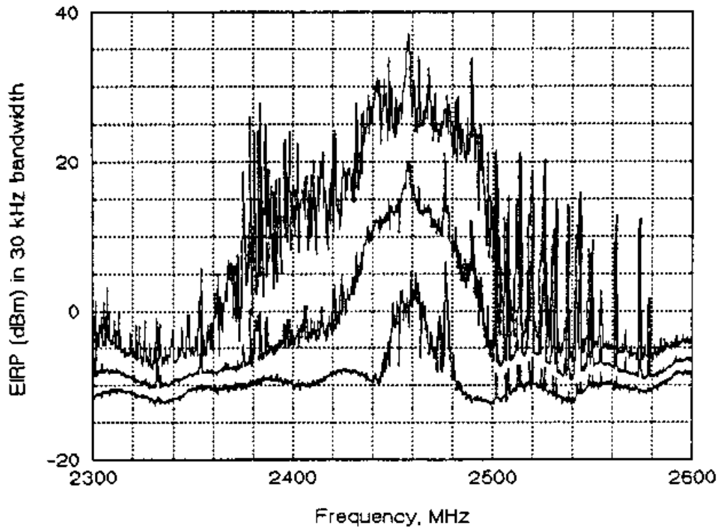
Figure 4-5. ISM environment EIRP for Boulder.
