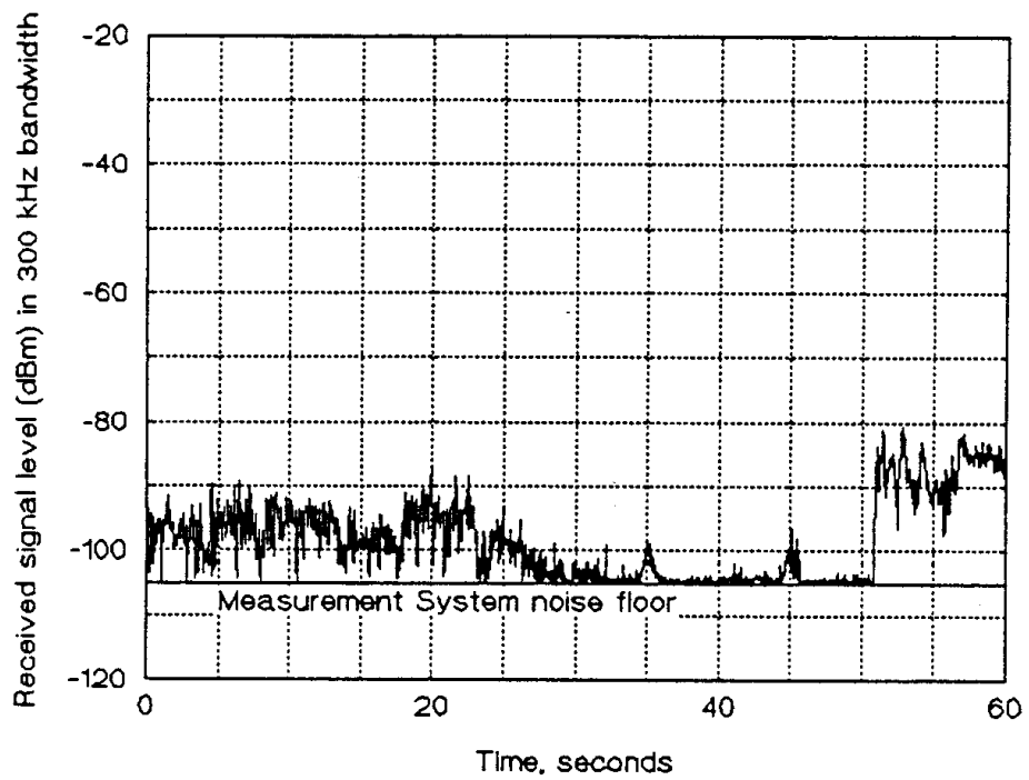
Figure 3-13. 60-Second time waveform outside apartment complex
