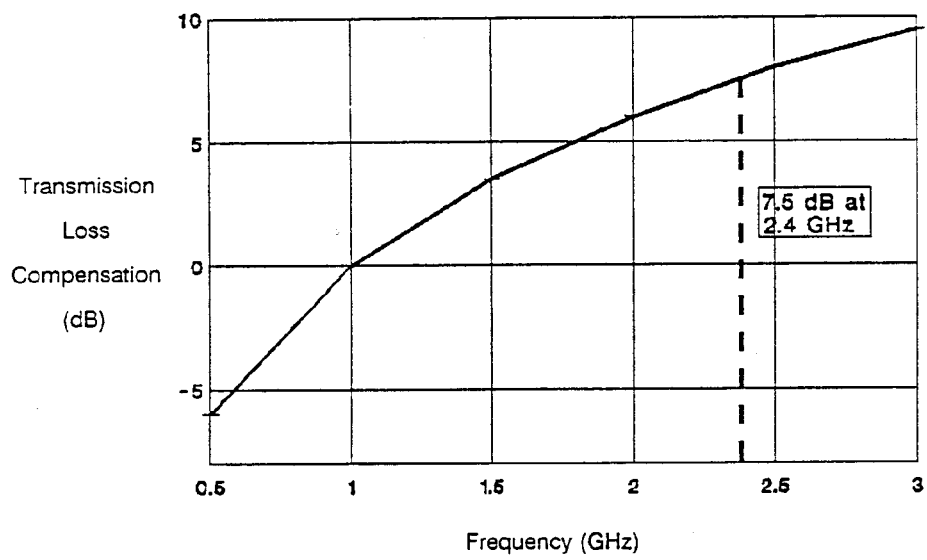
Figure 1. Frequency dependent compensation
