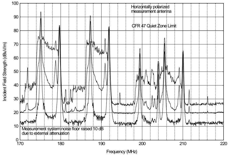
Figure A.38. Table Mountain NRQZ, 170-220 MHz, 10 kHz IF bandwidth, 2,300 sweeps, horizontal polarization.
