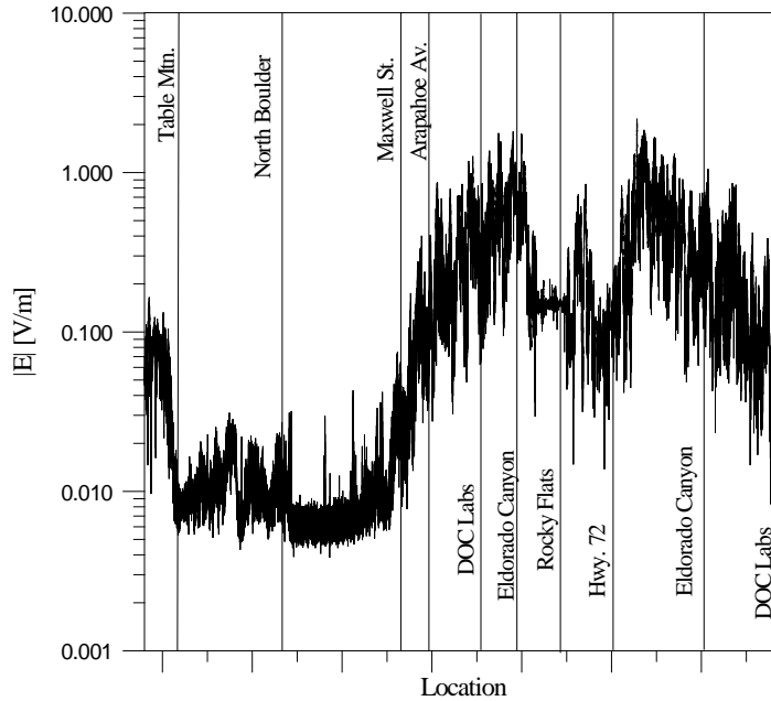
Figure 24. Measured E-field levels scaled to 1 MW EIRP from Table Mountain NRQZ to Highway 72 via Highway 36, Broadway, and Highway 93. These results are for a transmitter on Eldorado Mountain for a frequency of 772 MHz, a transmitter height of 3.66 m (12.0 ft), and a receiver height of 2.95 m (9.68 ft).
