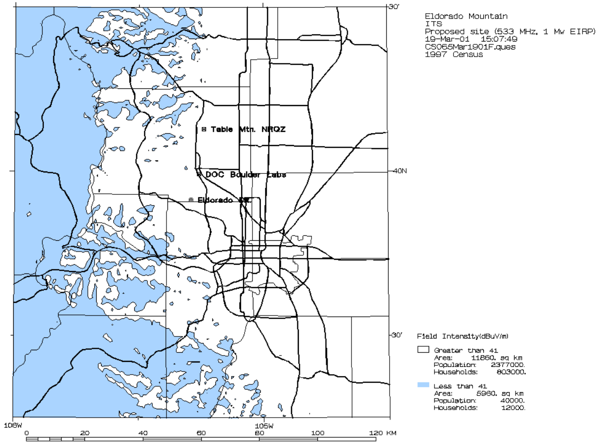
Figure 76. Area coverage plot of the 41 dBµV/m FCC recommendation around the Denver-Boulder area for a horizontally polarized antenna. These results are for a transmitter on Eldorado Mountain for a frequency of 533 MHz, EIRP=1 MW, a transmitter height of 116 m (379 ft), and a receiver height of 9.14 m (30 ft).
