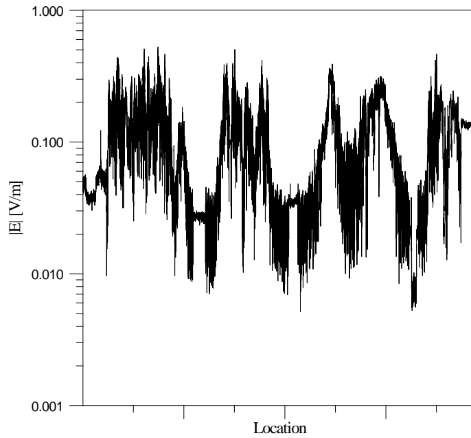
Figure 21. Measured E-field levels scaled to 1 MW EIRP at the DOC Laboratories. These results are for a transmitter on Eldorado Mountain for a frequency of 772 MHz, a transmitter height of 3.66 m (12.0 ft), and a receiver height of 2.95 m (9.68 ft).
