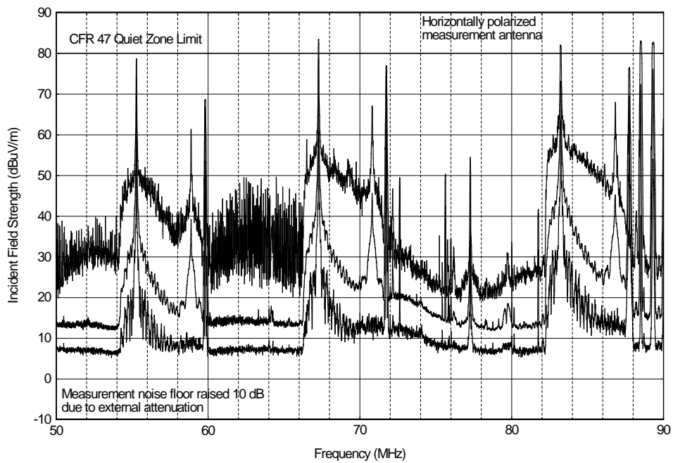
Figure A.35. Table Mountain NRQZ, 50-90 MHz, 10 kHz IF bandwidth, 2,300 sweeps, horizontal polarization.
