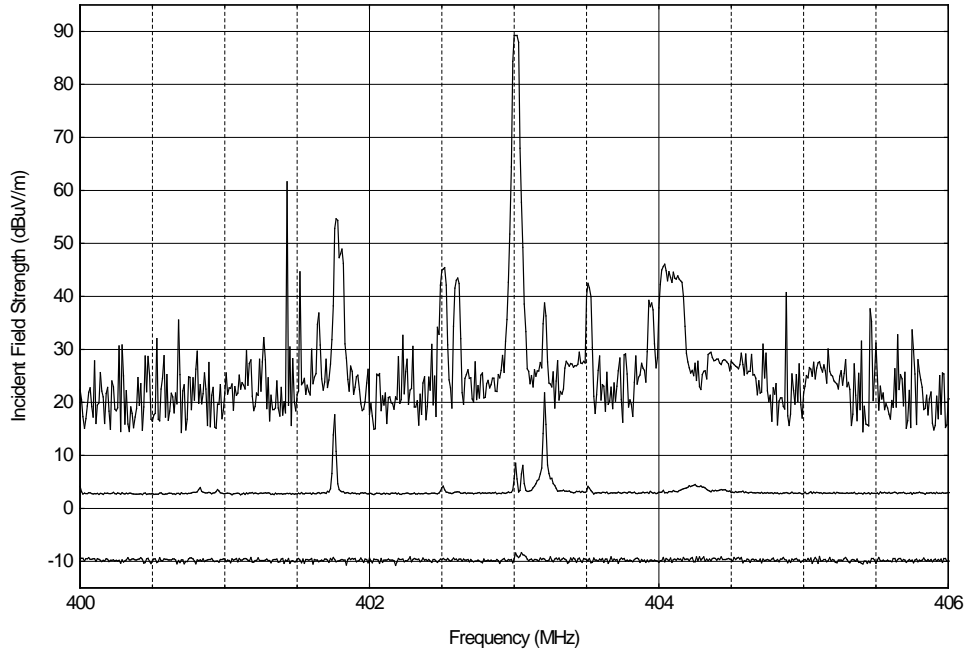
Figure A.26. NIST groundscreen, 400-406 MHz, 58,800 sweeps, vertical polarization.
