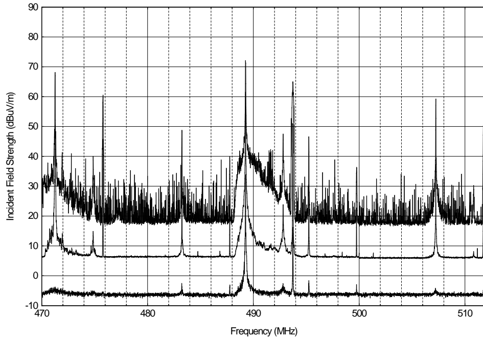
Figure A.30. NIST ground screen, 470-512 MHz, 10 kHz IF bandwidth, 29,000 sweeps, vertical polarization.
