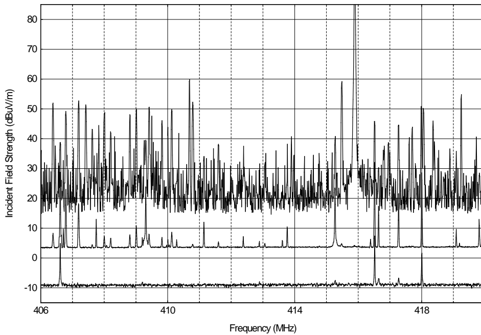
Figure A.27. NIST groundscreen, 406-420 MHz, 10 kHz IF bandwidth, 58,600 sweeps, vertical polarization.
