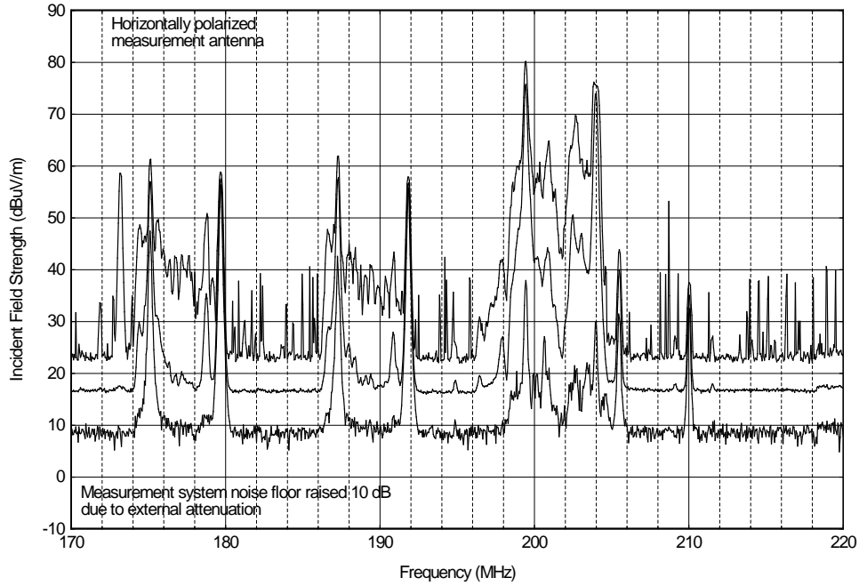
Figure A.40. Bldg. 1, Wing 4, 170-220 MHz, 100 kHz IF bandwidth, 2,100 sweeps, horizontal polarization.
