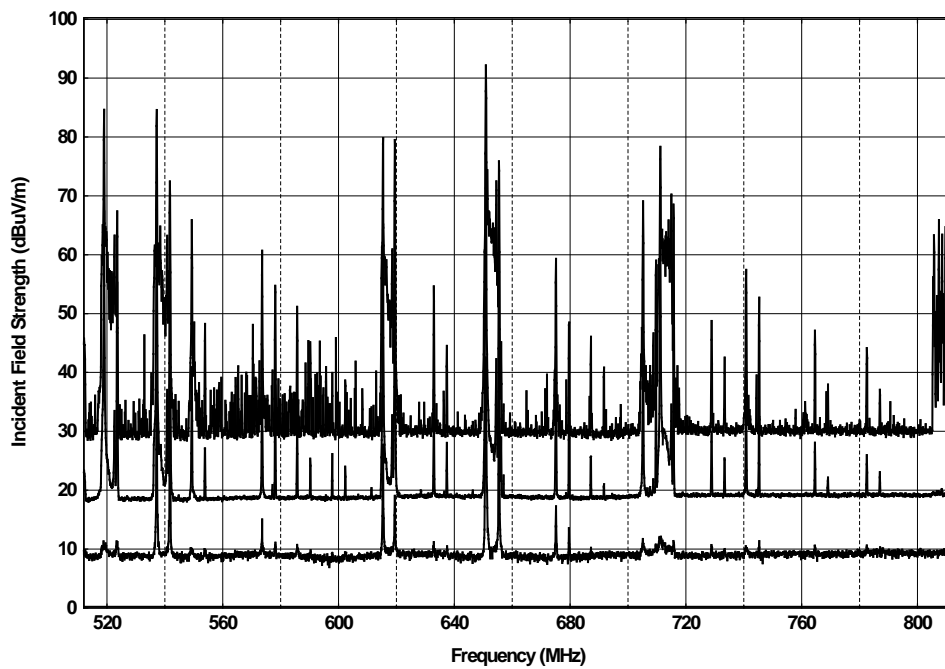
Figure A.31. NIST ground screen, 512-812 MHz, 100 kHz IF bandwidth, 19,200 sweeps, vertical polarization.
