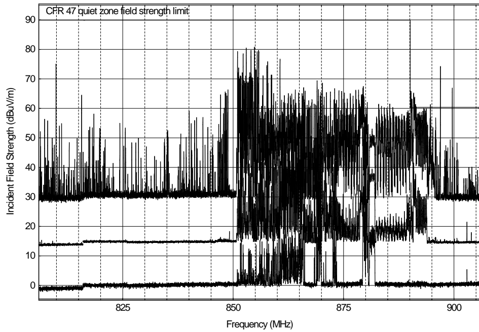
Figure A.15. Table Mountain NRQZ, 806-906 MHz, 10 kHz IF bandwidth, 7,200 sweeps, vertical polarization.
