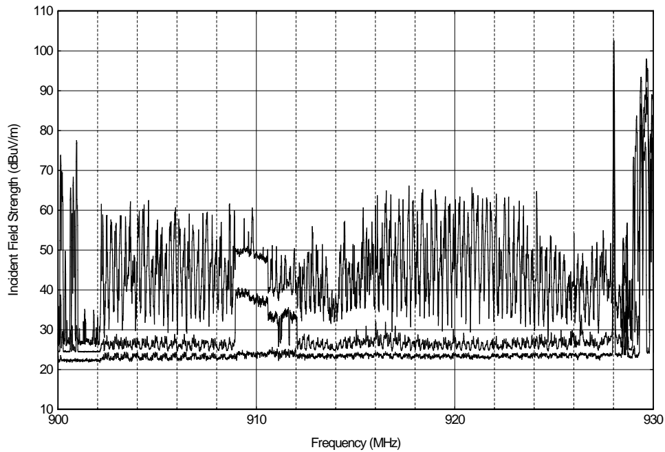
Figure A.33. NIST groundscreen, 900-930 MHz, 10 kHz IF bandwidth, 195 sweeps, vertical polarization.
