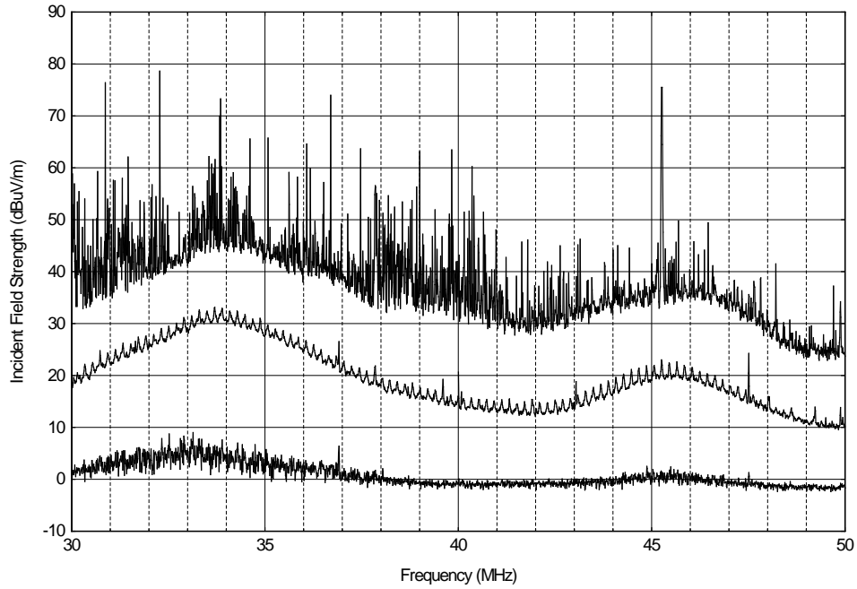
Figure A.18. NIST groundscreen, 30-50 MHz, 10 kHz IF bandwidth, 8,400 sweeps, vertical polarization.
