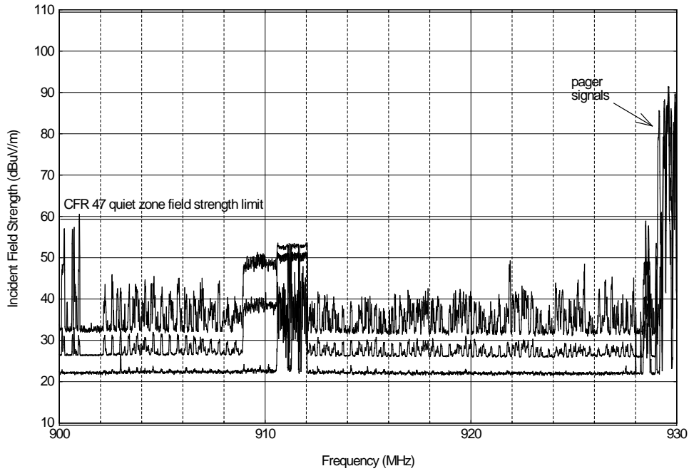
Figure A.16. Table Mountain NRQZ, 900-930 MHz, 10 kHz IF bandwidth, 120 sweeps, vertical polarization.
