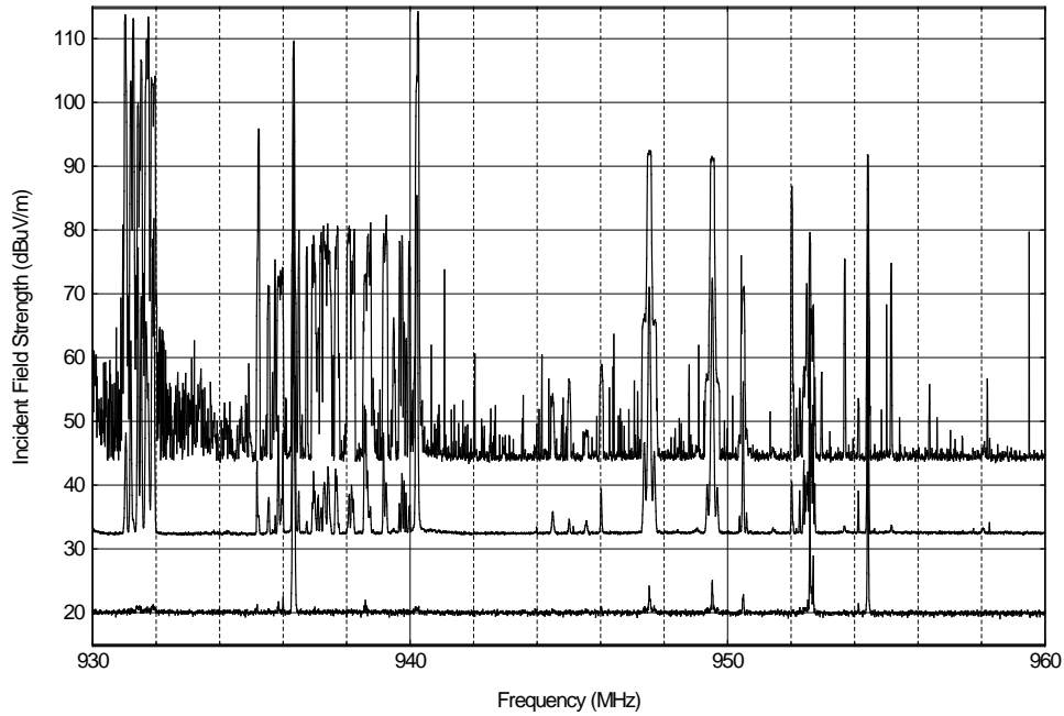
Figure A.34. NIST groundscreen, 930-960 MHz, 10 kHz IF bandwidth, 87,000 sweeps, vertical polarization.
