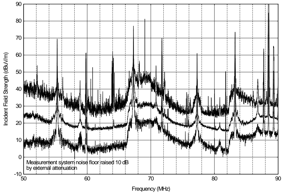
Figure A.36. NIST groundscreen, 50-90 MHz, 10 kHz IF bandwidth, 700 sweeps, horizontal polarization.
