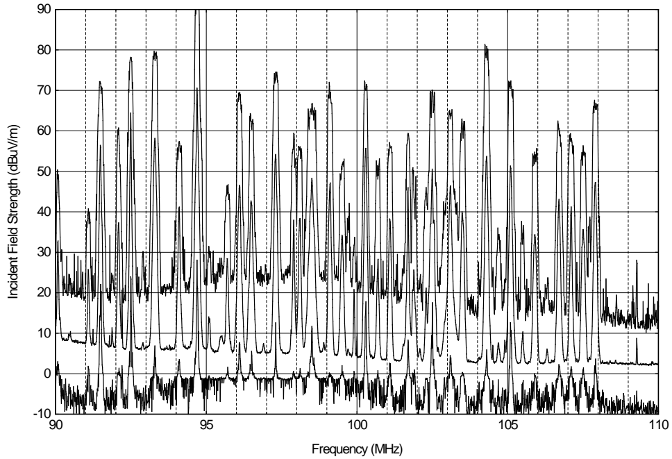
Figure A.20. NIST groundscreen, 90-110 MHz, 10 kHz IF bandwidth, 3,060 sweeps, vertical polarization.
