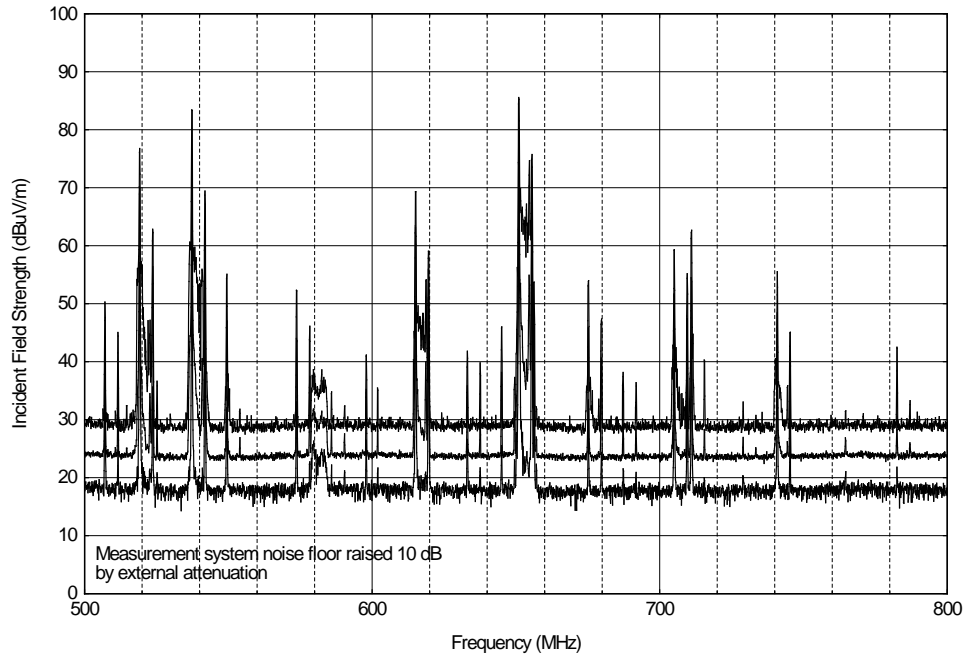
Figure A.42. NIST groundscreen, 500-800 MHz, 100 kHz IF bandwidth, 700 sweeps, horizontal polarization.
