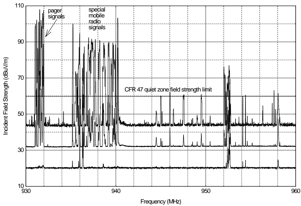
Figure A.17. Table Mountain NRQZ, 930-960 MHz, 53,700 sweeps, vertical polarization.
