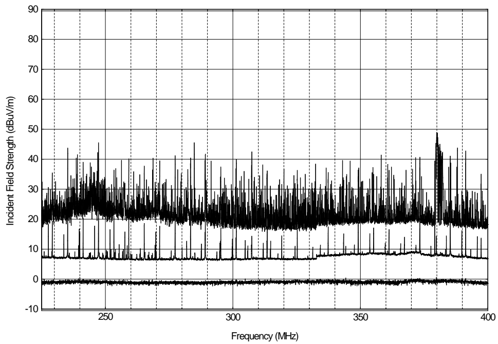
Figure A.25. NIST groundscreen, 225-400 MHz, 30 kHz IF bandwidth, 9,600 sweeps, vertical polarization.
