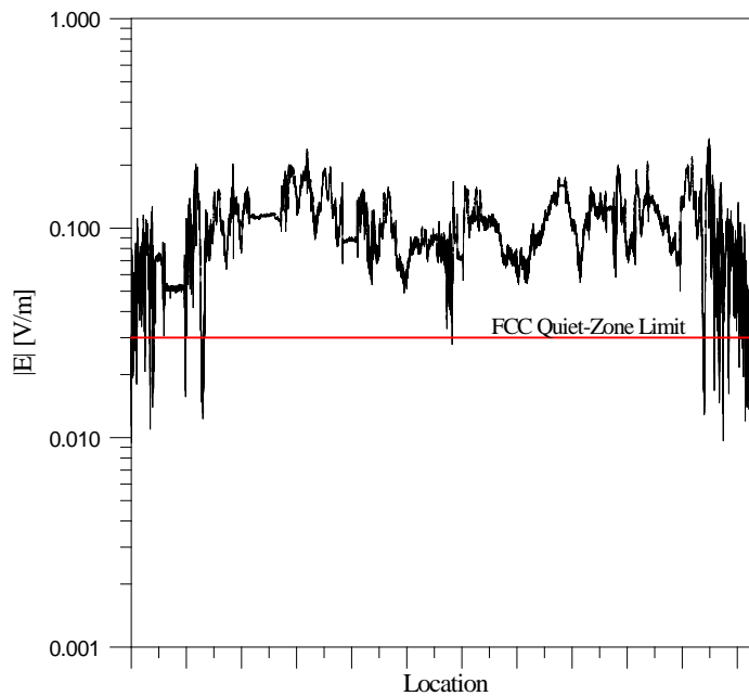
Figure 22. Measured E-field levels scaled to 1 MW EIRP at the Table Mountain NRQZ. These results are for a transmitter on Eldorado Mountain for a frequency of 772 MHz, a transmitter height of 3.66 m (12.0 ft), and a receiver height of 2.95 m (9.68 ft).
