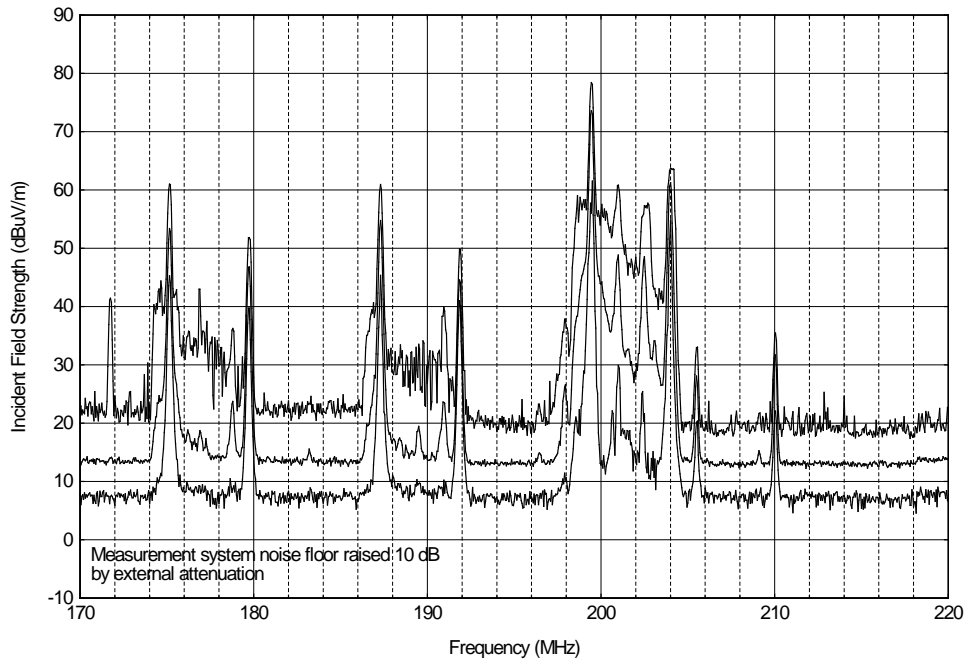
Figure A.39. NIST groundscreen, 170-220 MHz, 100 kHz IF bandwidth, 700 sweeps, horizontal polarization.
