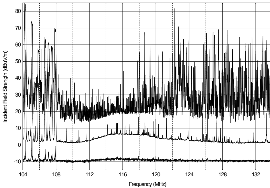
Figure A.21. NIST groundscreen, 104-134 MHz, 10 kHz IF bandwidth, 21,600 sweeps, vertical polarization.
