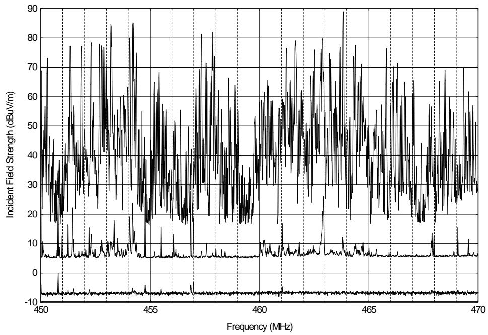
Figure A.29. NIST groundscreen, 450-470 MHz, 10 kHz IF bandwidth, 58,500 sweeps, vertical polarization.
