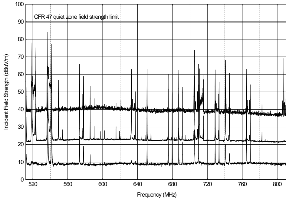
Figure A.14. Table Mountain NRQZ, 512-812 MHz, 100 kHz IF bandwidth, 12,000 sweeps, vertical polarization.
