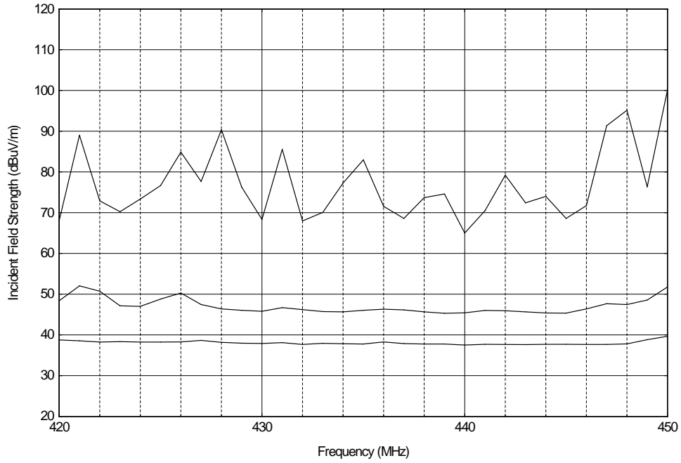
Figure A.28. NIST groundscreen, 420-450 MHz, 1 MHz IF bandwidth, 193 stepped passes, vertical polarization.
