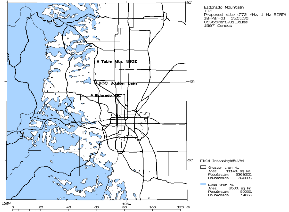
Figure 77. Area coverage plot of the 41 dBµV/m FCC recommendation around the Denver-Boulder area for a horizontally polarized antenna. These results are for a transmitter on Eldorado Mountain for a frequency of 772 MHz, EIRP=1 MW, a transmitter height of 116 m (379 ft), and a receiver height of 9.14 m (30 ft).
