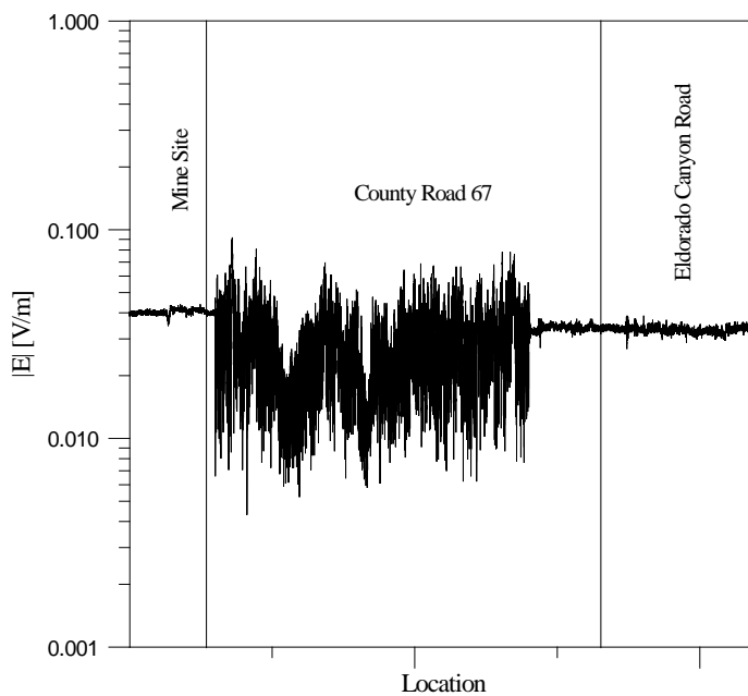
Figure 28. Measured E-field levels scaled to 1 MW EIRP on County Road 67. These results are for a transmitter on Eldorado Mountain for a frequency of 772 MHz, a transmitter height of 3.66 m (12.0 ft), and a receiver height of 2.95 m (9.68 ft).
