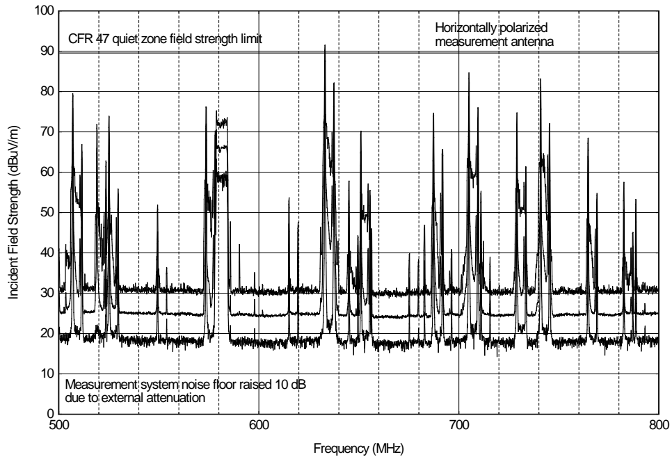
Figure A.41. Table Mountain NRQZ, 500-800 MHz, 100 kHz IF bandwidth, 2,300 sweeps, horizontal polarization.
