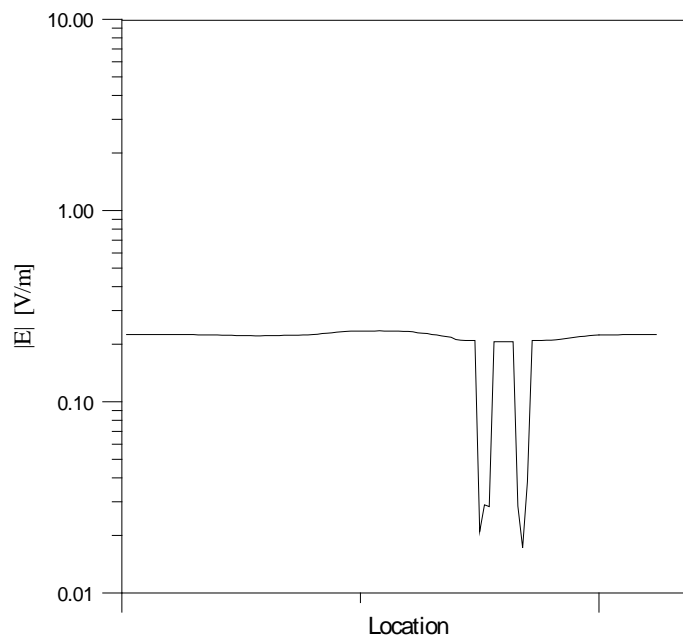
Figure 56. Modeled (or predicted) E-field levels at the Table Mountain NRQZ. These results are for a transmitter on Eldorado Mountain for a frequency of 533 MHz, EIRP=1 MW, a transmitter height of 3.66 m (12 ft), and a receiver height of 2.95 m (9.68 ft).
