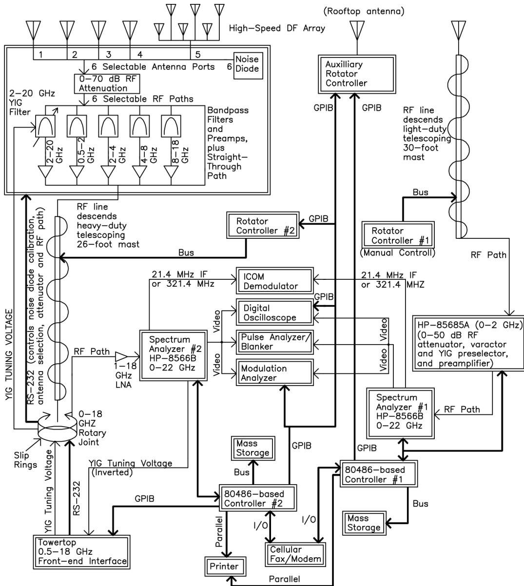
Figure 6. Block diagram of the RSMS measurement system.
