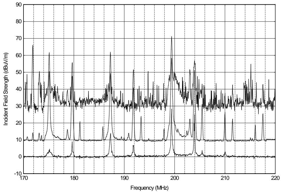
Figure A.23. NIST groundscreen, 170-220 MHz, 100 kHz IF bandwidth, 50,000 sweeps, vertical polarization.
