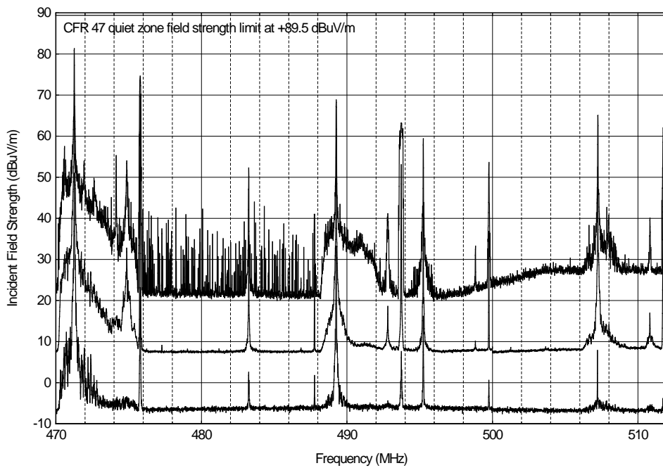
Figure A.13. Table Mountain NRQZ, 470-512 MHz, 10 kHz IF bandwidth, 18,000 sweeps, vertical polarization.
