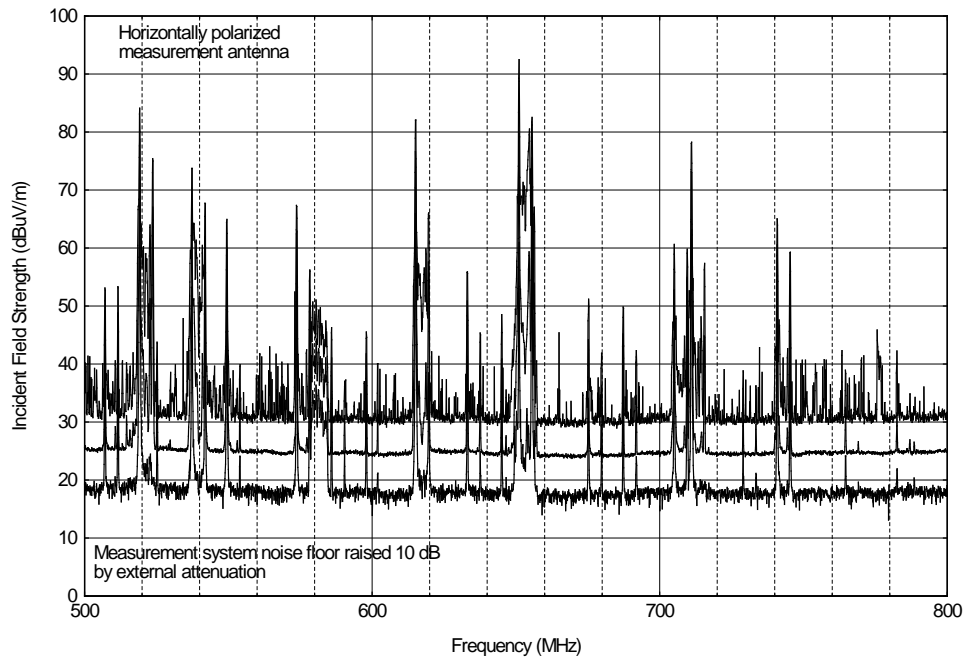
Figure A.43. Bldg. 1, Wing 4, 500-800 MHz, 100 kHz IF bandwidth, 2,100 sweeps, horizontal polarization.
