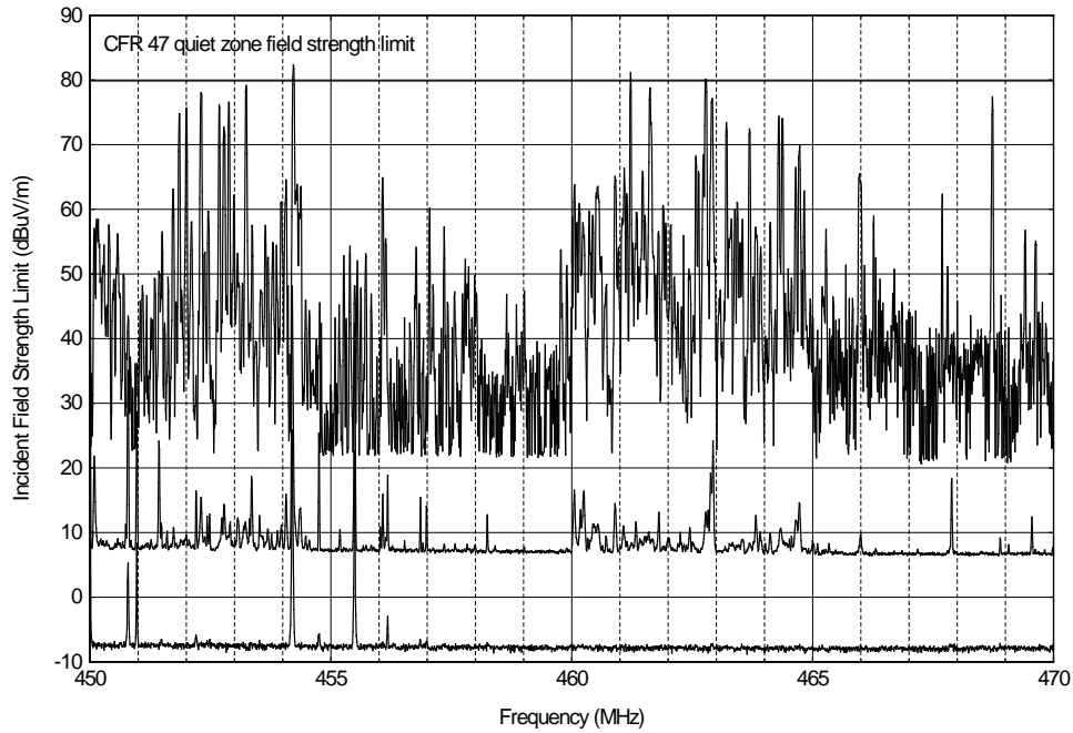
Figure A.12. Table Mountain NRQZ, 450-470 MHz, 10 kHz IF bandwidth, 36,300 sweeps, vertical polarization.
