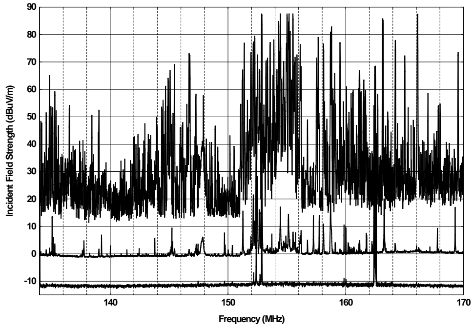
Figure A.22. NIST groundscreen, 134-170 MHz, 10 kHz IF bandwidth, 21,600 sweeps, vertical polarization.
