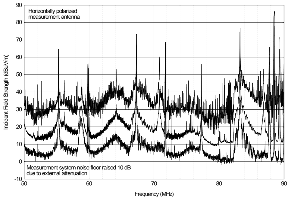
Figure A.37. Bldg. 1, Wing 4, 50-90 MHz, 10 kHz IF bandwidth, 2,100 sweeps, horizontal polarization.
