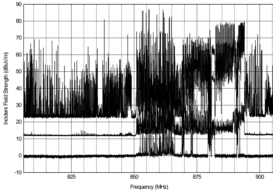
Figure A.32. NIST groundscreen, 806-906 MHz, 10 kHz IF bandwidth, 11,760 sweeps, vertical polarization.
