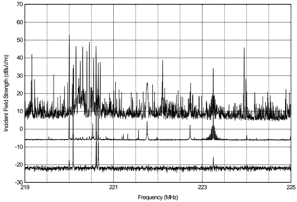
Figure A.24. NIST groundscreen, 219-225 MHz, 3 kHz IF bandwidth, 11,760 sweeps, vertical polarization.
