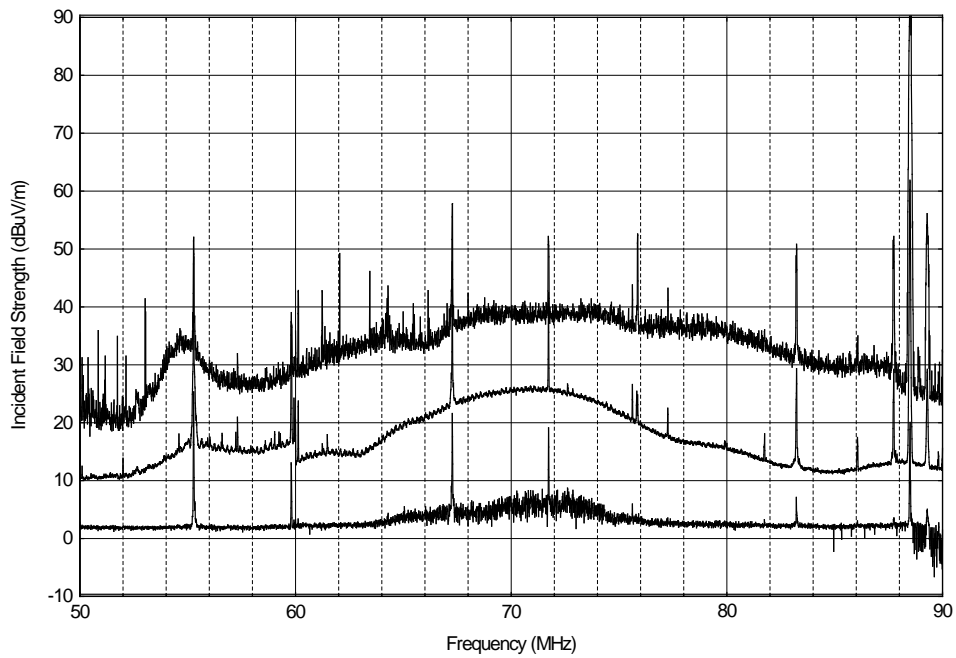
Figure A.19. NIST groundscreen, 50-90 MHz, 10 kHz IF bandwidth, 3,060 sweeps, vertical polarization.
