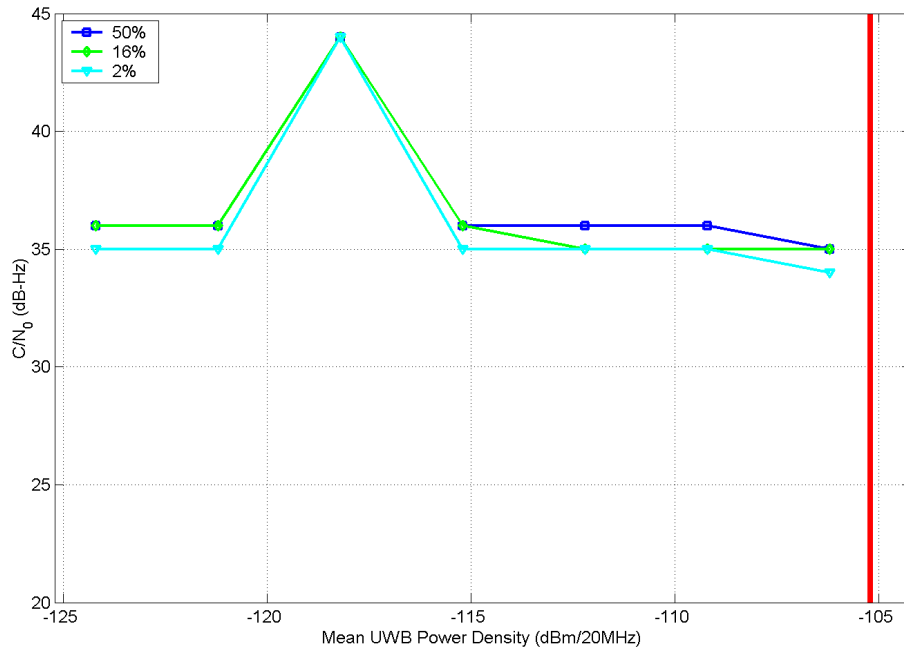
Figure B.2.10. Measured GPS parameters (Rx 4) as a function of 20-MHz PRF, OOK, non-gated UWB interference.
