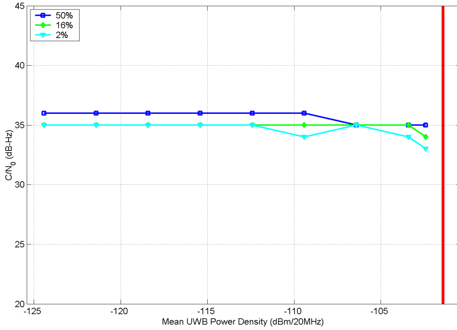
Figure B.2.4. Measured GPS parameters (Rx 4) as a function of 5-MHz PRF, UPS, non-gated UWB interference.
