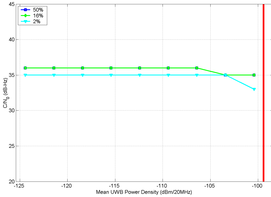
Figure B.2.12. Measured GPS parameters (Rx 4) as a function of 5-MHz PRF, OOK, non-gated UWB interference.
