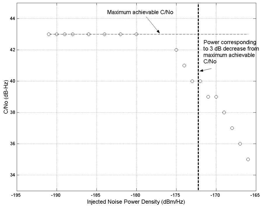
Figure 2.3. C/N_o receiver output versus injected noise power density for Rx 4.
