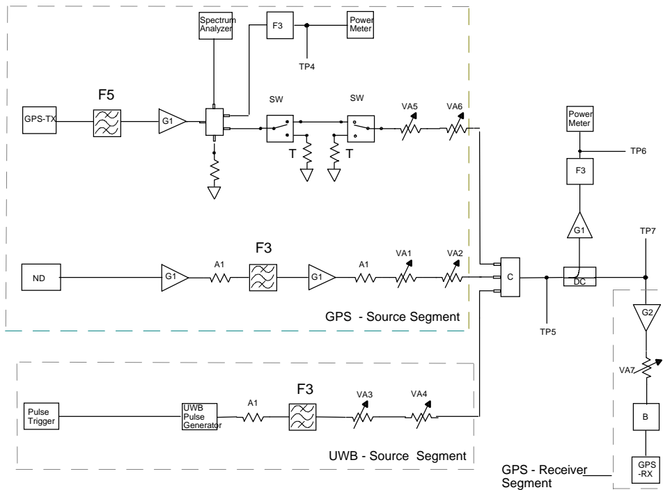
Figure 2.1. Block diagram.
