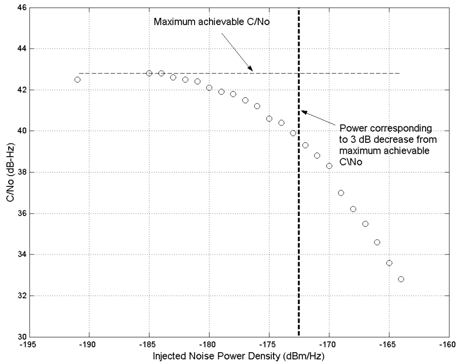
Figure 2.2. C/N_o receiver output versus injected noise power density for Rx 3.
