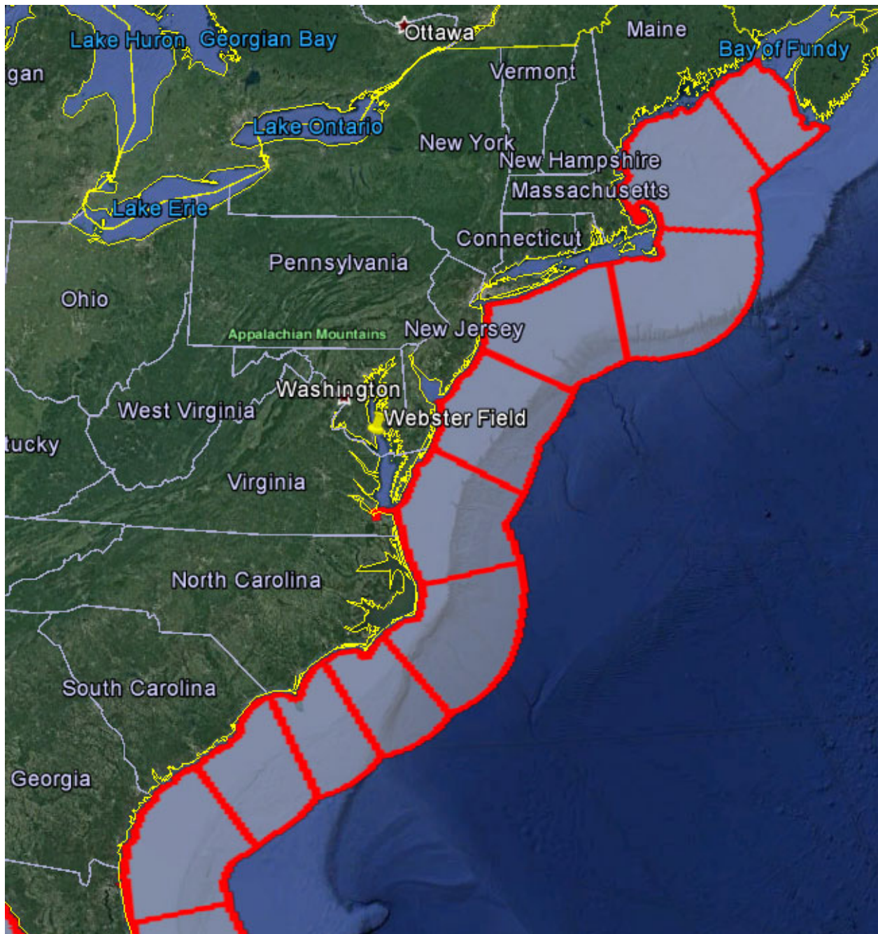
Figure 57. Shipborne Radar Dynamic coordination zones for the Eastern Coast of the United States
