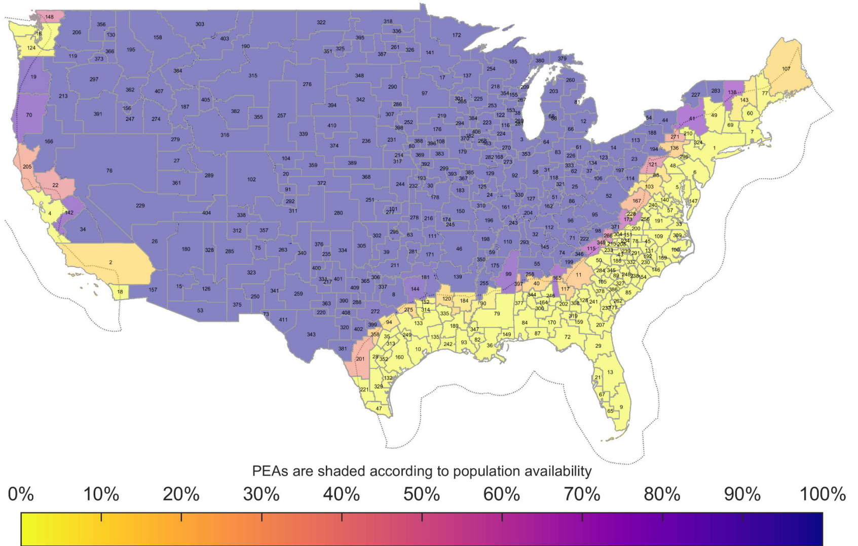
Figure 119. BS Shipborne Exclusion Zone Population Availability: BS EIRP: 47 dBm/10 MHz, AP EIRP: 30 dBm/10 MHz IMT-Advanced Deployment
