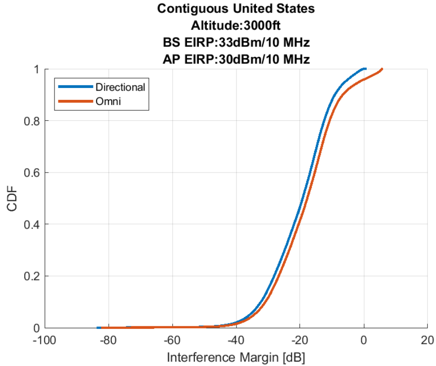
Figure 35. Airborne 1-2: Cumulative Distribution Function of the Interference Margin 100 Megahertz Sharing Option, 3,000ft (AGL) Altitude
