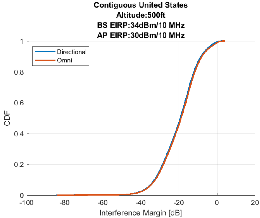
Figure 23. Airborne 1-2: Cumulative Distribution Function of the Interference Margin 100 Megahertz Sharing Option, 500 ft (AGL) Altitude
