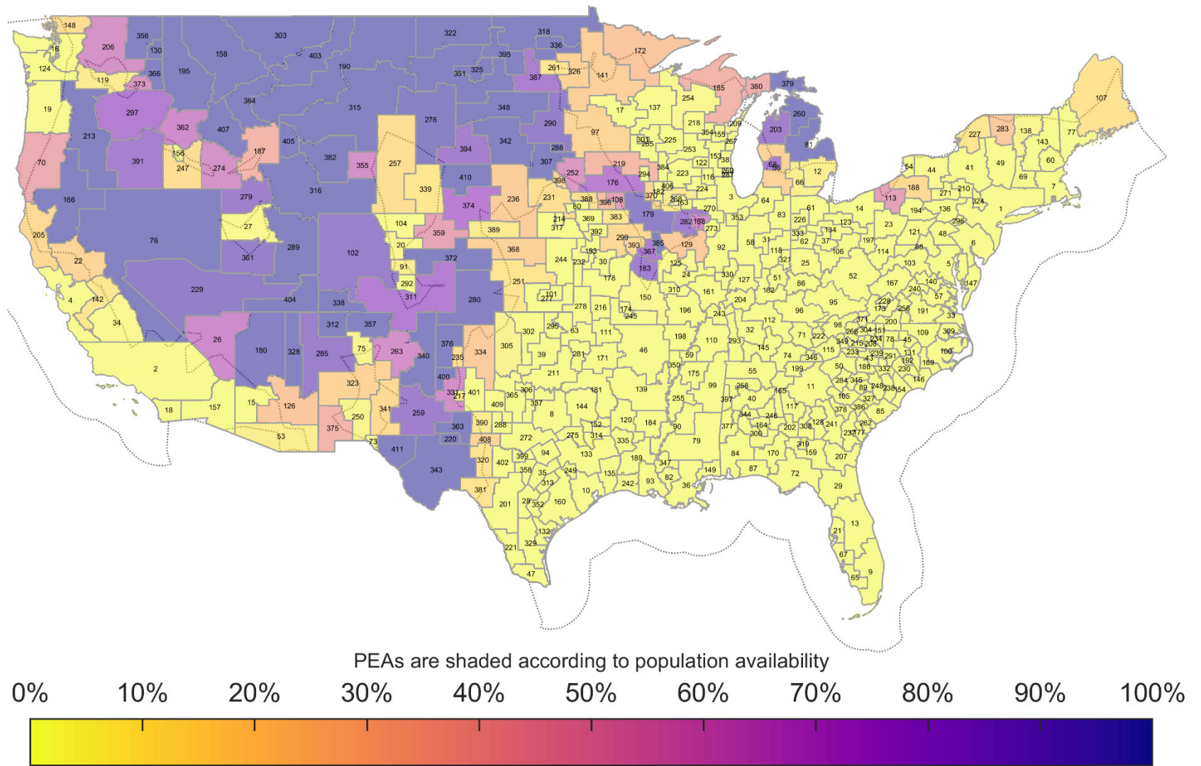
Figure 82. IMT-Advanced Deployment Accessibility: BS EIRP: 61 dBm/10 MHz 100 Megahertz Sharing Option
