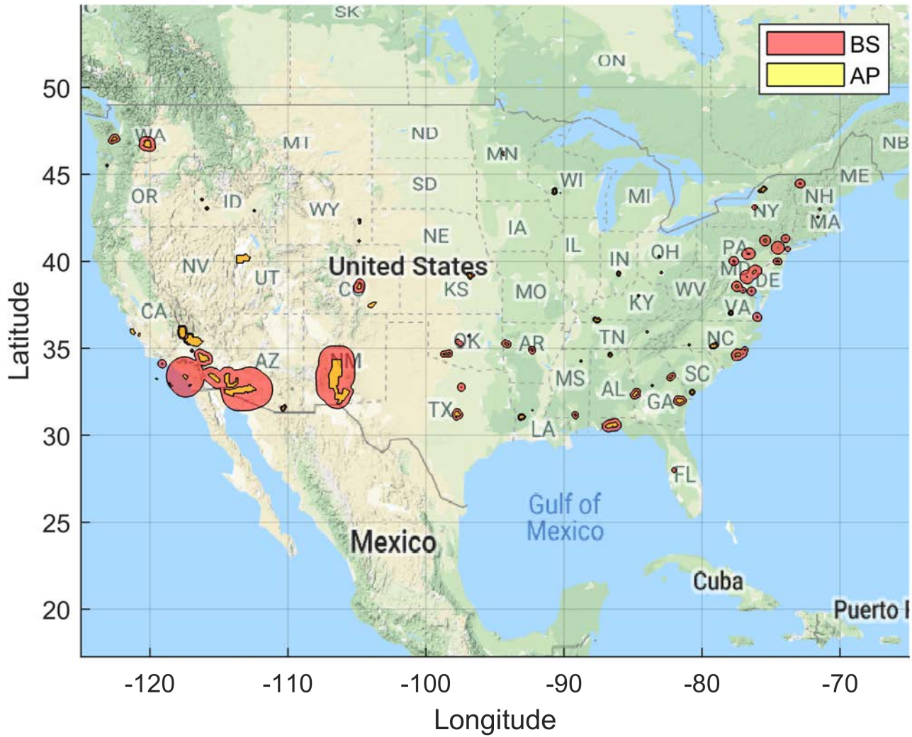
Figure 41. Ground Based Dynamic Coordination Zone Neighborhood: BS EIRP: 47 dBm/10 MHz, AP EIRP: 30 dBm/10 MHz 30 Megahertz Sharing Option and IMT-Advanced Deployment
