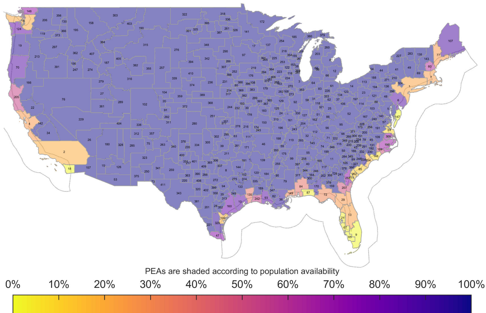
Figure 114. AP Shipborne Exclusion Zone Population Availability: BS EIRP: 47 dBm/10 MHz, AP EIRP: 30 dBm/10 MHz Population Deployment
