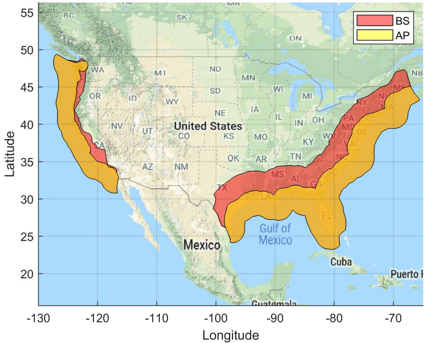
Figure 52. Shipborne Exclusion Zone: BS EIRP: 61 dBm/10 MHz, AP EIRP: 47 dBm/10 MHz Population Deployment
