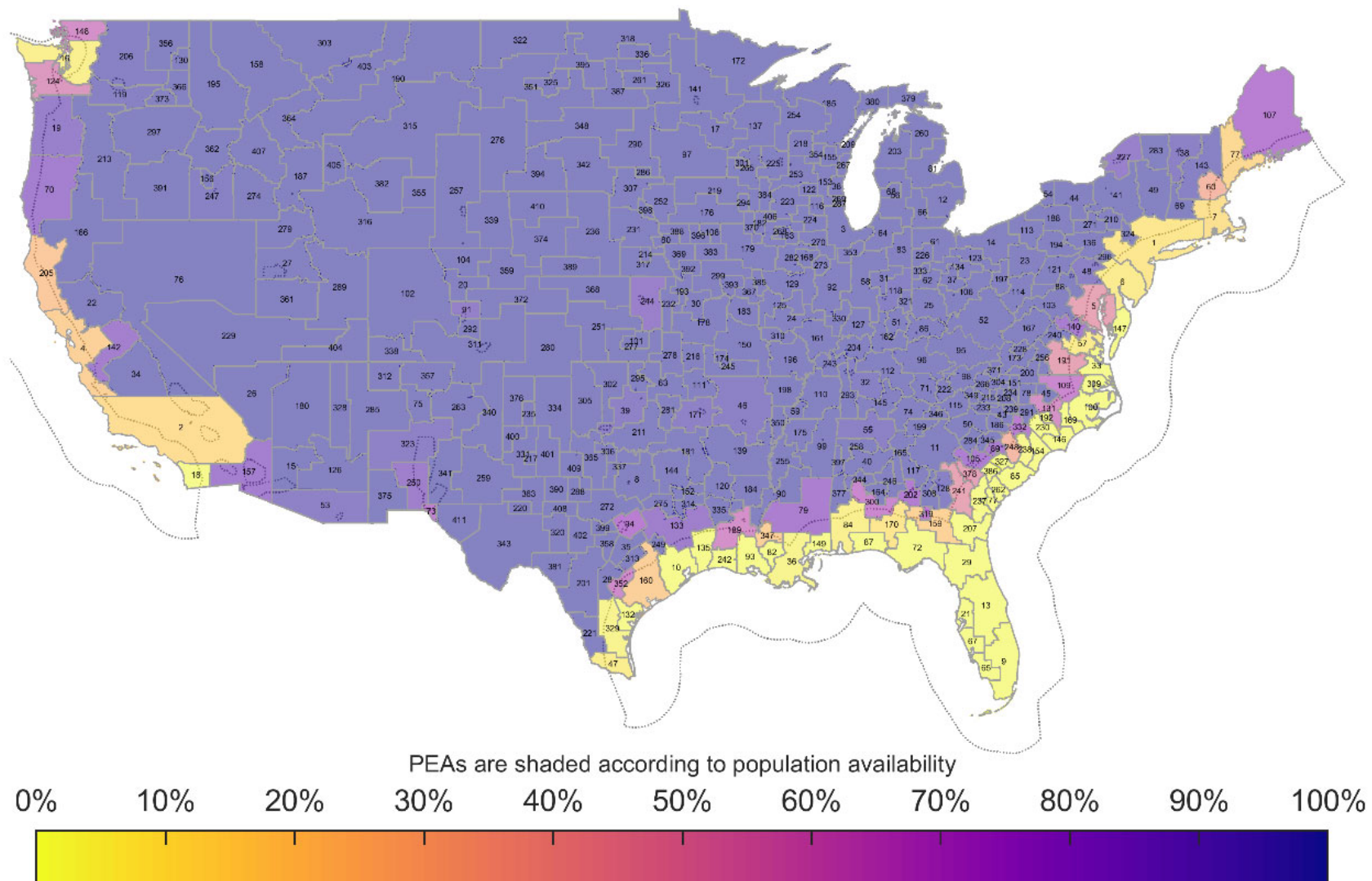
Figure 70. Population Based Deployment Accessibility: AP EIRP: 47 dBm/10 MHz 30 Megahertz Sharing Option
