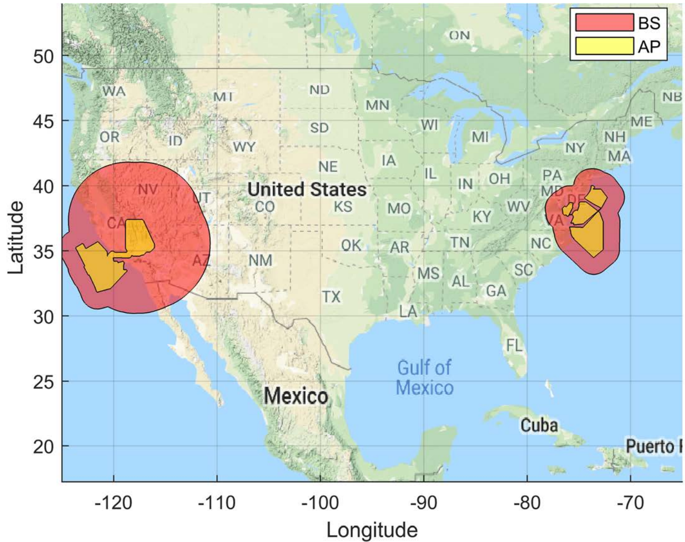
Figure 18. Airborne 3 Dynamic Coordination Zone Neighborhood: BS EIRP: 61 dBm/10 MHz, AP EIRP: 47 dBm/10 MHz, 100 Megahertz Sharing Option and Population Deployment
