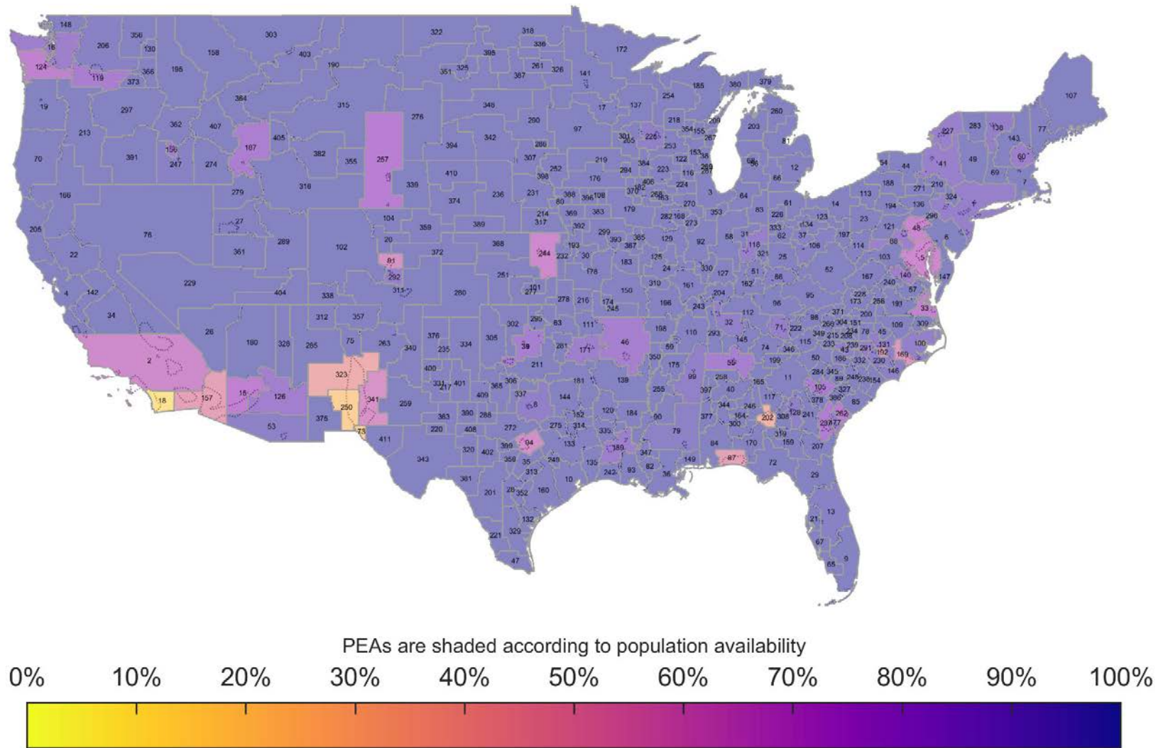
Figure 71. BS Ground Based Exclusion Zone Population Availability BS EIRP: 47 dBm/10 MHz, AP EIRP: 30 dBm/10 MHz 30 Megahertz Sharing Option, IMT-Advanced Deployment
