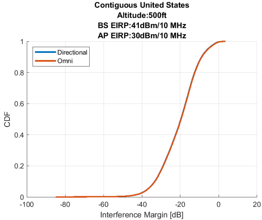
Figure 3. Airborne 1-2: Cumulative Distribution Function of the Interference Margin 30 Megahertz Sharing Option, 500 ft (AGL) Altitude
