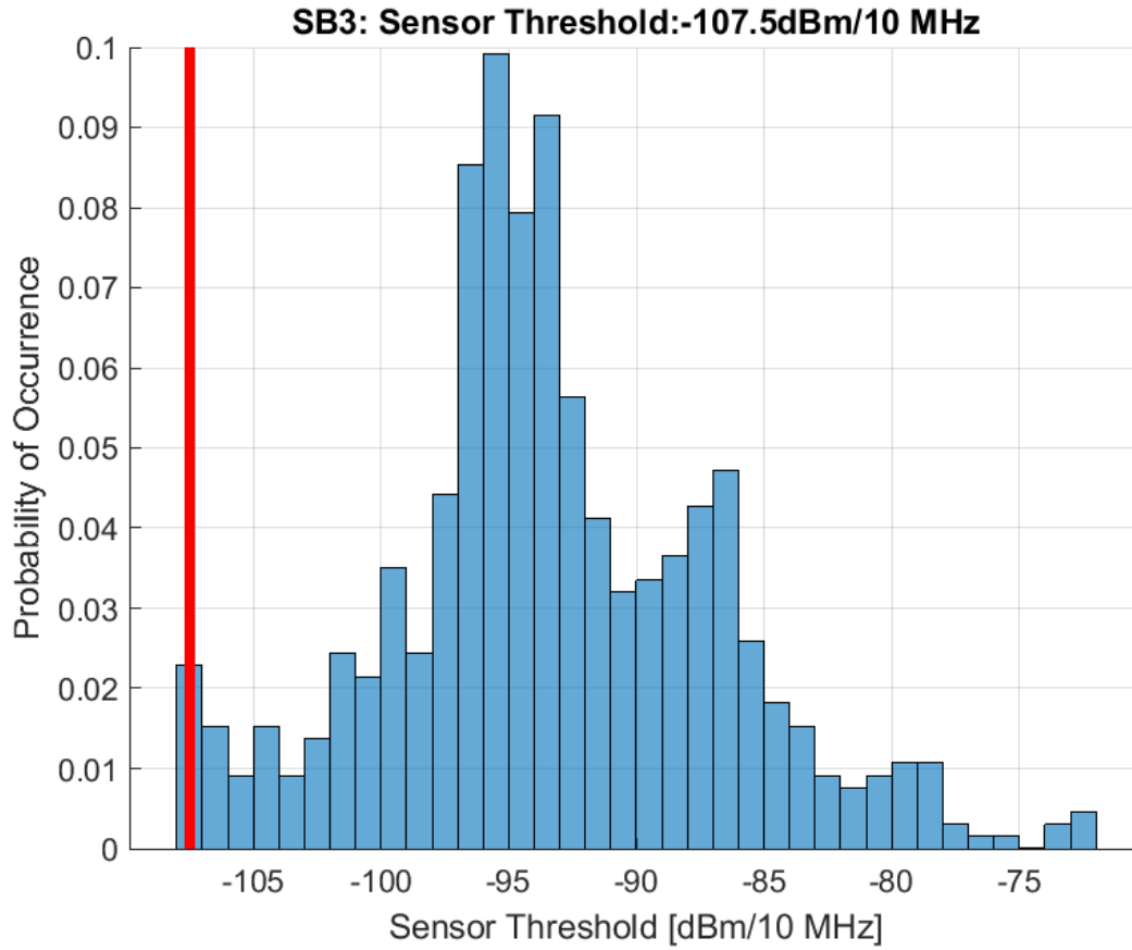
Figure 142. Sensor Detection Threshold BS EIRP: 61 dBm/10 MHz, AP EIRP: 47 dBm/10 MHz IMT-Advanced Deployment
