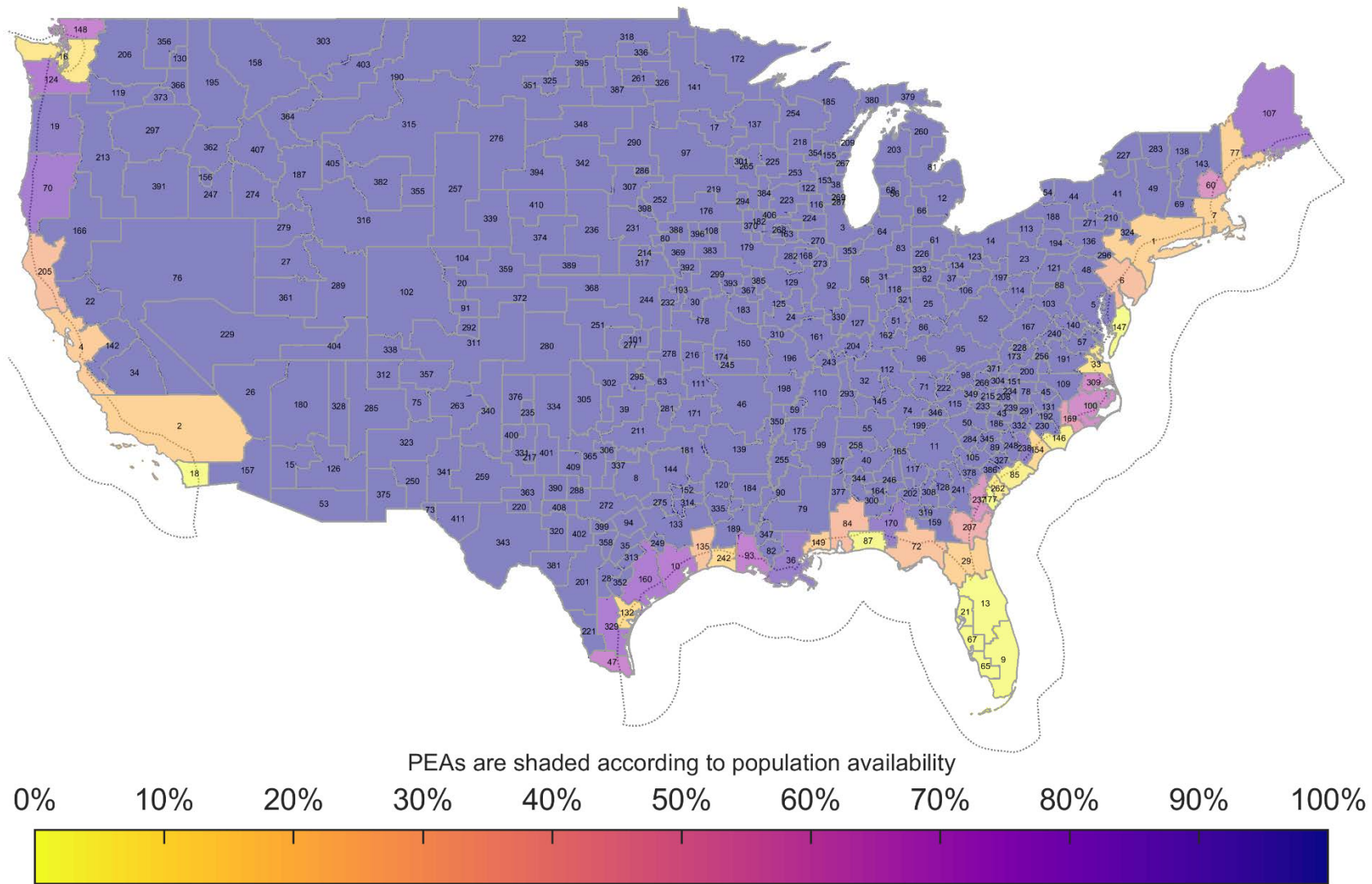
Figure 116. AP Shipborne Exclusion Zone Population Availability: BS EIRP: 47 dBm/10 MHz, AP EIRP: 36 dBm/10 MHz Population Deployment
