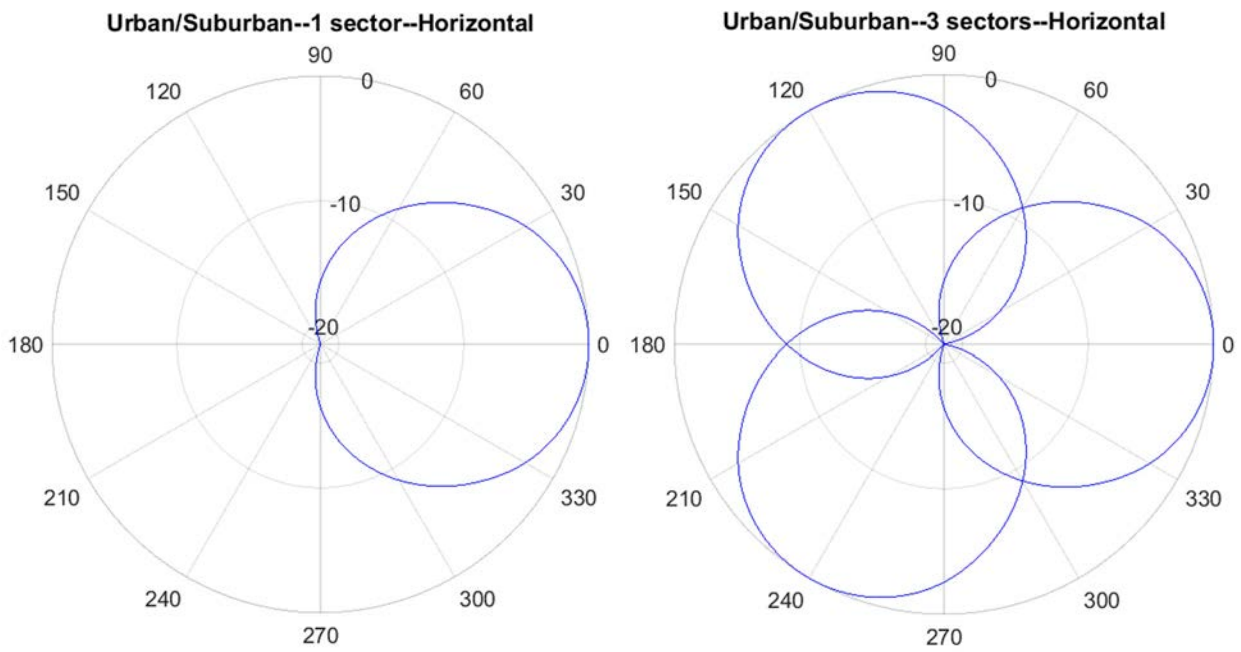
Figure 3. Urban and Suburban Horizontal Antenna Gain Pattern
