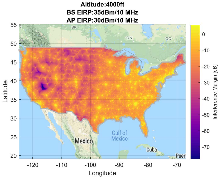
Figure 40. Airborne 1-2: Geographical Interference Margin 100 Megahertz Sharing Option, 4,000ft (AGL) Altitude
