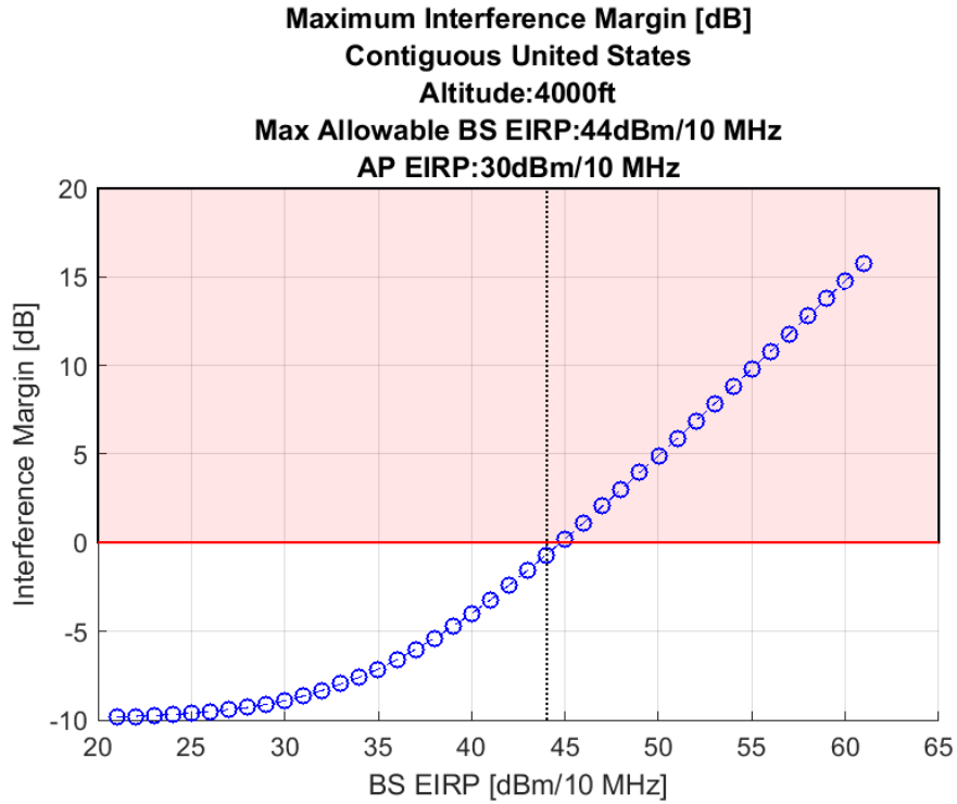
Figure 17. Airborne 1-2: Maximum Allowable EIRP 30 Megahertz Sharing Option, 4,000 ft (AGL) Altitude
