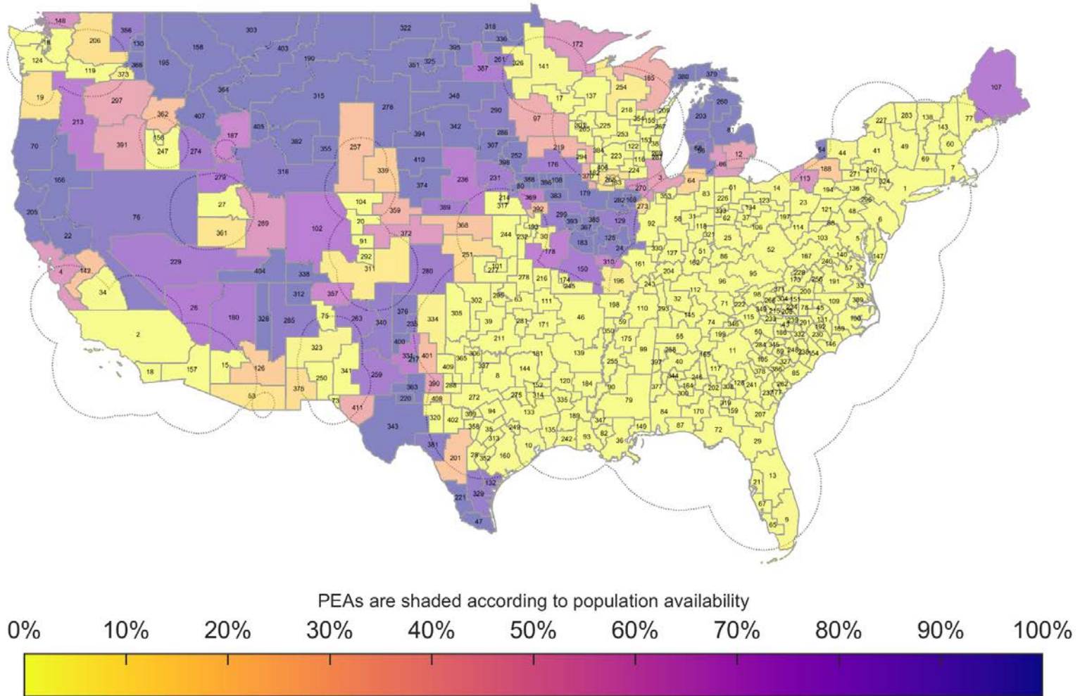
Figure 107. BS Dynamic Coordination Zone Neighborhood Population Availability BS EIRP: 47 dBm/10 MHz, AP EIRP: 30 dBm/10 MHz 100 Megahertz Sharing Option, IMT-Advanced Deployment
