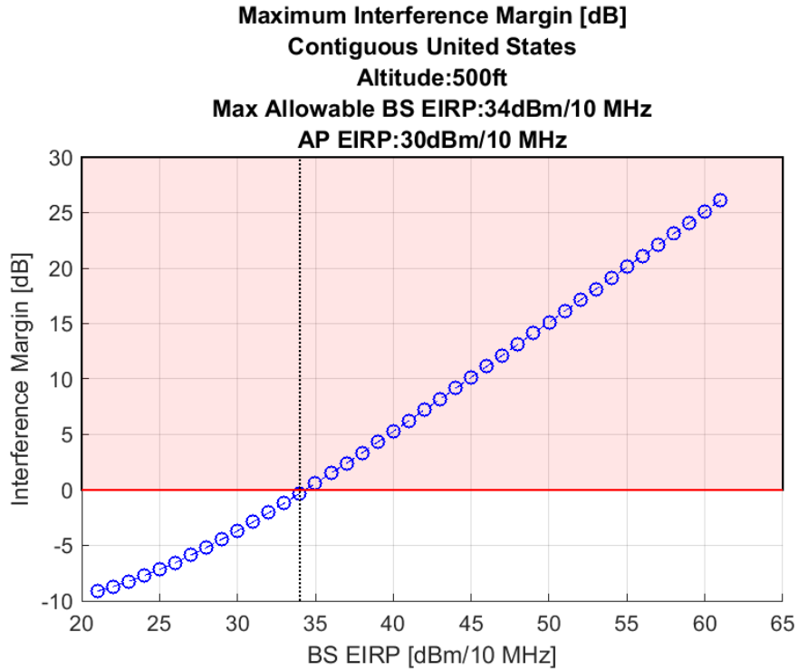
Figure 21. Airborne 1-2: Maximum Allowable EIRP 100 Megahertz Sharing Option, 500 ft (AGL) Altitude
