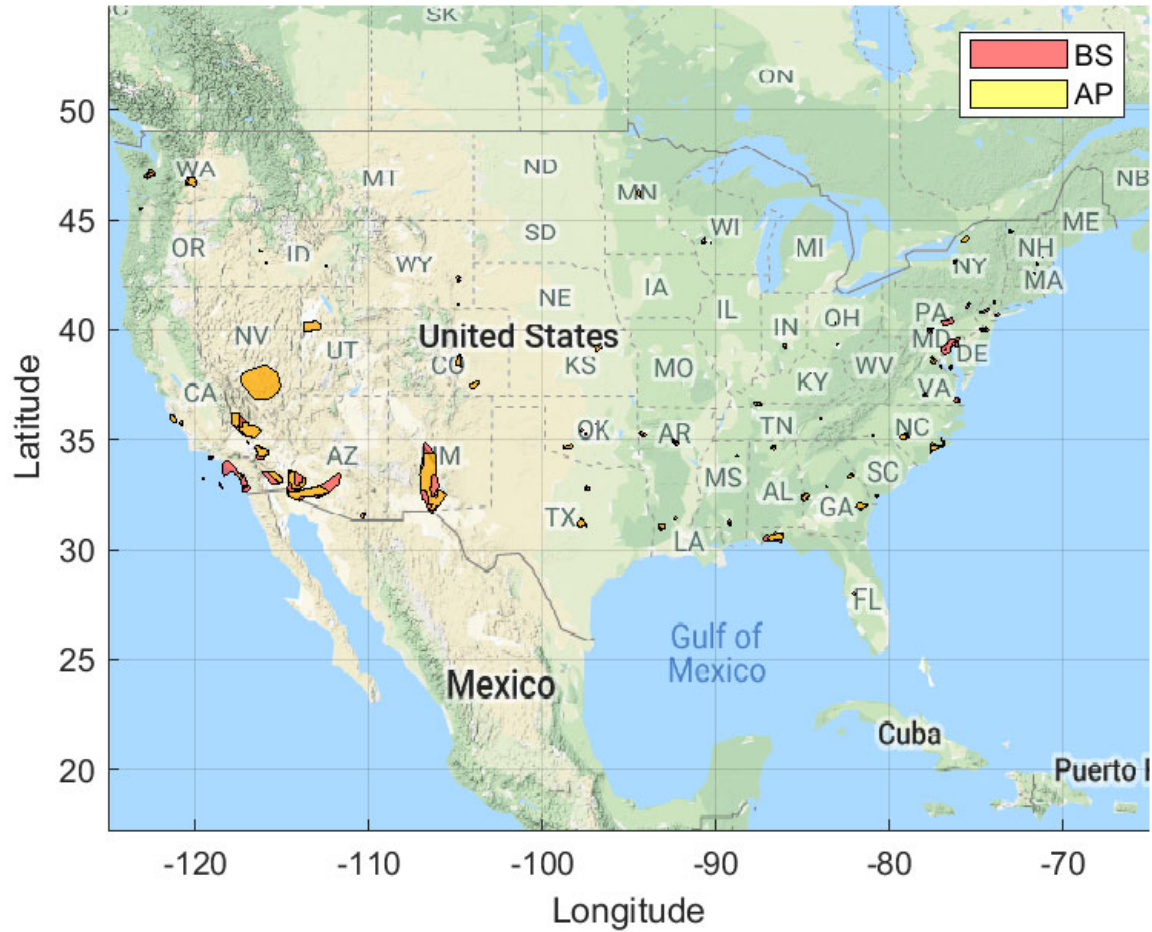
Figure 27. Ground Based Exclusion Zone: BS EIRP: 47 dBm/10 MHz, AP EIRP: 30 dBm/10 MHz 30 Megahertz Sharing Option and IMT-Advanced Deployment
