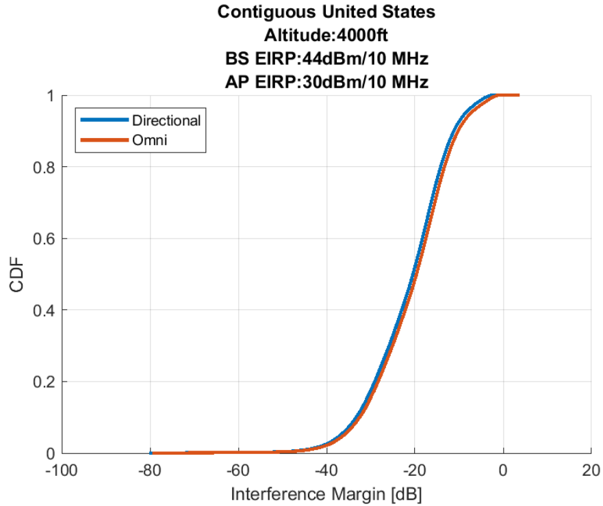
Figure 19. Airborne 1-2: Cumulative Distribution Function of the Interference Margin 30 Megahertz Sharing Option, 4,000ft (AGL) Altitude
