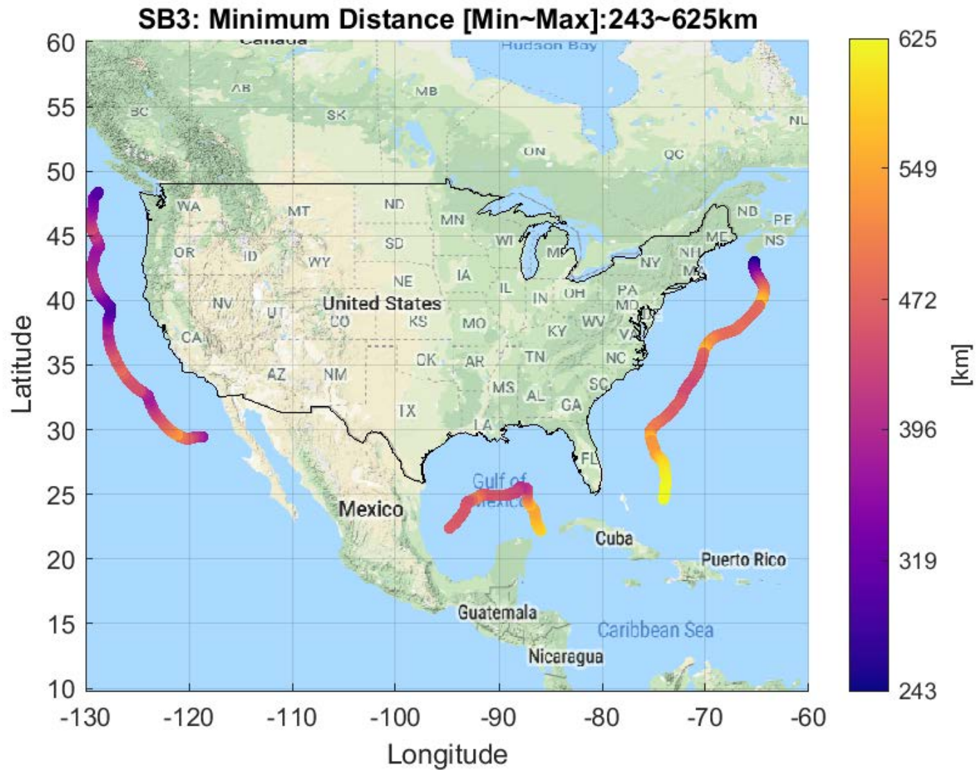
Figure 140. Minimum Distance: BS EIRP: 61 dBm/10 MHz, AP EIRP: 47 dBm/10 MHz IMT-Advanced Deployment
