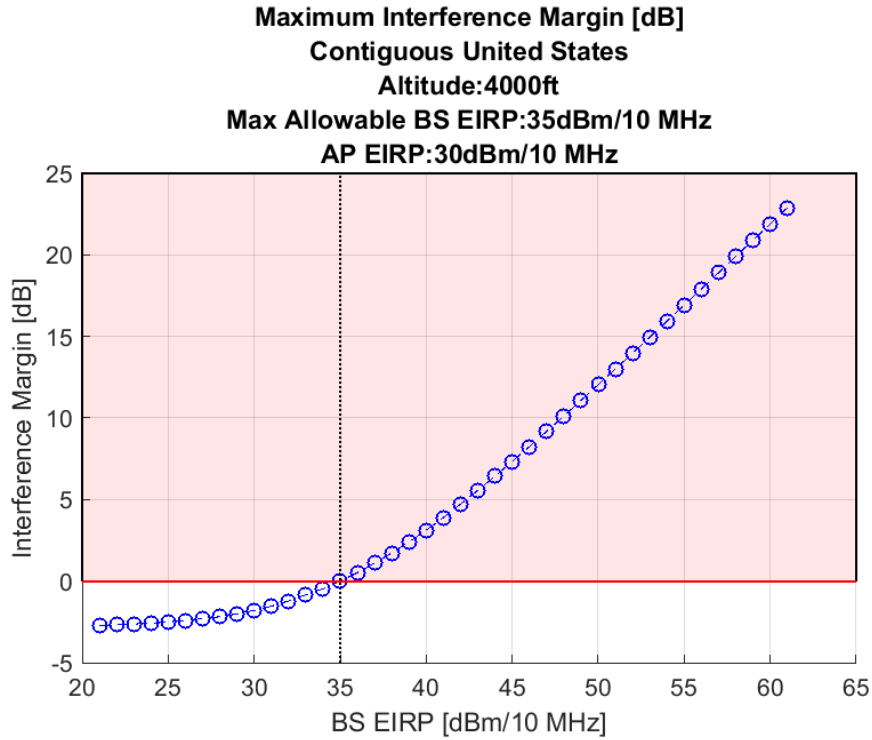
Figure 37. Airborne 1-2: Maximum Allowable EIRP 100 Megahertz Sharing Option, 4,000 ft (AGL) Altitude
