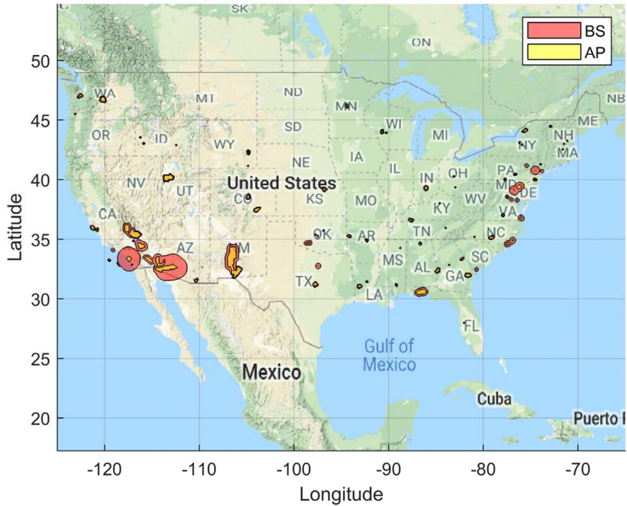
Figure 38. Ground Based Dynamic Coordination Zone Neighborhood: BS EIRP: 47 dBm/10 MHz, AP EIRP: 30 dBm/10 MHz 30 Megahertz Sharing Option and Population Deployment
