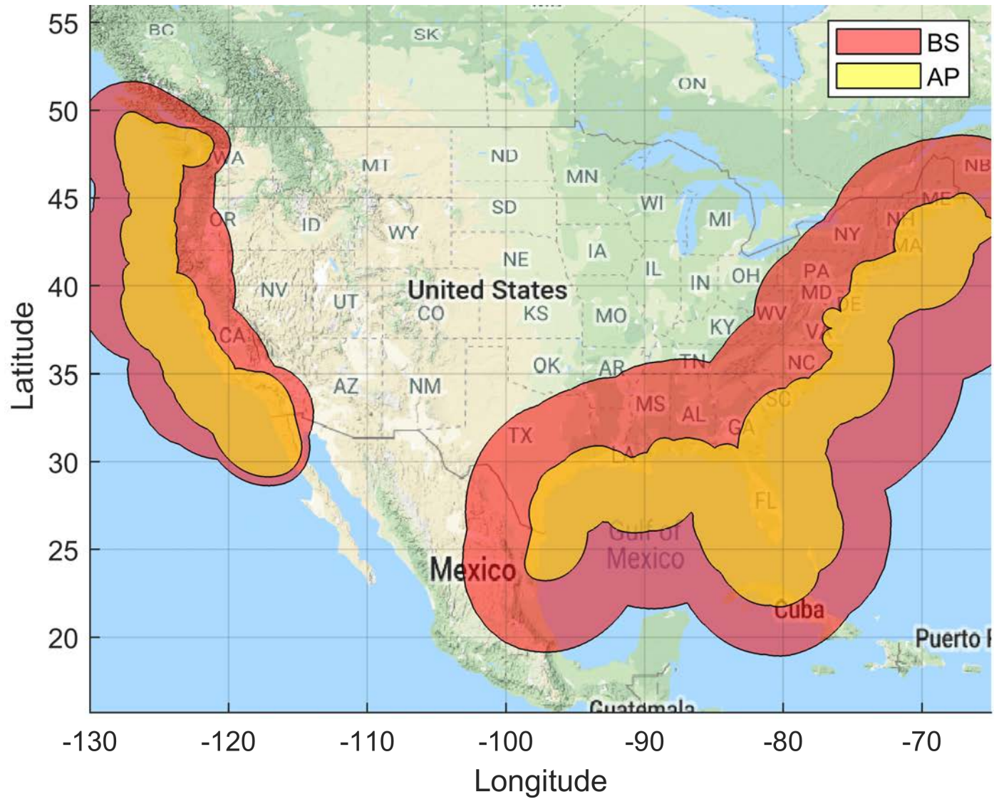
Figure 65. Shipborne Dynamic Coordination Zone Neighborhood: BS EIRP: 61 dBm/10 MHz, AP EIRP: 47 dBm/10 MHz IMT-Advanced Deployment
