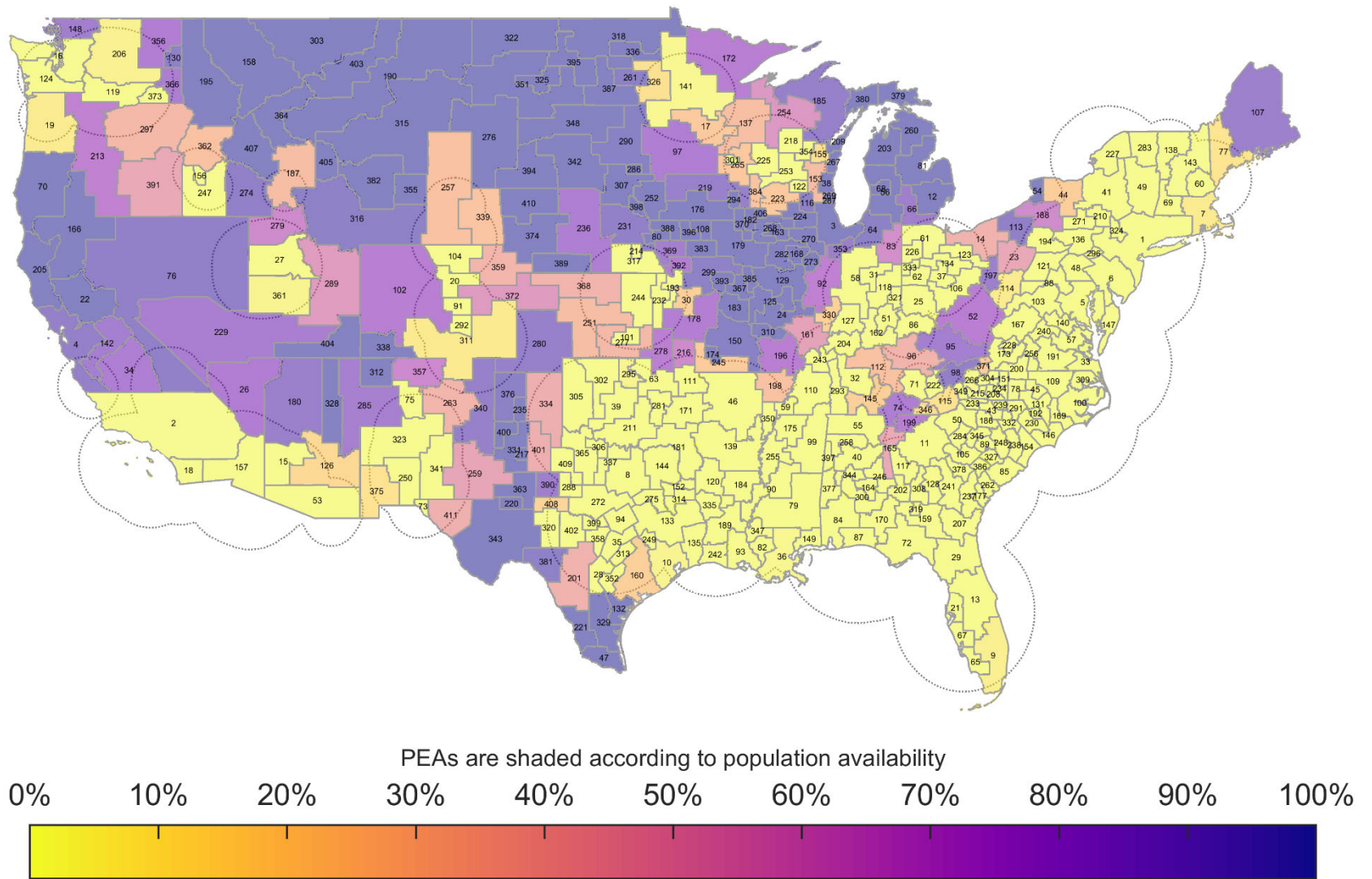
Figure 103. BS Dynamic Coordination Zone Neighborhood Population Availability BS EIRP: 47 dBm/10 MHz, AP EIRP: 36 dBm/10 MHz 100 Megahertz Sharing Option, Population Deployment
