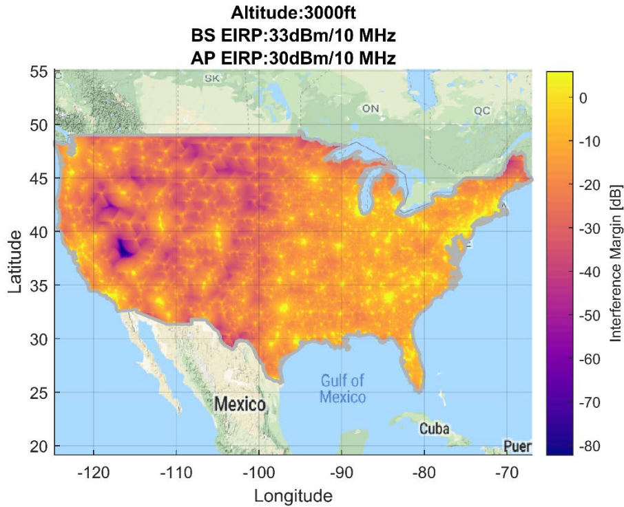
Figure 36. Airborne 1-2: Geographical Interference Margin 100 Megahertz Sharing Option, 3,000ft (AGL) Altitude
