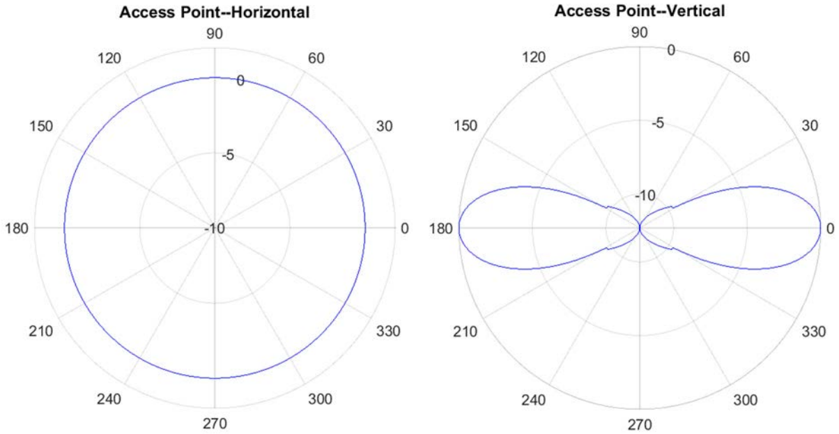
Figure 1. Access Point Antenna Gain Patterns
