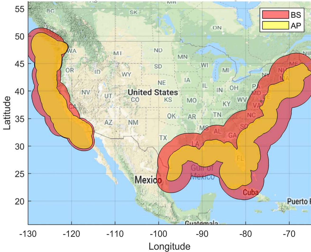
Figure 60. Shipborne Dynamic Coordination Zone Neighborhood: BS EIRP: 47 dBm/10 MHz, AP EIRP: 30 dBm/10 MHz Population Deployment
