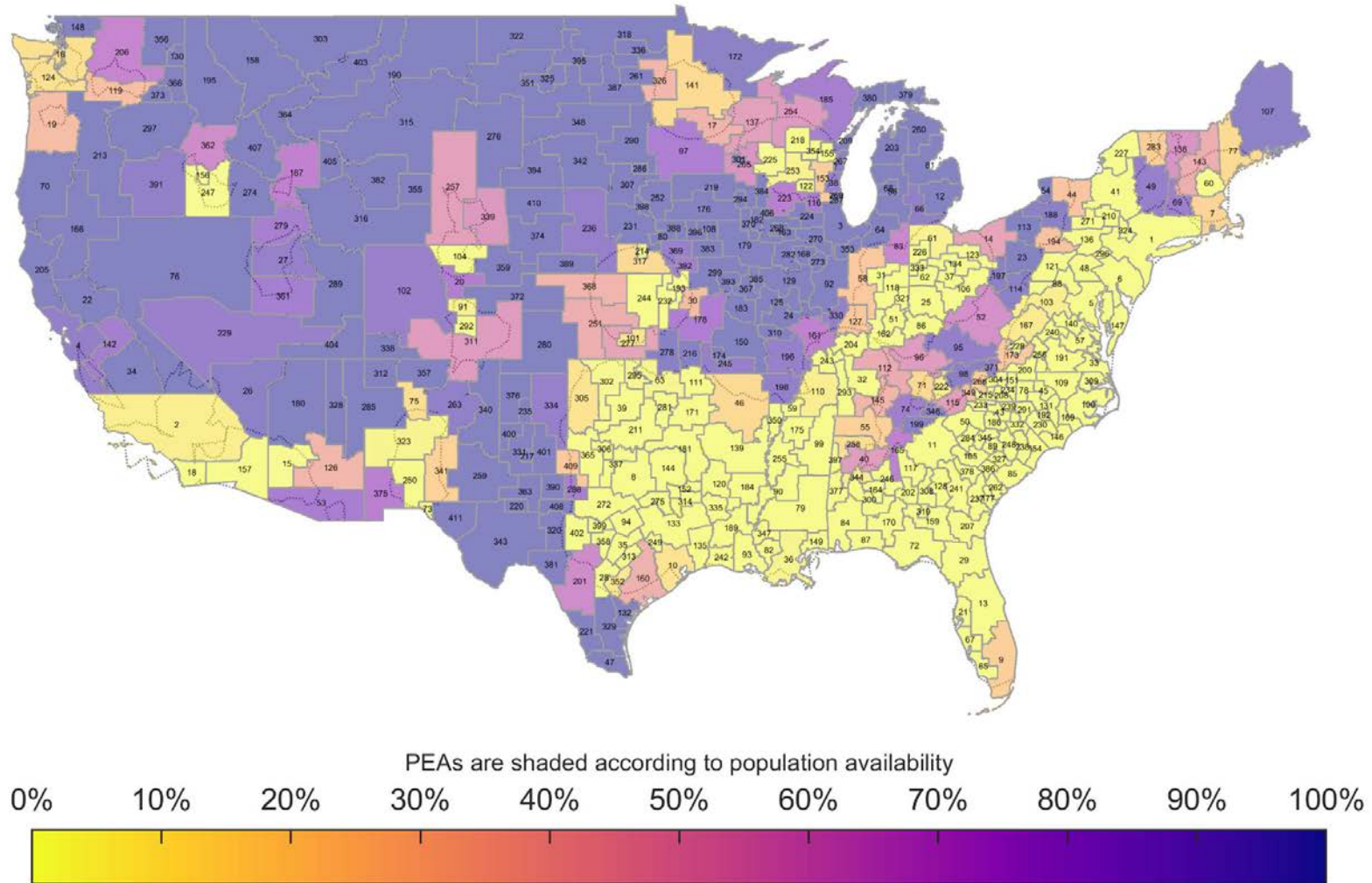
Figure 77. BS Ground Based Exclusion Zone Population Impact BS EIRP: 47 dBm/10 MHz, AP EIRP: 30 dBm/10 MHz 100 Megahertz Sharing Option, Population Deployment
