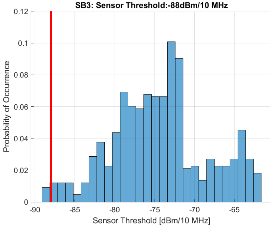
Figure 127. Sensor Detection Threshold BS EIRP: 47 dBm/10 MHz, AP EIRP: 30 dBm/10 MHz Population Deployment
