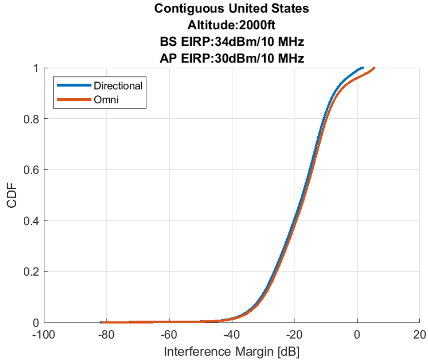
Figure 31. Airborne 1-2: Cumulative Distribution Function of the Interference Margin 100 Megahertz Sharing Option, 2,000ft (AGL) Altitude
