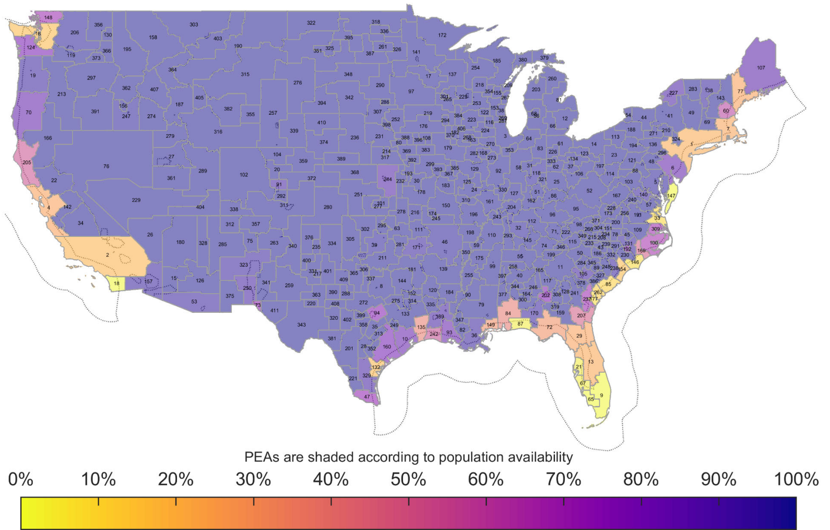
Figure 68. Population Based Deployment Accessibility: AP EIRP: 30 dBm/10 MHz 30 Megahertz Sharing Option
