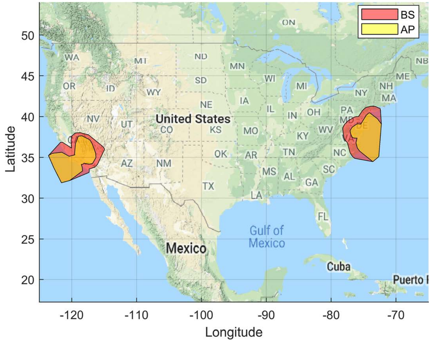
Figure 11. Airborne 3 Exclusion Zone: BS EIRP: 47 dBm/10 MHz, AP EIRP: 36 dBm/10 MHz 100 Megahertz Sharing Option and Population Deployment
