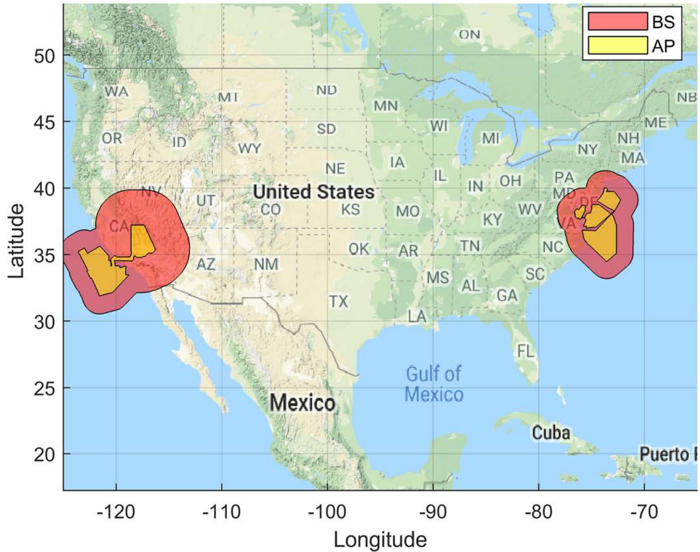
Figure 17. Airborne 3 Dynamic Coordination Zone Neighborhood: BS EIRP: 47 dBm/10 MHz, AP EIRP: 36 dBm/10 MHz, 100 Megahertz Sharing Option and Population Deployment
