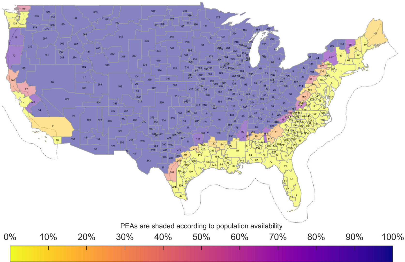
Figure 121. BS Shipborne Exclusion Zone Population Availability: BS EIRP: 47 dBm/10 MHz, AP EIRP: 36 dBm/10 MHz IMT-Advanced Deployment
