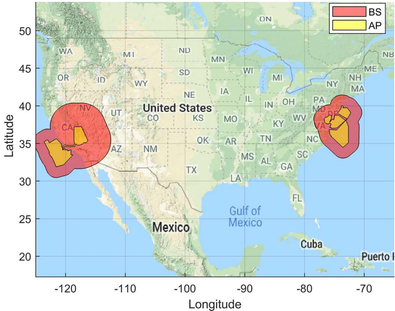
Figure 19. Airborne 3 Dynamic Coordination Zone Neighborhood: BS EIRP: 47 dBm/10 MHz, AP EIRP: 30 dBm/10 MHz, 100 Megahertz Sharing Option and IMT-Advanced Deployment
