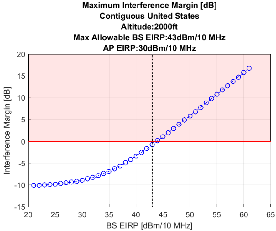
Figure 9. Airborne 1-2: Maximum Allowable EIRP 30 Megahertz Sharing Option, 2,000 ft (AGL) Altitude
