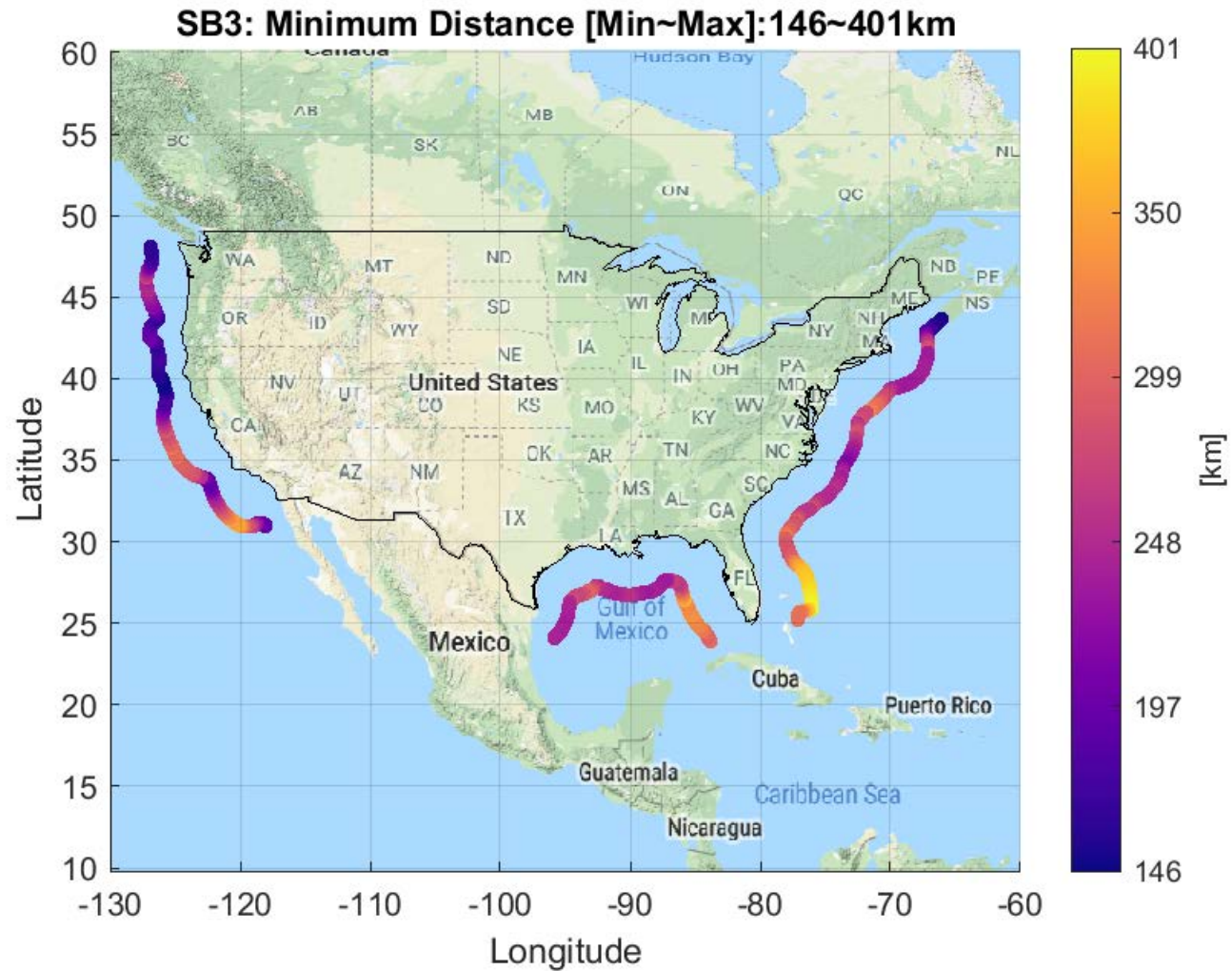
Figure 125. Minimum Distance: BS EIRP: 47 dBm/10 MHz, AP EIRP: 30 dBm/10 MHz Population Deployment
