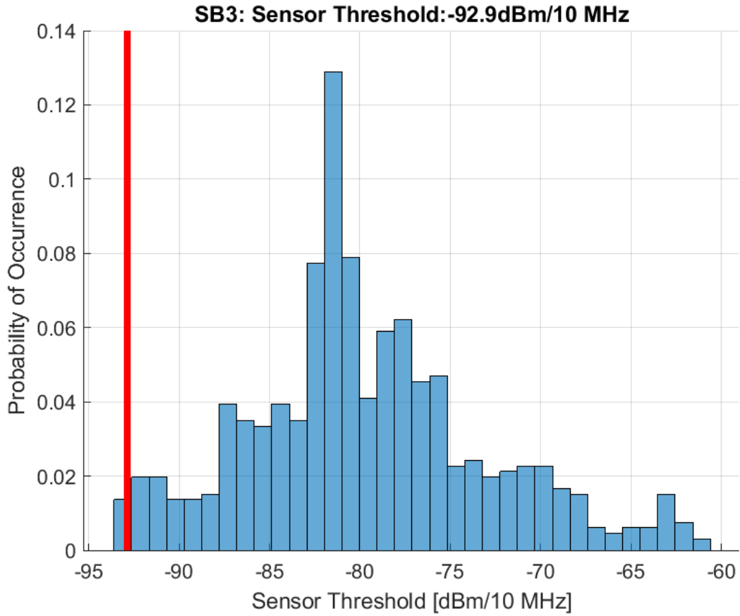
Figure 139. Sensor Detection Threshold BS EIRP: 47 dBm/10 MHz, AP EIRP: 36 dBm/10 MHz IMT-Advanced Deployment
