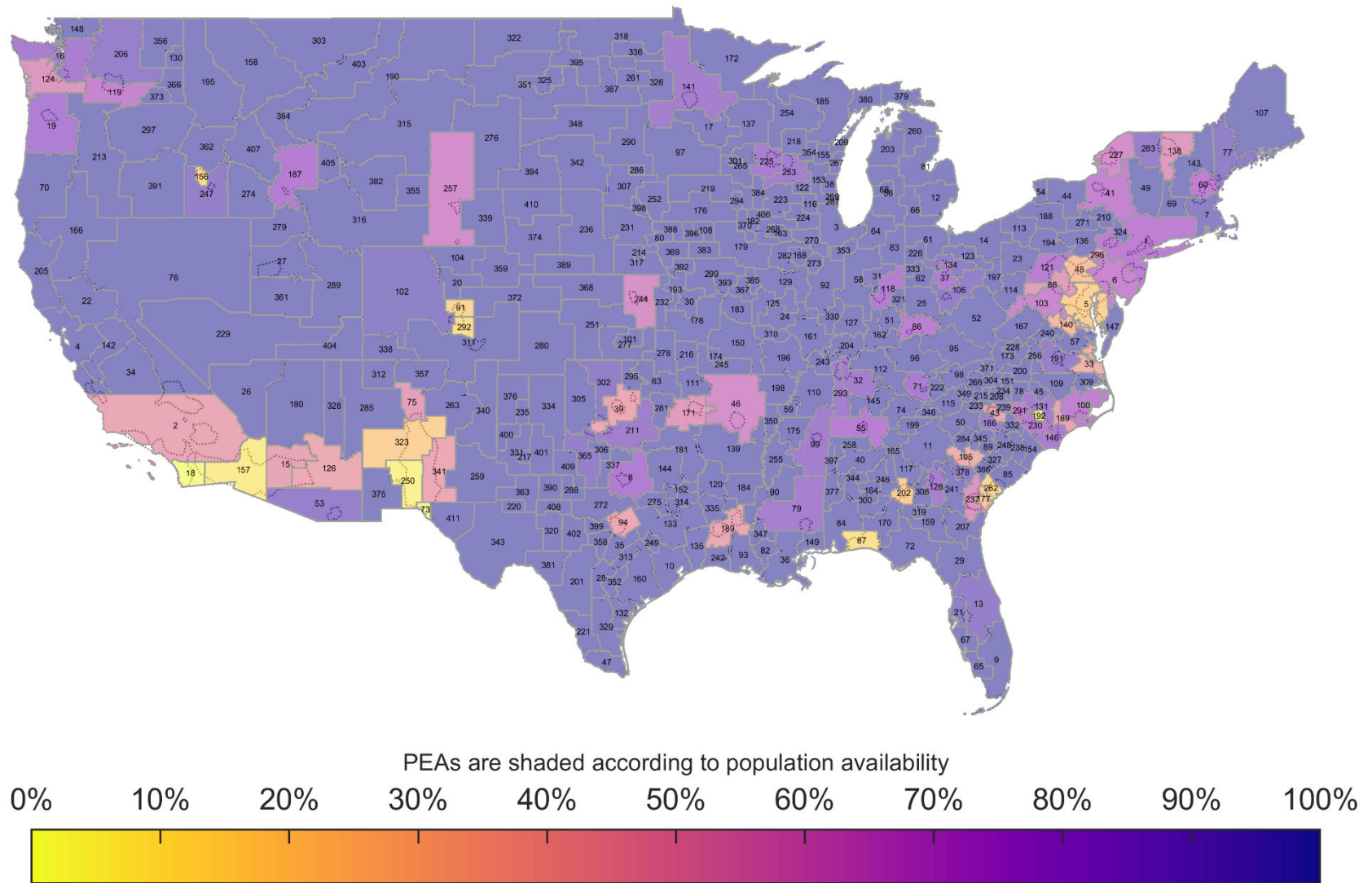
Figure 69. BS Ground Based Exclusion Zone Population Availability BS EIRP: 61 dBm/10 MHz, AP EIRP: 47 dBm/10 MHz 30 Megahertz Sharing Option, Population Deployment
