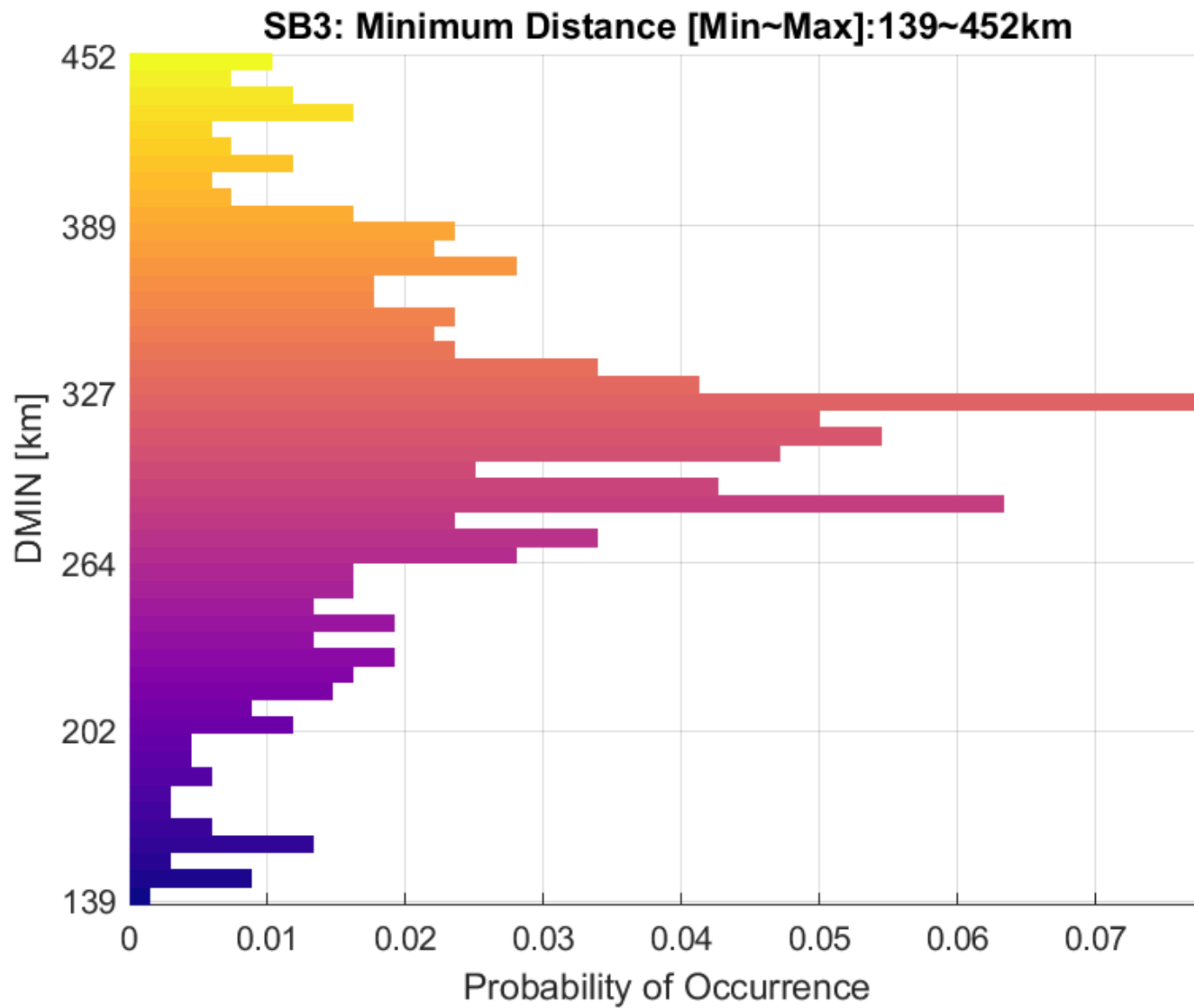
Figure 138. Minimum Distance Distribution: BS EIRP: 47 dBm/10 MHz, AP EIRP: 36 dBm/10 MHz IMT-Advanced Deployment
