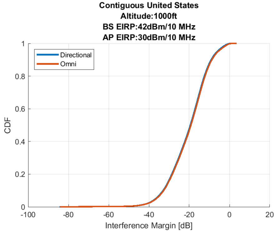
Figure 7. Airborne 1-2: Cumulative Distribution Function of the Interference Margin 30 Megahertz Sharing Option, 1,000ft (AGL) Altitude
