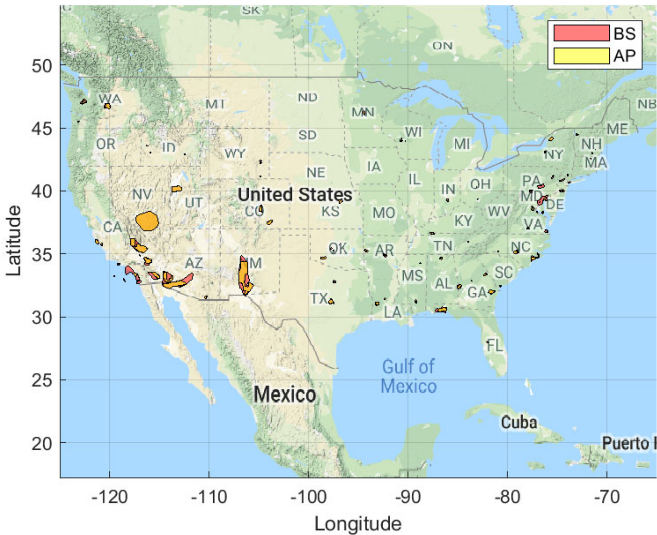
Figure 28. Ground Based Exclusion Zone: BS EIRP: 47 dBm/10 MHz, AP EIRP: 36 dBm/10 MHz 30 Megahertz Sharing Option and IMT-Advanced Deployment
