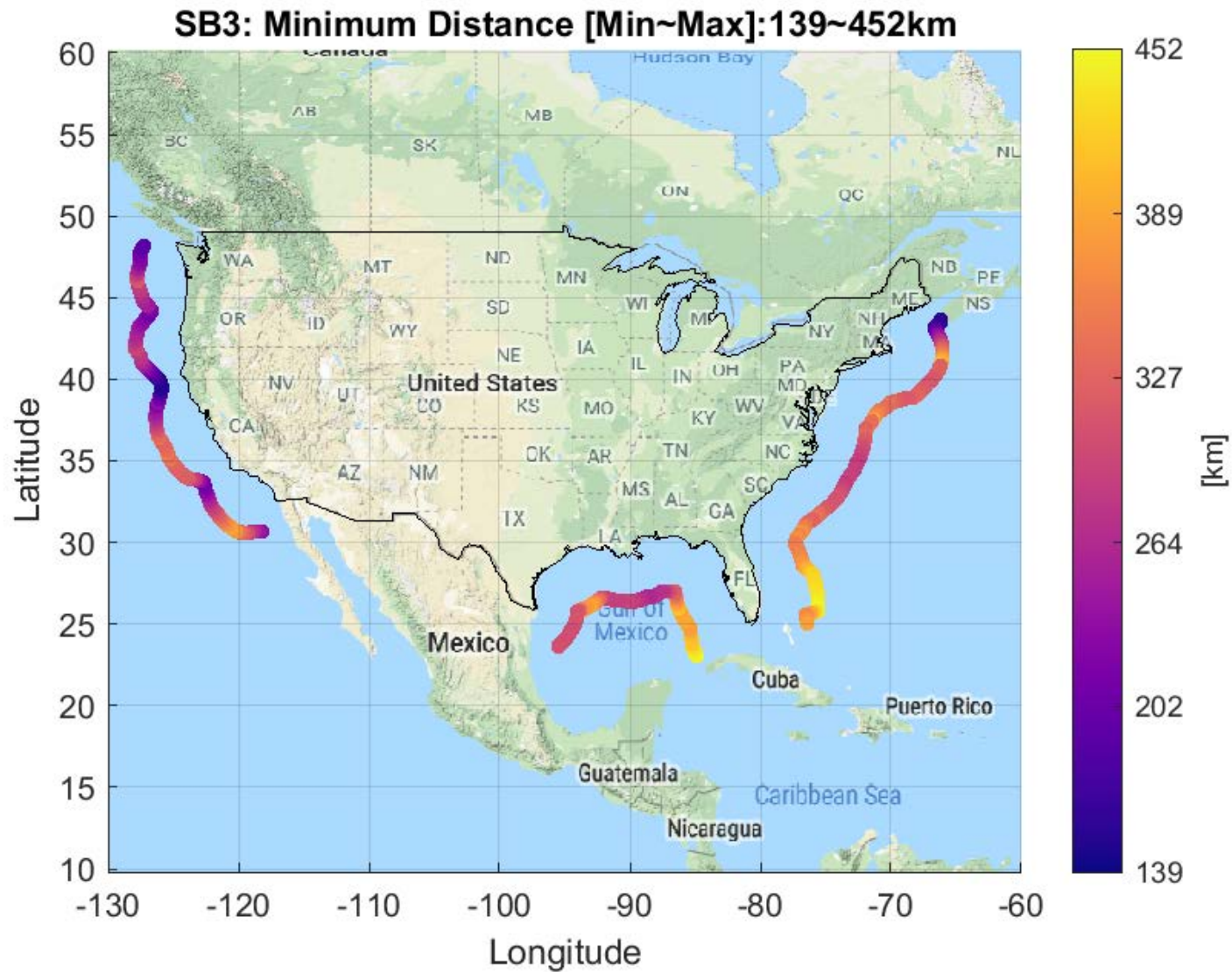
Figure 137. Minimum Distance: BS EIRP: 47 dBm/10 MHz, AP EIRP: 36 dBm/10 MHz IMT-Advanced Deployment
