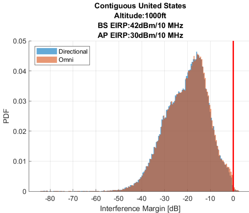
Figure 6. Airborne 1-2: Probability Distribution Function of the Interference Margin 30 Megahertz Sharing Option, 1,000ft (AGL) Altitude
