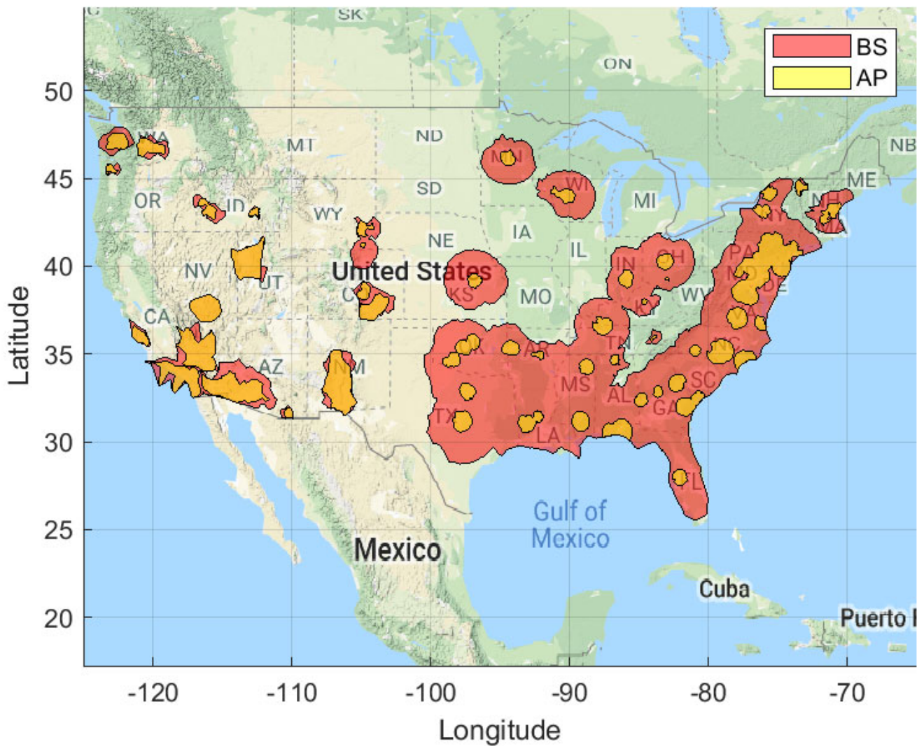
Figure 31. Ground Based Exclusion Zone: BS EIRP: 47 dBm/10 MHz, AP EIRP: 36 dBm/10 MHz 100 Megahertz Sharing Option and Population Deployment
