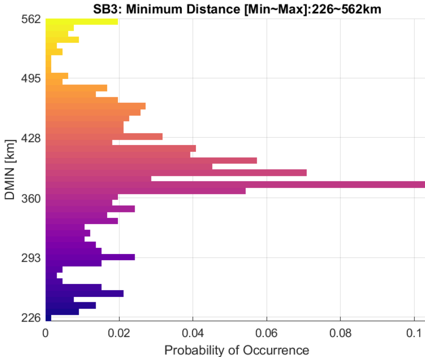
Figure 132. Minimum Distance Distribution: BS EIRP: 61 dBm/10 MHz, AP EIRP: 47 dBm/10 MHz Population Deployment
