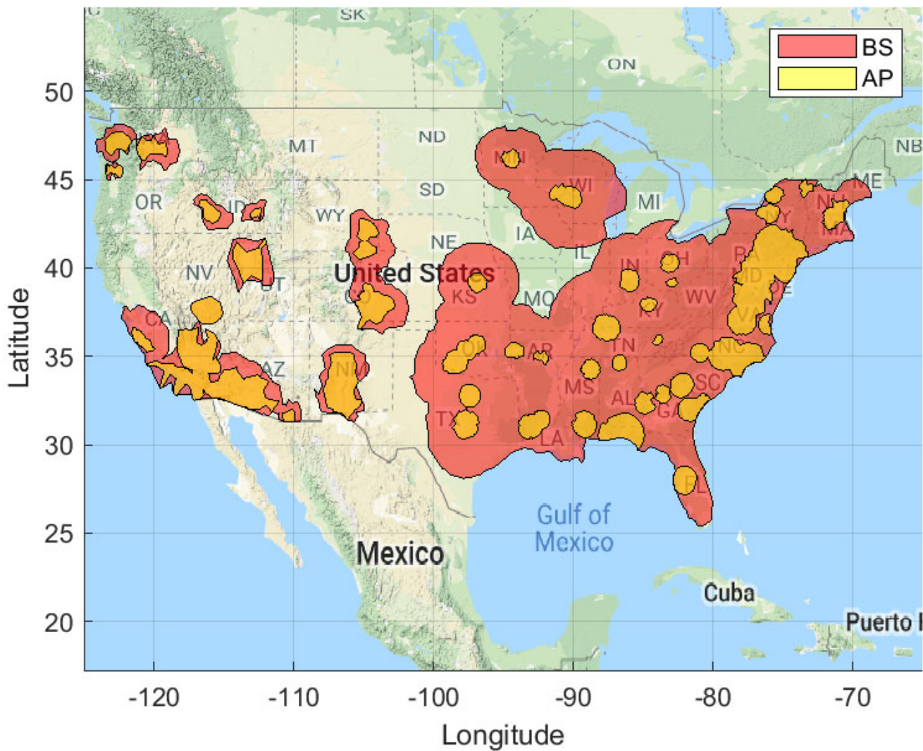
Figure 32. Ground Based Exclusion Zone: BS EIRP: 61 dBm/10 MHz, AP EIRP: 47 dBm/10 MHz 100 Megahertz Sharing Option and Population Deployment
