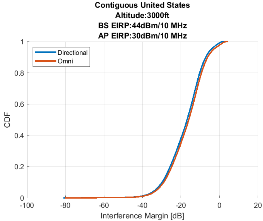
Figure 15. Airborne 1-2: Cumulative Distribution Function of the Interference Margin 30 Megahertz Sharing Option, 3,000ft (AGL) Altitude
