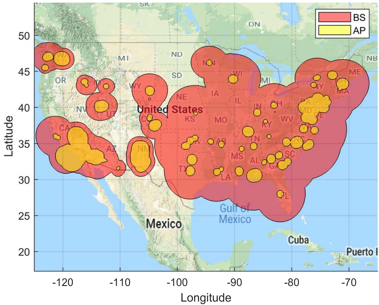
Figure 49. Ground Based Dynamic Coordination Zone Neighborhood: BS EIRP: 61 dBm/10 MHz, AP EIRP: 47 dBm/10 MHz 100 Megahertz Sharing Option and IMT-Advanced Deployment
