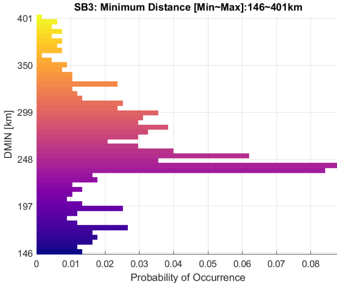
Figure 126. Minimum Distance Distribution: BS EIRP: 47 dBm/10 MHz, AP EIRP: 30 dBm/10 MHz Population Deployment
