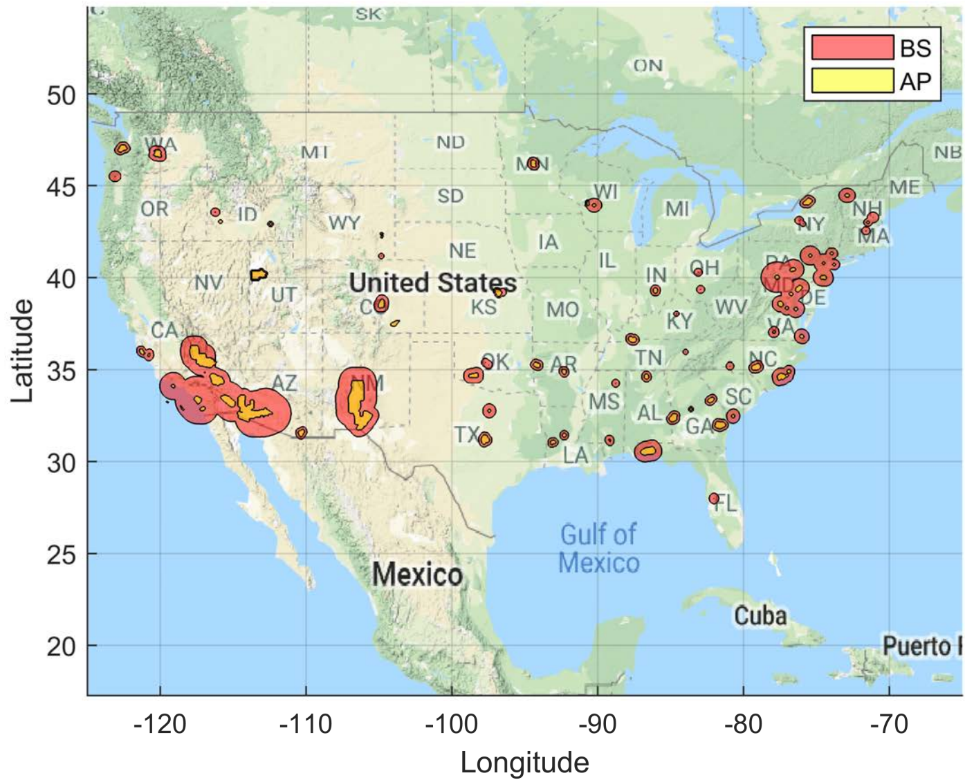
Figure 40. Ground Based Dynamic Coordination Zone Neighborhood: BS EIRP: 61 dBm/10 MHz, AP EIRP: 47 dBm/10 MHz 30 Megahertz Sharing Option and Population Deployment
