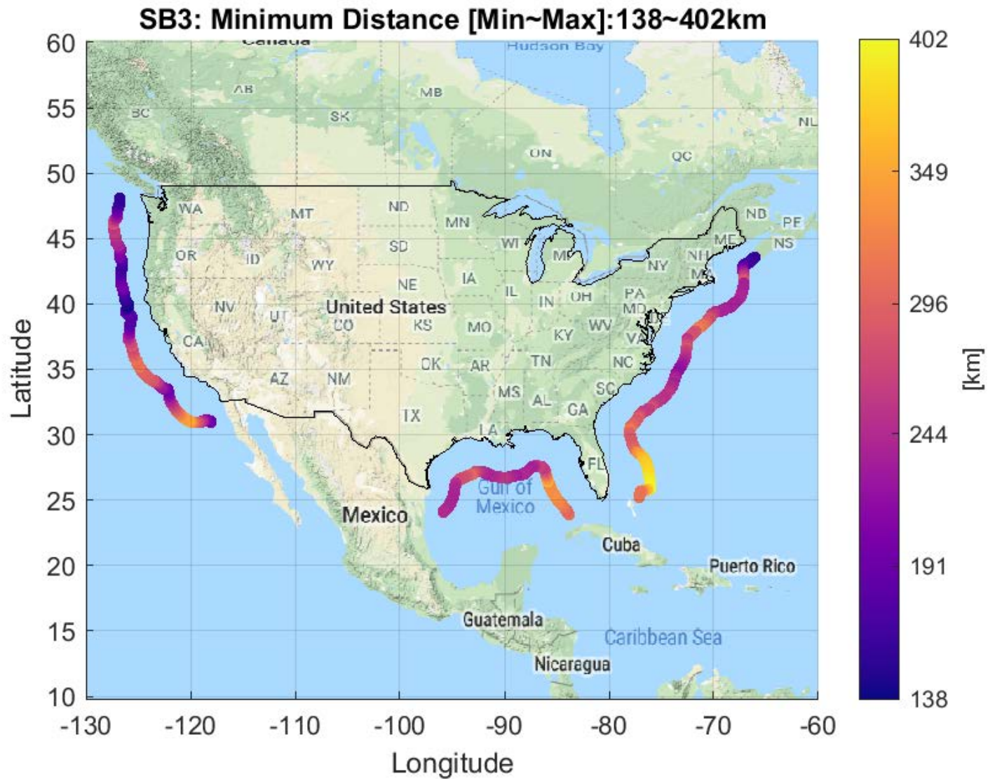
Figure 128. Minimum Distance: BS EIRP: 47 dBm/10 MHz, AP EIRP: 36 dBm/10 MHz Population Deployment
