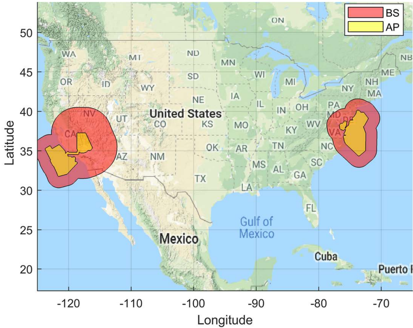
Figure 21. Airborne 3 Dynamic Coordination Zone Neighborhood: BS EIRP: 61 dBm/10 MHz, AP EIRP: 47 dBm/10 MHz, 100 Megahertz Sharing Option and IMT-Advanced Deployment
