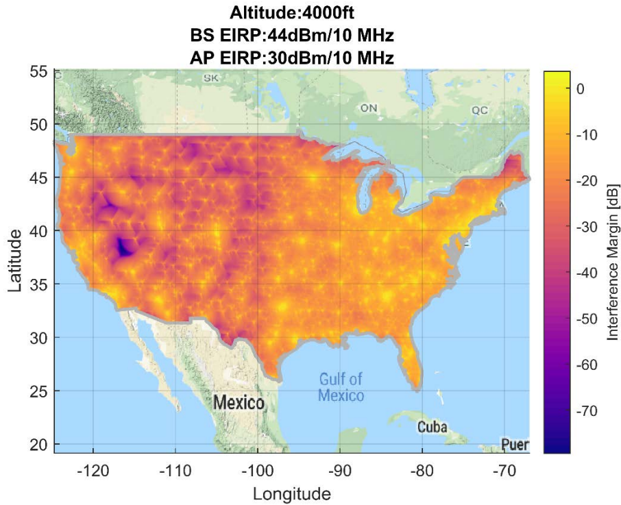
Figure 20. Airborne 1-2: Geographical Interference Margin 30 Megahertz Sharing Option, 4,000ft (AGL) Altitude
