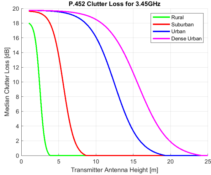
Figure 8. Example calculated clutter loss as a function of transmitter antenna height.
