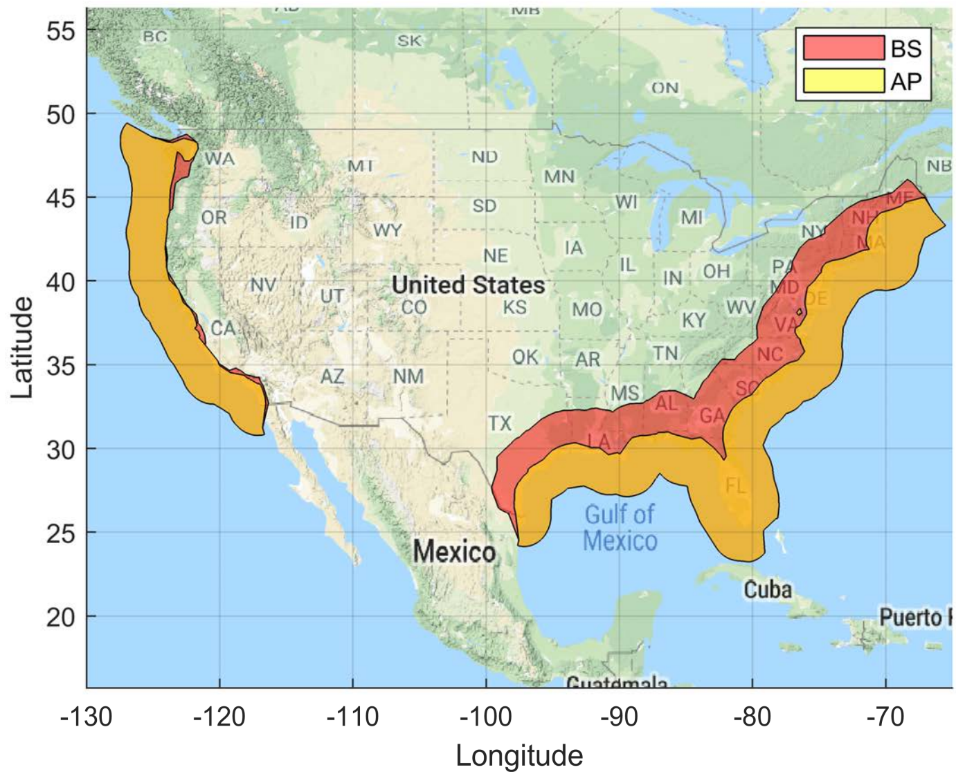
Figure 51. Shipborne Exclusion Zone: BS EIRP: 47 dBm/10 MHz, AP EIRP: 36 dBm/10 MHz Population Deployment
