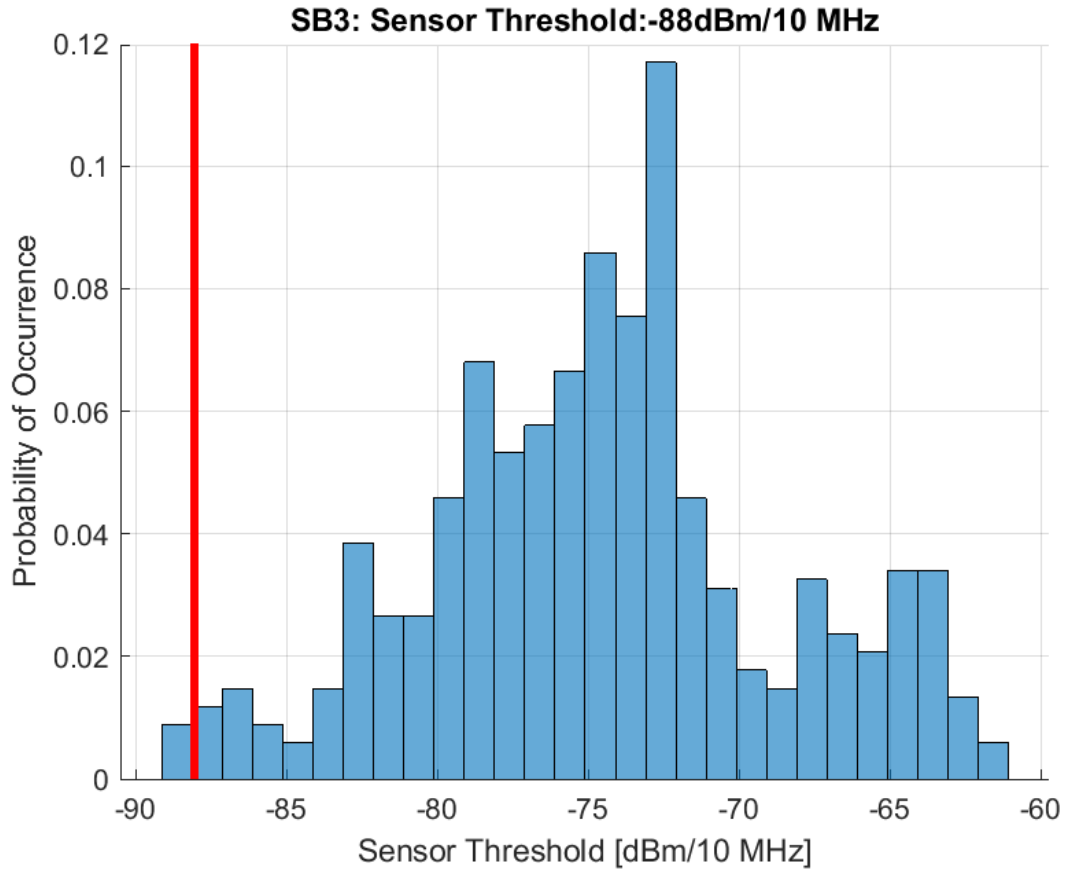
Figure 130. Sensor Detection Threshold BS EIRP: 47 dBm/10 MHz, AP EIRP: 36 dBm/10 MHz Population Deployment
