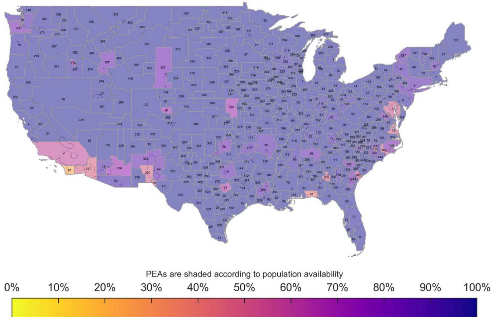
Figure 65. BS Ground Based Exclusion Zone Population Availability BS EIRP: 47 dBm/10 MHz, AP EIRP: 30 dBm/10 MHz 30 Megahertz Sharing Option, Population Deployment
