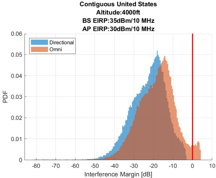
Figure 38. Airborne 1-2: Probability Distribution Function of the Interference Margin 100 Megahertz Sharing Option, 4,000ft (AGL) Altitude
