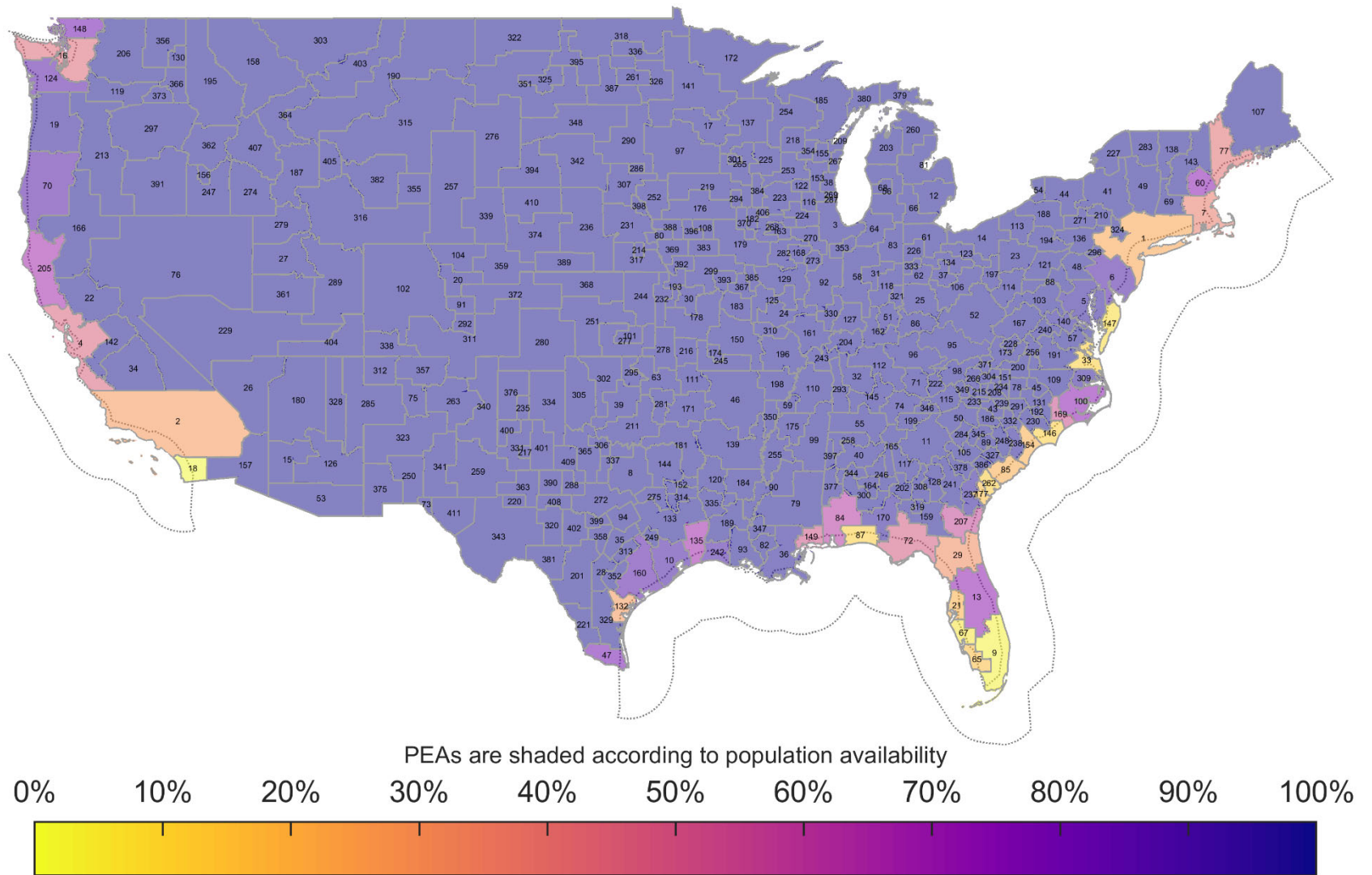
Figure 120. AP Shipborne Exclusion Zone Population Availability: BS EIRP: 47 dBm/10 MHz, AP EIRP: 30 dBm/10 MHz IMT-Advanced Deployment
