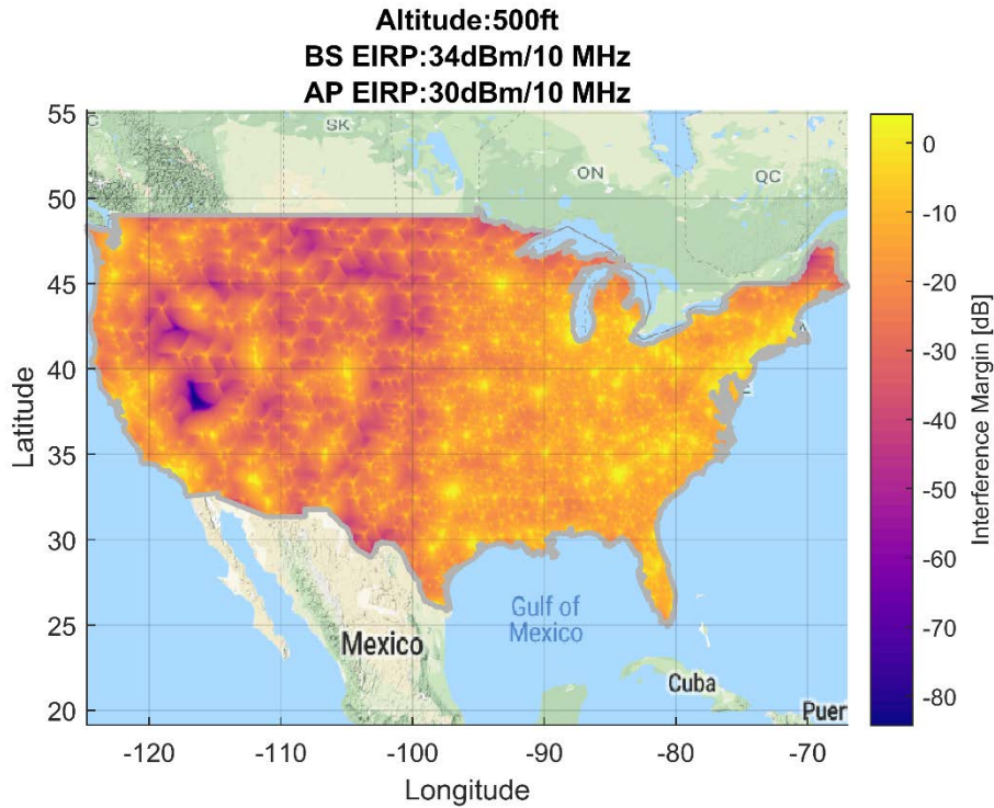
Figure 24. Airborne 1-2: Geographical Interference Margin 100 Megahertz Sharing Option, 500 ft (AGL) Altitude
