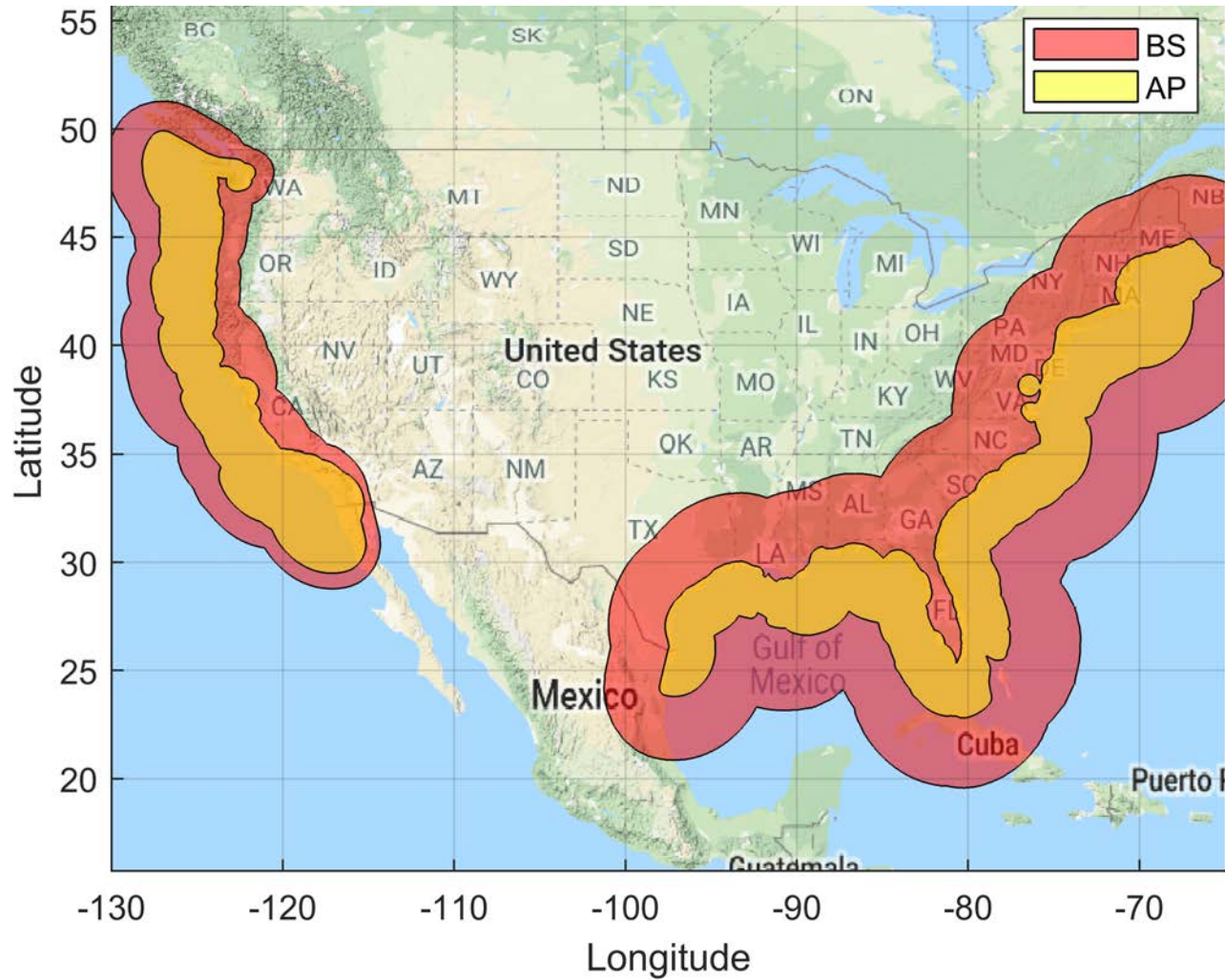
Figure 63. Shipborne Dynamic Coordination Zone Neighborhood: BS EIRP: 47 dBm/10 MHz, AP EIRP: 30 dBm/10 MHz IMT-Advanced Deployment
