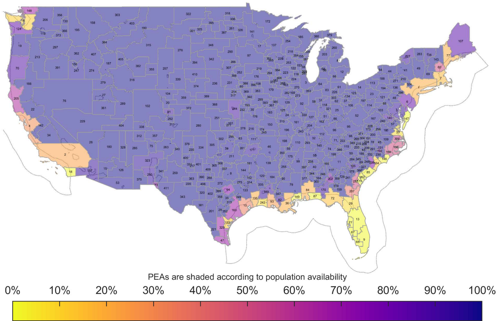
Figure 75. IMT-Advanced Deployment Accessibility: AP EIRP: 47 dBm/10 MHz 30 Megahertz Sharing Option
