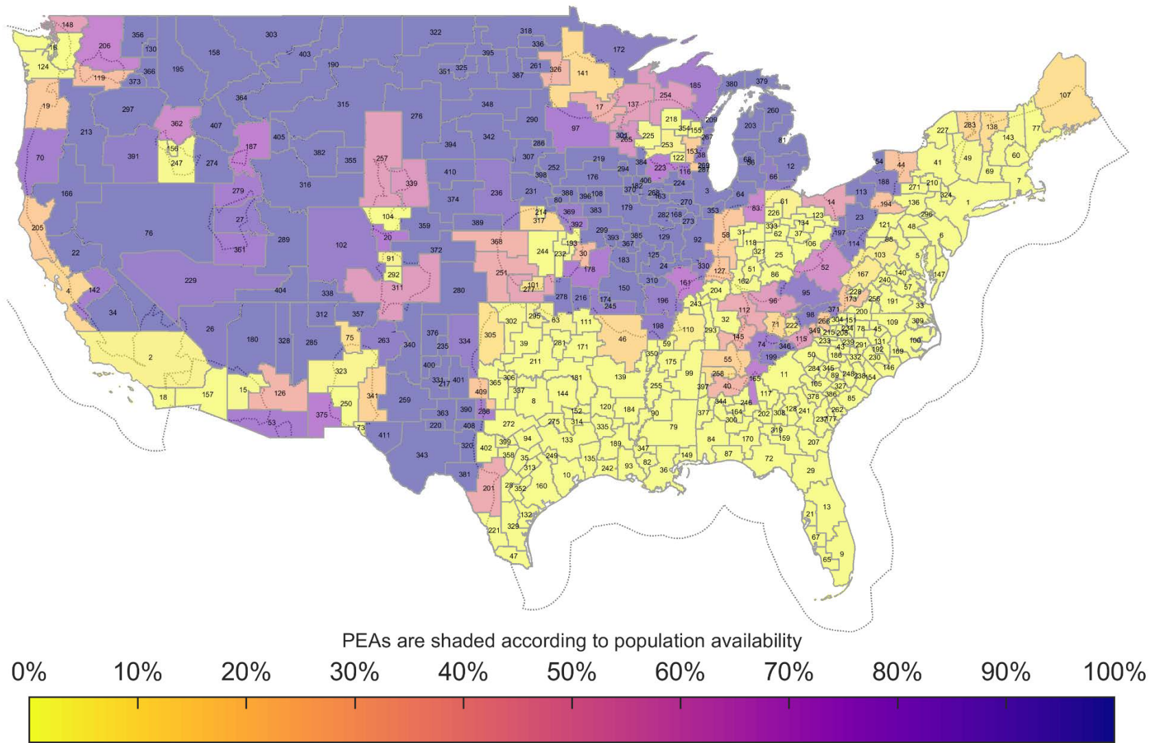
Figure 76. Population Based Deployment Accessibility: BS EIRP: 47 dBm/10 MHz 100 Megahertz Sharing Option
