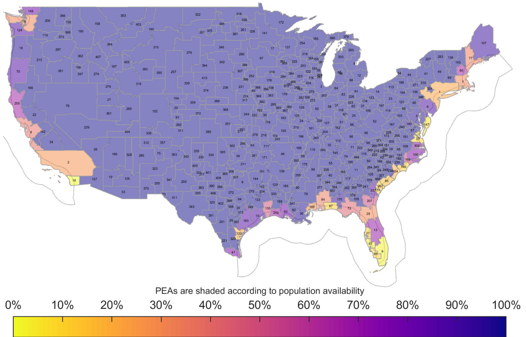
Figure 122. AP Shipborne Exclusion Zone Population Availability: BS EIRP: 47 dBm/10 MHz, AP EIRP: 36 dBm/10 MHz IMT-Advanced Deployment
