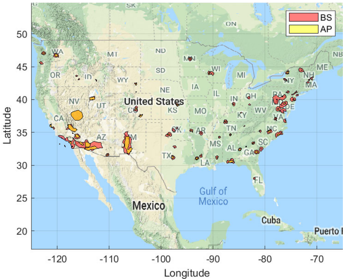
Figure 26. Ground Based Exclusion Zone: BS EIRP: 61 dBm/10 MHz, AP EIRP: 47 dBm/10 MHz 30 Megahertz Sharing Option and Population Deployment
