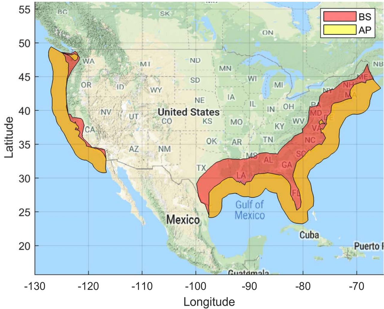
Figure 53. Shipborne Exclusion Zone: BS EIRP: 47 dBm/10 MHz, AP EIRP: 30 dBm/10 MHz IMT-Advanced Deployment
