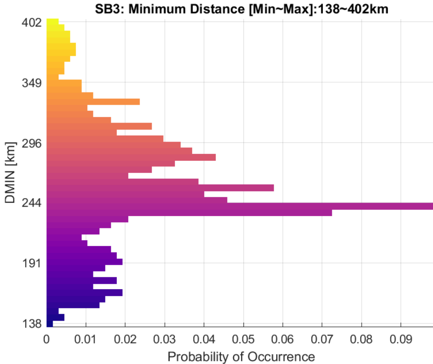
Figure 129. Minimum Distance Distribution: BS EIRP: 47 dBm/10 MHz, AP EIRP: 36 dBm/10 MHz Population Deployment
