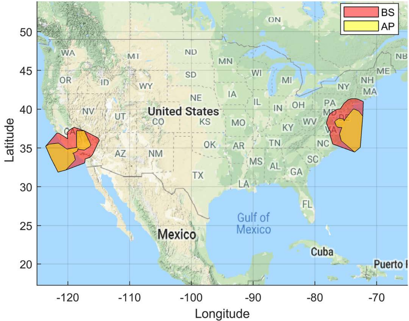
Figure 13. Airborne 3 Exclusion Zone: BS EIRP: 47 dBm/10 MHz, AP EIRP: 30 dBm/10 MHz 100 Megahertz Sharing Option and IMT-Advanced Deployment
