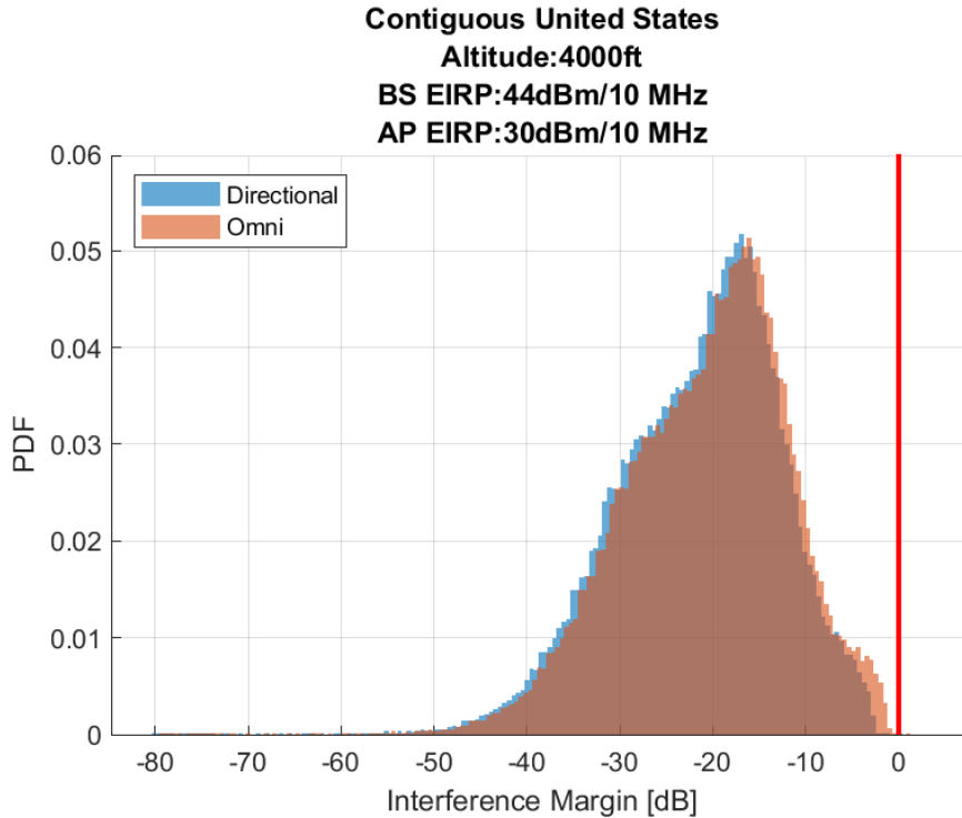
Figure 18. Airborne 1-2: Probability Distribution Function of the Interference Margin 30 Megahertz Sharing Option, 4,000ft (AGL) Altitude
