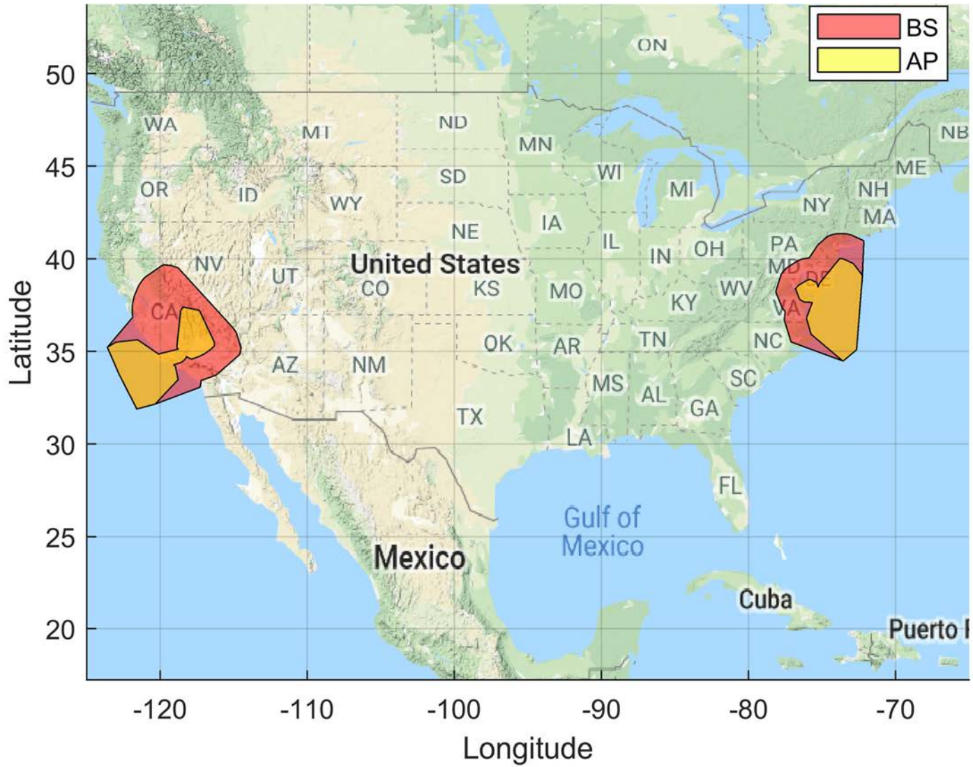
Figure 14. Airborne 3 Exclusion Zone: BS EIRP: 47 dBm/10 MHz, AP EIRP: 36 dBm/10 MHz 100 Megahertz Sharing Option and IMT-Advanced Deployment
