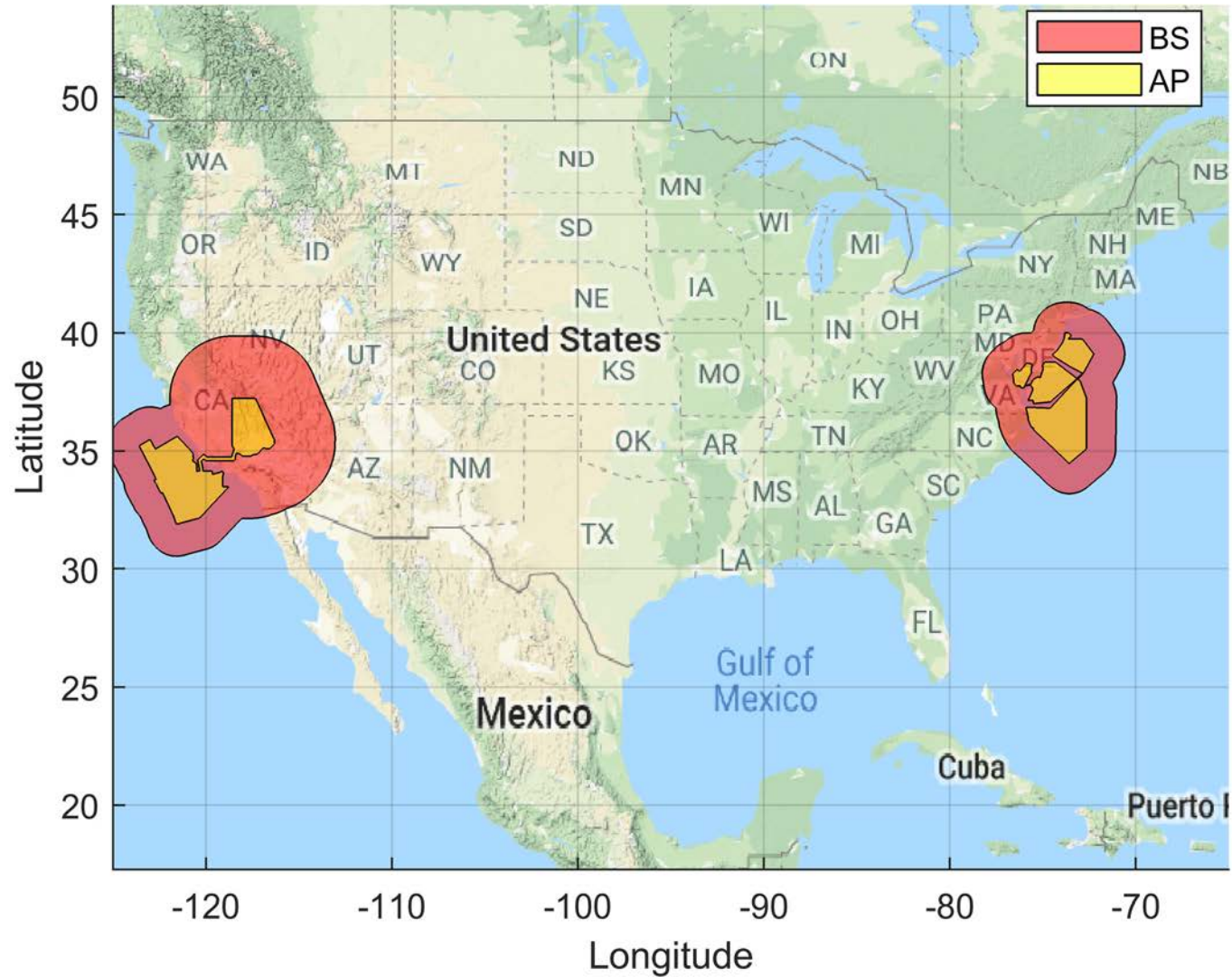
Figure 16. Airborne 3 Dynamic Coordination Zone Neighborhood: BS EIRP: 47 dBm/10 MHz, AP EIRP: 30 dBm/10 MHz, 100 Megahertz Sharing Option and Population Deployment
