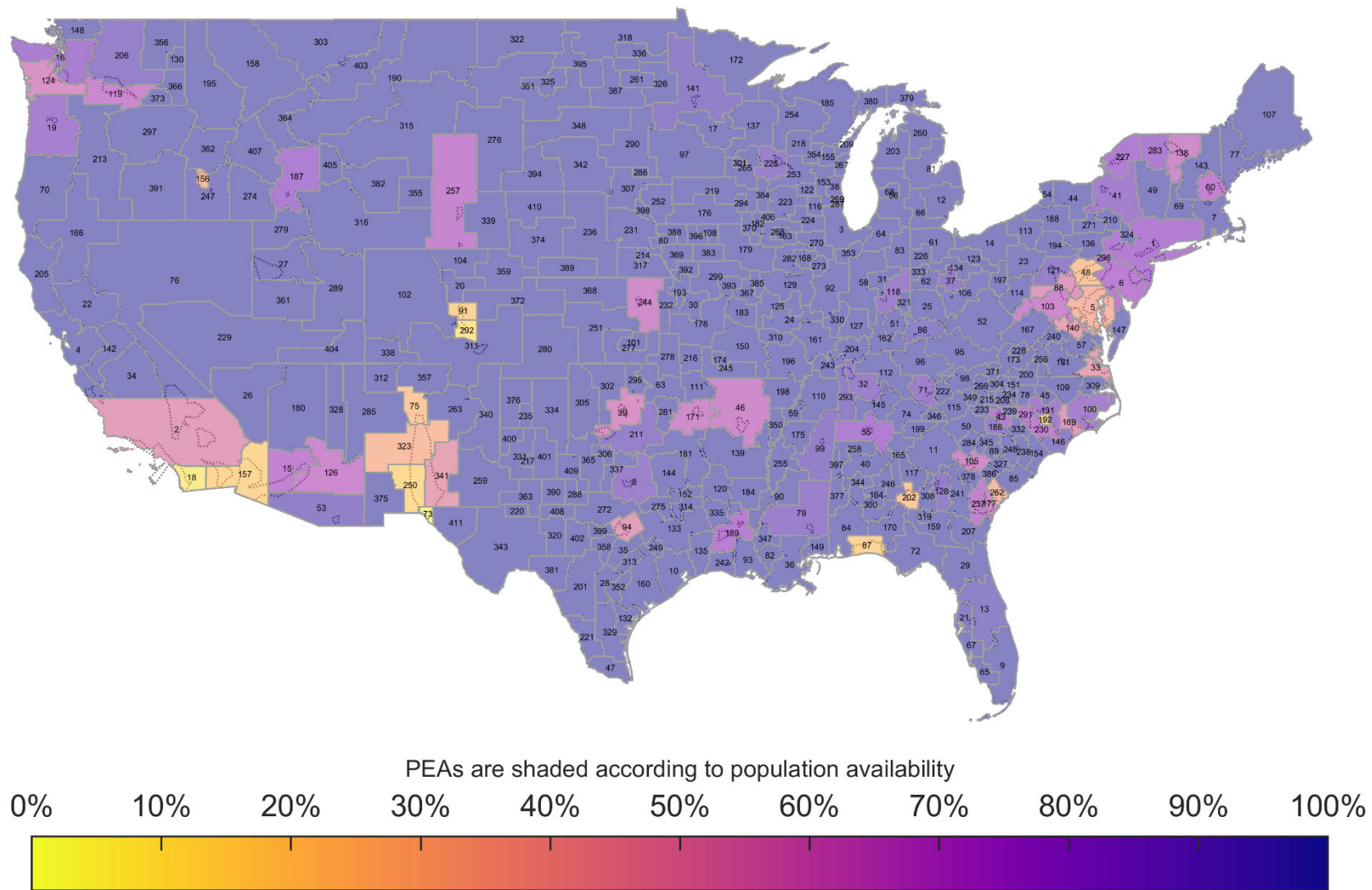
Figure 75. BS Ground Based Exclusion Zone Population Availability BS EIRP: 61 dBm/10 MHz, AP EIRP: 47 dBm/10 MHz 30 Megahertz Sharing Option, IMT-Advanced Deployment
