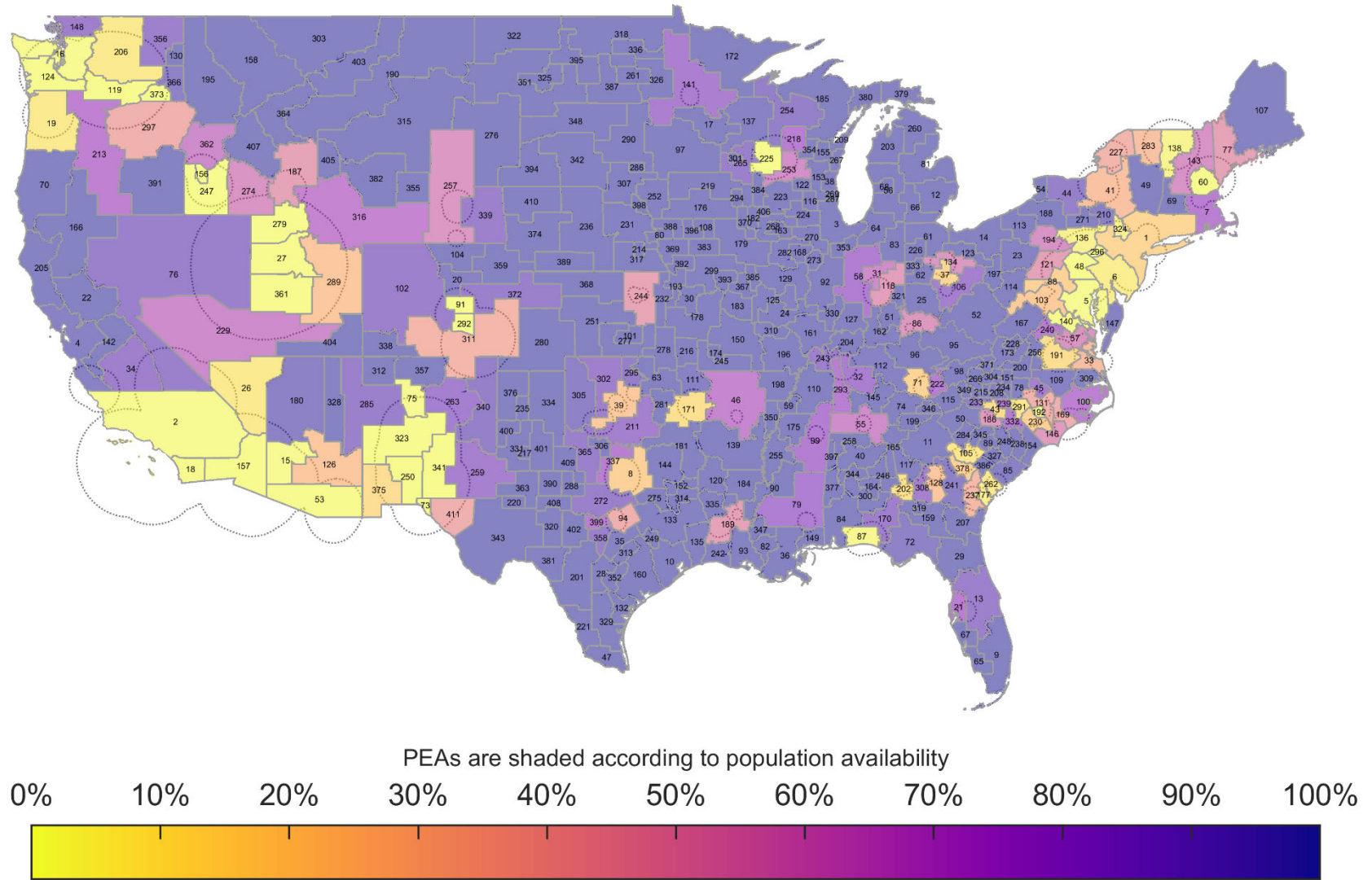
Figure 102. AP Dynamic Coordination Zone Neighborhood Population Availability BS EIRP: 47 dBm/10 MHz, AP EIRP: 30 dBm/10 MHz 100 Megahertz Sharing Option, Population Deployment
