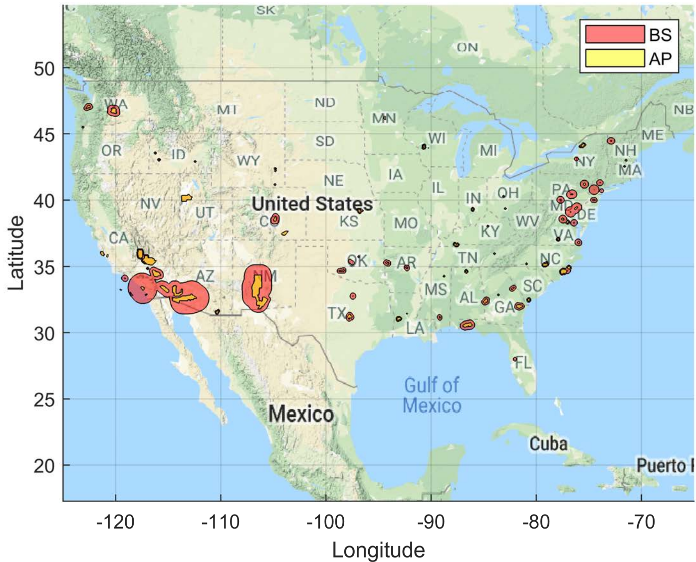
Figure 42. Ground Based Dynamic Coordination Zone Neighborhood: BS EIRP: 47 dBm/10 MHz, AP EIRP: 36 dBm/10 MHz 30 Megahertz Sharing Option and IMT-Advanced Deployment
