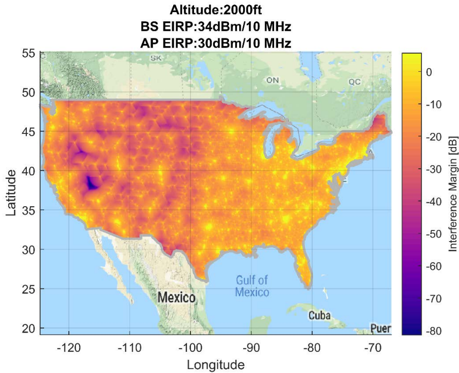
Figure 32. Airborne 1-2: Geographical Interference Margin 100 Megahertz Sharing Option, 2,000ft (AGL) Altitude
