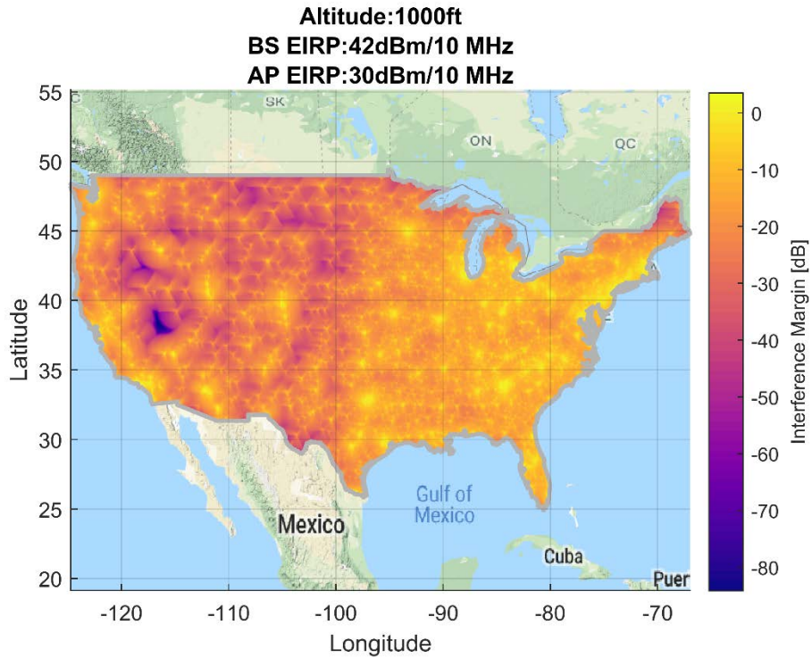
Figure 8. Airborne 1-2: Geographical Interference Margin 30 Megahertz Sharing Option, 1,000ft (AGL) Altitude
