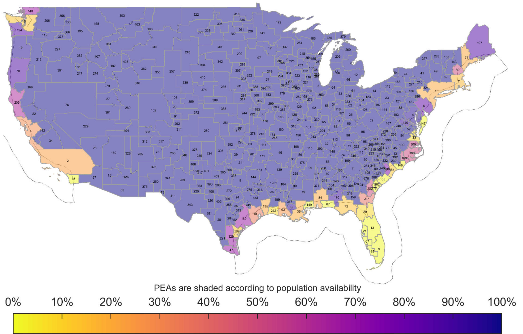
Figure 124. AP Shipborne Exclusion Zone Population Availability: BS EIRP: 61 dBm/10 MHz, AP EIRP: 47 dBm/10 MHz IMT-Advanced Deployment
