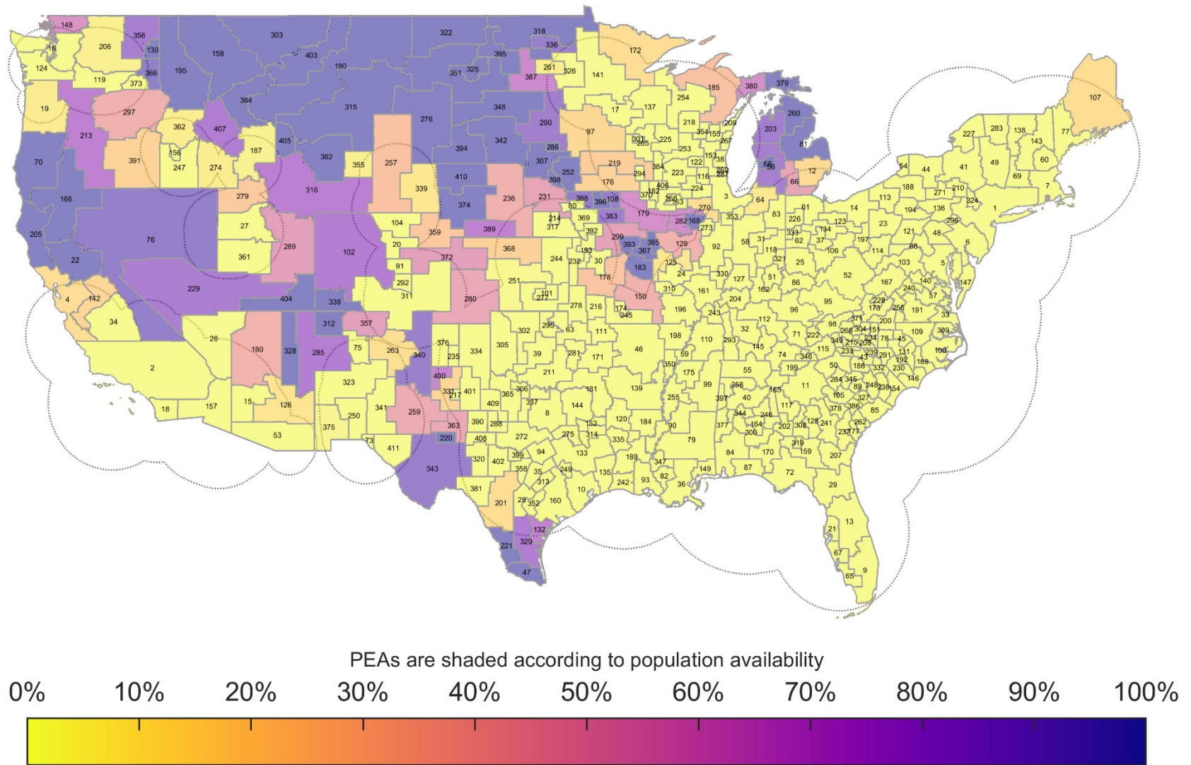
Figure 105. BS Dynamic Coordination Zone Neighborhood Population Availability BS EIRP: 61 dBm/10 MHz, AP EIRP: 47 dBm/10 MHz 100 Megahertz Sharing Option, Population Deployment
