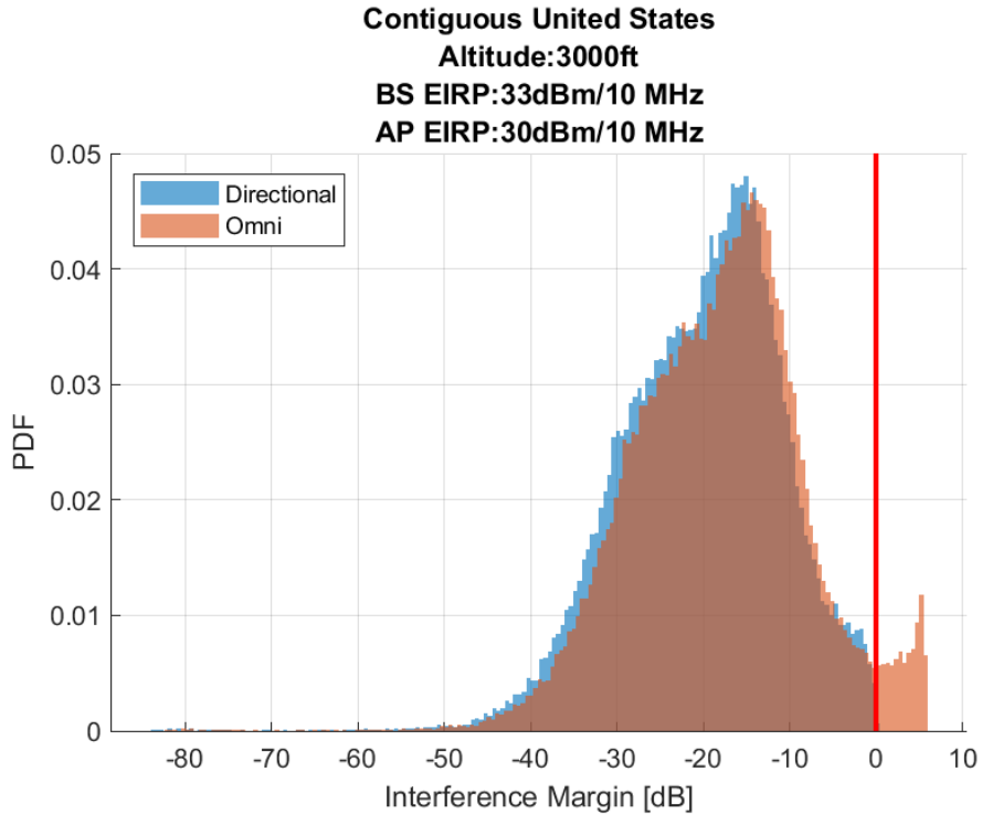
Figure 34. Airborne 1-2: Probability Distribution Function of the Interference Margin 100 Megahertz Sharing Option, 3,000ft (AGL) Altitude
