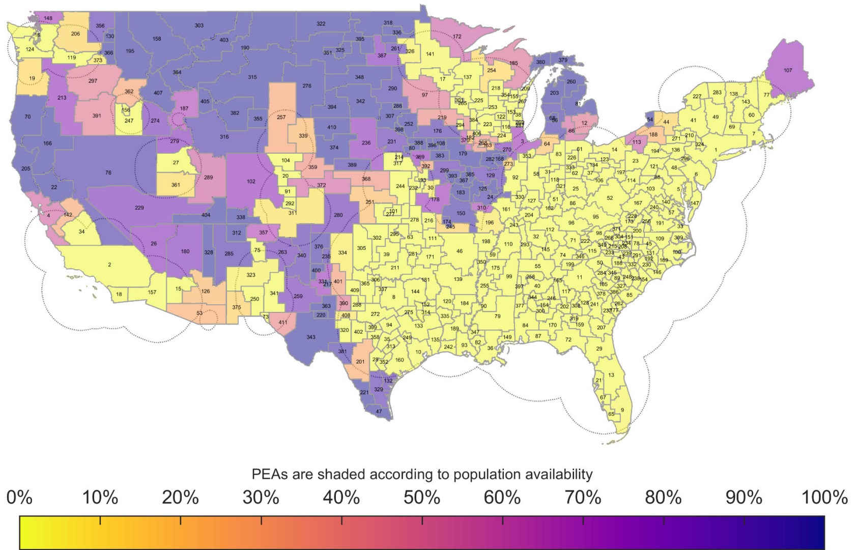
Figure 109. BS Dynamic Coordination Zone Neighborhood Population Availability BS EIRP: 47 dBm/10 MHz, AP EIRP: 36 dBm/10 MHz 100 Megahertz Sharing Option, IMT-Advanced Deployment
