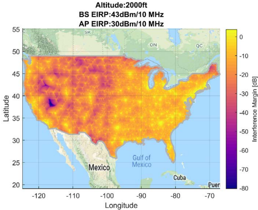
Figure 12. Airborne 1-2: Geographical Interference Margin 30 Megahertz Sharing Option, 2,000ft (AGL) Altitude
