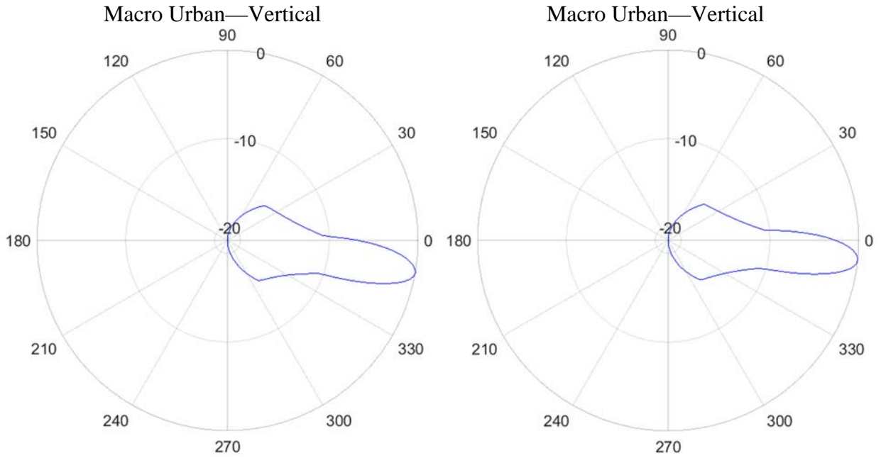
Figure 2. Urban and Suburban Vertical Antenna Gain Pattern (showing downtilt)
