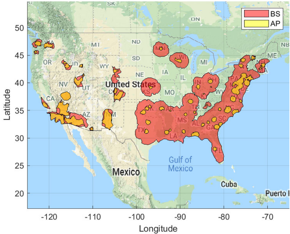
Figure 30. Ground Based Exclusion Zone: BS EIRP: 47 dBm/10 MHz, AP EIRP: 30 dBm/10 MHz 100 Megahertz Sharing Option and Population Deployment
