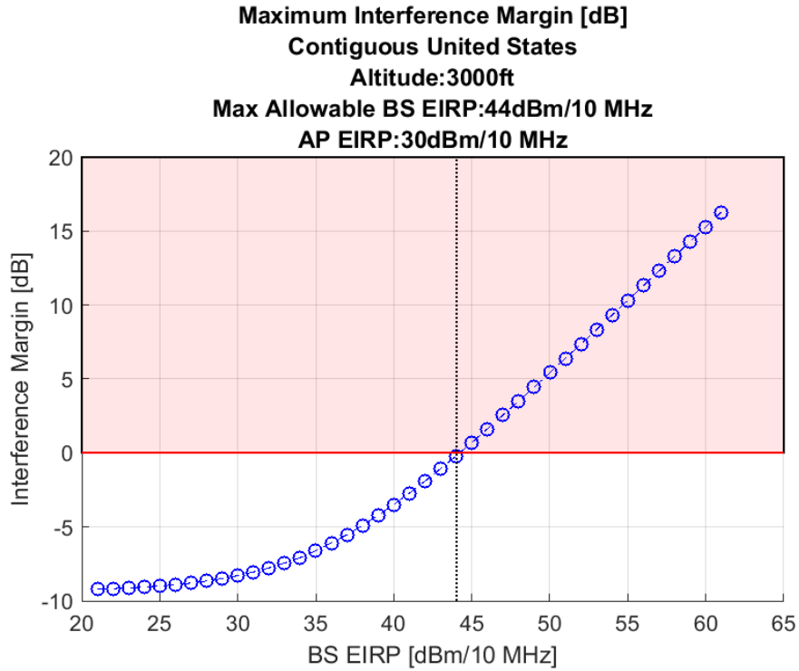
Figure 13. Airborne 1-2: Maximum Allowable EIRP 30 Megahertz Sharing Option, 3,000 ft (AGL) Altitude
