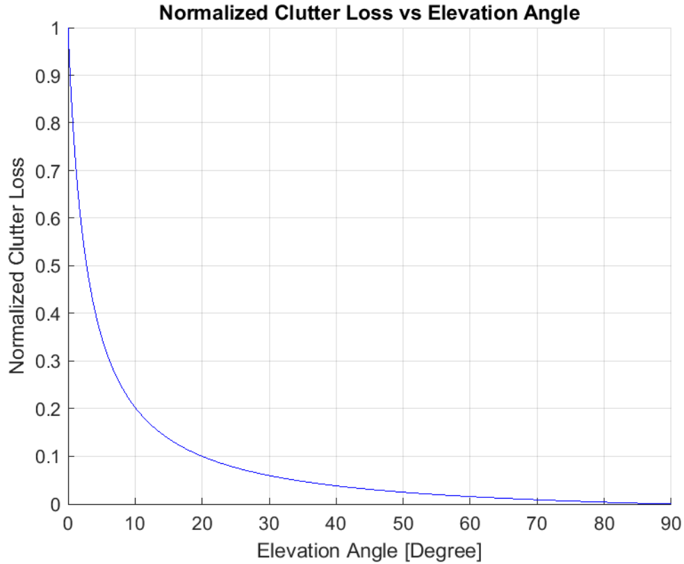
Figure 9. Normalized Clutter Loss Constant
