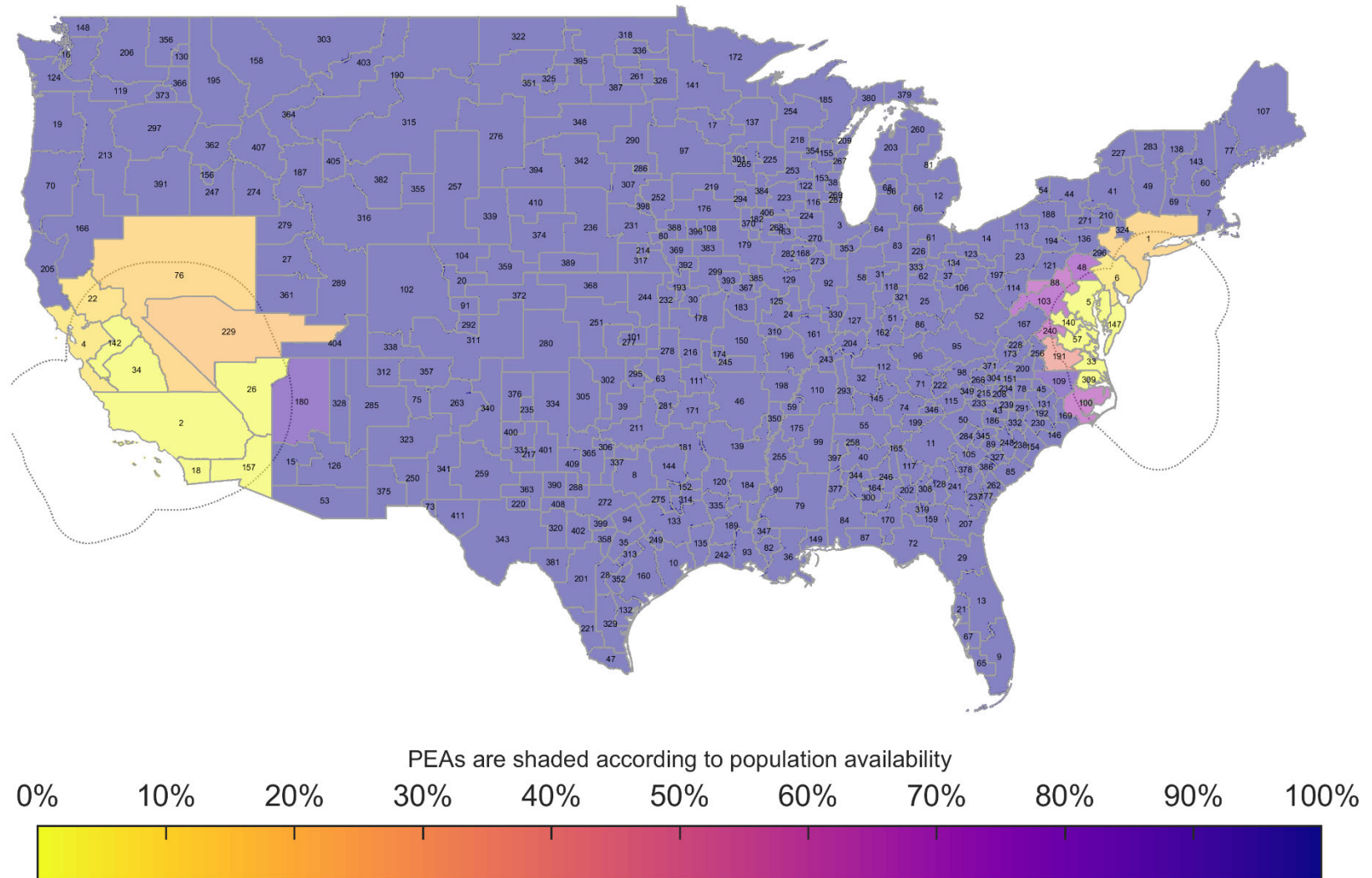
Figure 59. BS Dynamic Coordination Zone Neighborhood Population Availability BS EIRP: 47 dBm/10 MHz, AP EIRP: 30 dBm/10 MHz 100 Megahertz Sharing Option, IMT-Advanced Deployment
