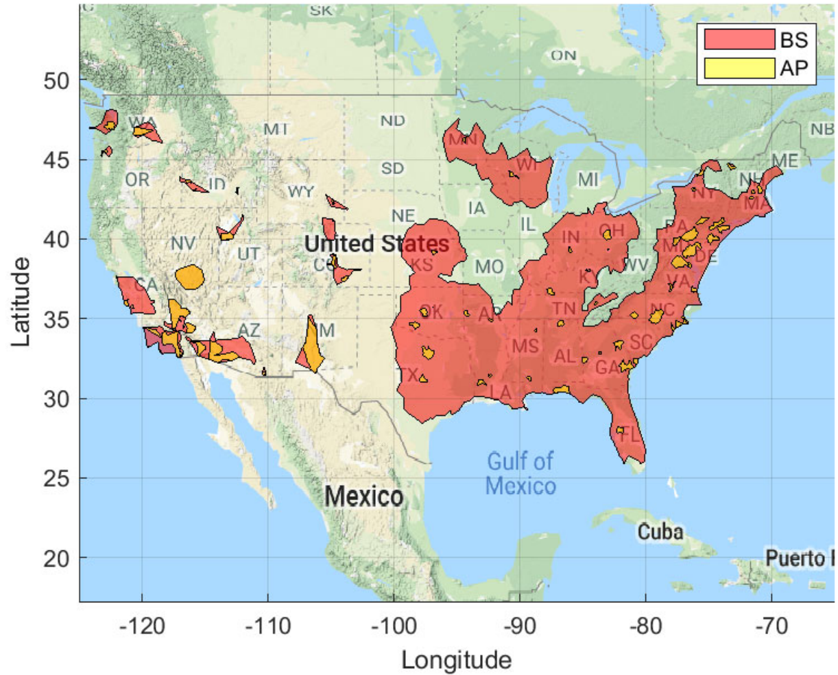
Figure 33. Ground Based Exclusion Zone: BS EIRP: 47 dBm/10 MHz, AP EIRP: 30 dBm/10 MHz 100 Megahertz Sharing Option and IMT-Advanced Deployment
