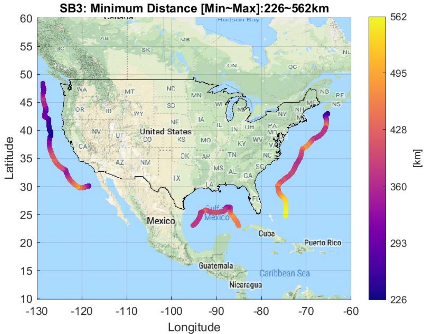
Figure 131. Minimum Distance: BS EIRP: 61 dBm/10 MHz, AP EIRP: 47 dBm/10 MHz Population Deployment
