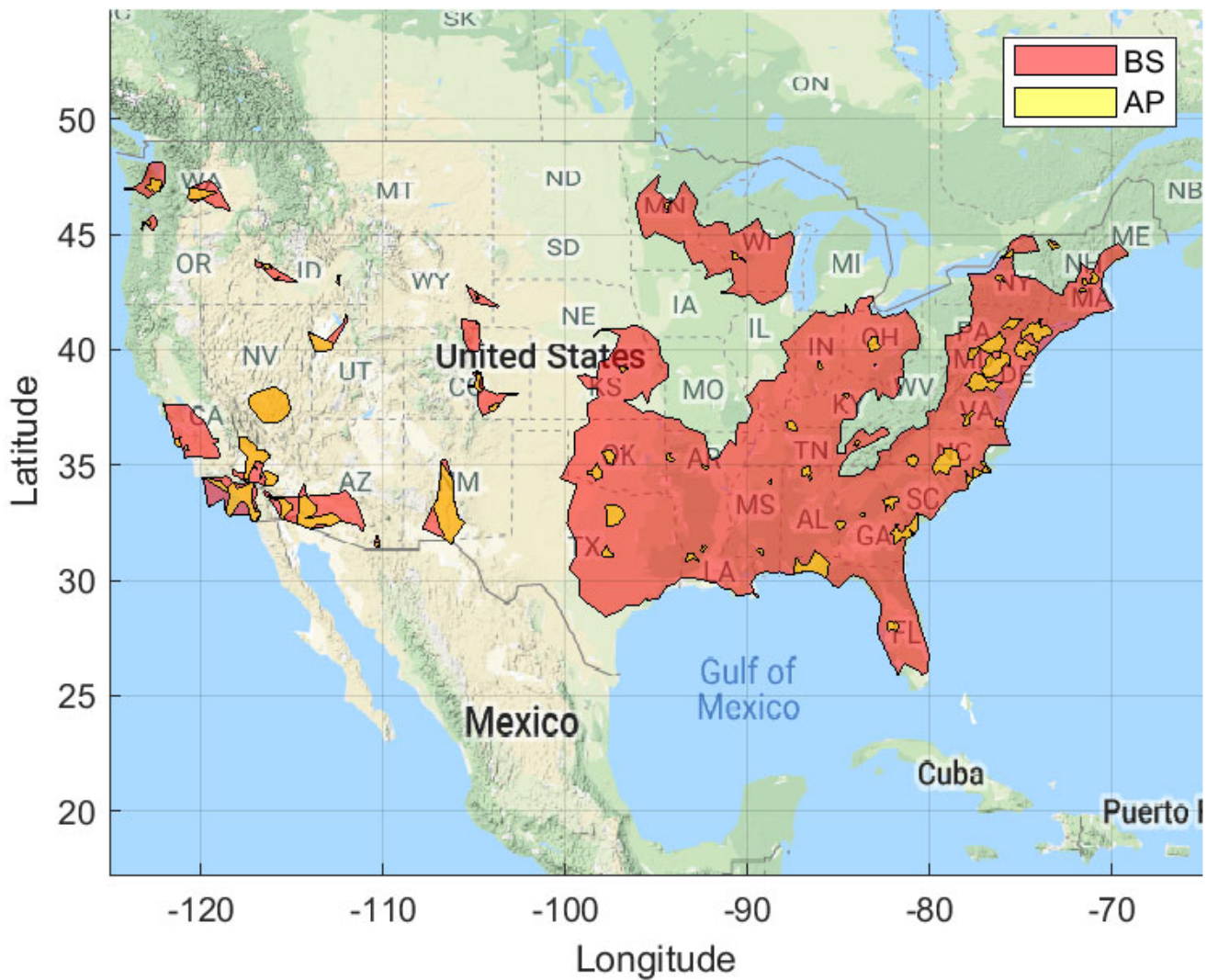
Figure 34. Ground Based Exclusion Zone: BS EIRP: 47 dBm/10 MHz, AP EIRP: 36 dBm/10 MHz 100 Megahertz Sharing Option and IMT-Advanced Deployment
