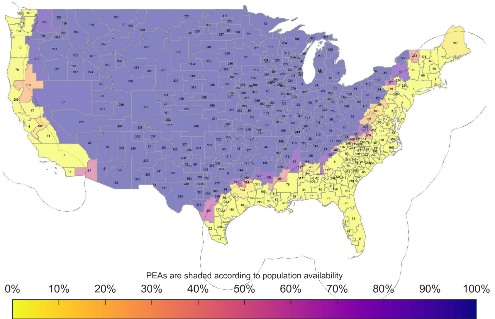
Figure 145. BS Dynamic Coordination Zone Neighborhood Population Availability BS EIRP: 47 dBm/10 MHz, AP EIRP: 36 dBm/10 MHz Population Deployment
