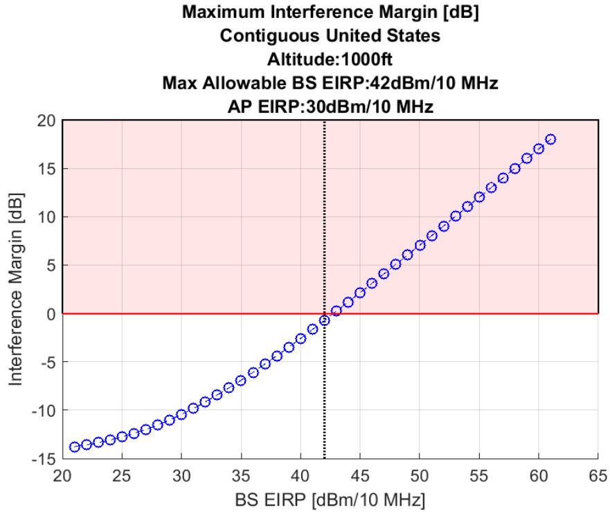
Figure 5. Airborne 1-2: Maximum Allowable EIRP 30 Megahertz Sharing Option, 1,000 ft (AGL) Altitude
