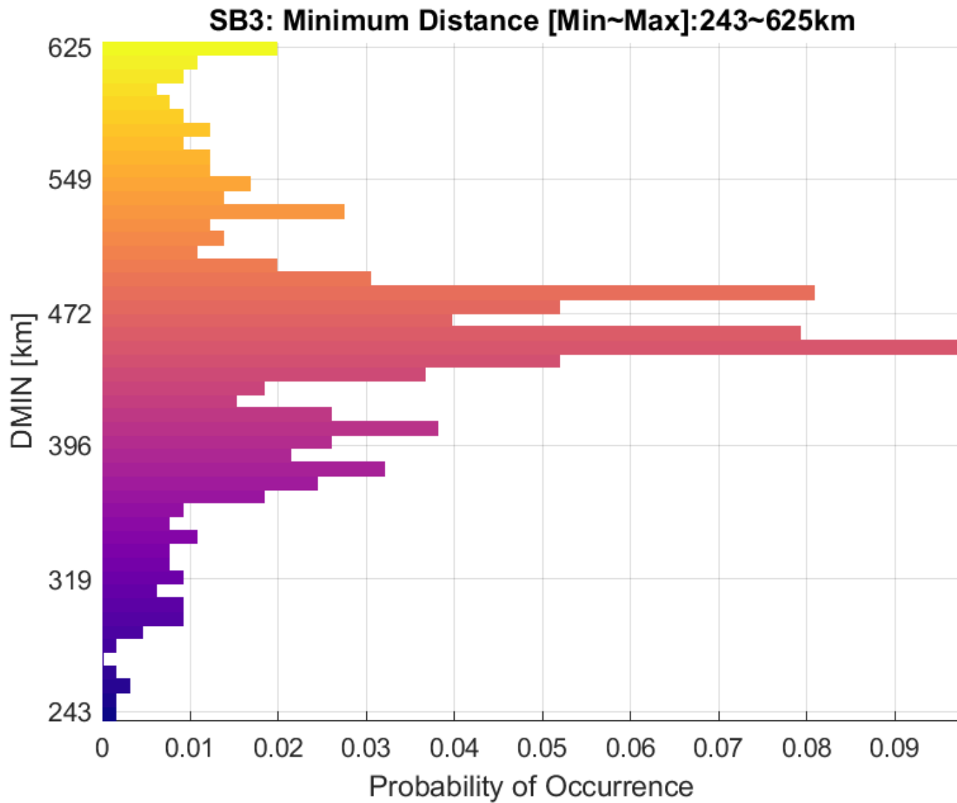
Figure 141. Minimum Distance Distribution: BS EIRP: 61 dBm/10 MHz, AP EIRP: 47 dBm/10 MHz IMT-Advanced Deployment
