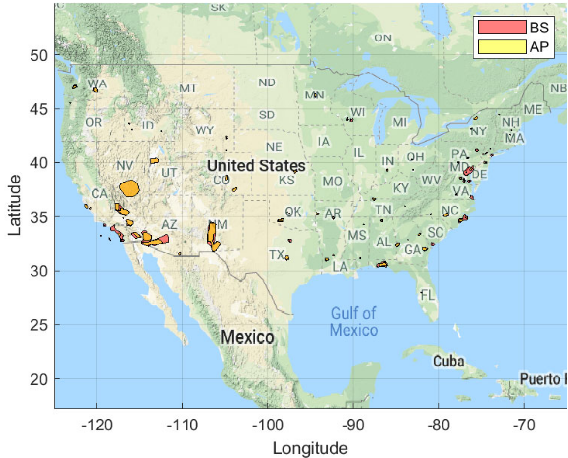
Figure 24. Ground Based Exclusion Zone: BS EIRP: 47 dBm/10 MHz, AP EIRP: 30 dBm/10 MHz 30 Megahertz Sharing Option and Population Deployment
