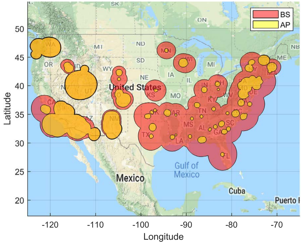
Figure 44. Ground Based Dynamic Coordination Zone Neighborhood: BS EIRP: 47 dBm/10 MHz, AP EIRP: 30 dBm/10 MHz 100 Megahertz Sharing Option and Population Deployment
