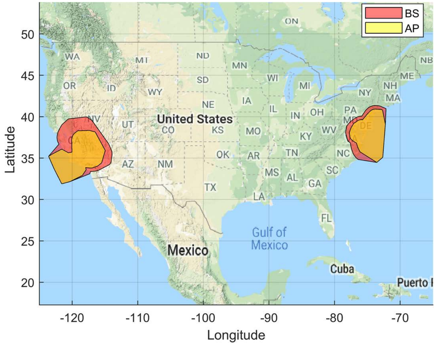
Figure 12. Airborne 3 Exclusion Zone: BS EIRP: 61 dBm/10 MHz, AP EIRP: 47 dBm/10 MHz 100 Megahertz Sharing Option and Population Deployment
