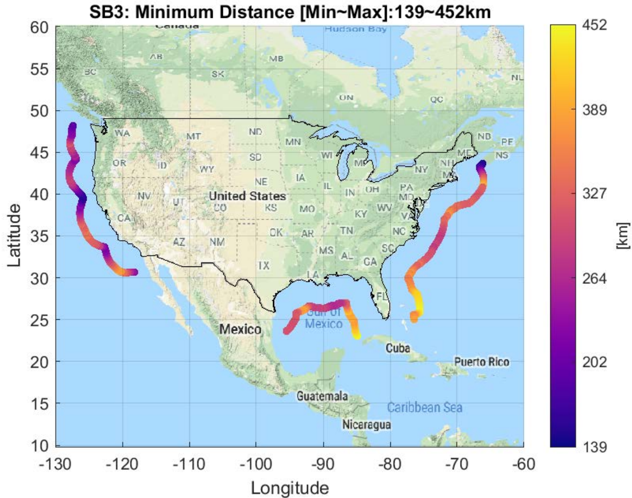
Figure 134. Minimum Distance: BS EIRP: 47 dBm/10 MHz, AP EIRP: 30 dBm/10 MHz IMT-Advanced Deployment
