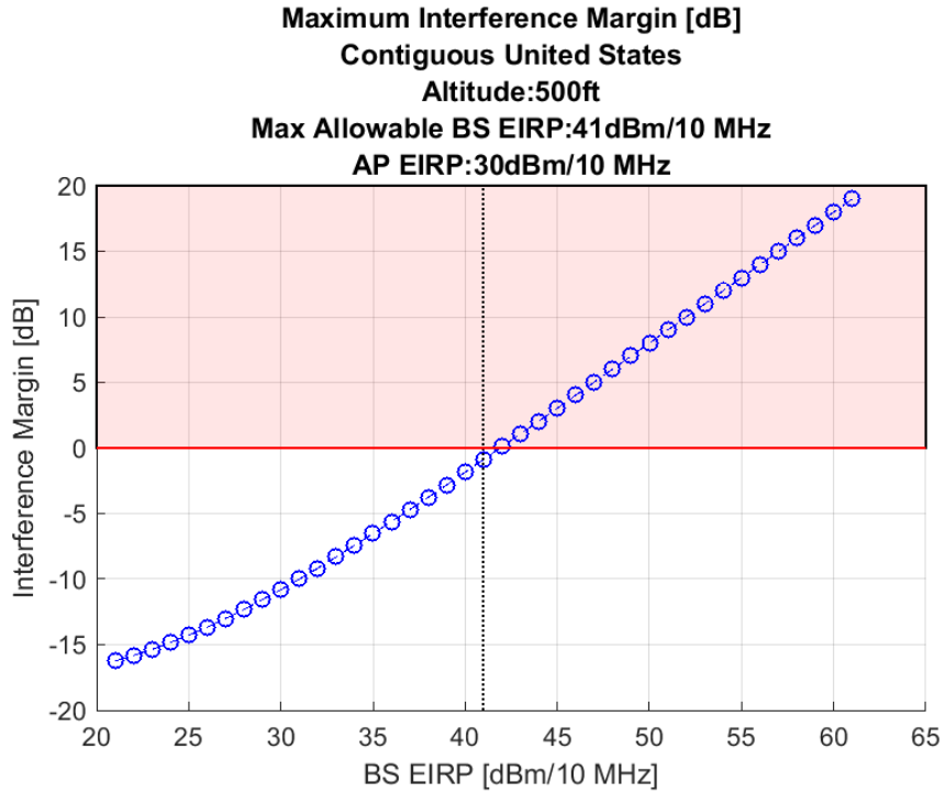
Figure 1. Airborne 1-2: Maximum Allowable EIRP 30 Megahertz Sharing Option, 500 ft (AGL) Altitude
