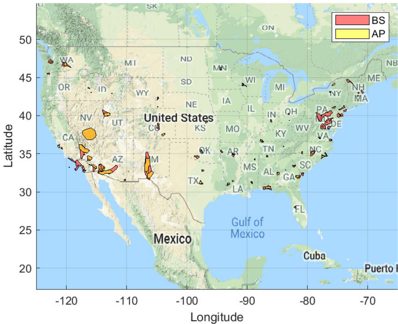
Figure 29. Ground Based Exclusion Zone: BS EIRP: 61 dBm/10 MHz, AP EIRP: 47 dBm/10 MHz 30 Megahertz Sharing Option and IMT-Advanced Deployment
