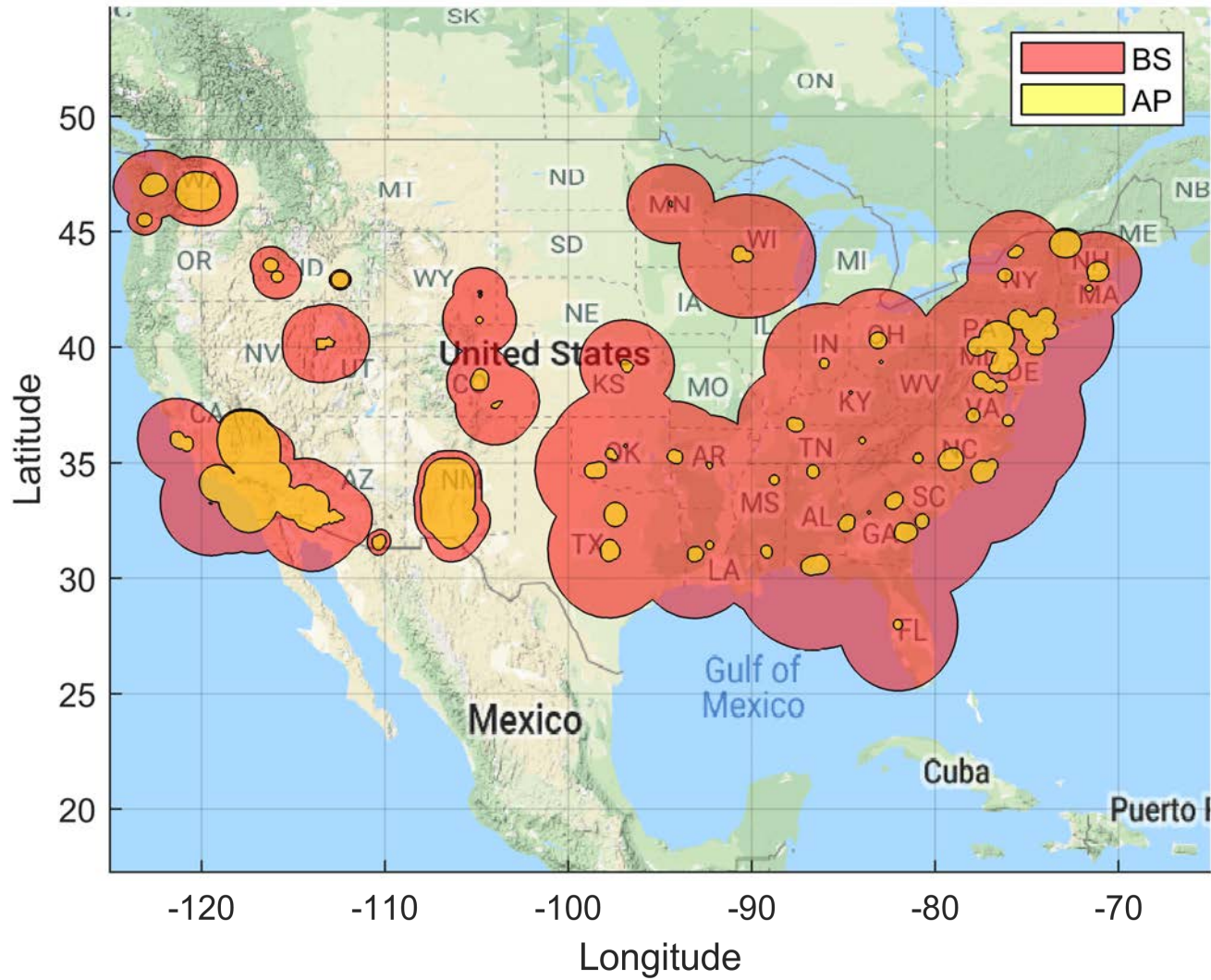
Figure 47. Ground Based Dynamic Coordination Zone Neighborhood: BS EIRP: 47 dBm/10 MHz, AP EIRP: 30 dBm/10 MHz 100 Megahertz Sharing Option and IMT-Advanced Deployment
