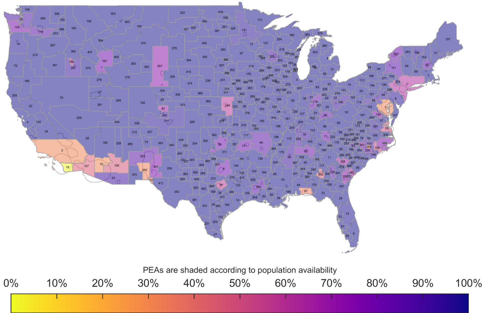
Figure 89. BS Dynamic Coordination Zone Neighborhood Population Availability BS EIRP: 47 dBm/10 MHz, AP EIRP: 30 dBm/10 MHz 30 Megahertz Sharing Option, Population Deployment
