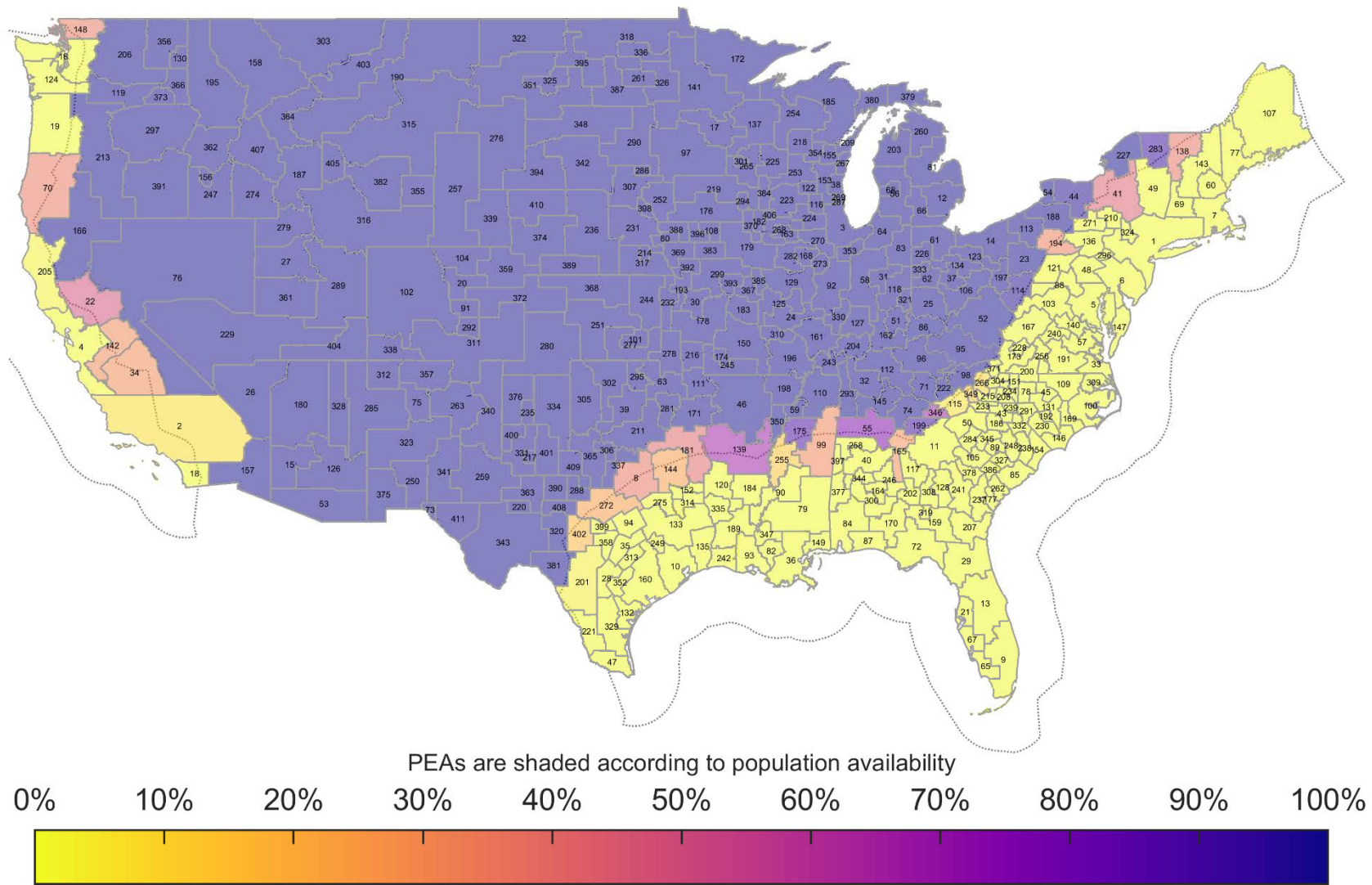
Figure 117. BS Shipborne Exclusion Zone Population Availability: BS EIRP: 61 dBm/10 MHz, AP EIRP: 47 dBm/10 MHz Population Deployment
