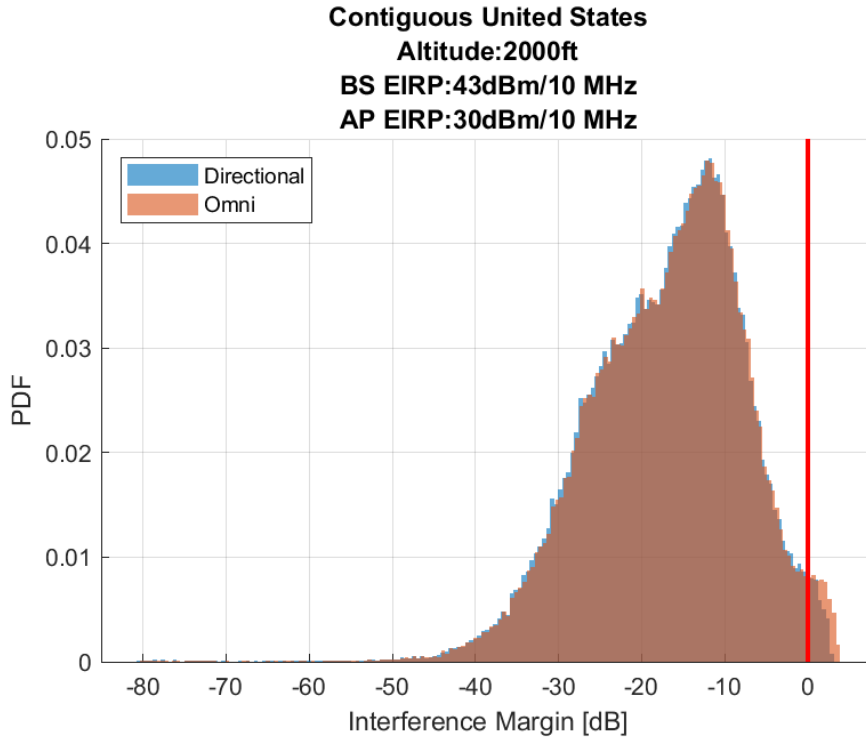
Figure 10. Airborne 1-2: Probability Distribution Function of the Interference Margin 30 Megahertz Sharing Option, 2,000ft (AGL) Altitude
