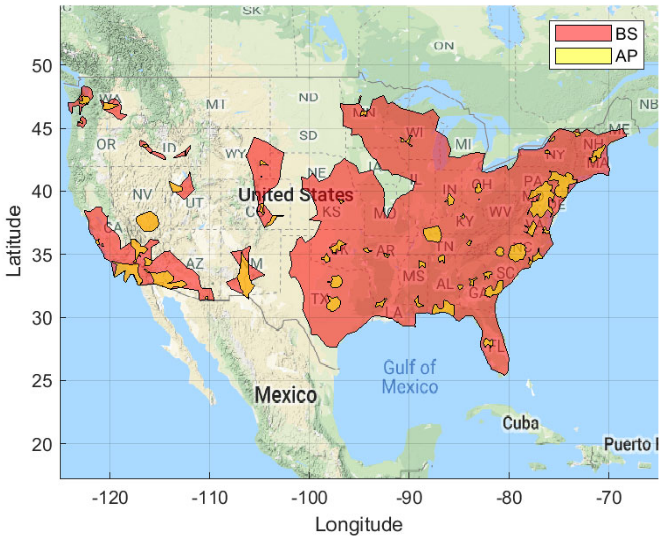
Figure 35. Ground Based Exclusion Zone: BS EIRP: 61 dBm/10 MHz, AP EIRP: 47 dBm/10 MHz 100 Megahertz Sharing Option and IMT-Advanced Deployment
