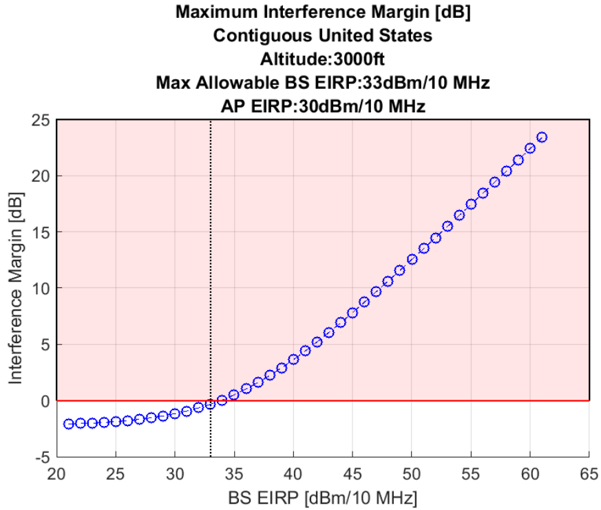
Figure 33. Airborne 1-2: Maximum Allowable EIRP 100 Megahertz Sharing Option, 3,000 ft (AGL) Altitude
