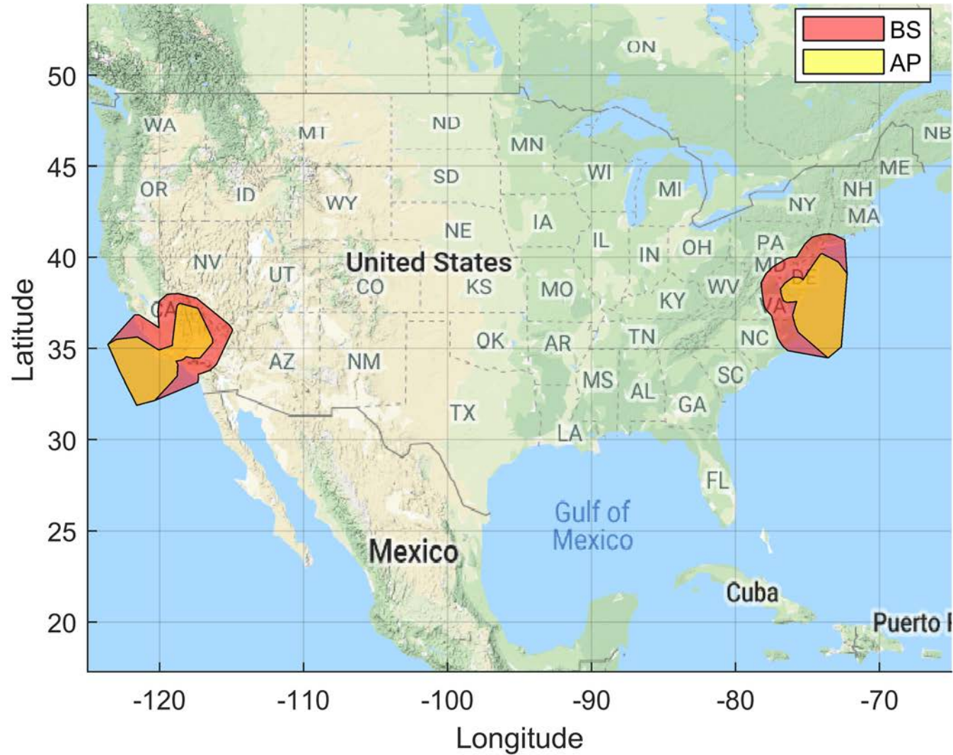
Figure 10. Airborne 3 Exclusion Zone: BS EIRP: 47 dBm/10 MHz, AP EIRP: 30 dBm/10 MHz 100 Megahertz Sharing Option and Population Deployment
