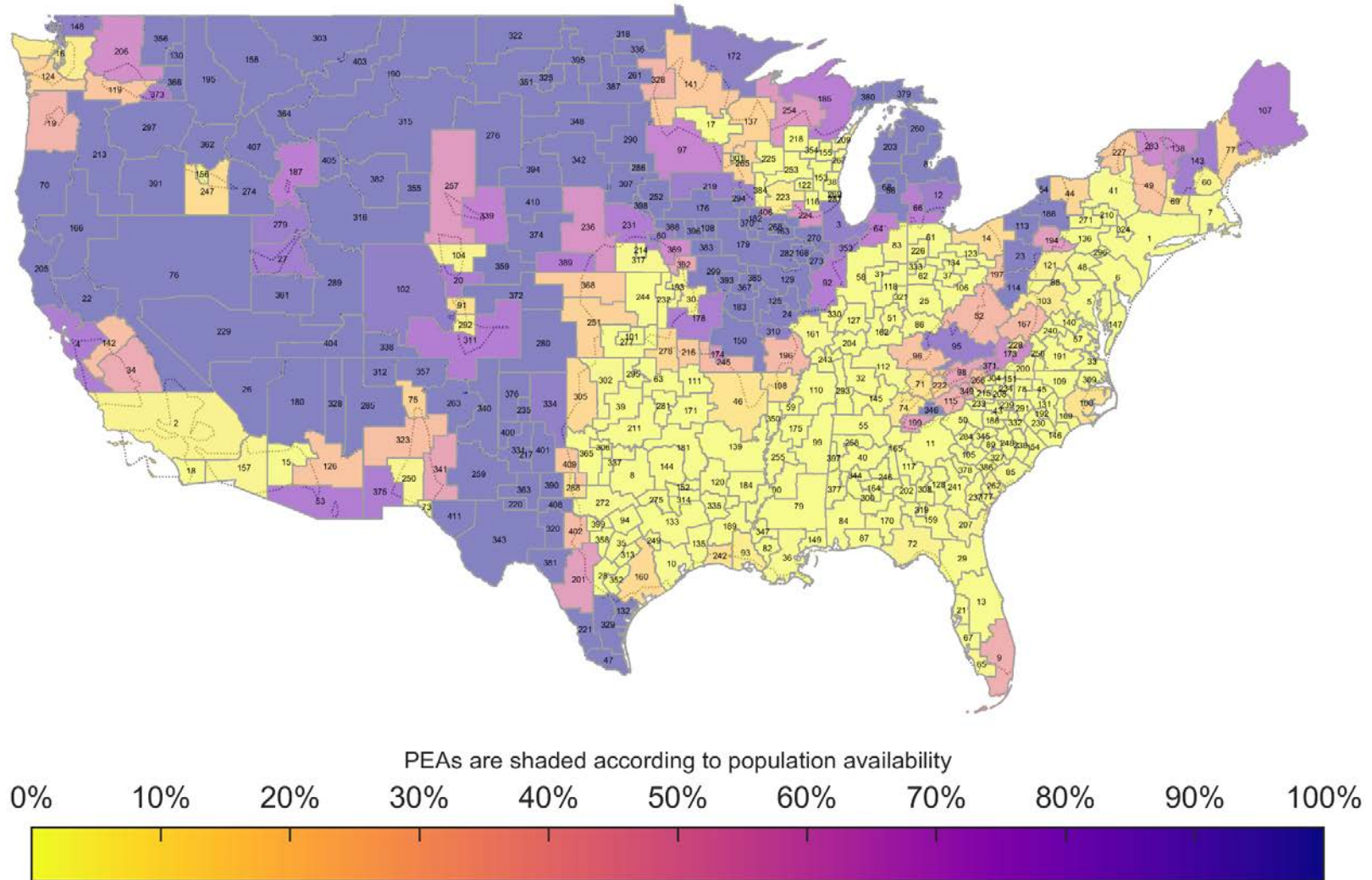
Figure 83. BS Ground Based Exclusion Zone Population Availability: BS EIRP: 47 dBm/10 MHz, AP EIRP: 30 dBm/10 MHz 100 Megahertz Sharing Option, IMT-Advanced Deployment
