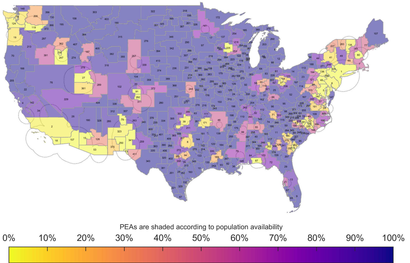
Figure 104. AP Dynamic Coordination Zone Neighborhood Population Availability BS EIRP: 47 dBm/10 MHz, AP EIRP: 36 dBm/10MHz 100 Megahertz Sharing Option, Population Deployment
