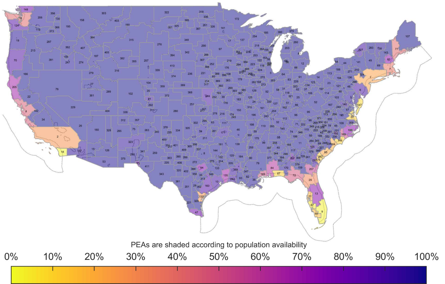
Figure 73. IMT-Advanced Deployment Accessibility: AP EIRP: 30 dBm/10 MHz 30 Megahertz Sharing Option
