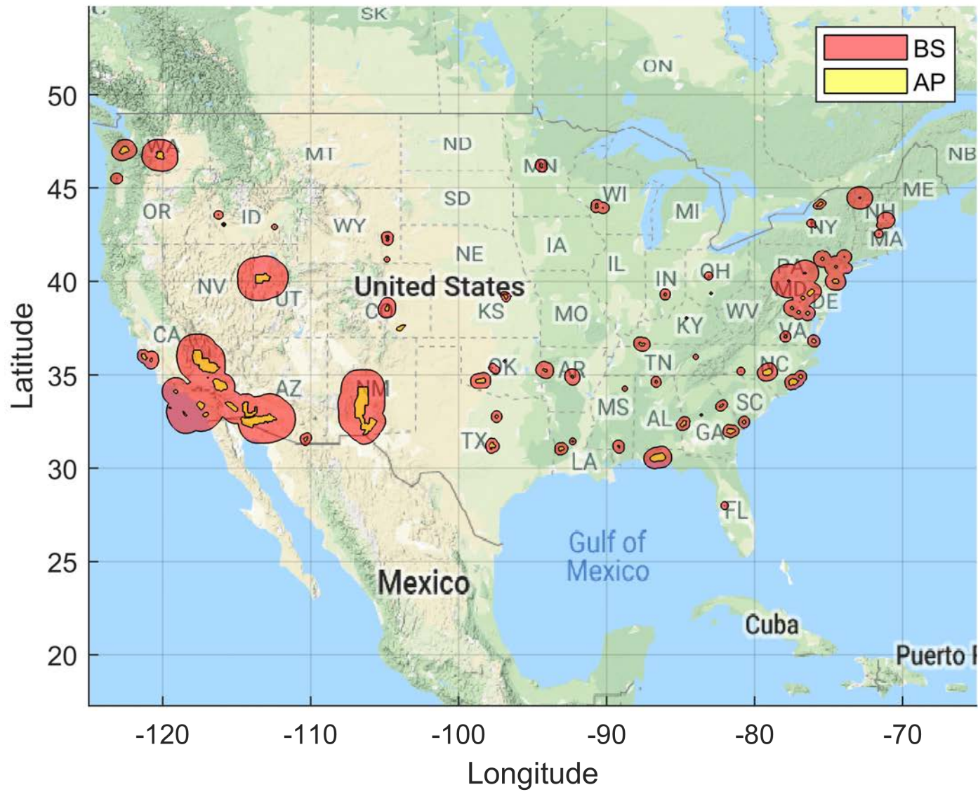
Figure 43. Ground Based Dynamic Coordination Zone Neighborhood: BS EIRP: 61 dBm/10 MHz, AP EIRP: 47 dBm/10 MHz 30 Megahertz Sharing Option and IMT-Advanced Deployment
