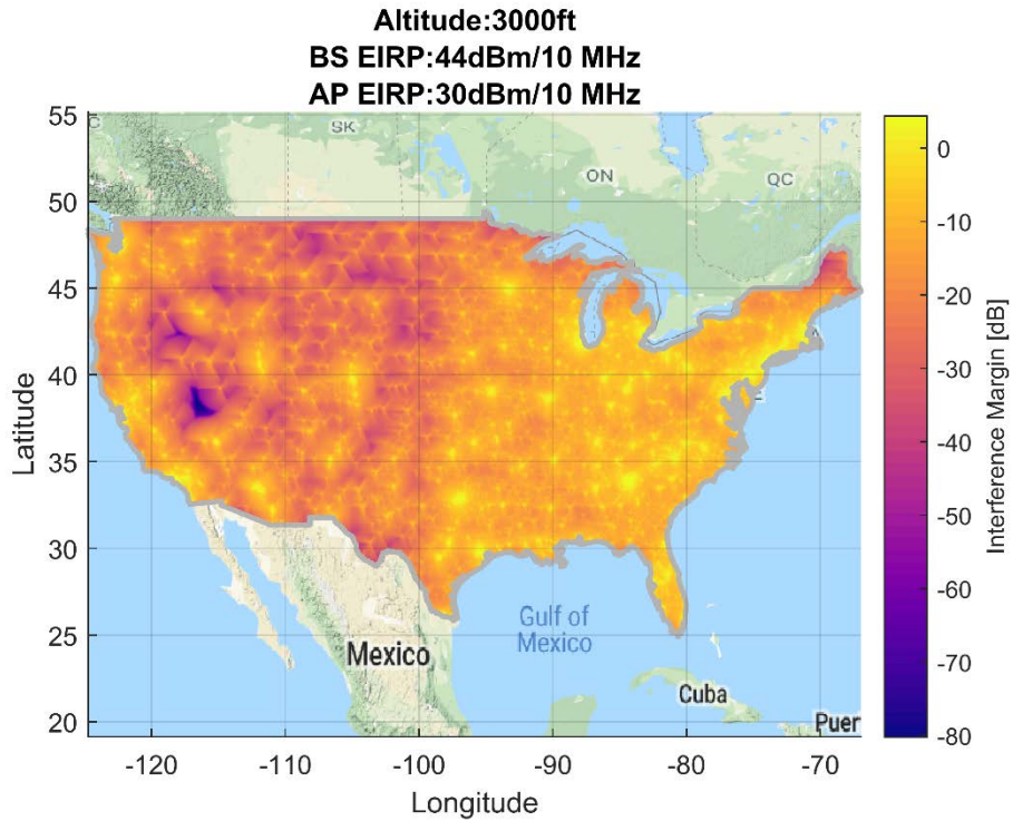
Figure 16. Airborne 1-2: Geographical Interference Margin 30 Megahertz Sharing Option, 3,000ft (AGL) Altitude
