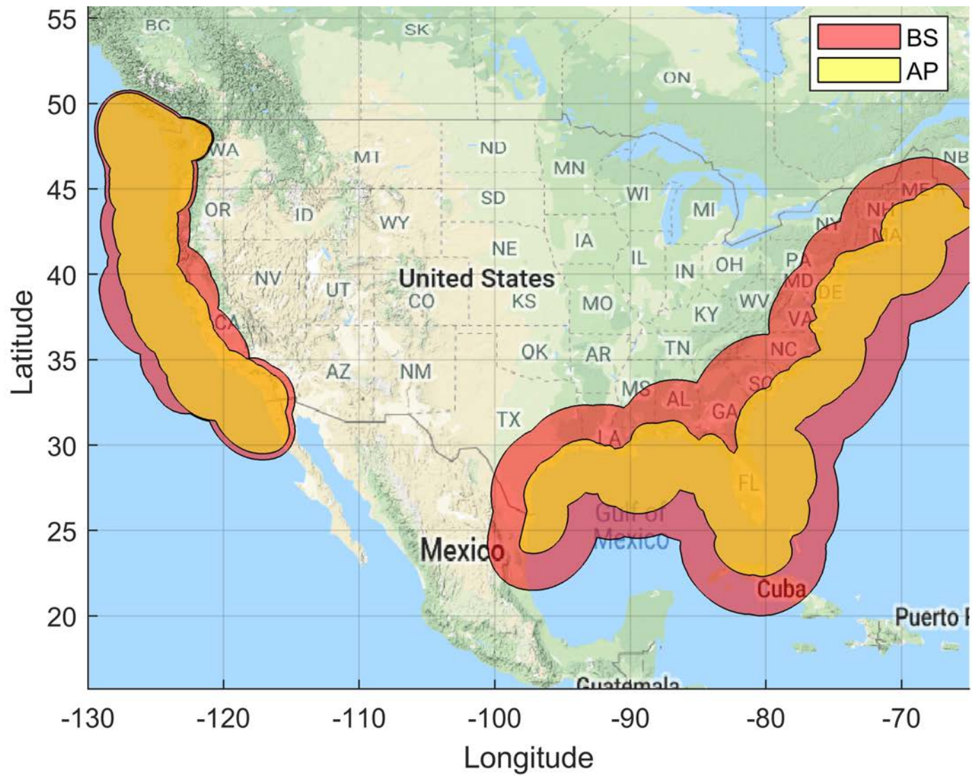
Figure 61. Shipborne Dynamic Coordination Zone Neighborhood: BS EIRP: 47 dBm/10 MHz, AP EIRP: 36 dBm/10 MHz Population Deployment
