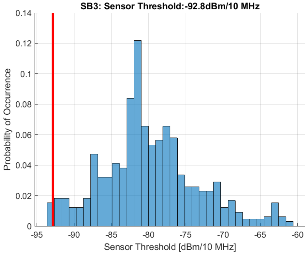
Figure 136. Sensor Detection Threshold BS EIRP: 47 dBm/10 MHz, AP EIRP: 30 dBm/10 MHz IMT-Advanced Deployment
