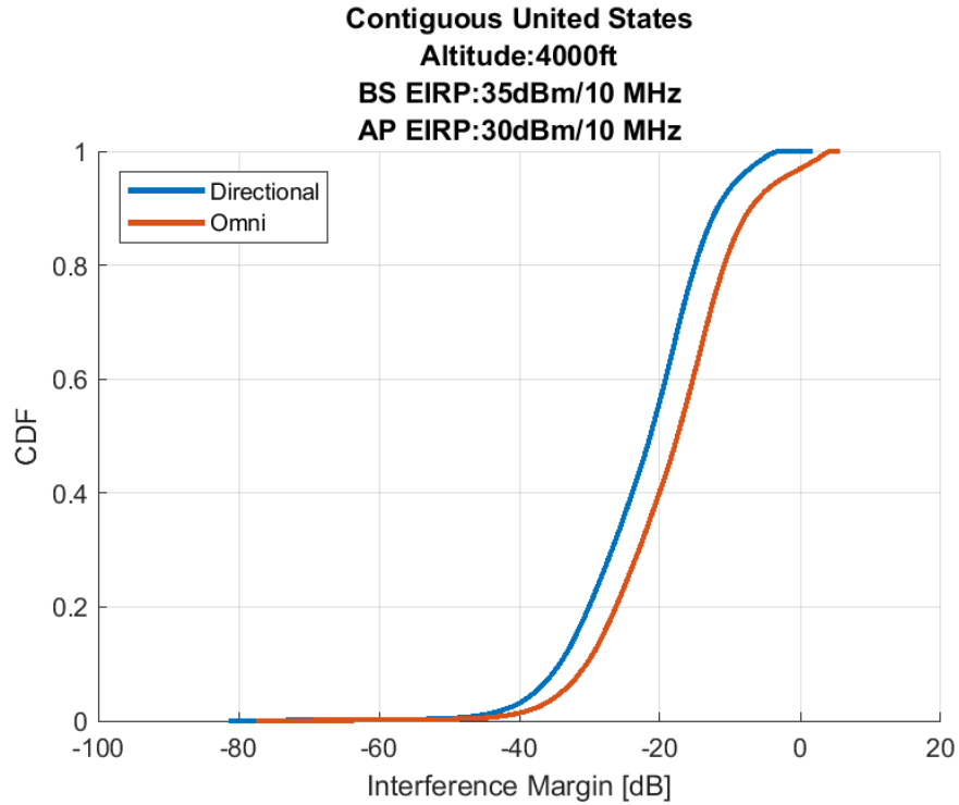
Figure 39. Airborne 1-2: Cumulative Distribution Function of the Interference Margin 100 Megahertz Sharing Option, 4,000ft (AGL) Altitude
