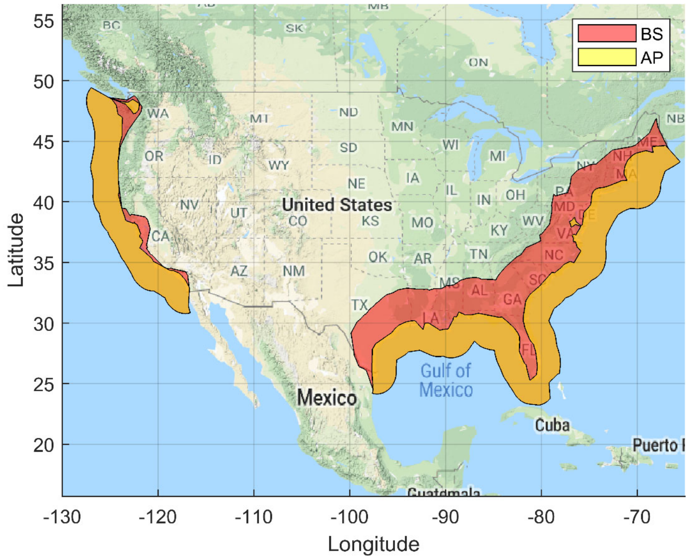
Figure 54. Shipborne Exclusion Zone: BS EIRP: 47 dBm/10 MHz, AP EIRP: 36 dBm/10 MHz IMT-Advanced Deployment
