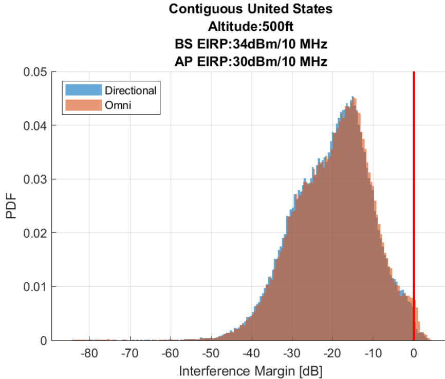
Figure 22. Airborne 1-2: Probability Distribution Function of the Interference Margin 100 Megahertz Sharing Option, 500 ft (AGL) Altitude
