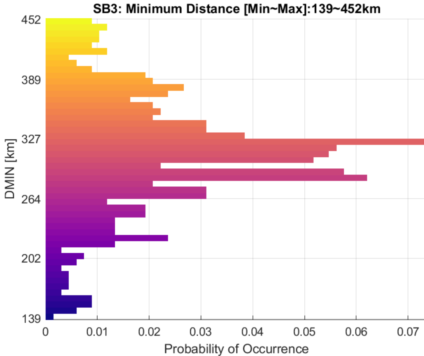
Figure 135. Minimum Distance Distribution: BS EIRP: 47 dBm/10 MHz, AP EIRP: 30 dBm/10 MHz IMT-Advanced Deployment
