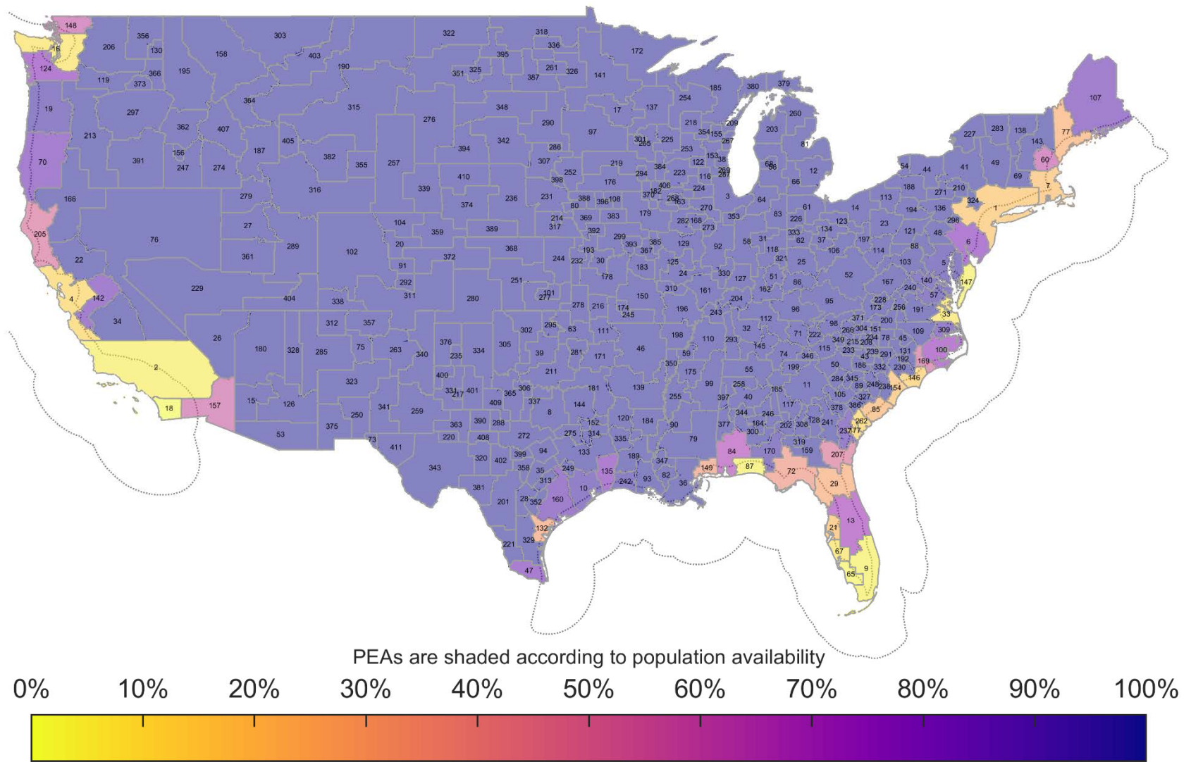
Figure 150. AP Dynamic Coordination Zone Neighborhood Population Availability: BS EIRP:47 dBm/10 MHz, AP EIRP: 30 dBm/10 MHz IMT-Advanced Deployment
