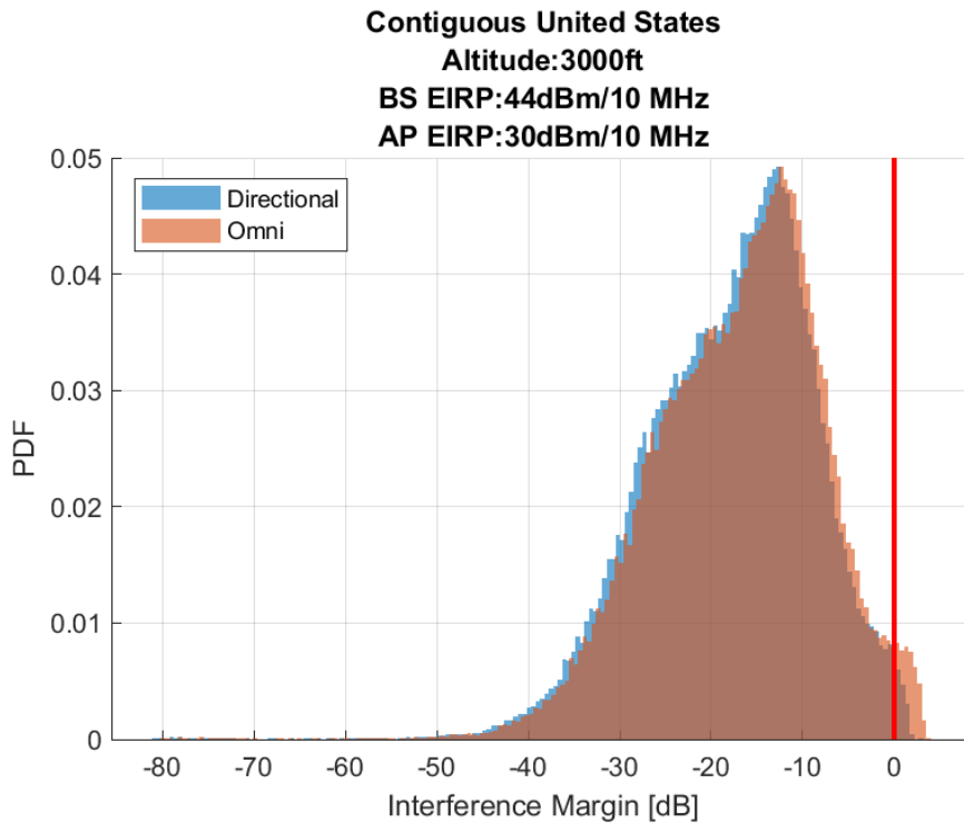
Figure 14. Airborne 1-2: Probability Distribution Function of the Interference Margin 30 Megahertz Sharing Option, 3,000ft (AGL) Altitude
