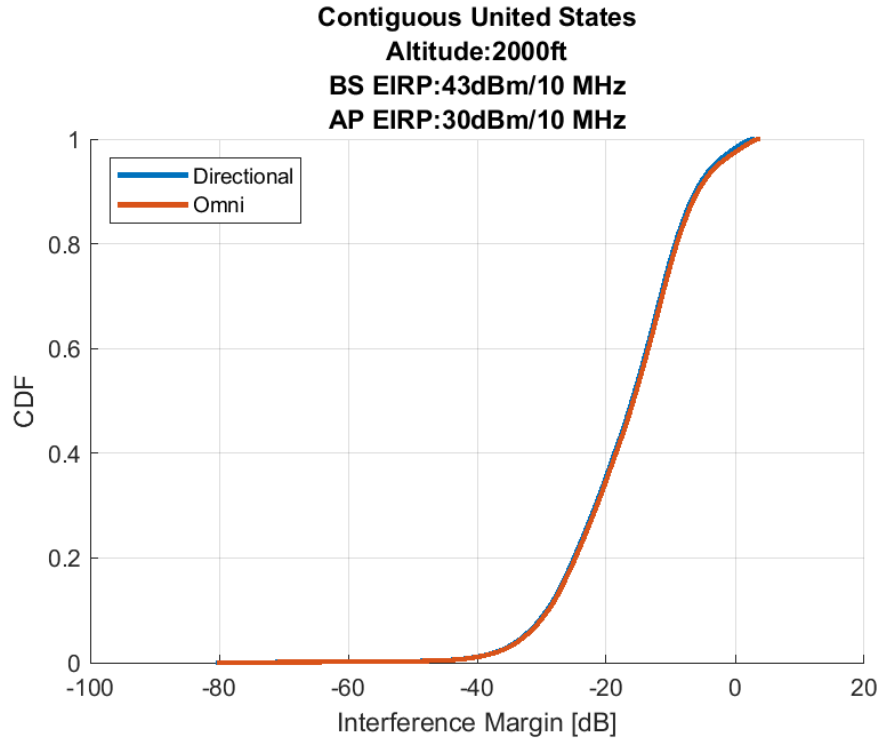
Figure 11. Airborne 1-2: Cumulative Distribution Function of the Interference Margin 30 Megahertz Sharing Option, 2,000ft (AGL) Altitude
