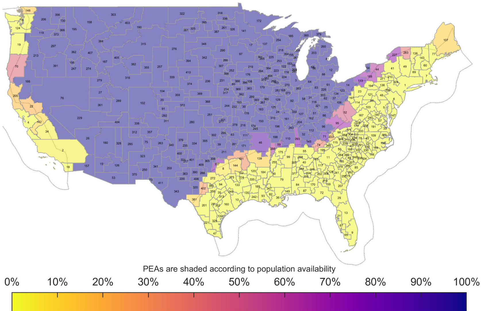
Figure 123. BS Shipborne Exclusion Zone Population Availability: BS EIRP: 61 dBm/10 MHz, AP EIRP: 47 dBm/10 MHz IMT-Advanced Deployment
