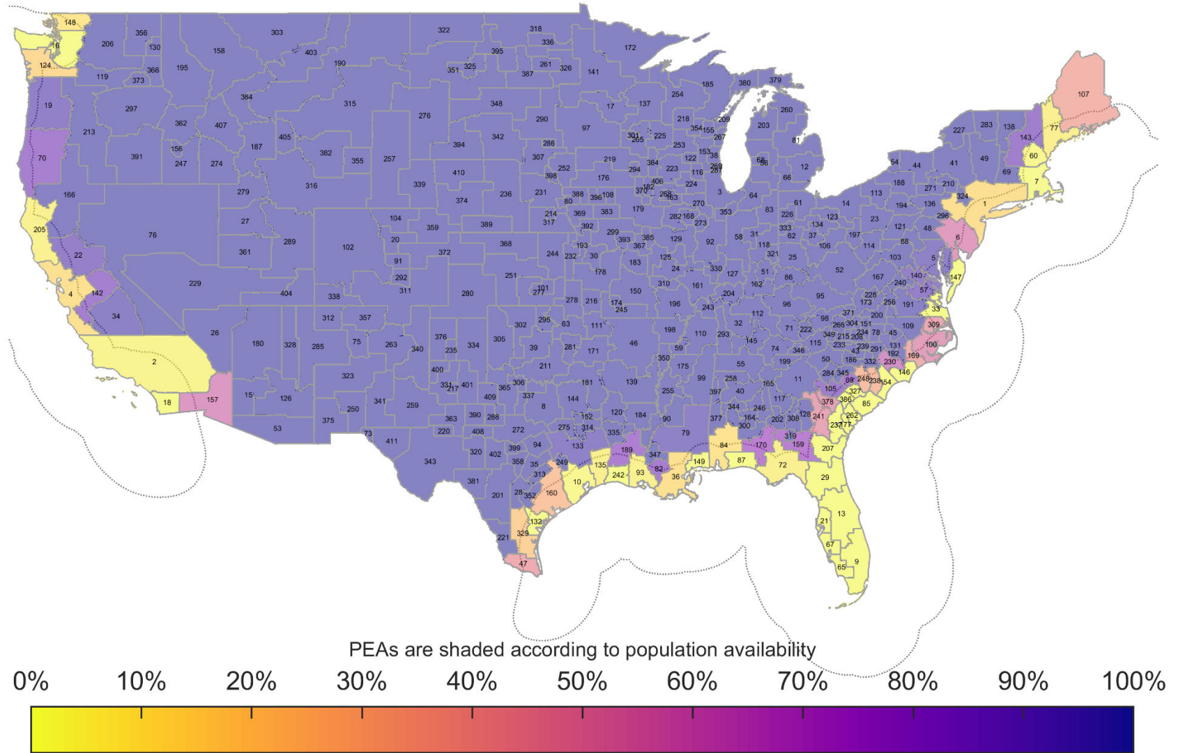
Figure 154. AP Dynamic Coordination Zone Neighborhood Population Availability: BS EIRP: 61 dBm/10 MHz, AP EIRP: 47 dBm/10MHz IMT-Advanced Deployment
