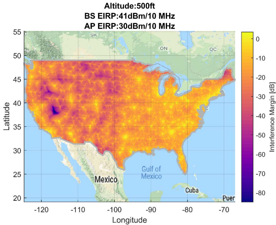
Figure 4. Airborne 1-2: Geographical Interference Margin 30 Megahertz Sharing Option, 500 ft (AGL) Altitude
