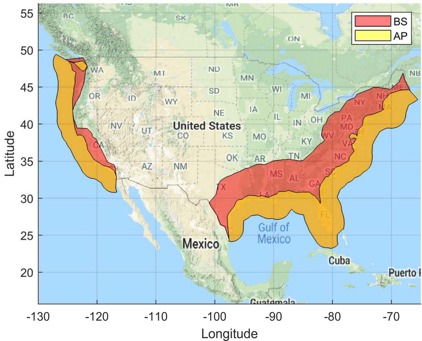
Figure 55. Shipborne Exclusion Zone: BS EIRP: 61 dBm/10 MHz, AP EIRP: 47 dBm/10 MHz IMT-Advanced Deployment
