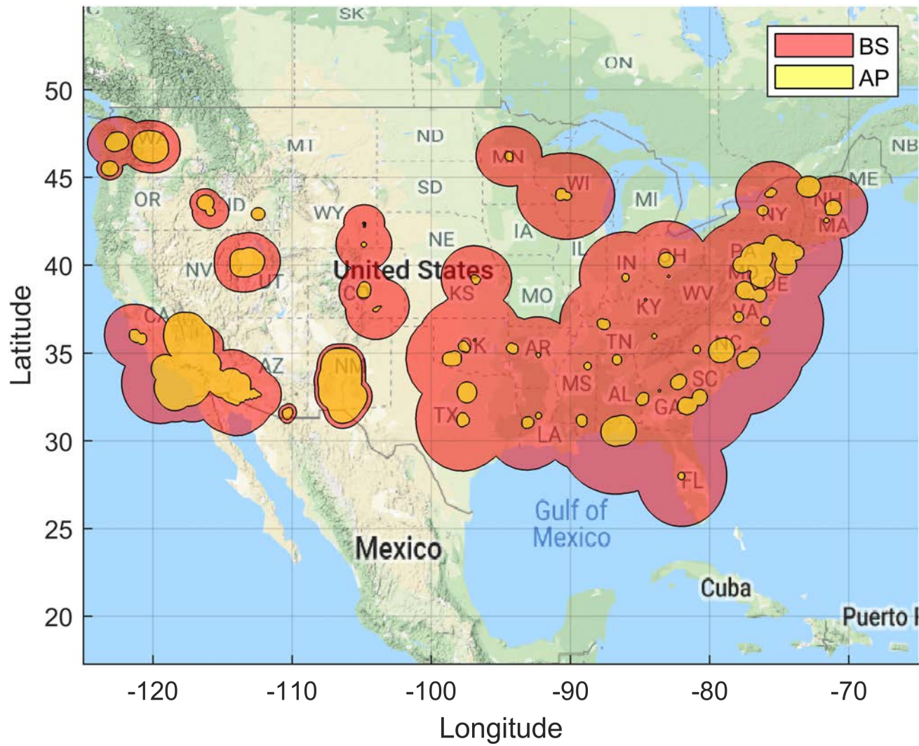
Figure 48. Ground Based Dynamic Coordination Zone Neighborhood: BS EIRP: 47 dBm/10 MHz, AP EIRP: 36 dBm/10 MHz 100 Megahertz Sharing Option and IMT-Advanced Deployment
