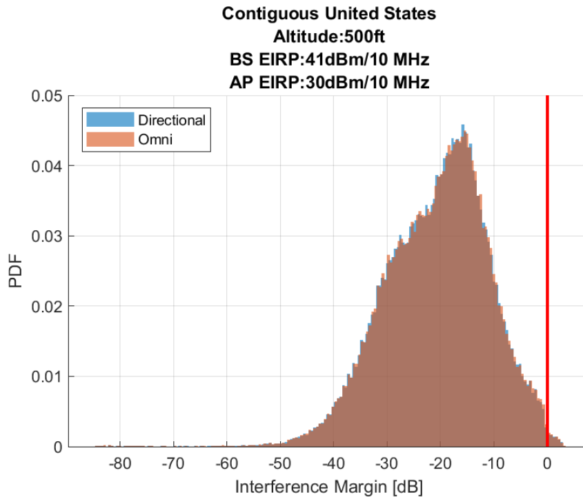
Figure 2. Airborne 1-2: Probability Distribution Function of the Interference Margin 30 Megahertz Sharing Option, 500 ft (AGL) Altitude
