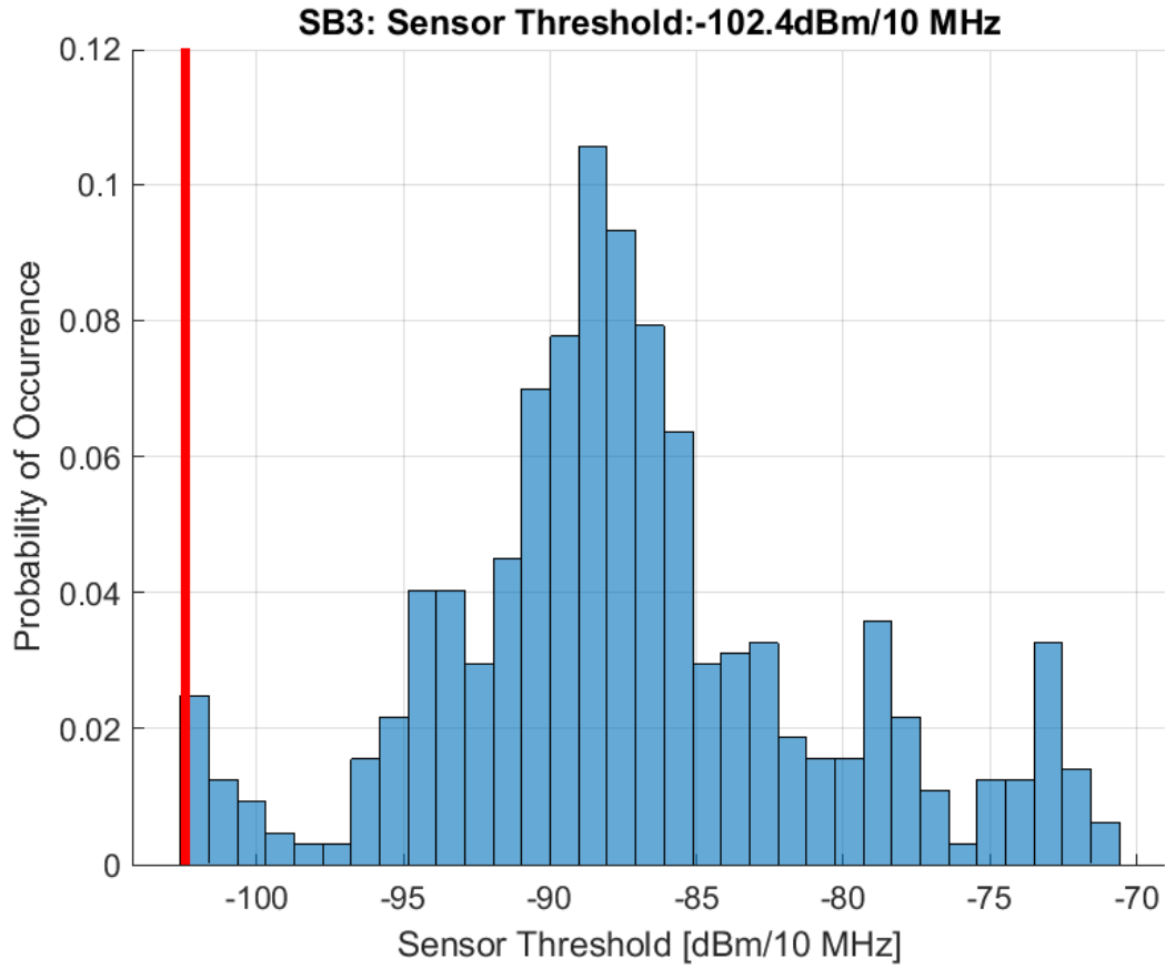
Figure 133. Sensor Detection Threshold BS EIRP: 61 dBm/10 MHz, AP EIRP: 47 dBm/10 MHz Population Deployment
