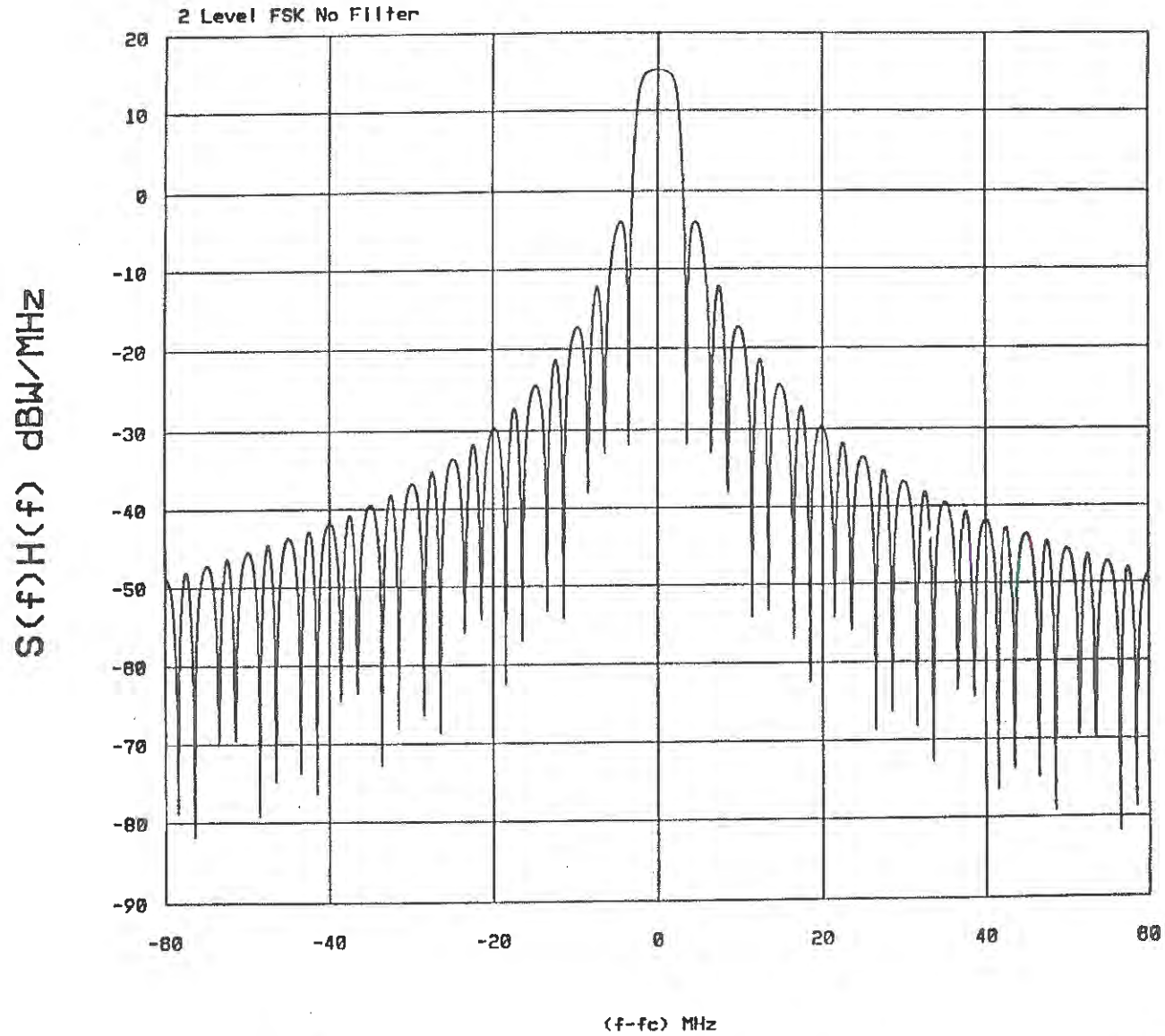
Figure 2-19. Power spectral density two level FSK.
