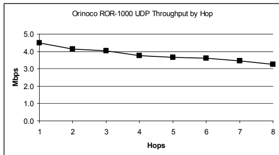
Figure 11 Average UDP throughput at each hop illustrating throughput degradation
