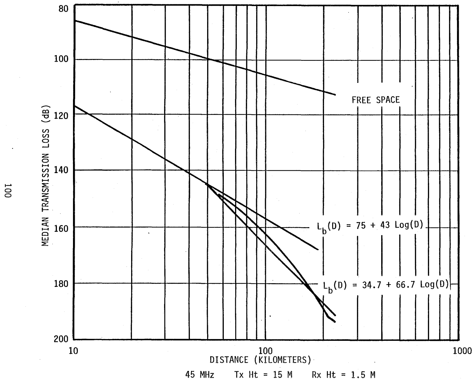
Figure E-3. Propagation Model for (a) Mobile Interference to a Meteor Burst Receiver, (b) Meteor Burst Transmitted Signal Received by a Cordless Telephone.
