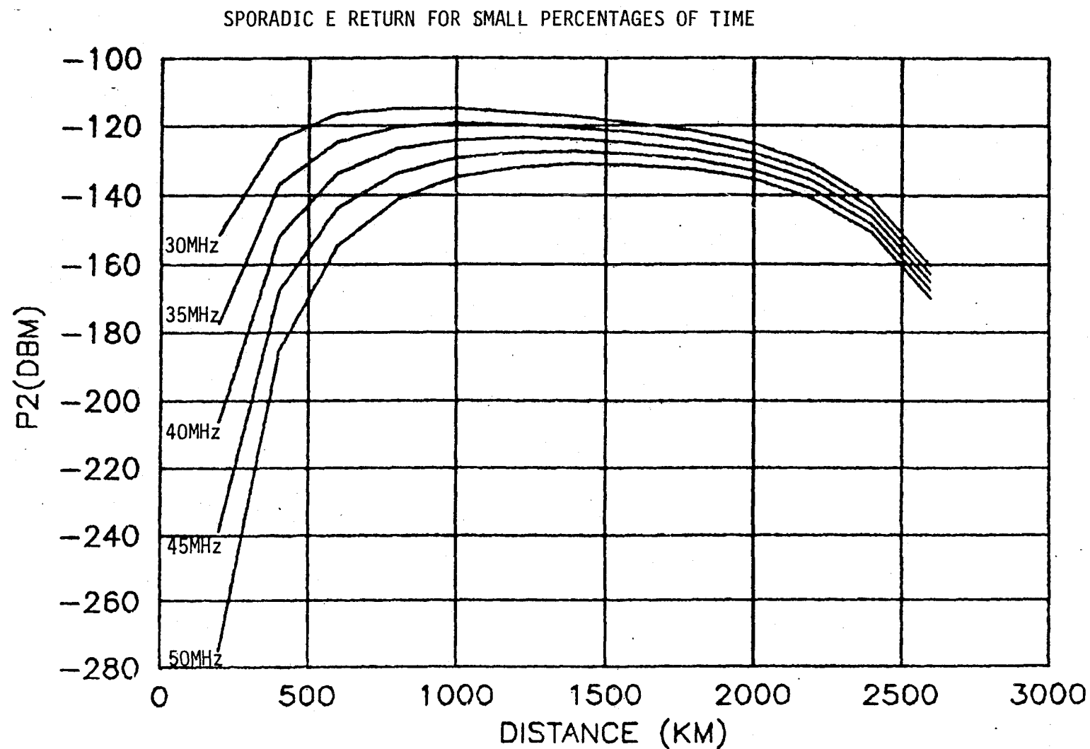
Figure 3. Received power vs. distance separation between transmitter and receiver. 10,000 watt transmitter G_T = G_R = 10 dBi, ionosphere f_0 = 13 MHz
