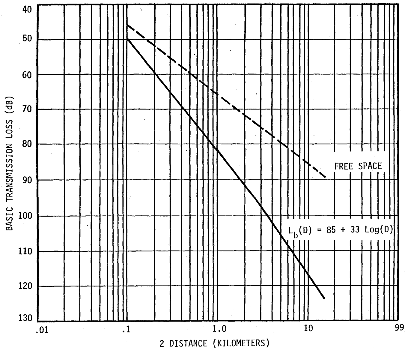
Figure E-4. Propagation Model for a Cordless Telephone Signal Interference to a Meteor Burst Receiver.
