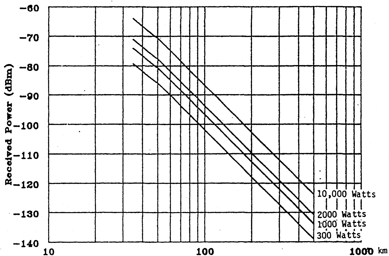
Figure 21. Received Power from Meteor Burst Transmitter, Sidelobe to Sidelobe, Meteor Burst to Meteor Burst.
