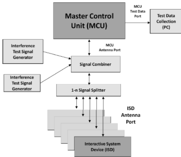
Figure 7. Test Set-Up.
