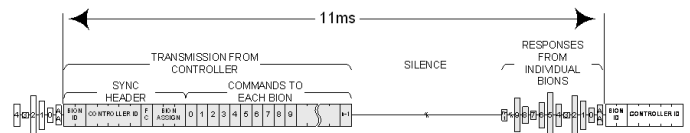
Figure 6. MMN Frame format.
