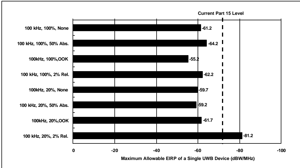
Figure 4-5. Maximum Allowable EIRP as a Function of UWB Signal Structure for the Semi-Codeless Receiver Architecture (Pulse-Like UWB Signals)
