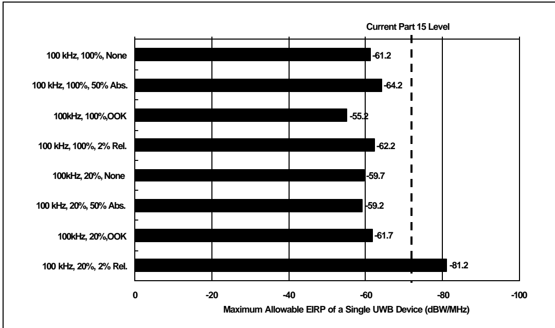
Figure 5. Maximum Allowable EIRP as a Function of UWB Signal Structure for the Semi-Codeless Receiver Architecture (Pulse-Like UWB Signals)
