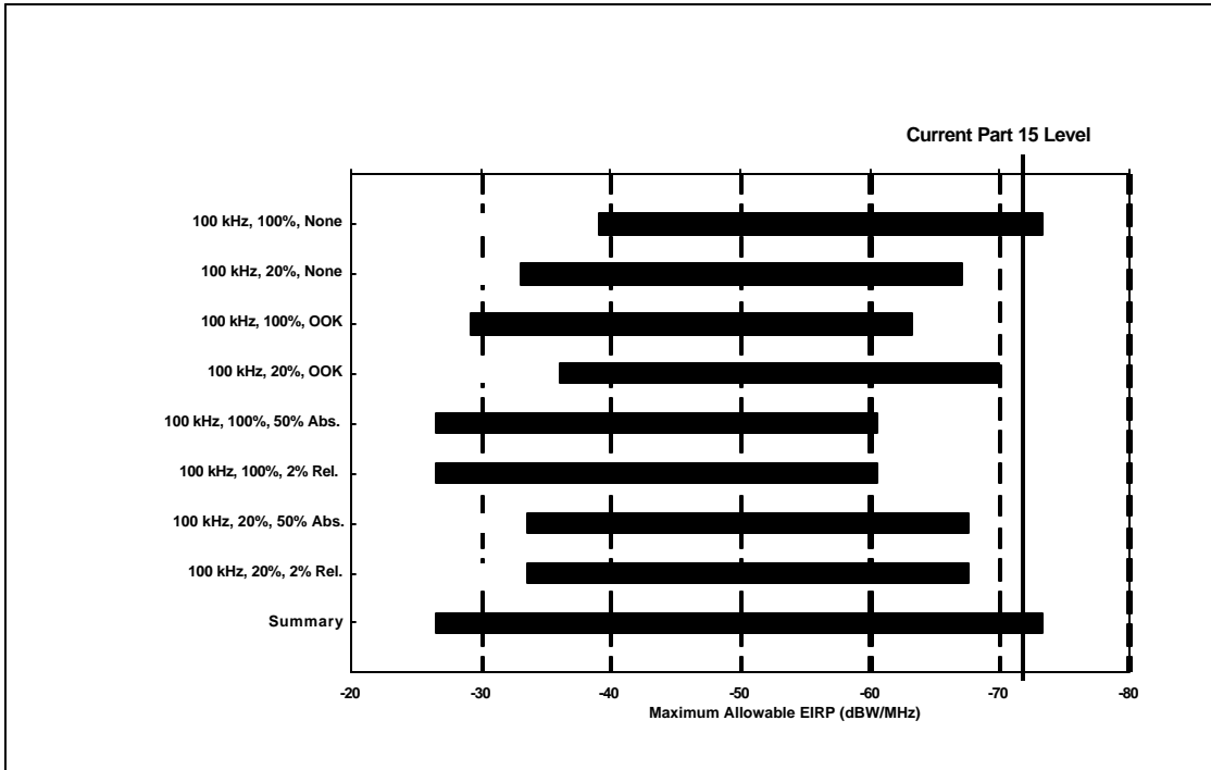
Figure 4-2. Range of Maximum Allowable EIRP for Pulse-Like UWB Signal Structures for the C/A-code Receiver Architecture (Multiple UWB Device Operational Scenarios)
