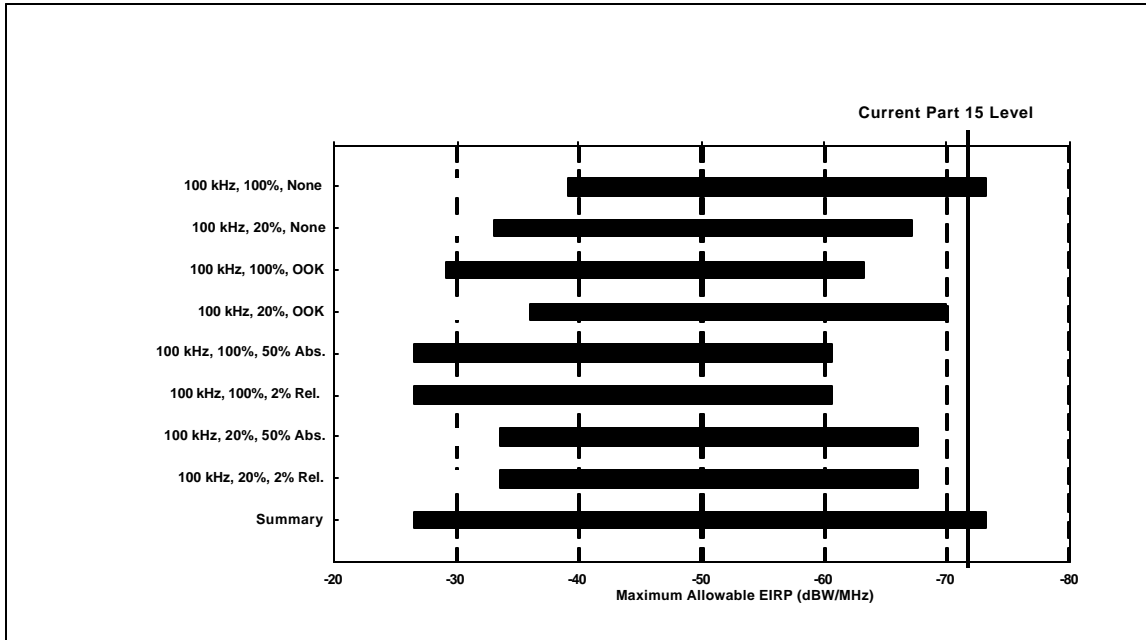
Figure 1. Range of Maximum Allowable EIRP for Pulse-Like UWB Signal Structures for the C/A-Code Receiver Architecture (Multiple UWB Device Operational Scenario)
