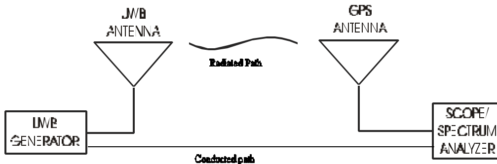
Figure 2-2. Radiated Measurement Test Setup.
