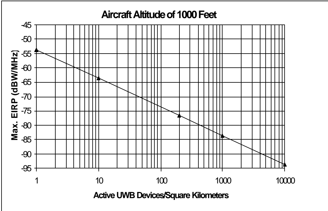
Figure 3-37. Analysis Results for Aviation (En-Route Navigation) Operational Scenario: C/A-code Receiver and Multiple UWB Devices - Outdoor Operation
