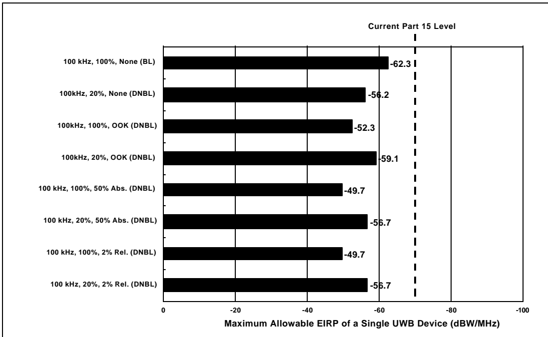
Figure 3-9. Analysis Results for Terrestrial Operational Scenario: C/A-code Receiver and Multiple UWB Devices - Outdoor Operation (Pulse-Like UWB Signals)
