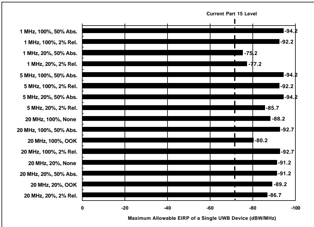
Figure 4-6. Maximum Allowable EIRP as a Function of UWB Signal Structure for the Semi-Codeless Receiver Architecture (Noise-Like UWB Signals)
