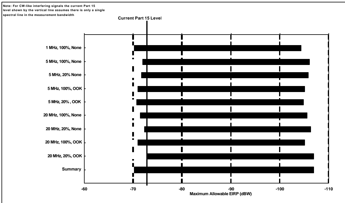
Figure 4-5. Range of Maximum Allowable EIRP for CW-Like UWB Signal Structures for the C/A-code Receiver Architecture (Multiple UWB Device Operational Scenarios)
